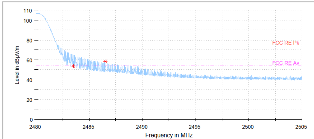
BLE 2Mbps (255 pkt), Highest Channel, Average
