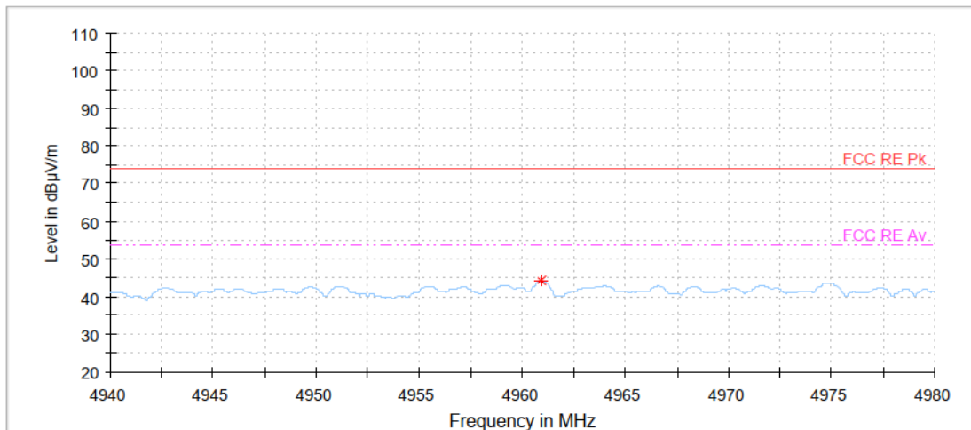
BLE 2Mbps (255 pkt), Highest Channel, Zoom scan, 4 960 MHz, Average
