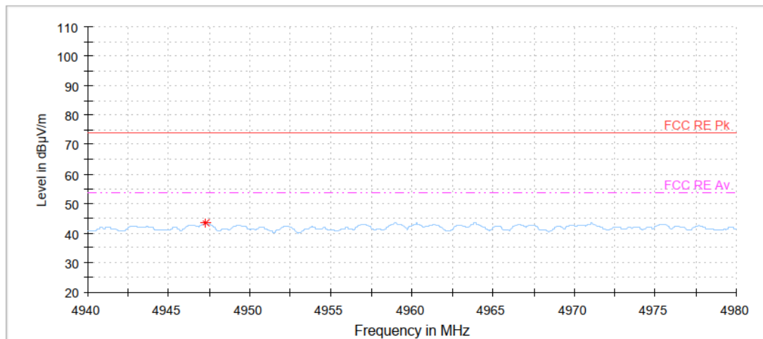
BLE 1Mbps (255 pkt), Highest Channel, Zoom scan, 4 960 MHz, Average
