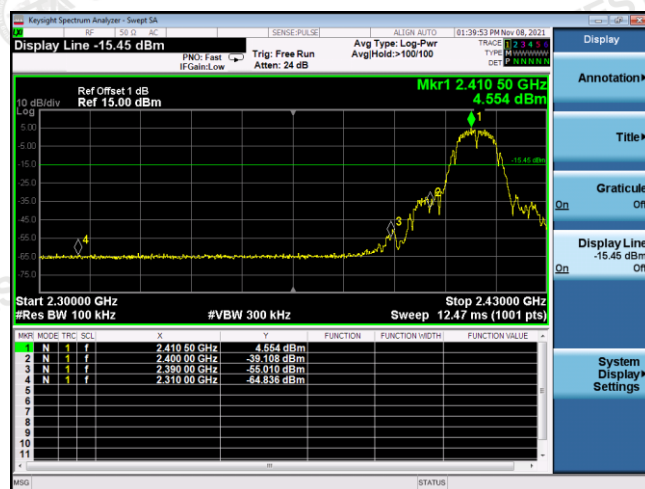
Left bandedge
