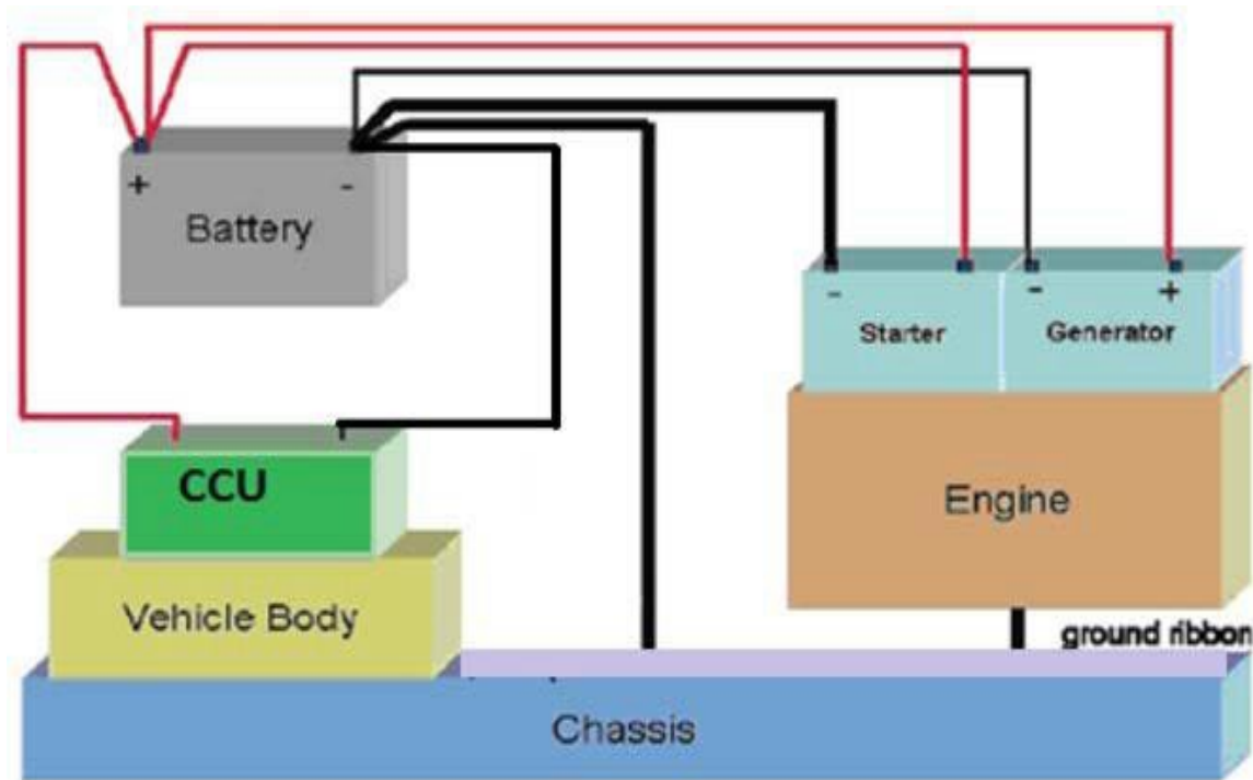
Figure 4 Grounding Scheme
