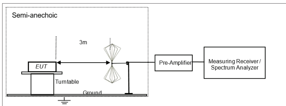
Figure 2: Frequency Range 30 MHz – 200 MHz
