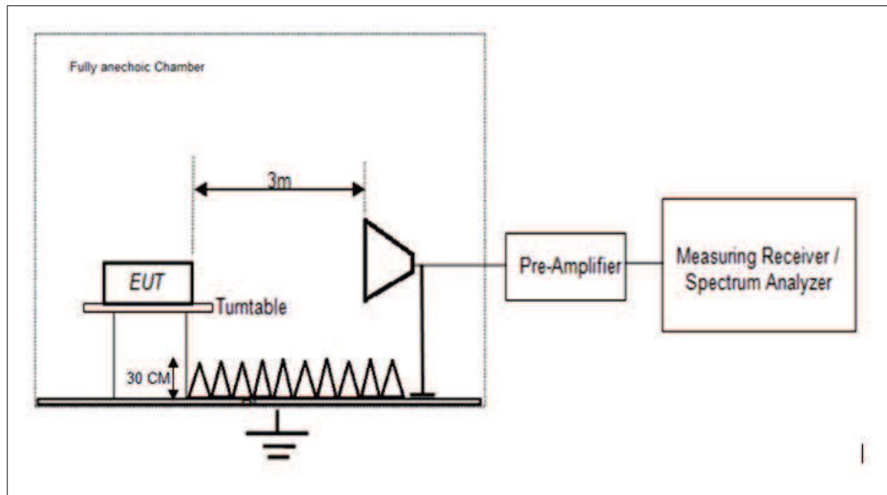
Figure 4: Frequency Range above 1 GHz
