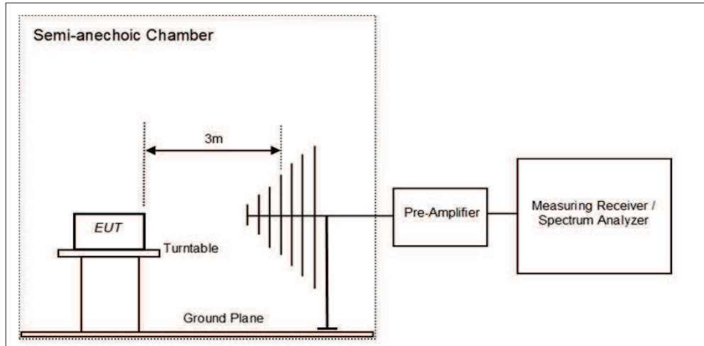
Figure 3: Frequency Range 200 MHz - 1GHz
