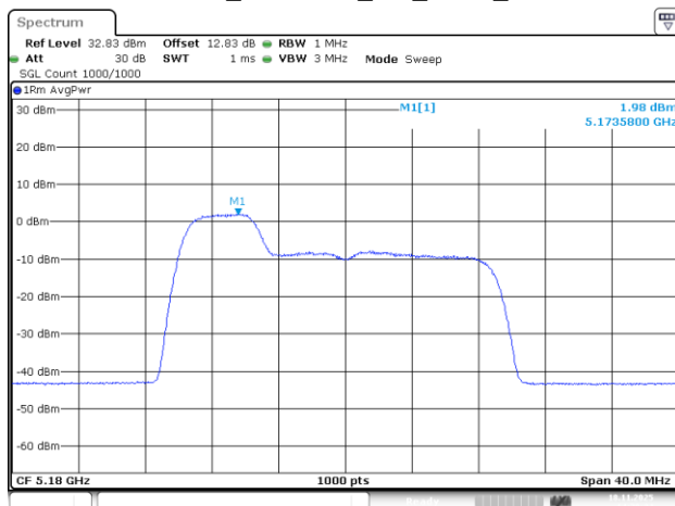
802.11be20_5180MHz_RU_52/37_Chain 1
