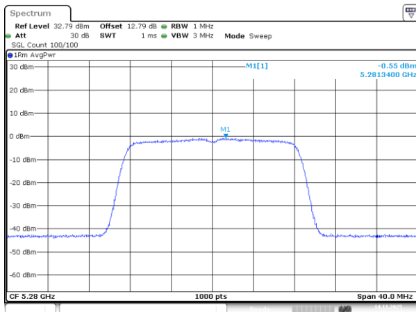
802.11a_5280MHz_Chain 0
