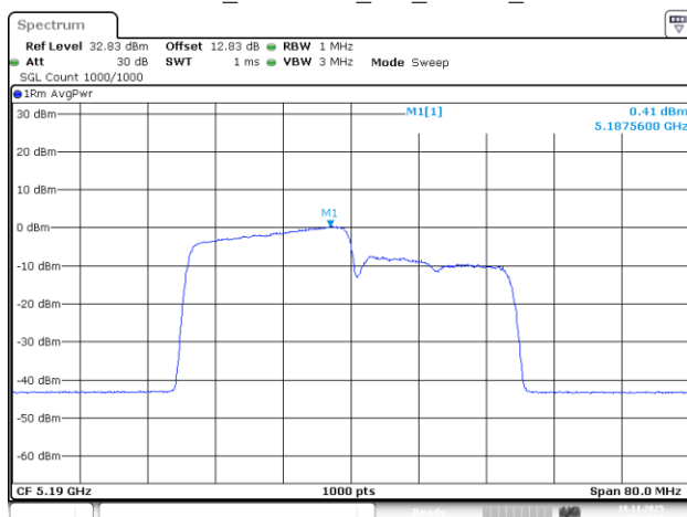
802.11be40_5190MHz_RU_242/61_Chain 0
