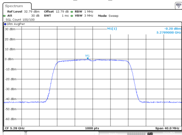
802.11a_5280MHz_Chain 2
