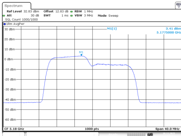
802.11be20_5180MHz_RU_106/53_Chain 2
