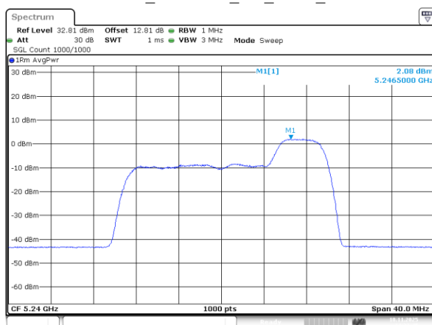
802.11be20_5240MHz_RU_52/40_Chain 3
