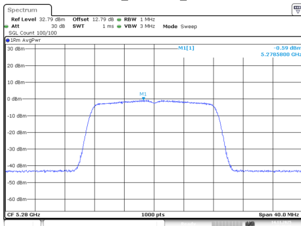
802.11a_5280MHz_Chain 3
