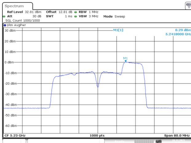
802.11be40_5230MHz_RU_106/56_Chain 0
