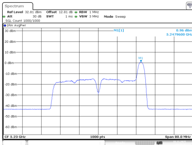
802.11be40_5230MHz_RU_26/17_Chain 0
