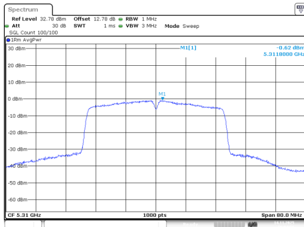
802.11ac40_5310MHz_Chain 2
