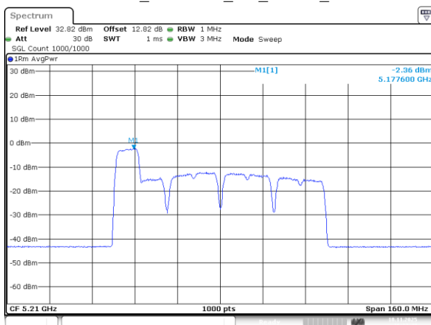
802.11be80_5210MHz_RU_106/53_Chain 1
