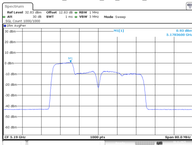
802.11be40_5190MHz_RU_106/53_Chain 2
