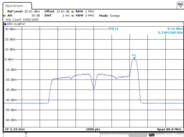
802.11be40_5230MHz_RU_26/17_Chain 1
