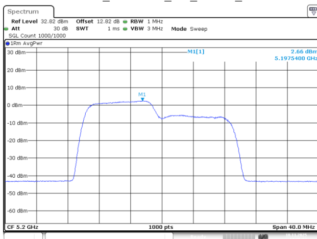
802.11be20_5200MHz_RU_106/53_Chain 0
