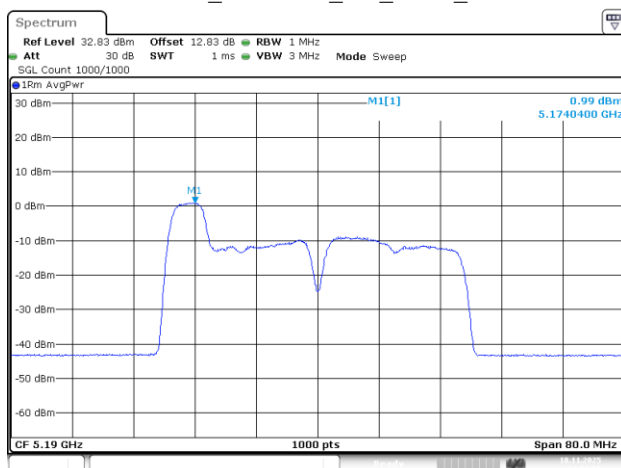
802.11be40_5190MHz_RU_52/37_Chain 2
