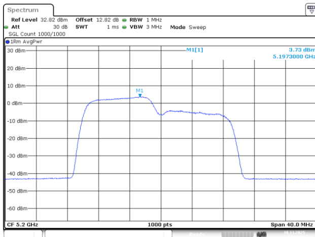
802.11be20_5200MHz_RU_106/53_Chain 2
