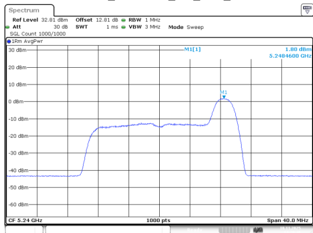
802.11be20_5240MHz_RU_26/8_Chain 3
