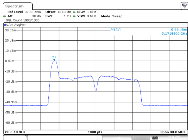
802.11be40_5190MHz_RU_26/0_Chain 1
