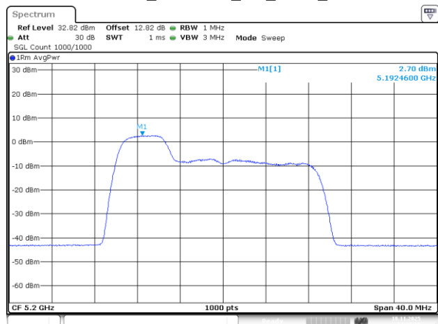
802.11be20_5200MHz_RU_52/37_Chain 1
