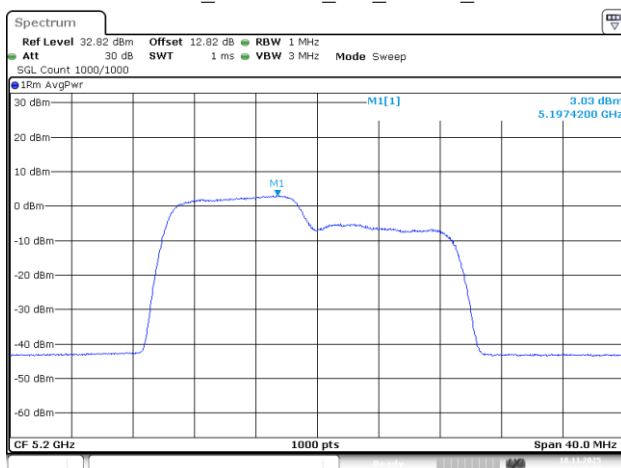
802.11be20_5200MHz_RU_106/53_Chain 1
