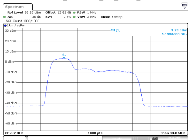
802.11be20_5200MHz_RU_52/37_Chain 3
