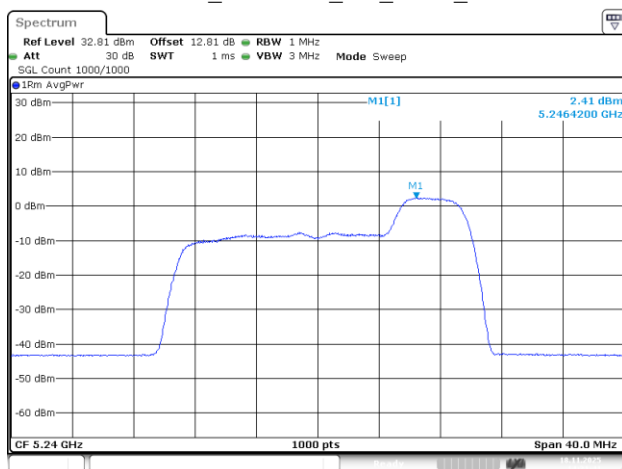
802.11be20_5240MHz_RU_52/40_Chain 0
