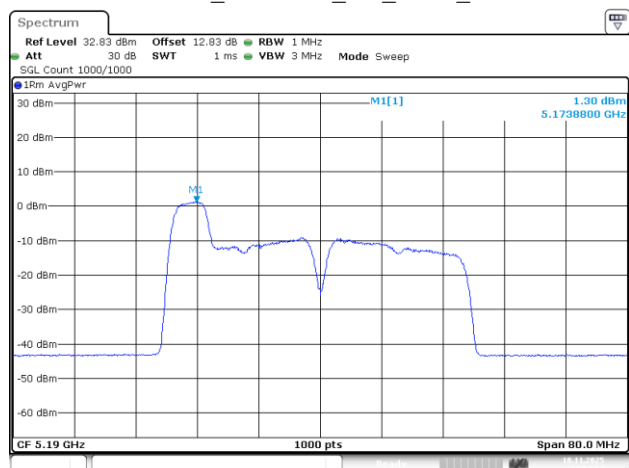
802.11be40_5190MHz_RU_52/37_Chain 3
