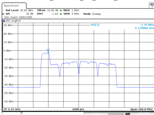
802.11be80_5210MHz_RU_106/53_Chain 0
