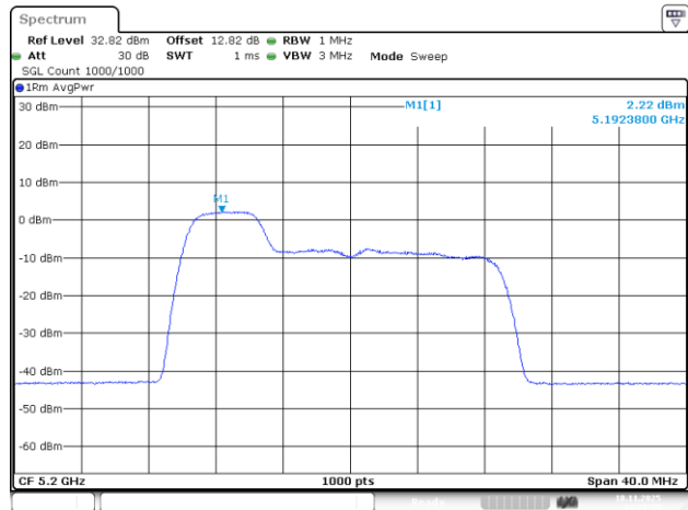
802.11be20_5200MHz_RU_52/37_Chain 0
