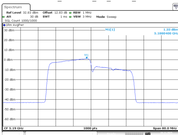
802.11be40_5190MHz_RU_242/61_Chain 3
