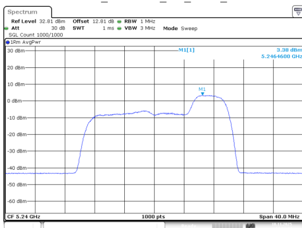
802.11be20_5240MHz_RU_52/40_Chain 2
