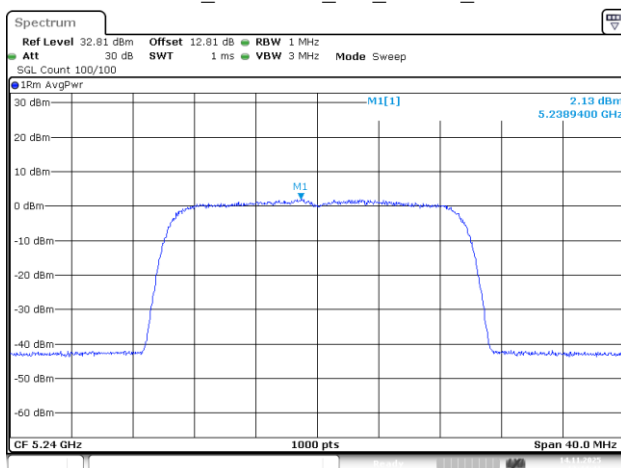
802.11be20_5240MHz_RU_242/61_Chain 3
