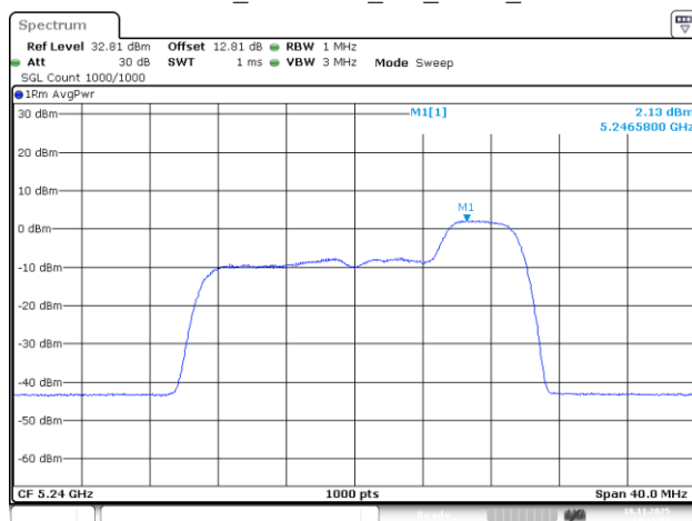
802.11be20_5240MHz_RU_52/40_Chain 1
