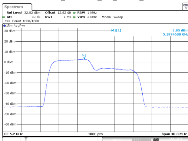
802.11be20_5200MHz_RU_106/53_Chain 3
