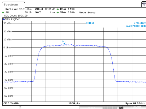
802.11be20_5240MHz_RU_242/61_Chain 2
