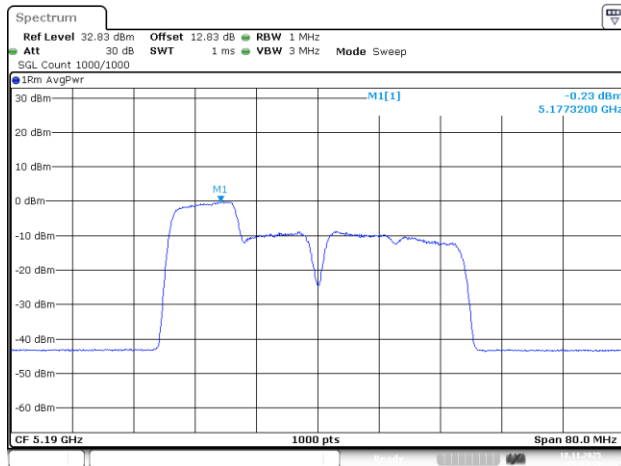
802.11be40_5190MHz_RU_106/53_Chain 0
