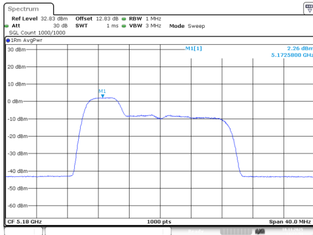
802.11be20_5180MHz_RU_52/37_Chain 0
