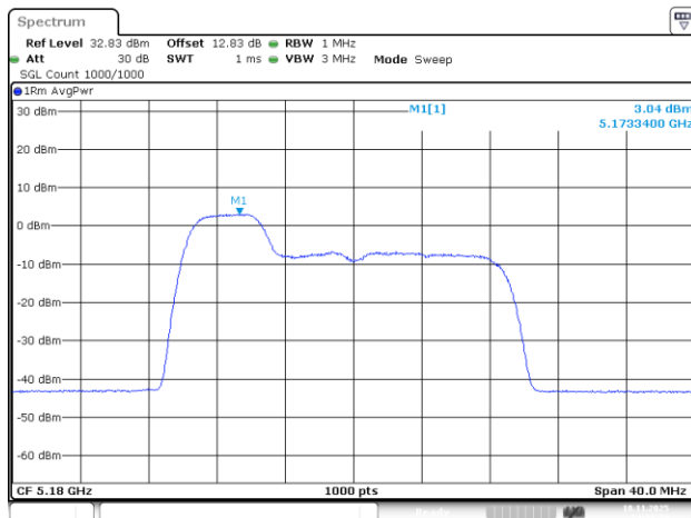
802.11be20_5180MHz_RU_52/37_Chain 2
