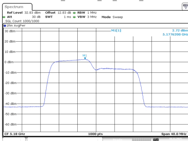
802.11be20_5180MHz_RU_106/53_Chain 1
