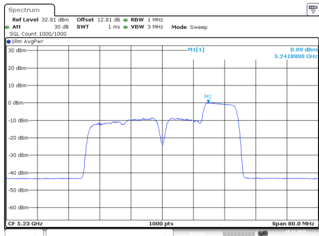
802.11be40_5230MHz_RU_106/56_Chain 1
