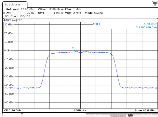
802.11a_5260MHz_Chain 3
