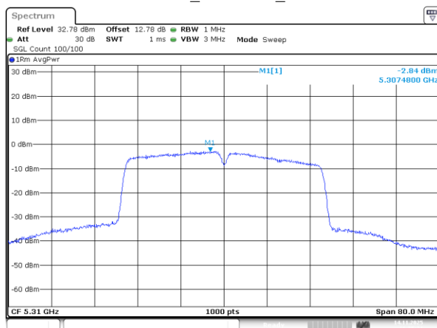
802.11ac40_5310MHz_Chain 3
