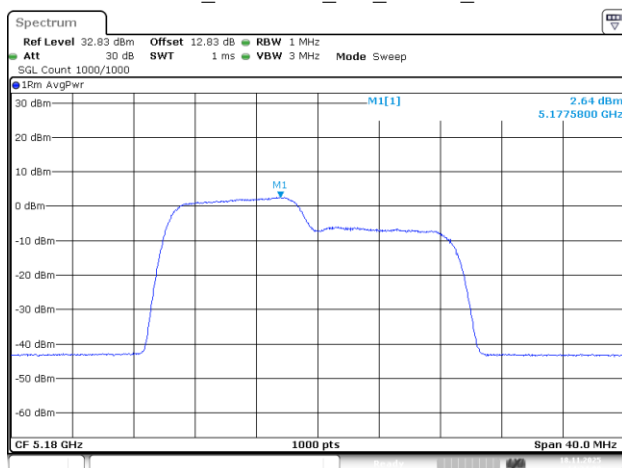
802.11be20_5180MHz_RU_106/53_Chain 0
