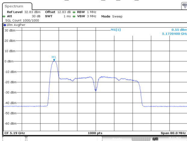
802.11be40_5190MHz_RU_26/0_Chain 0
