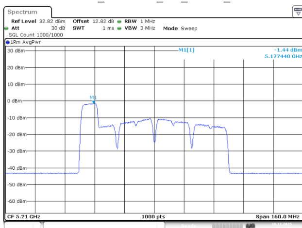
802.11be80_5210MHz_RU_106/53_Chain 2
