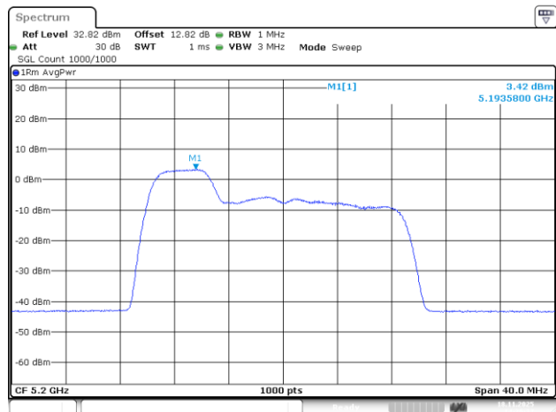
802.11be20_5200MHz_RU_52/37_Chain 2
