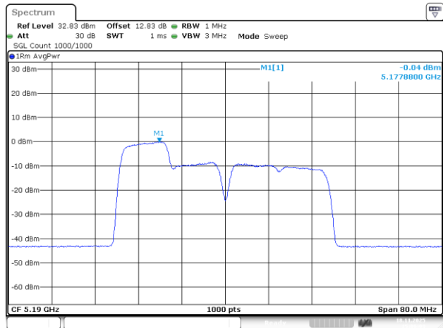
802.11be40_5190MHz_RU_106/53_Chain 1
