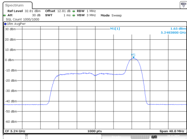
802.11be20_5240MHz_RU_26/8_Chain 1
