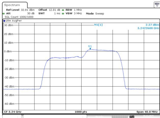
802.11be20_5240MHz_RU_106/54_Chain 1
