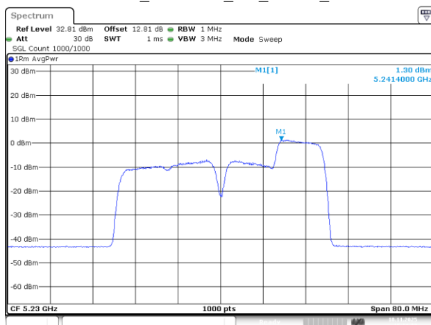
802.11be40_5230MHz_RU_106/56_Chain 2
