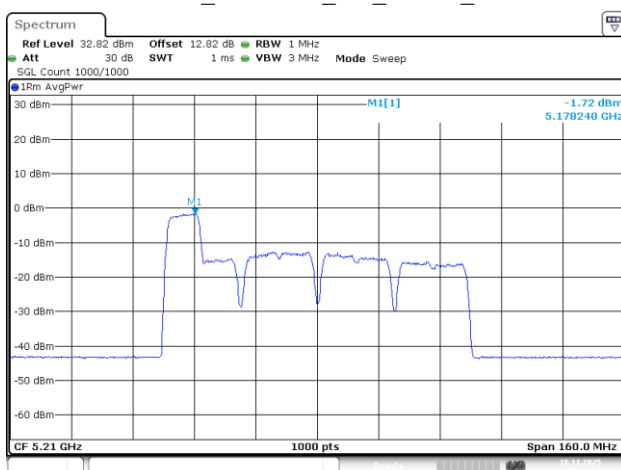
802.11be80_5210MHz_RU_106/53_Chain 3
