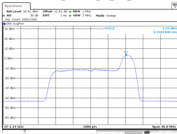
802.11be20_5240MHz_RU_26/8_Chain 2
