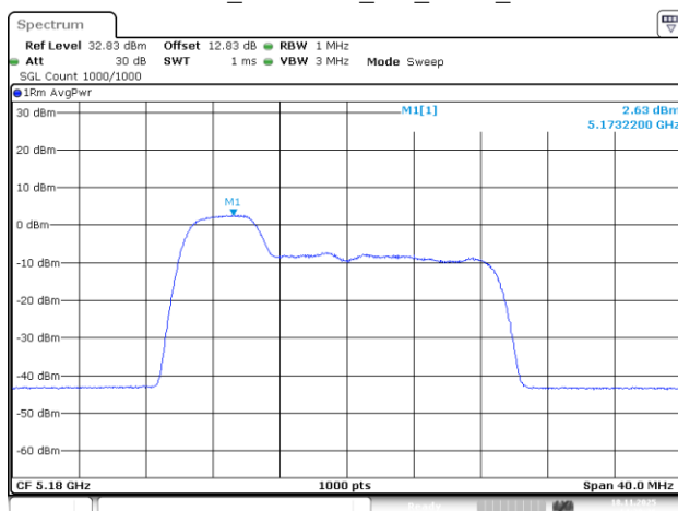
802.11be20_5180MHz_RU_52/37_Chain 3
