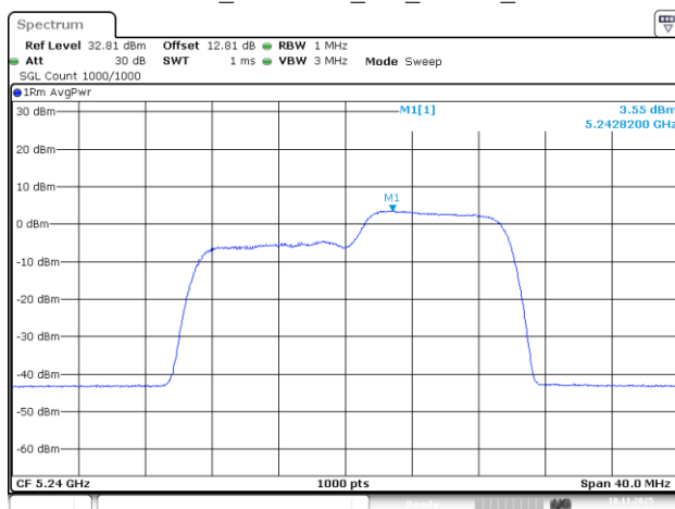
802.11be20_5240MHz_RU_106/54_Chain 2
