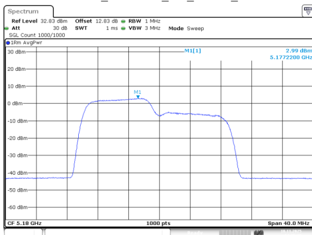
802.11be20_5180MHz_RU_106/53_Chain 3
