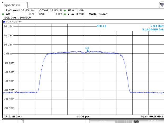
802.11be20_5180MHz_RU_242/61_Chain 3
