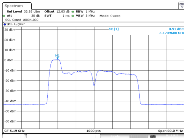
802.11be40_5190MHz_RU_52/37_Chain 0
