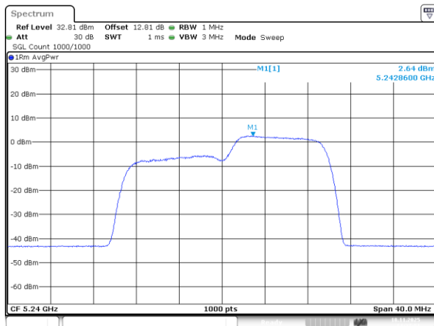
802.11be20_5240MHz_RU_106/54_Chain 0
