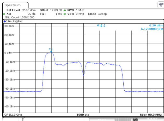
802.11be40_5190MHz_RU_52/37_Chain 1
