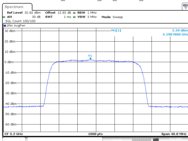
802.11be20_5200MHz_RU_242/61_Chain 3
