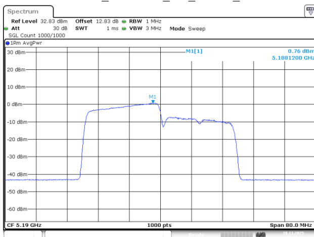
802.11be40_5190MHz_RU_242/61_Chain 1
