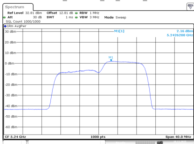
802.11be20_5240MHz_RU_106/54_Chain 3
