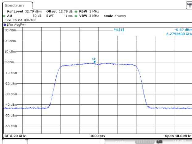
802.11a_5280MHz_Chain 1
