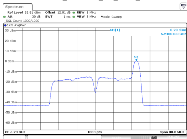
802.11be40_5230MHz_RU_26/17_Chain 3
