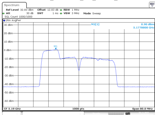
802.11be40_5190MHz_RU_106/53_Chain 3
