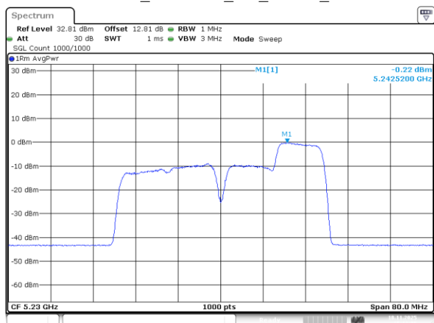
802.11be40_5230MHz_RU_106/56_Chain 3
