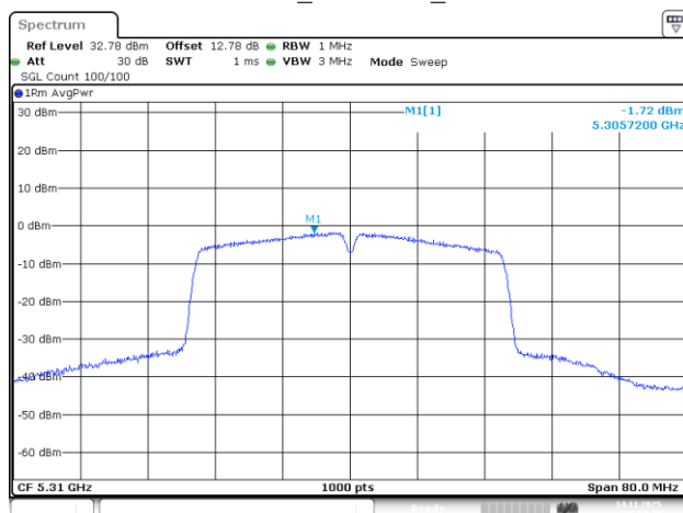
802.11ac40_5310MHz_Chain 1
