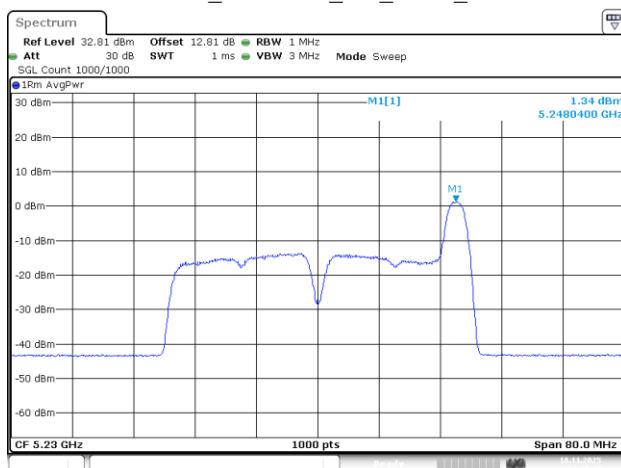
802.11be40_5230MHz_RU_26/17_Chain 2
