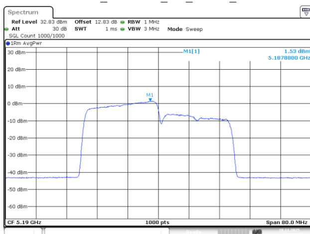
802.11be40_5190MHz_RU_242/61_Chain 2
