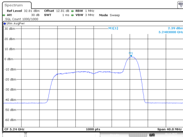
802.11be20_5240MHz_RU_26/8_Chain 0
