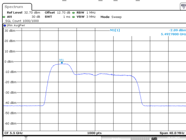
802.11be20_5500MHz_RU_52/37_Chain 3
