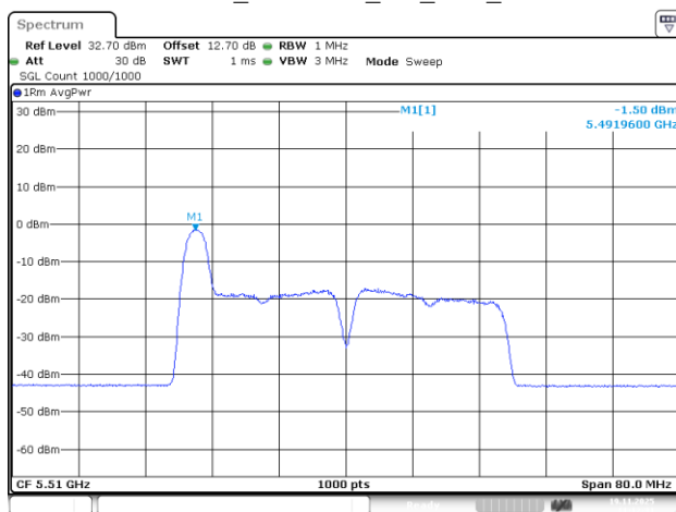
802.11be40_5510MHz_RU_26/0_Chain 1
