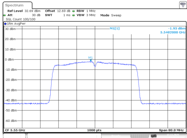
802.11ac40_5550MHz_Chain 0
