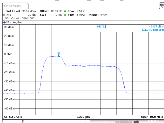
802.11be20_5580MHz_RU_52/37_Chain 3
