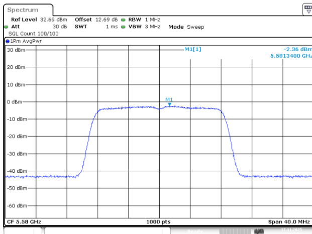
802.11a_5580MHz_Chain 3
