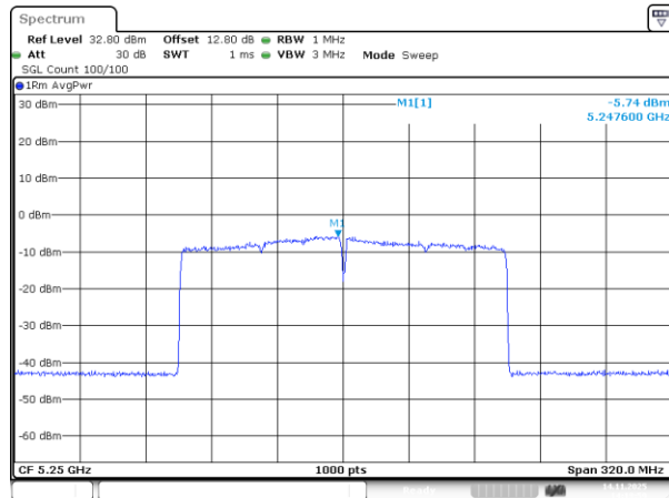
802.11be160_5250MHz_RU_2*996_Chain 0
