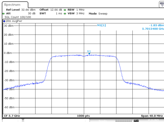
802.11a_5700MHz_Chain 0
