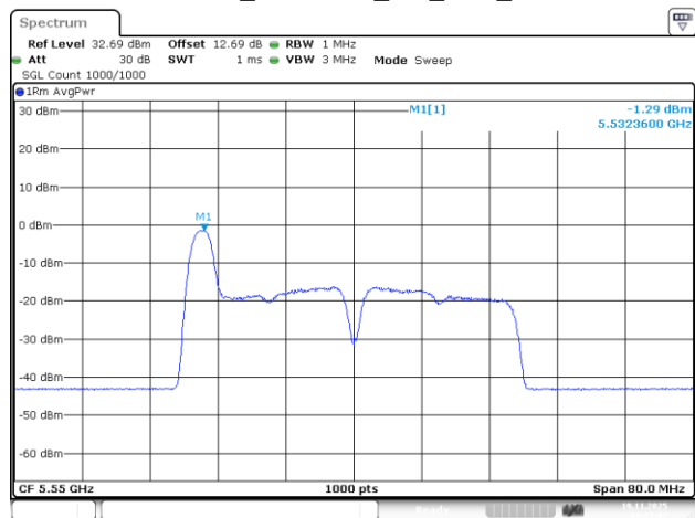
802.11be40_5550MHz_RU_26/0_Chain 0
