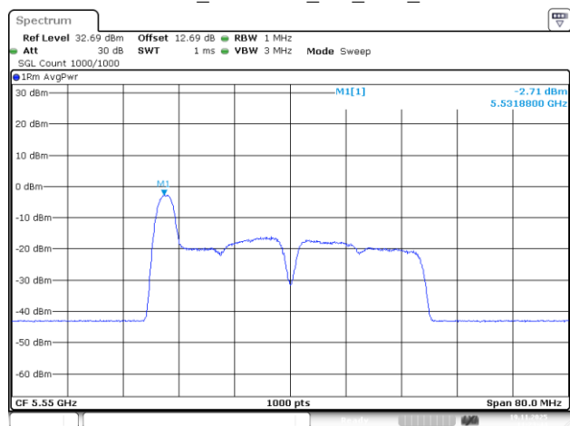
802.11be40_5550MHz_RU_26/0_Chain 1
