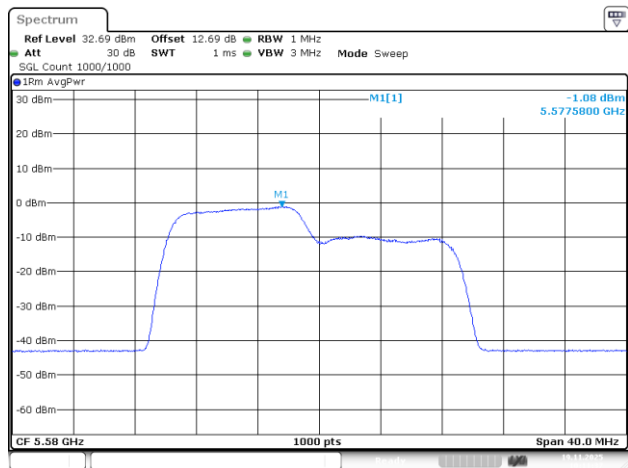
802.11be20_5580MHz_RU_106/53_Chain 0
