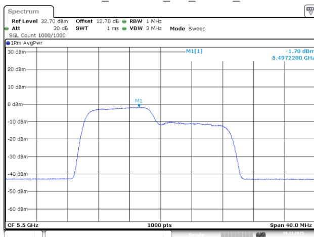
802.11be20_5500MHz_RU_106/53_Chain 1
