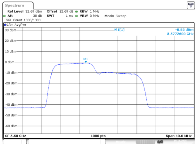
802.11be20_5580MHz_RU_106/53_Chain 2
