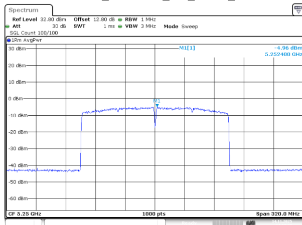
802.11be160_5250MHz_RU_2*996_Chain 2
