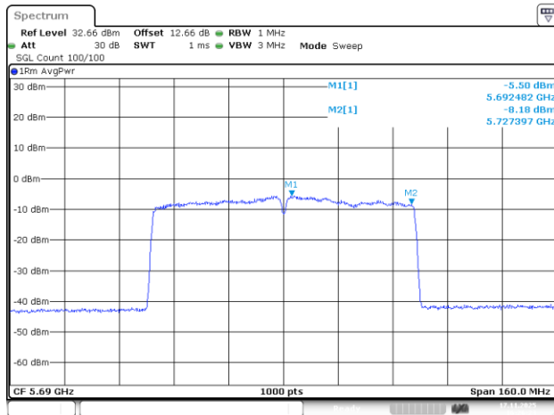
802.11ac80_5690MHz_Chain 2
