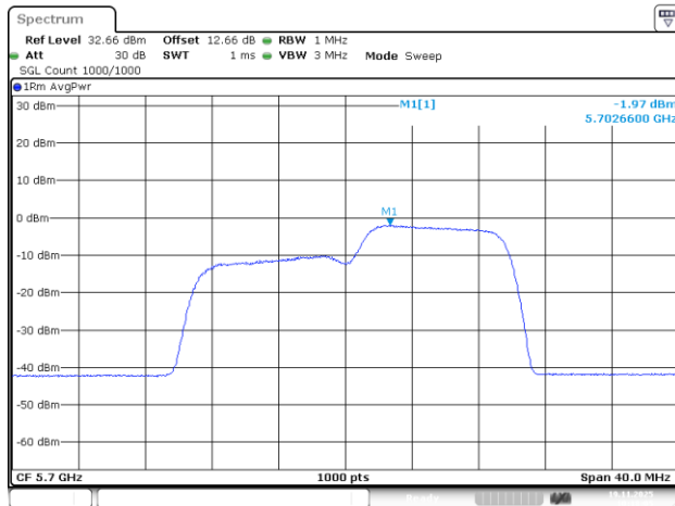
802.11be20_5700MHz_RU_106/54_Chain 2
