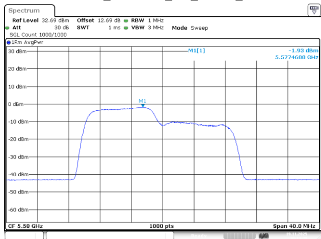
802.11be20_5580MHz_RU_106/53_Chain 3
