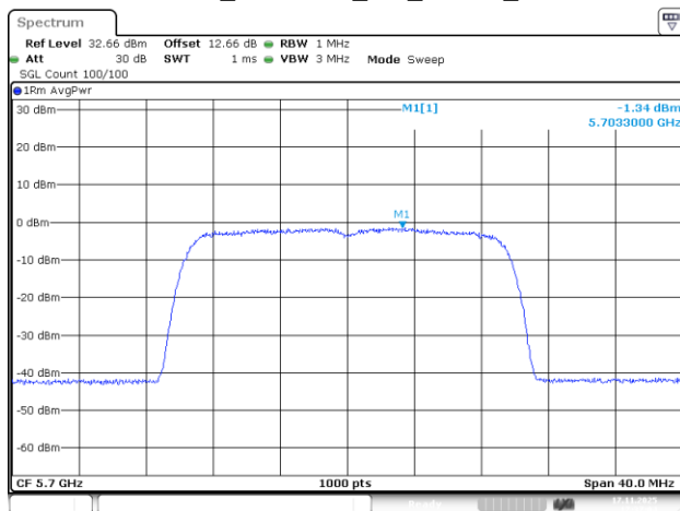
802.11be20_5700MHz_RU_242/61_Chain 0
