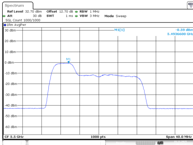
802.11be20_5500MHz_RU_52/37_Chain 0
