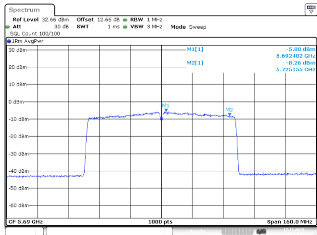
802.11ac80_5690MHz_Chain 1
