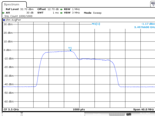
802.11be20_5500MHz_RU_106/53_Chain 2
