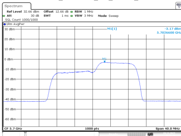
802.11be20_5700MHz_RU_106/54_Chain 3
