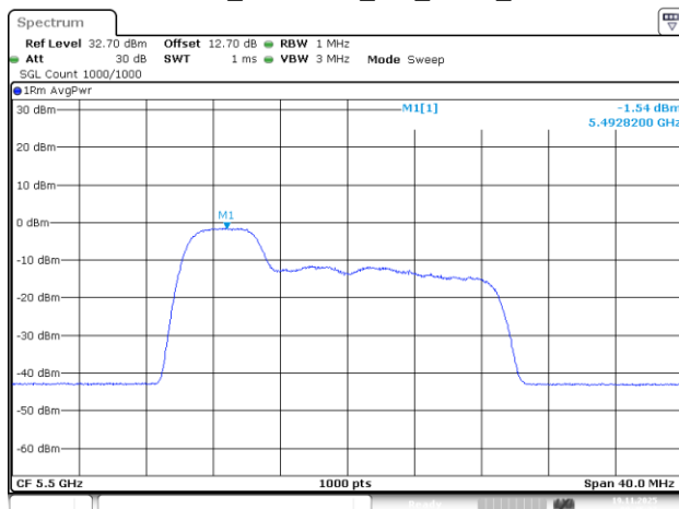
802.11be20_5500MHz_RU_52/37_Chain 1
