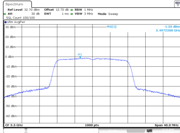
802.11a_5500MHz_Chain 0
