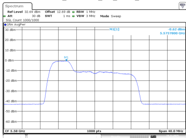
802.11be20_5580MHz_RU_52/37_Chain 1
