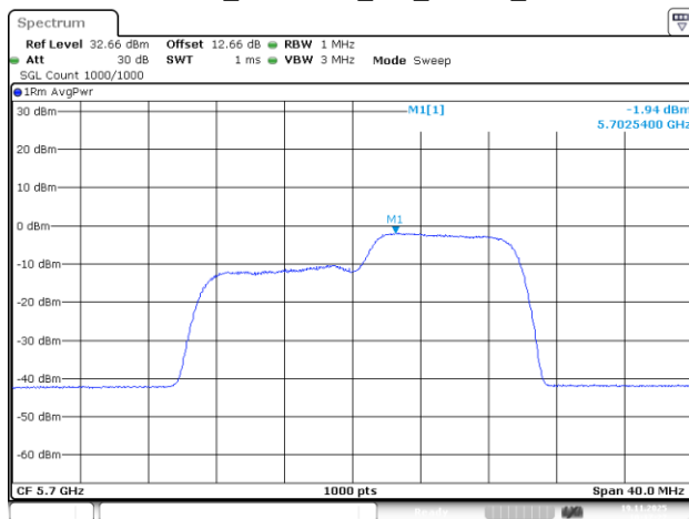
802.11be20_5700MHz_RU_106/54_Chain 1
