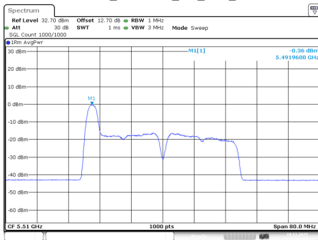
802.11be40_5510MHz_RU_26/0_Chain 0
