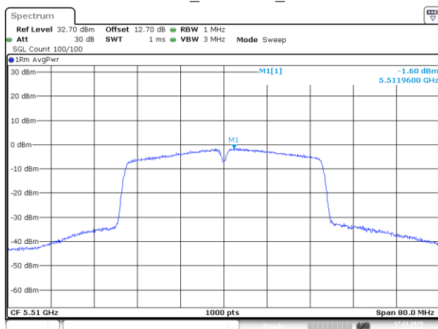
802.11ac40_5510MHz_Chain 3
