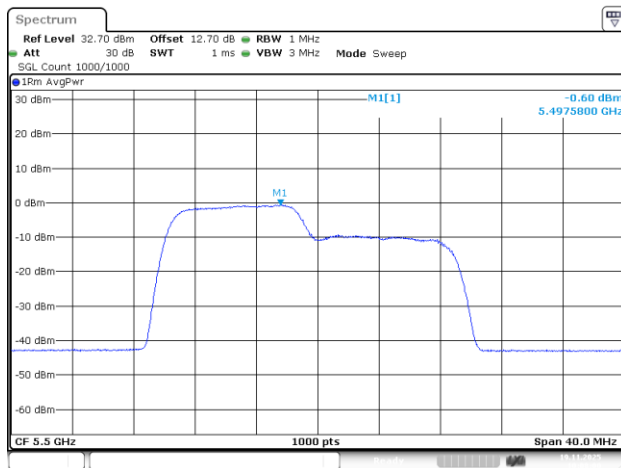
802.11be20_5500MHz_RU_106/53_Chain 0
