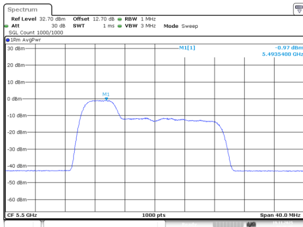
802.11be20_5500MHz_RU_52/37_Chain 2
