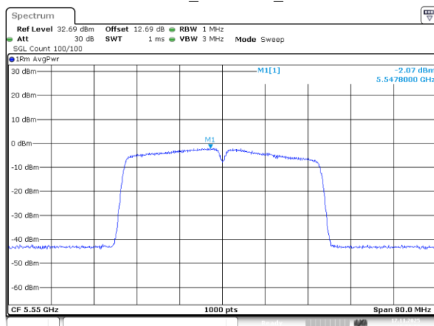
802.11ac40_5550MHz_Chain 3
