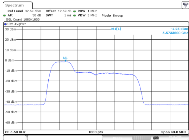
802.11be20_5580MHz_RU_52/37_Chain 0
