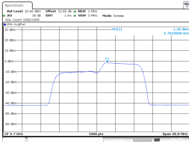
802.11be20_5700MHz_RU_106/54_Chain 0
