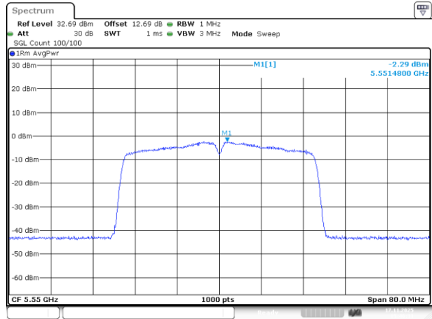
802.11ac40_5550MHz_Chain 1
