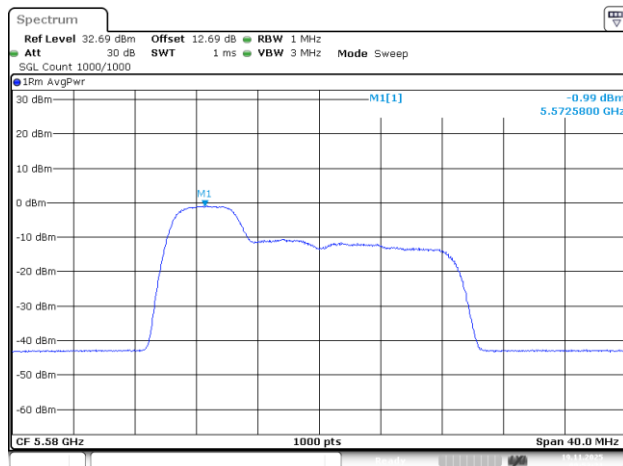
802.11be20_5580MHz_RU_52/37_Chain 2
