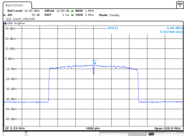
802.11be160_5250MHz_RU_2*996_Chain 1
