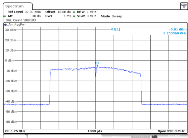
802.11be160_5250MHz_RU_2*996_Chain 3
