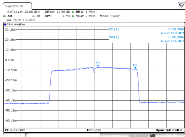
802.11ac80_5690MHz_Chain 3
