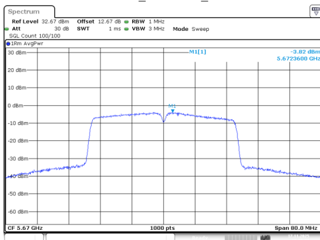
802.11ac40_5670MHz_Chain 3
