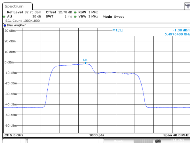
802.11be20_5500MHz_RU_106/53_Chain 3
