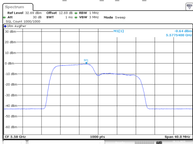
802.11be20_5580MHz_RU_106/53_Chain 1
