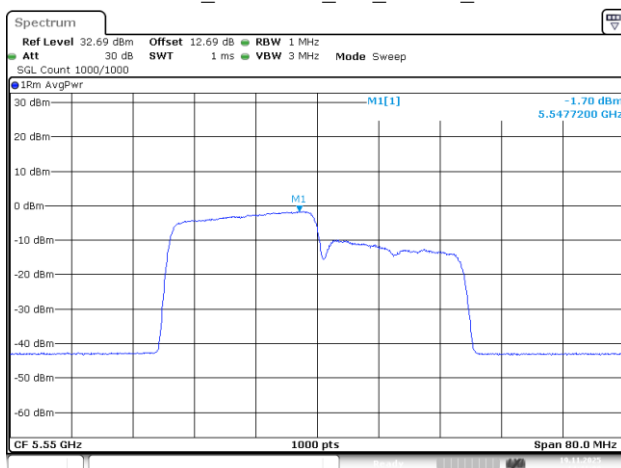
802.11be40_5550MHz_RU_242/61_Chain 3
