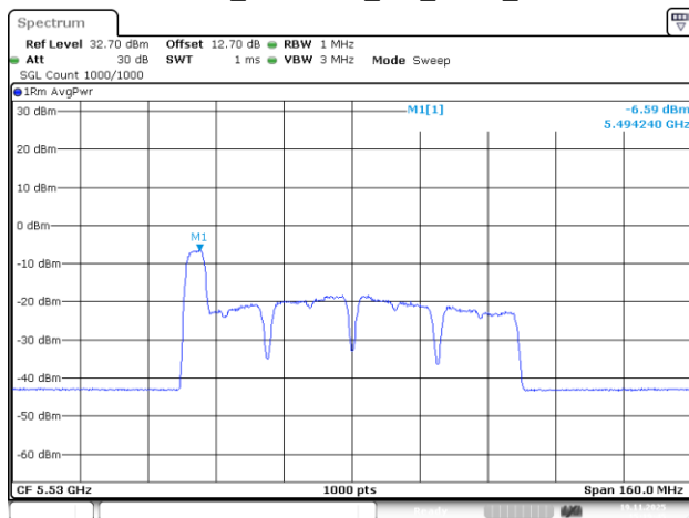
802.11be80_5530MHz_RU_52/37_Chain 3
