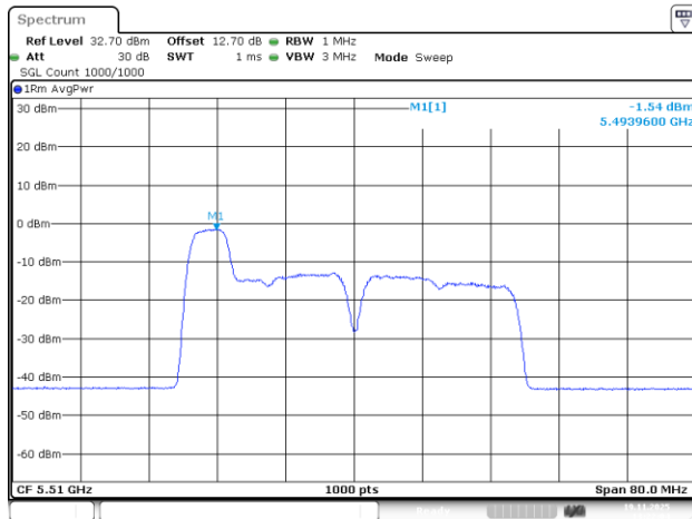
802.11be40_5510MHz_RU_52/37_Chain 2
