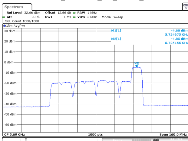
802.11be80_5690MHz_RU_106/60_Chain 1
