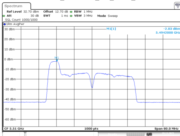
802.11be40_5510MHz_RU_52/37_Chain 1
