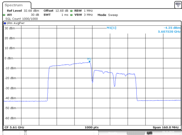
802.11be80_5610MHz_RU_484/65_Chain 0
