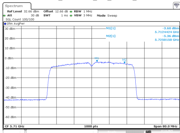
802.11be40_5710MHz_RU_484/65_Chain 3
