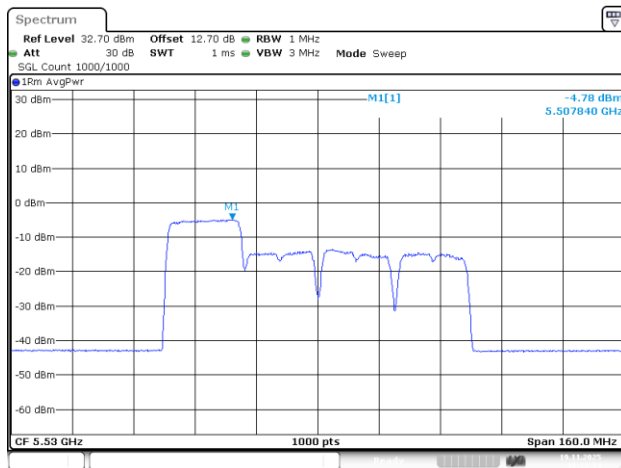
802.11be80_5530MHz_RU_242/61_Chain 0
