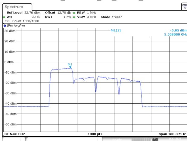
802.11be80_5530MHz_RU_242/61_Chain 1
