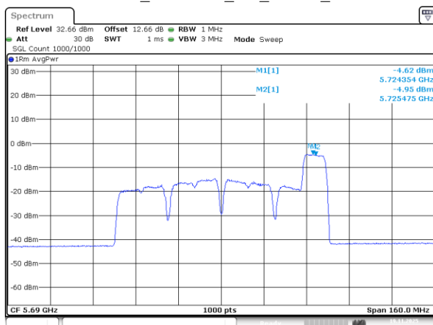
802.11be80_5690MHz_RU_106/60_Chain 0
