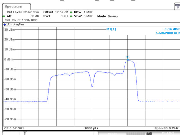
802.11be40_5670MHz_RU_52/44_Chain 0
