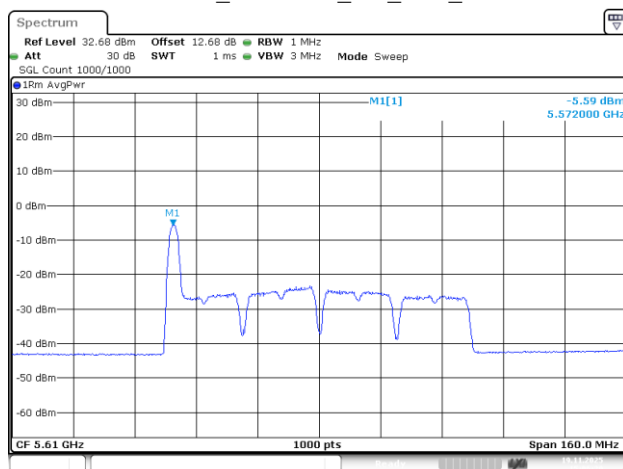
802.11be80_5610MHz_RU_26/0_Chain 0
