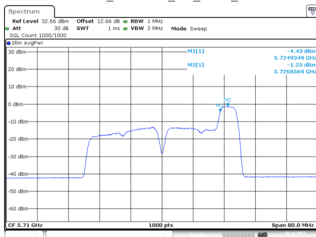
802.11be40_5710MHz_RU_52/44_Chain 1
