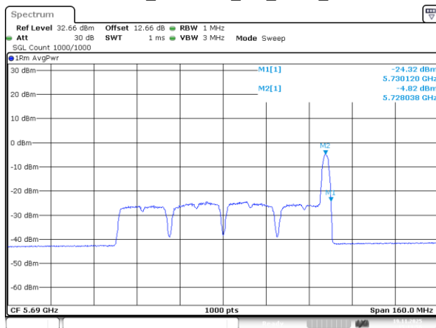
802.11be80_5690MHz_RU_26/36_Chain 2
