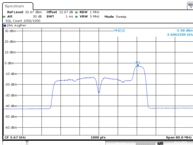
802.11be40_5670MHz_RU_52/44_Chain 2
