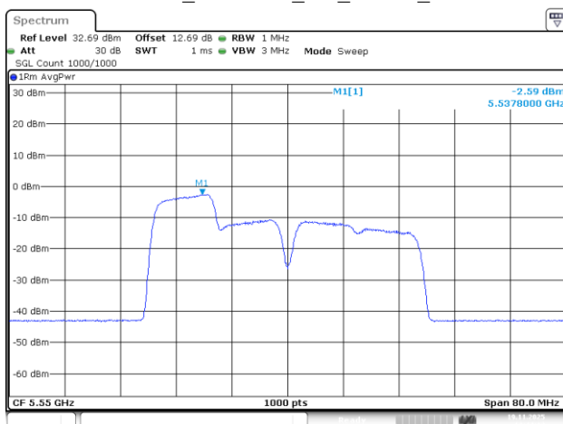
802.11be40_5550MHz_RU_106/53_Chain 1
