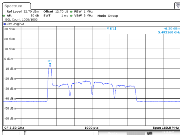
802.11be80_5530MHz_RU_26/0_Chain 3
