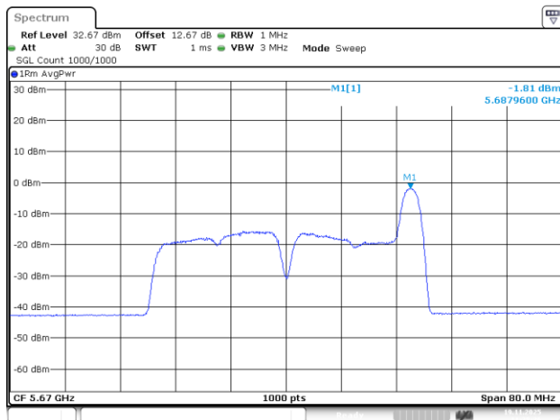
802.11be40_5670MHz_RU_26/17_Chain 0
