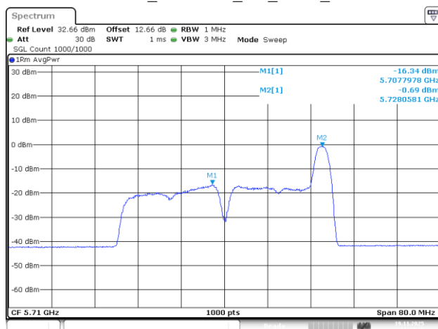
802.11be40_5710MHz_RU_26/17_Chain 1
