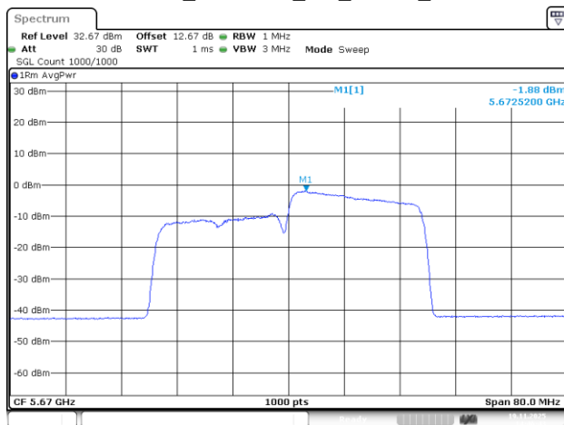
802.11be40_5670MHz_RU_242/62_Chain 1
