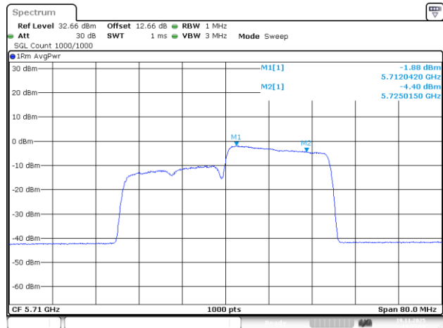
802.11be40_5710MHz_RU_242/62_Chain 0
