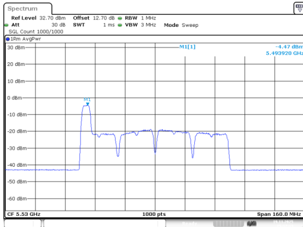
802.11be80_5530MHz_RU_52/37_Chain 0
