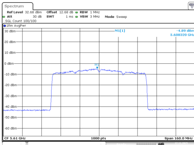
802.11be80_5610MHz_RU_996/67_Chain 0
