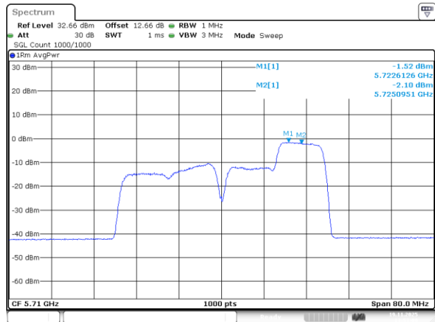
802.11be40_5710MHz_RU_106/56_Chain 2
