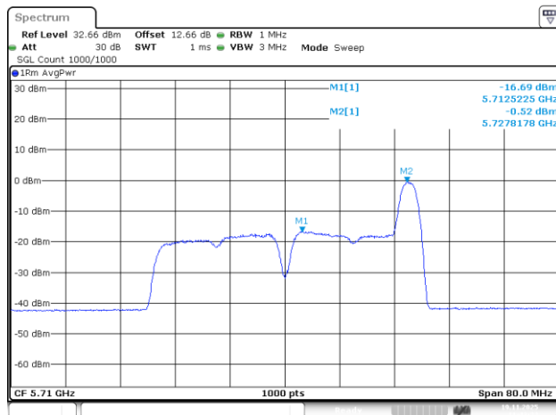
802.11be40_5710MHz_RU_26/17_Chain 0
