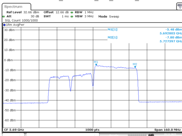
802.11be80_5690MHz_RU_484/66_Chain 3
