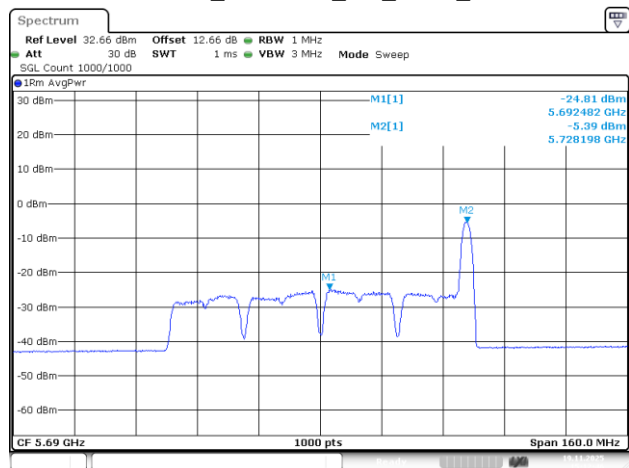
802.11be80_5690MHz_RU_26/36_Chain 3
