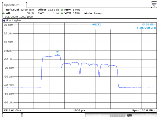
802.11be80_5610MHz_RU_242/61_Chain 0
