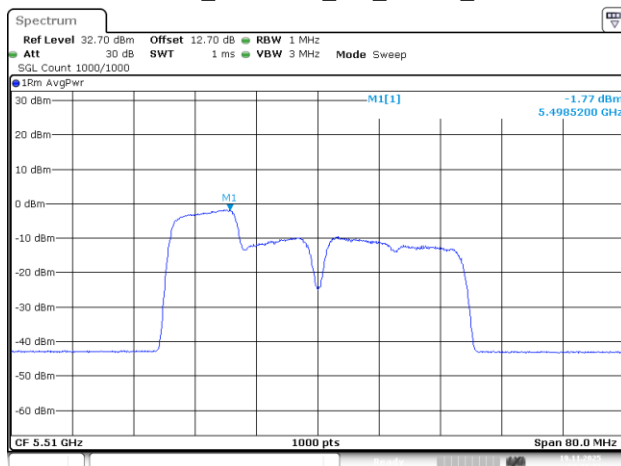
802.11be40_5510MHz_RU_106/53_Chain 3
