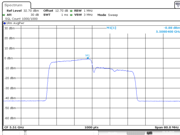
802.11be40_5510MHz_RU_242/61_Chain 0
