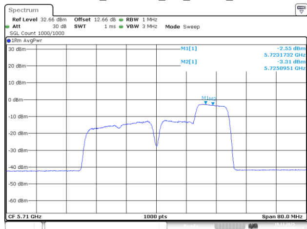
802.11be40_5710MHz_RU_106/56_Chain 3
