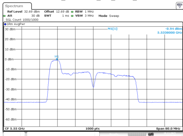
802.11be40_5550MHz_RU_52/37_Chain 3
