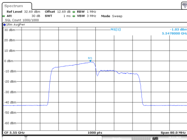
802.11be40_5550MHz_RU_242/61_Chain 2
