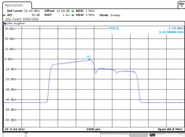
802.11be40_5550MHz_RU_242/61_Chain 0
