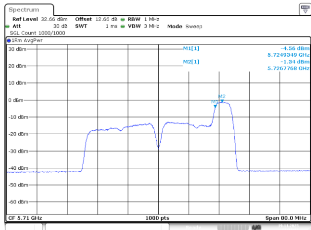
802.11be40_5710MHz_RU_52/44_Chain 2
