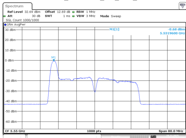
802.11be40_5550MHz_RU_26/0_Chain 3
