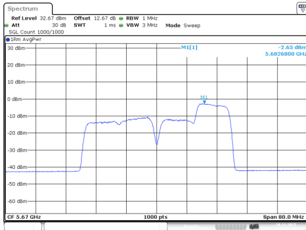
802.11be40_5670MHz_RU_106/56_Chain 2
