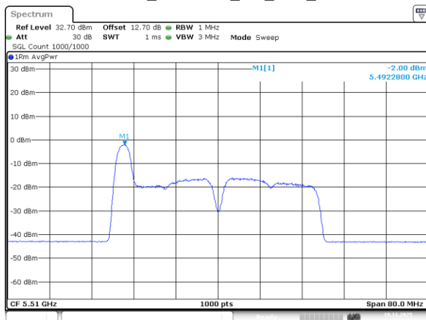
802.11be40_5510MHz_RU_26/0_Chain 3
