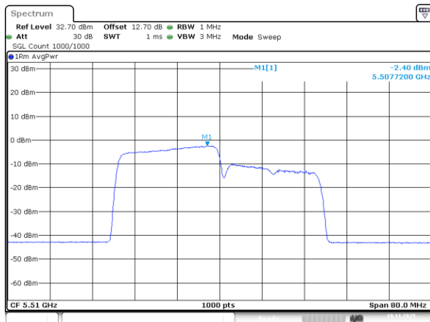
802.11be40_5510MHz_RU_242/61_Chain 2
