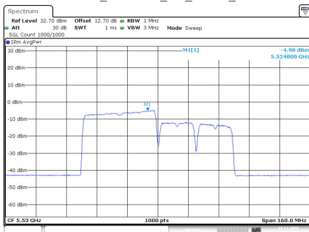
802.11be80_5530MHz_RU_484/65_Chain 2
