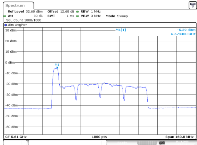
802.11be80_5610MHz_RU_52/37_Chain 0
