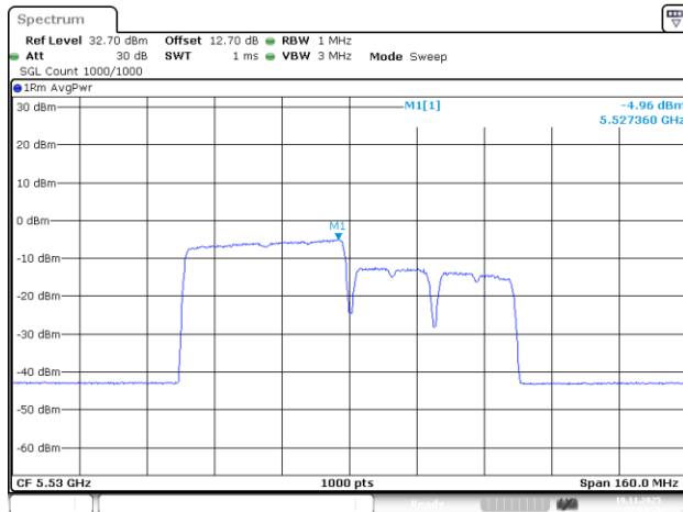
802.11be80_5530MHz_RU_484/65_Chain 0
