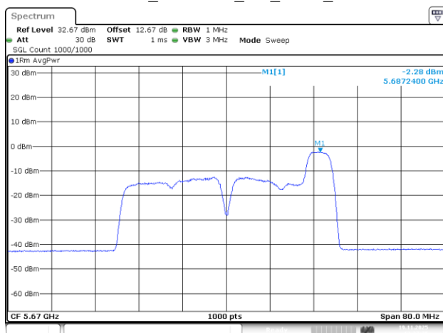
802.11be40_5670MHz_RU_52/44_Chain 1
