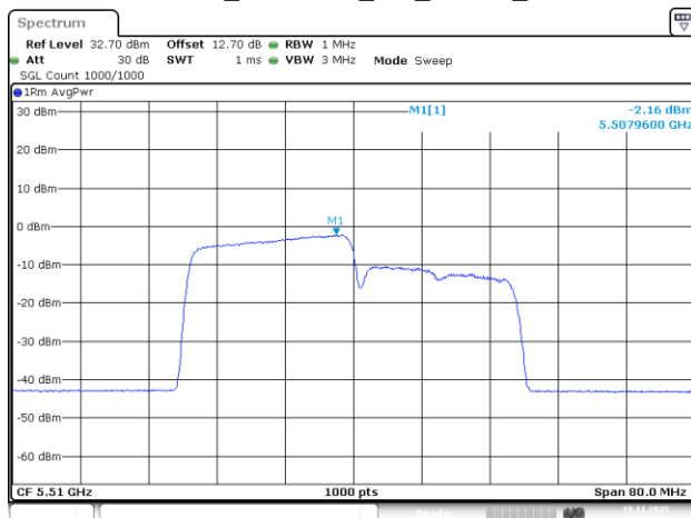
802.11be40_5510MHz_RU_242/61_Chain 1
