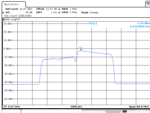
802.11be40_5670MHz_RU_242/62_Chain 2
