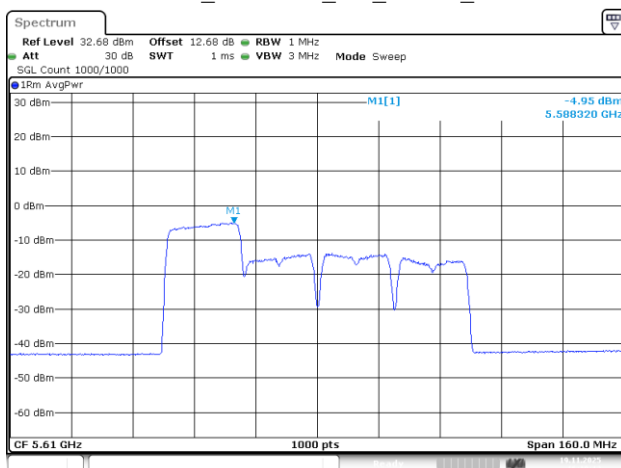
802.11be80_5610MHz_RU_242/61_Chain 2
