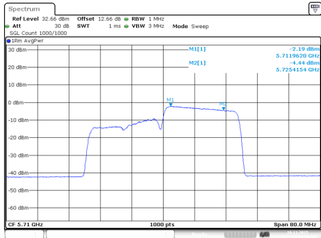
802.11be40_5710MHz_RU_242/62_Chain 2
