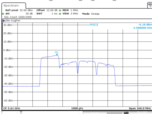
802.11be80_5610MHz_RU_242/61_Chain 3
