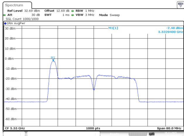
802.11be40_5550MHz_RU_26/0_Chain 2
