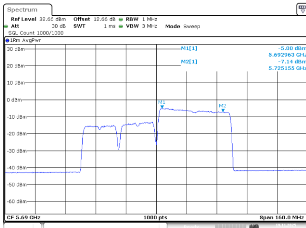
802.11be80_5690MHz_RU_484/66_Chain 1
