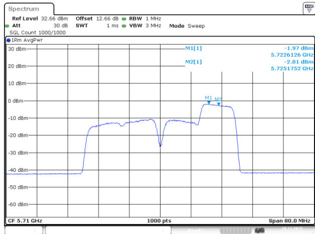
802.11be40_5710MHz_RU_106/56_Chain 0
