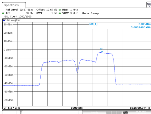
802.11be40_5670MHz_RU_106/56_Chain 3
