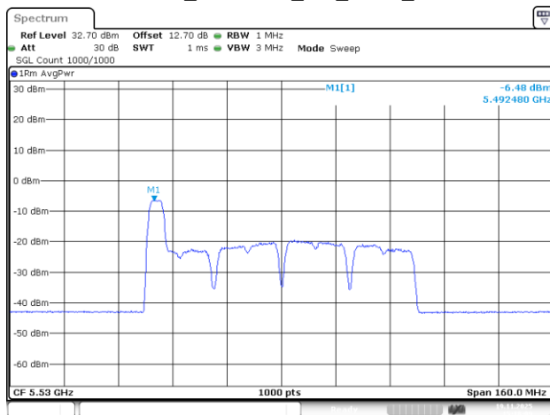
802.11be80_5530MHz_RU_52/37_Chain 1
