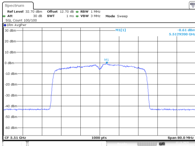
802.11be40_5510MHz_RU_484/65_Chain 3
