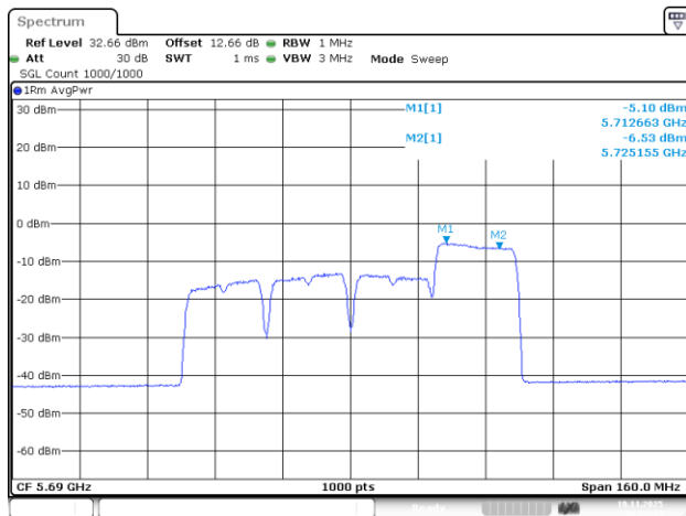
802.11be80_5690MHz_RU_242/64_Chain 0
