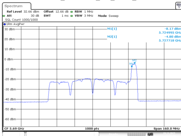
802.11be80_5690MHz_RU_52/52_Chain 2
