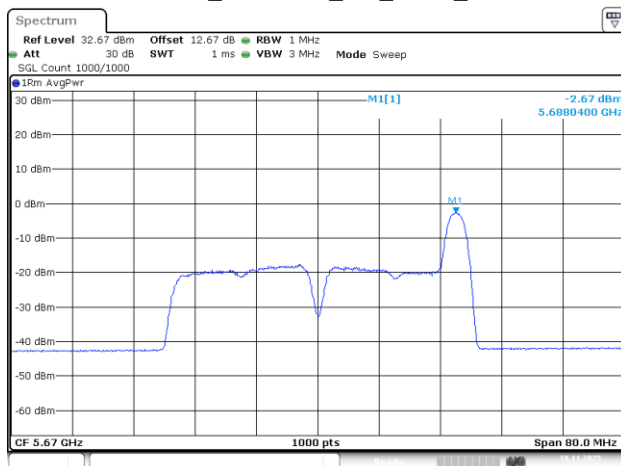
802.11be40_5670MHz_RU_26/17_Chain 3
