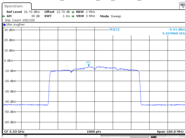
802.11be80_5530MHz_RU_996/67_Chain 1
