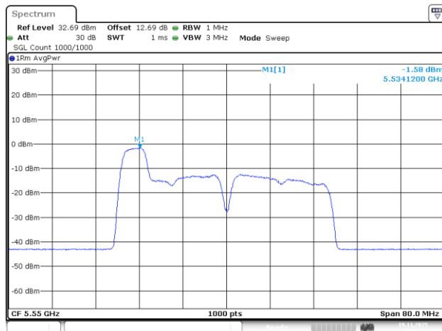
802.11be40_5550MHz_RU_52/37_Chain 0
