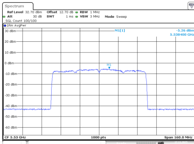
802.11be80_5530MHz_RU_996/67_Chain 0
