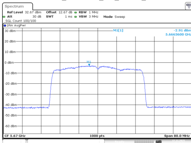
802.11be40_5670MHz_RU_484/65_Chain 3
