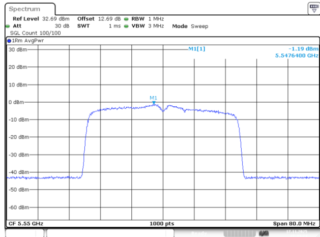
802.11be40_5550MHz_RU_484/65_Chain 3
