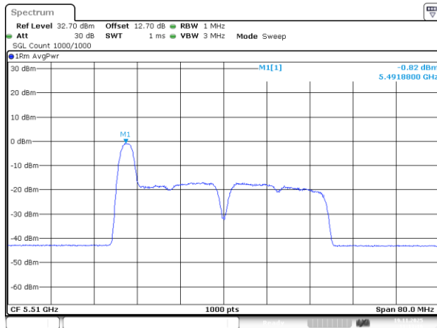
802.11be40_5510MHz_RU_26/0_Chain 2
