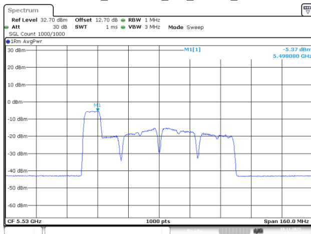
802.11be80_5530MHz_RU_106/53_Chain 1
