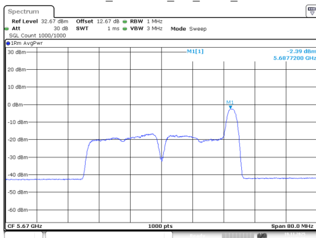
802.11be40_5670MHz_RU_26/17_Chain 1
