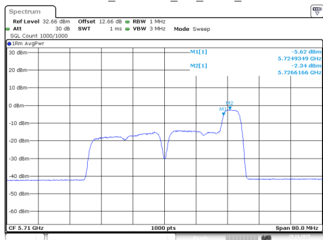
802.11be40_5710MHz_RU_52/44_Chain 3
