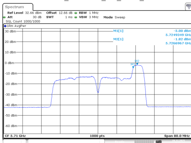
802.11be40_5710MHz_RU_52/44_Chain 0
