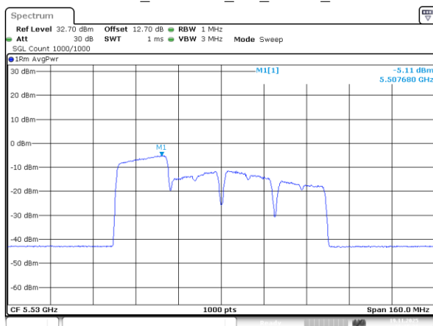
802.11be80_5530MHz_RU_242/61_Chain 3
