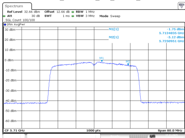
802.11be40_5710MHz_RU_484/65_Chain 0
