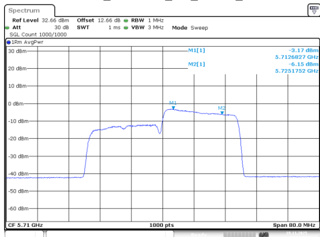
802.11be40_5710MHz_RU_242/62_Chain 3
