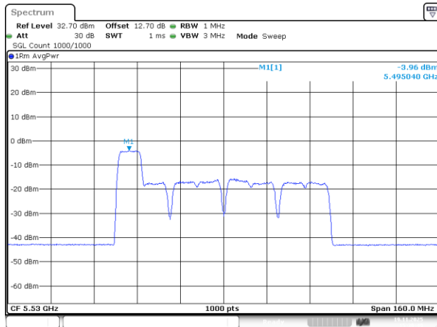
802.11be80_5530MHz_RU_106/53_Chain 0
