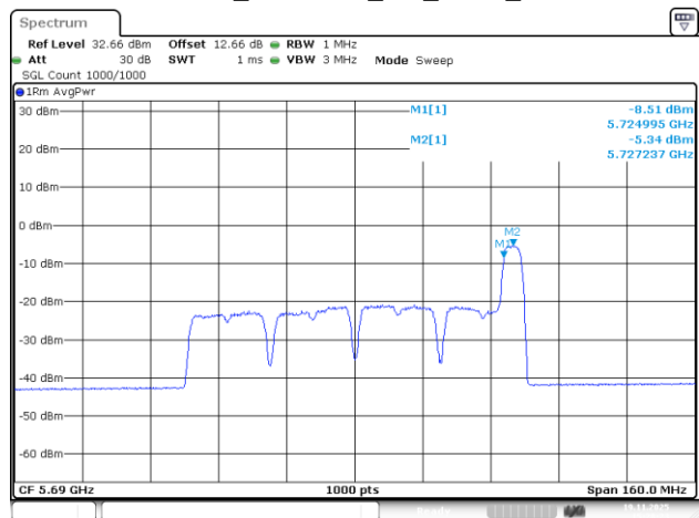
802.11be80_5690MHz_RU_52/52_Chain 3
