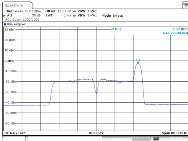
802.11be40_5670MHz_RU_26/17_Chain 2
