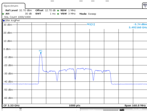
802.11be80_5530MHz_RU_26/0_Chain 1
