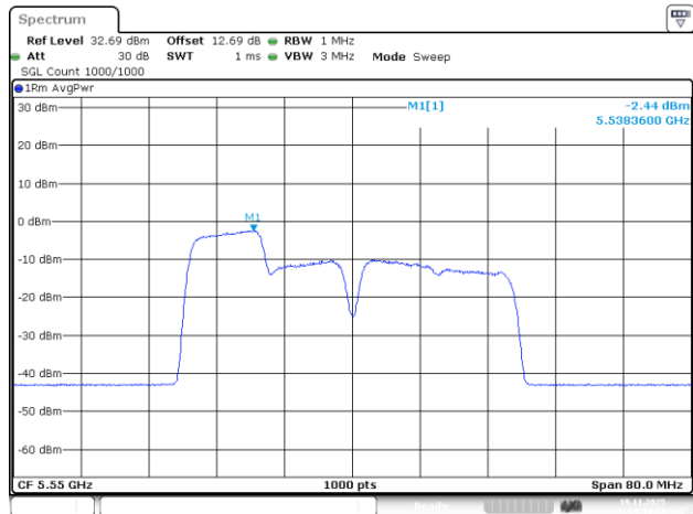
802.11be40_5550MHz_RU_106/53_Chain 2
