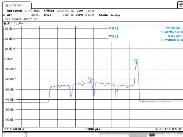
802.11be80_5690MHz_RU_26/36_Chain 0
