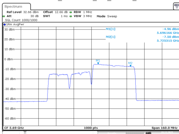
802.11be80_5690MHz_RU_484/66_Chain 2
