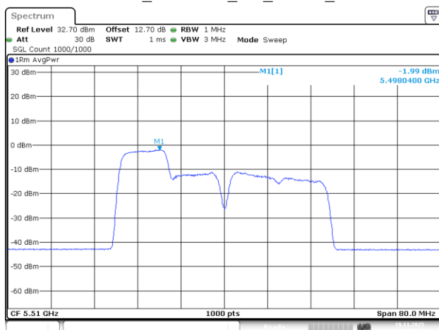
802.11be40_5510MHz_RU_106/53_Chain 1
