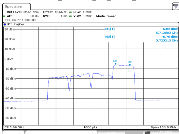
802.11be80_5690MHz_RU_242/64_Chain 3
