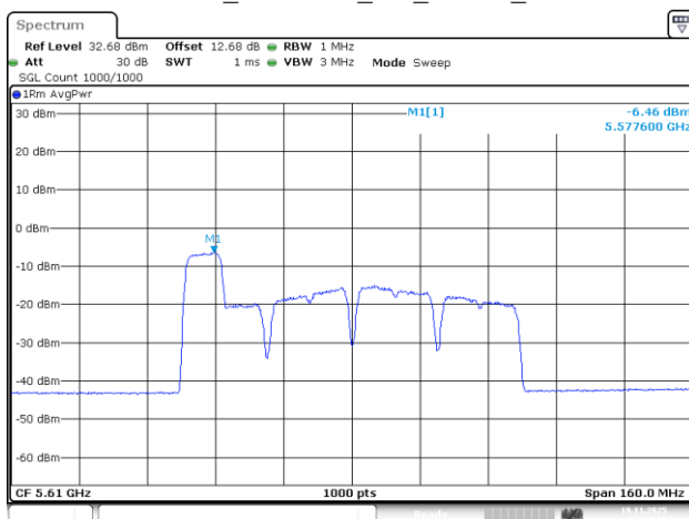
802.11be80_5610MHz_RU_106/53_Chain 3
