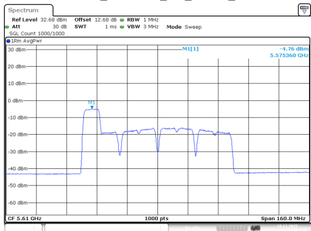
802.11be80_5610MHz_RU_106/53_Chain 1
