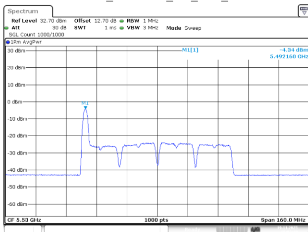
802.11be80_5530MHz_RU_26/0_Chain 0
