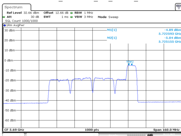
802.11be80_5690MHz_RU_106/60_Chain 2
