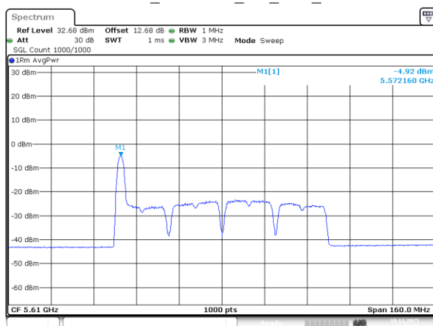
802.11be80_5610MHz_RU_26/0_Chain 1
