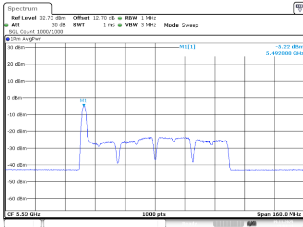
802.11be80_5530MHz_RU_26/0_Chain 2
