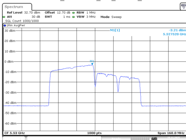
802.11be80_5530MHz_RU_484/65_Chain 3
