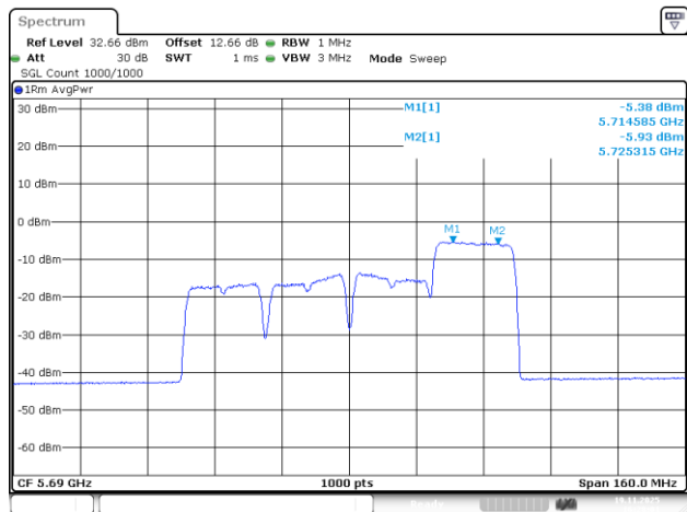
802.11be80_5690MHz_RU_242/64_Chain 1
