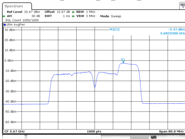
802.11be40_5670MHz_RU_106/56_Chain 1
