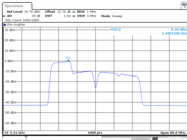
802.11be40_5510MHz_RU_106/53_Chain 0
