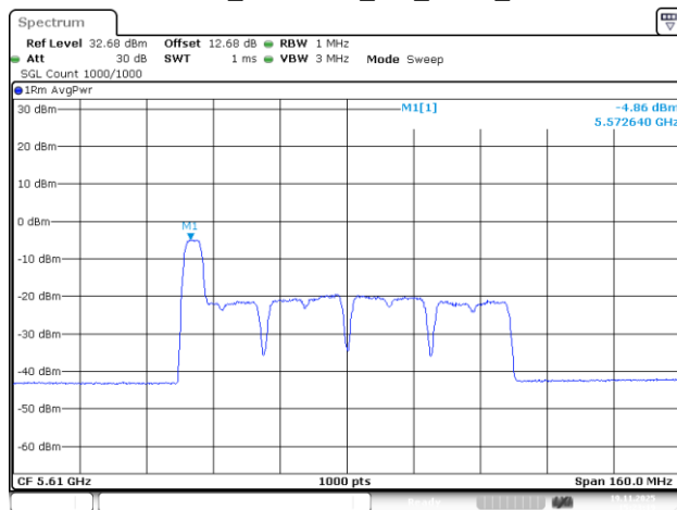
802.11be80_5610MHz_RU_52/37_Chain 2
