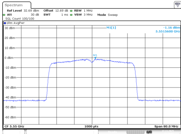
802.11be40_5550MHz_RU_484/65_Chain 0
