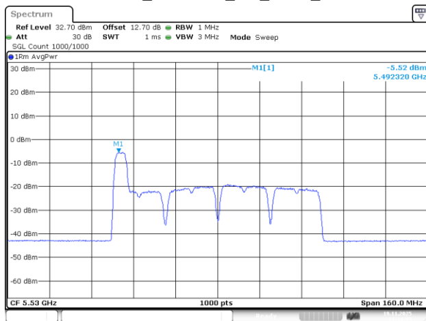
802.11be80_5530MHz_RU_52/37_Chain 2
