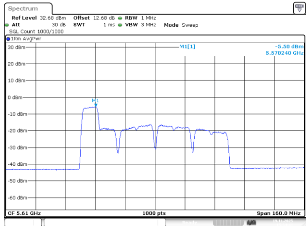
802.11be80_5610MHz_RU_106/53_Chain 0
