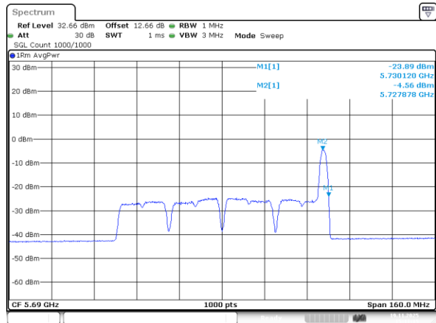
802.11be80_5690MHz_RU_26/36_Chain 1
