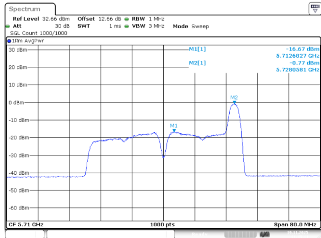
802.11be40_5710MHz_RU_26/17_Chain 2
