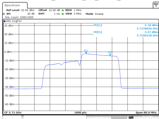
802.11be40_5710MHz_RU_242/62_Chain 1
