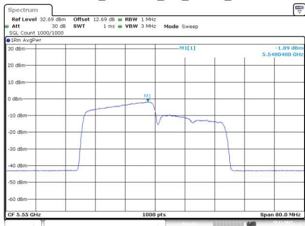
802.11be40_5550MHz_RU_242/61_Chain 1
