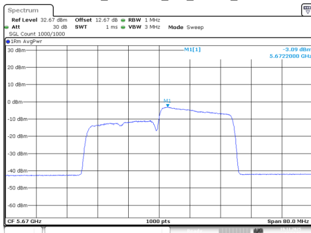
802.11be40_5670MHz_RU_242/62_Chain 3
