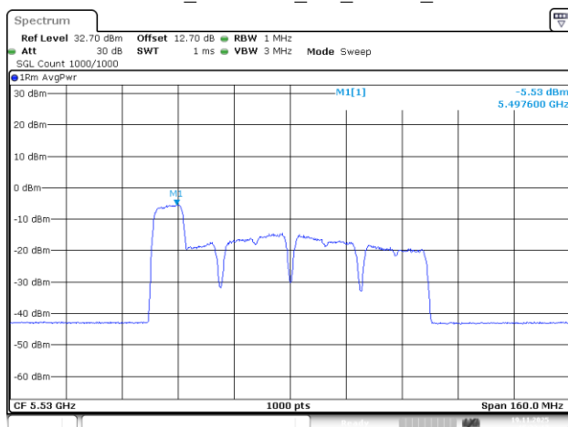
802.11be80_5530MHz_RU_106/53_Chain 3
