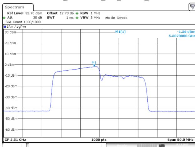
802.11be40_5510MHz_RU_242/61_Chain 3
