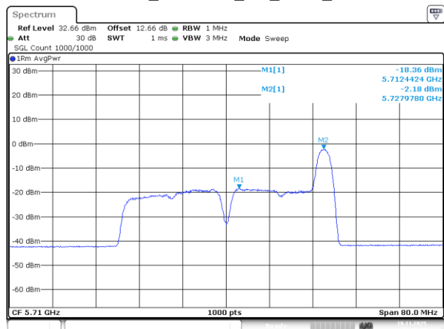
802.11be40_5710MHz_RU_26/17_Chain 3
