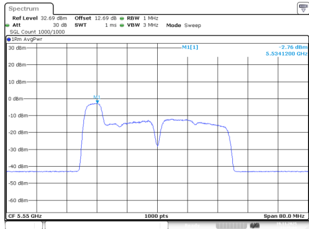
802.11be40_5550MHz_RU_52/37_Chain 2
