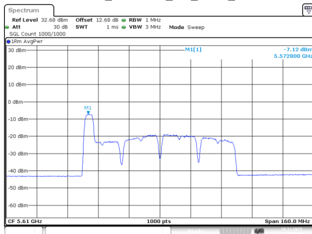
802.11be80_5610MHz_RU_52/37_Chain 3
