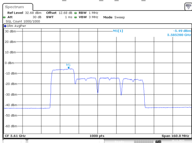
802.11be80_5610MHz_RU_242/61_Chain 1
