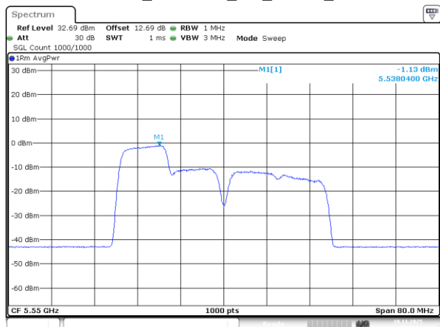
802.11be40_5550MHz_RU_106/53_Chain 3
