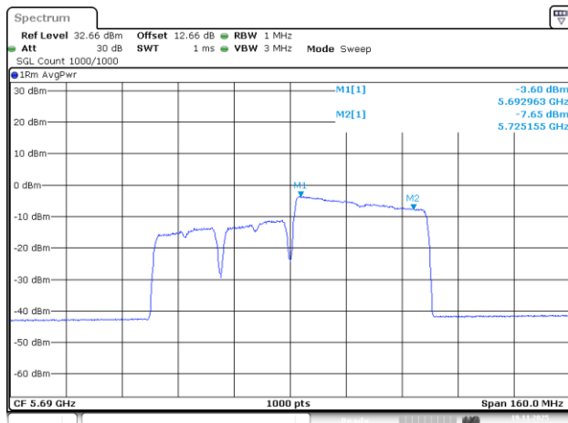
802.11be80_5690MHz_RU_484/66_Chain 0
