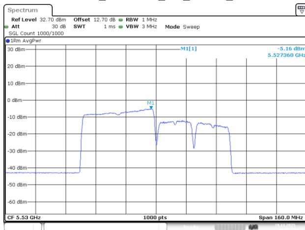
802.11be80_5530MHz_RU_484/65_Chain 1
