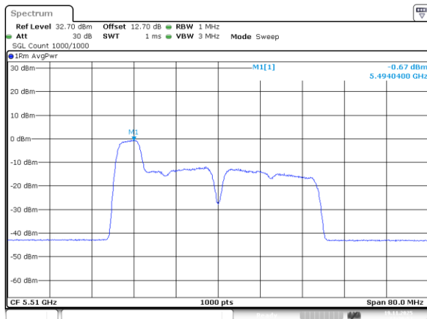
802.11be40_5510MHz_RU_52/37_Chain 0
