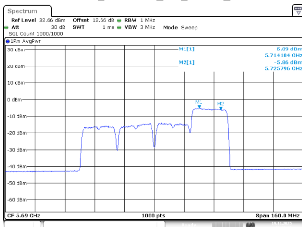
802.11be80_5690MHz_RU_242/64_Chain 2
