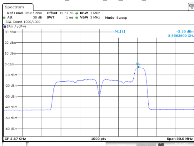
802.11be40_5670MHz_RU_52/44_Chain 3
