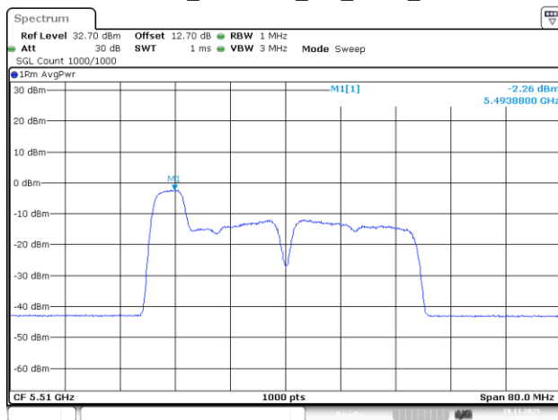
802.11be40_5510MHz_RU_52/37_Chain 3
