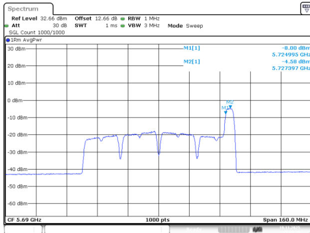
802.11be80_5690MHz_RU_52/52_Chain 0
