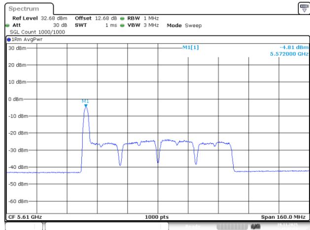
802.11be80_5610MHz_RU_26/0_Chain 2
