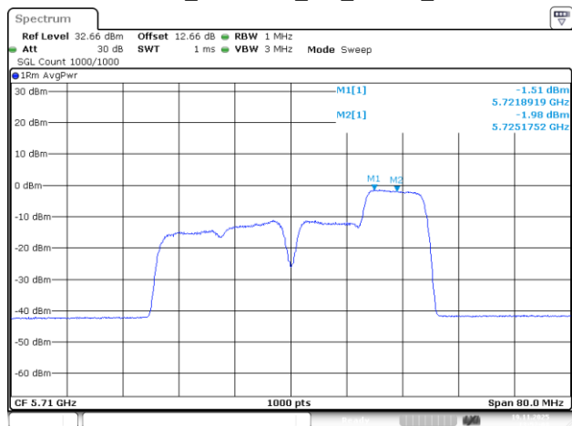
802.11be40_5710MHz_RU_106/56_Chain 1
