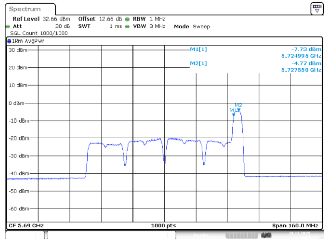
802.11be80_5690MHz_RU_52/52_Chain 1
