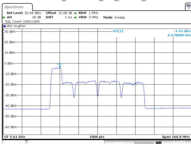
802.11be80_5610MHz_RU_106/53_Chain 2
