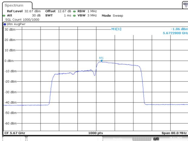
802.11be40_5670MHz_RU_242/62_Chain 0
