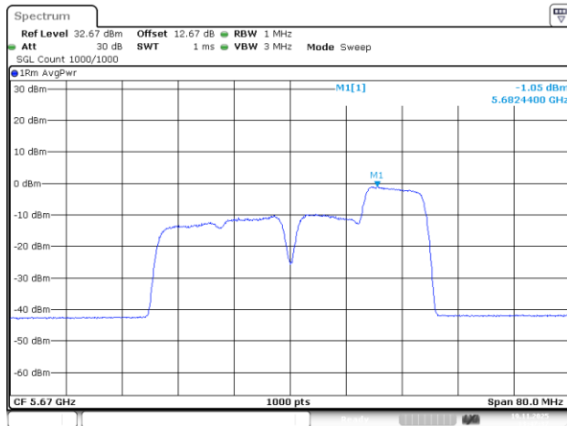
802.11be40_5670MHz_RU_106/56_Chain 0
