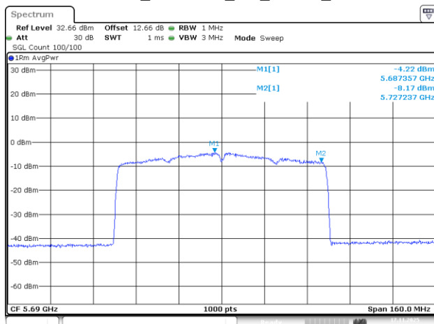
802.11be80_5690MHz_RU_996/67_Chain 0
