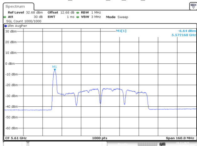
802.11be80_5610MHz_RU_26/0_Chain 3
