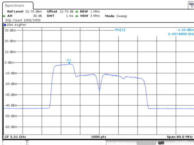
802.11be40_5510MHz_RU_106/53_Chain 2
