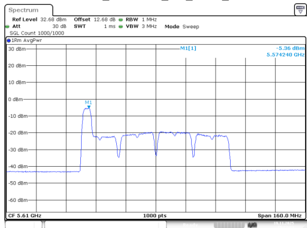
802.11be80_5610MHz_RU_52/37_Chain 1
