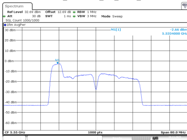
802.11be40_5550MHz_RU_52/37_Chain 1
