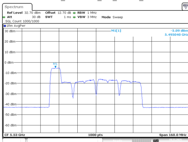
802.11be80_5530MHz_RU_106/53_Chain 2
