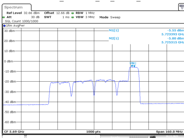
802.11be80_5690MHz_RU_106/60_Chain 3
