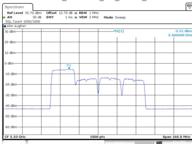
802.11be80_5530MHz_RU_242/61_Chain 2
