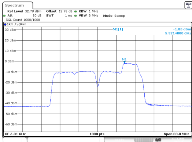
802.11be40_5310MHz_RU_26&52_MRU6_Chain 2
