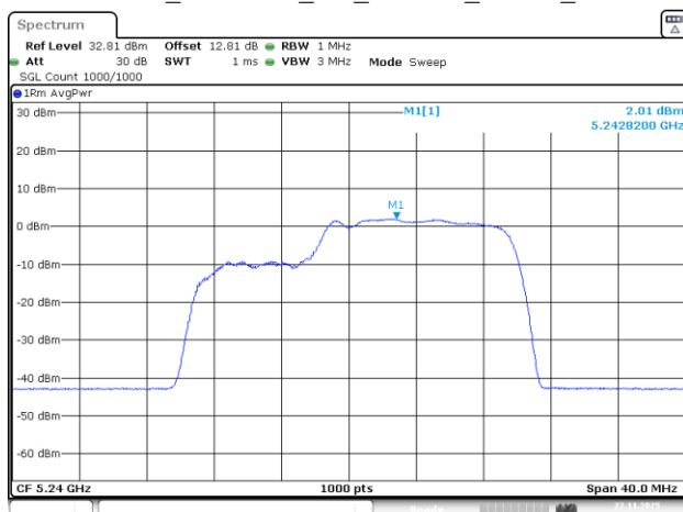
802.11be20_5240MHz_RU_26&106_MRU2_Chain 0
