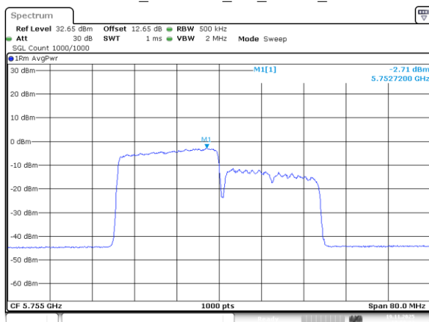
802.11be40_5755MHz_RU_242/61_Chain 2
