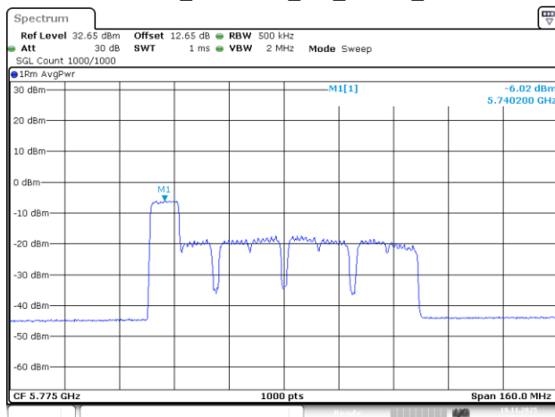
802.11be80_5775MHz_RU_106/53_Chain 2
