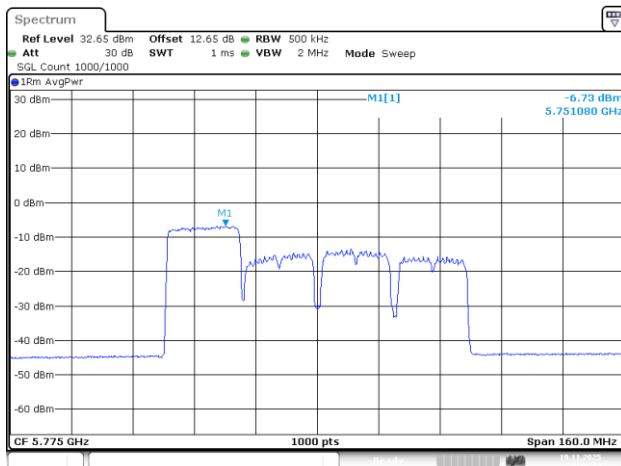
802.11be80_5775MHz_RU_242/61_Chain 1
