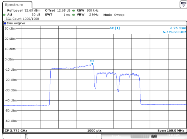
802.11be80_5775MHz_RU_484/65_Chain 1
