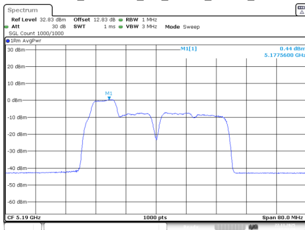
802.11be40_5190MHz_RU_26&52_MRU1_Chain 1
