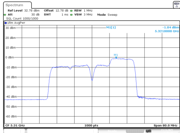
802.11be40_5310MHz_RU_26&106_MRU4_Chain 0
