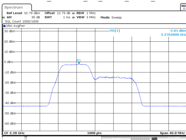
802.11be20_5280MHz_RU_26&52_MRU1_Chain 2
