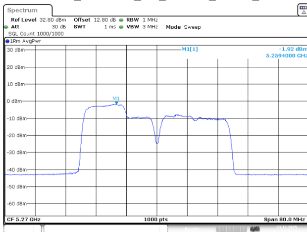
802.11be40_5270MHz_RU_26&106_MRU1_Chain 3
