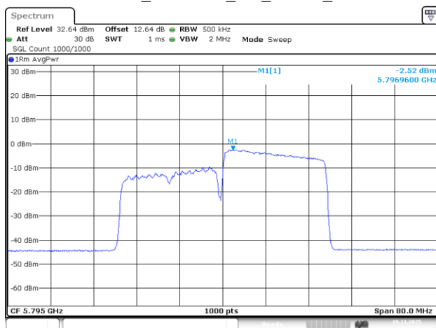
802.11be40_5795MHz_RU_242/62_Chain 0
