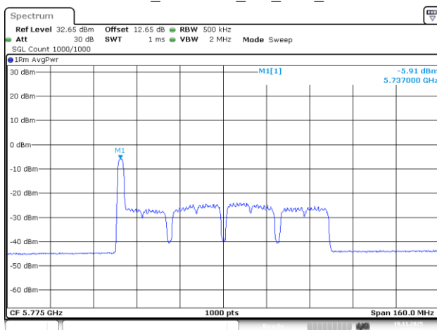
802.11be80_5775MHz_RU_26/0_Chain 1
