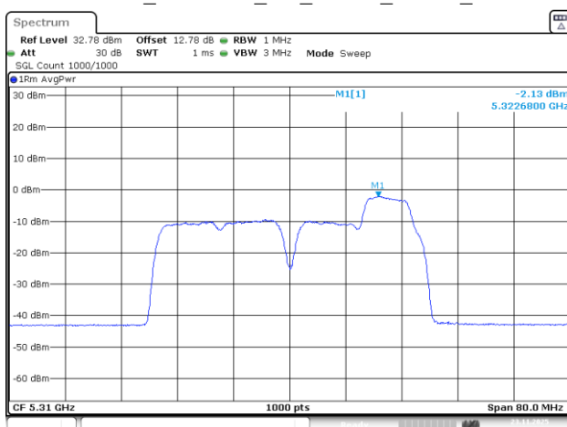
802.11be40_5310MHz_RU_26&52_MRU6_Chain 1
