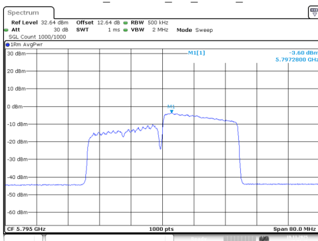
802.11be40_5795MHz_RU_242/62_Chain 3
