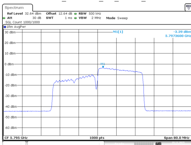
802.11be40_5795MHz_RU_242/62_Chain 2
