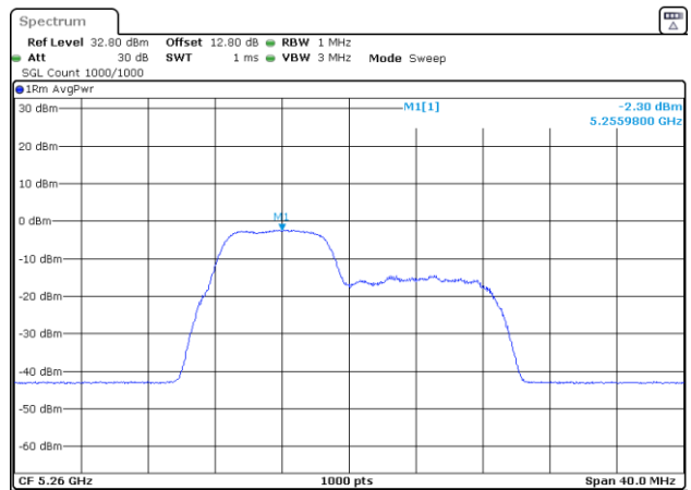
802.11be20_5260MHz_RU_26&52_MRUI_Chain 1
