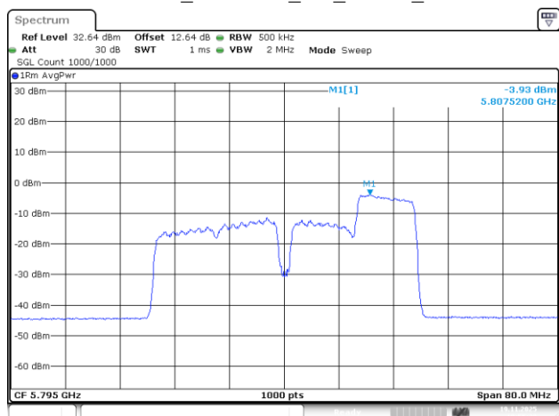
802.11be40_5795MHz_RU_106/56_Chain 3
