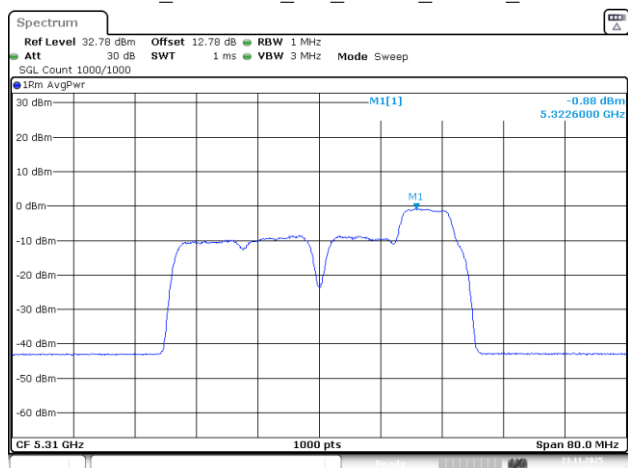
802.11be40_5310MHz_RU_26&52_MRU6_Chain 3
