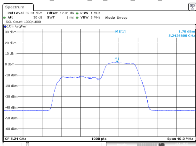
802.11be20_5240MHz_RU_26&52_MRU3_Chain 3
