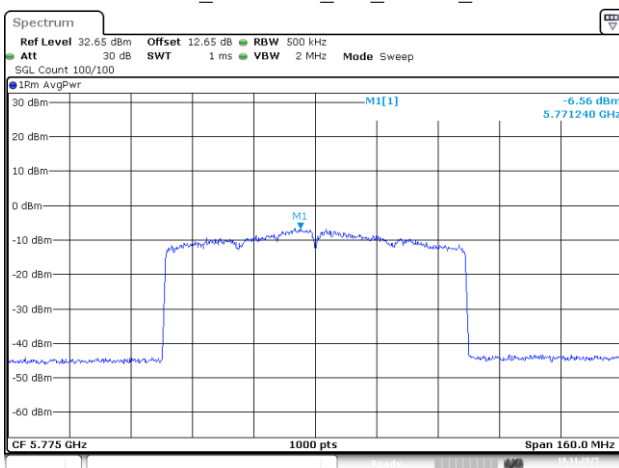
802.11be80_5775MHz_RU_996/67_Chain 3
