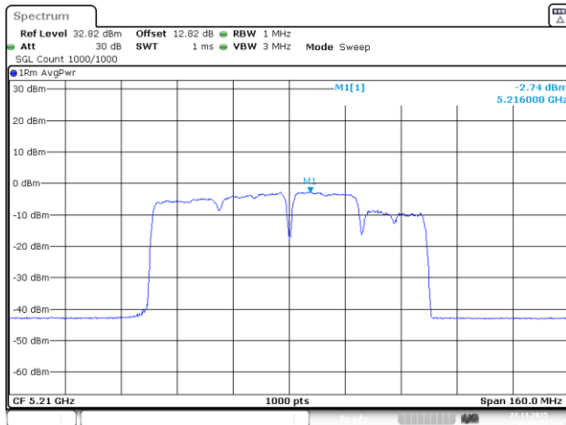
802.11be80_5210MHz_RU_242&484_MRU4_Chain 0
