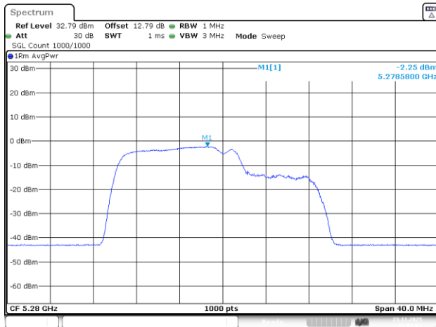
802.11be20_5280MHz_RU_26&106_MRU1_Chain 1
