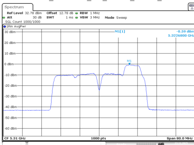
802.11be40_5310MHz_RU_26&52_MRU6_Chain 0
