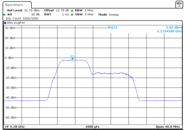
802.11be20_5280MHz_RU_26&52_MRUI_Chain 0
