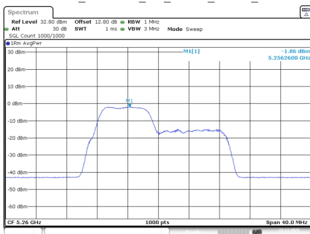
802.11be20_5260MHz_RU_26&52_MRU1_Chain 2
