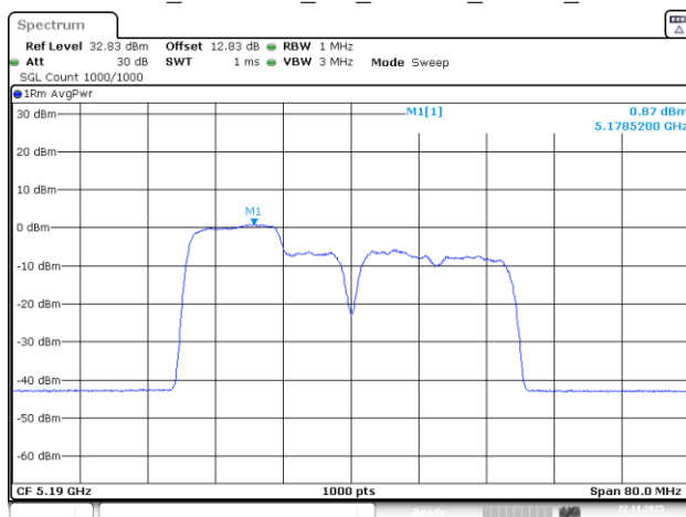
802.11be40_5190MHz_RU_26&106_MRU1_Chain 3
