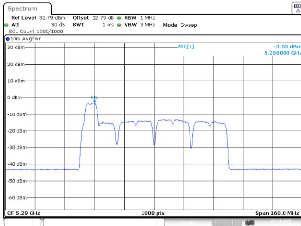
802.11be80_5290MHz_RU_26&52_MRU2_Chain 0
