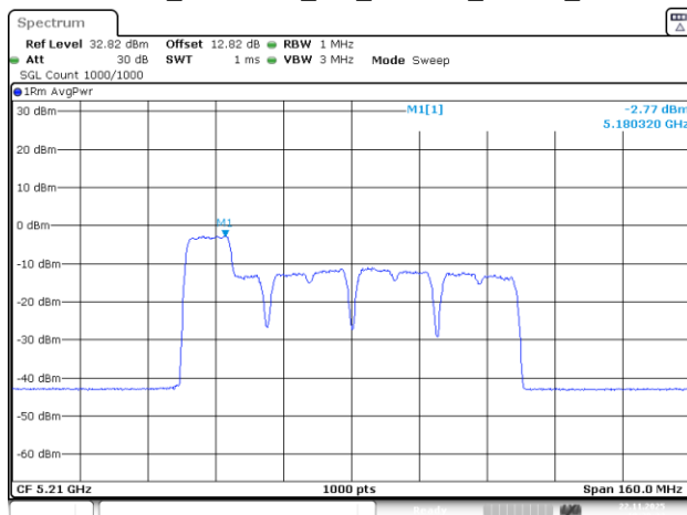
802.11be80_5210MHz_RU_26&106_MRU1_Chain 0
