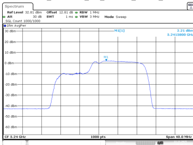
802.11be20_5240MHz_RU_26&106_MRU2_Chain 2
