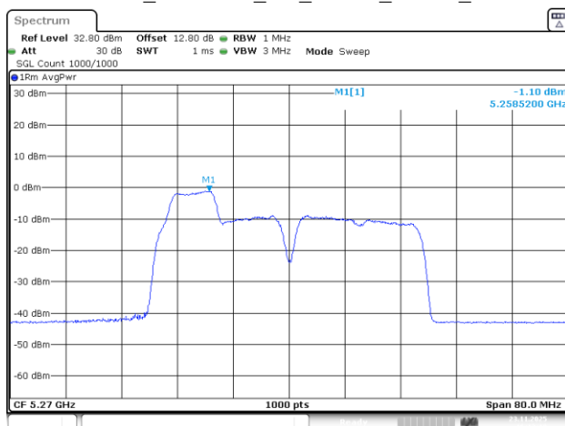
802.11be40_5270MHz_RU_26&52_MRU1_Chain 3
