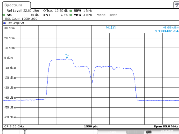
802.11be40_5270MHz_RU_26&106_MRU1_Chain 0
