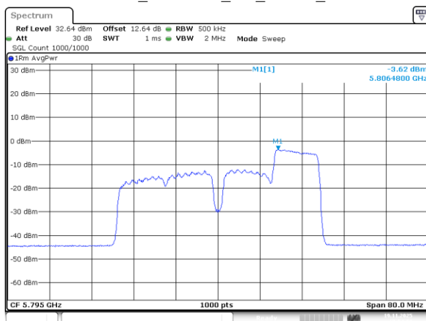
802.11be40_5795MHz_RU_106/56_Chain 2
