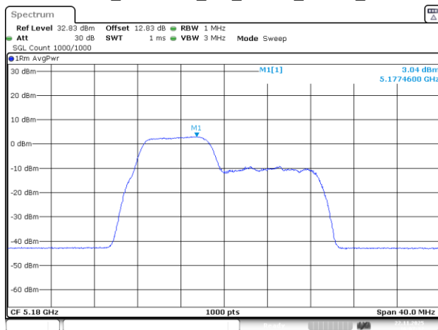
802.11be20_5180MHz_RU_26&52_MRU1_Chain 2
