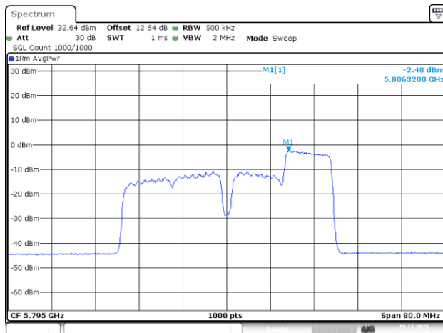
802.11be40_5795MHz_RU_106/56_Chain 0
