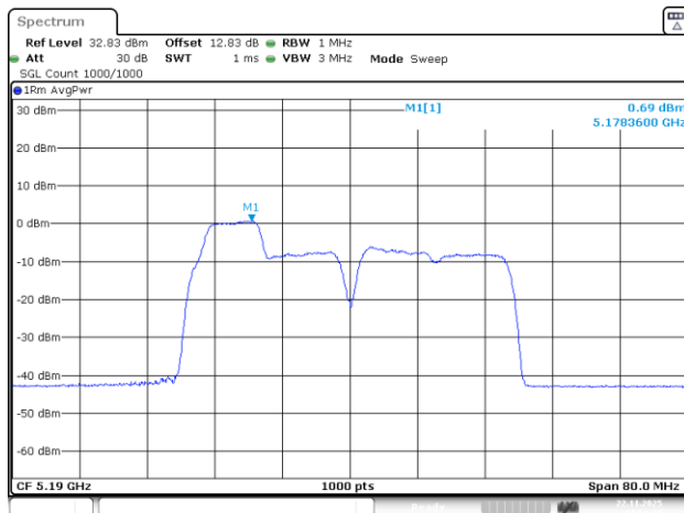
802.11be40_5190MHz_RU_26&52_MRU1_Chain 2
