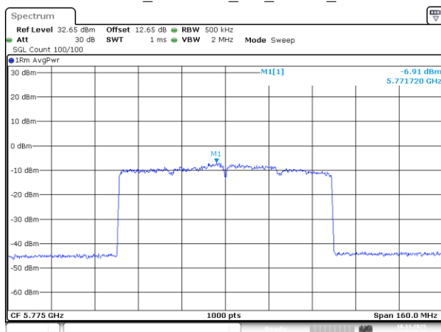
802.11be80_5775MHz_RU_996/67_Chain 2
