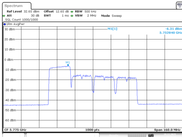
802.11be80_5775MHz_RU_242/61_Chain 0
