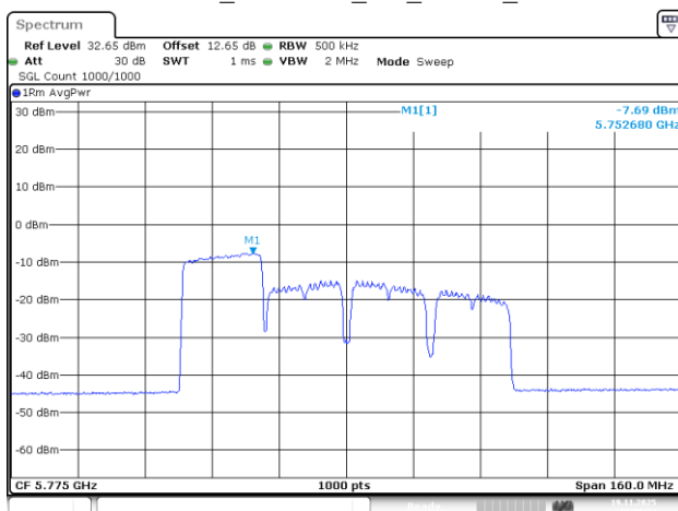
802.11be80_5775MHz_RU_242/61_Chain 3
