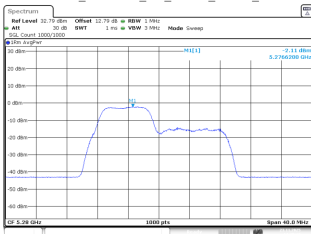
802.11be20_5280MHz_RU_26&52_MRU1_Chain 1
