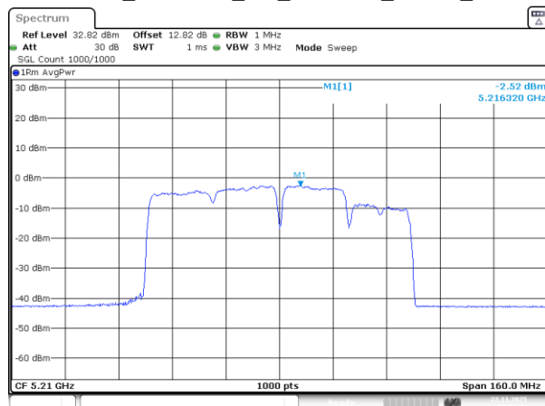
802.11be80_5210MHz_RU_242&484_MRU4_Chain 2
