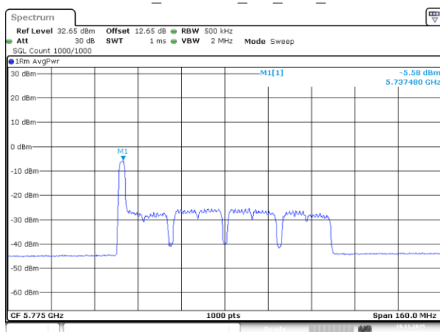
802.11be80_5775MHz_RU_26/0_Chain 2
