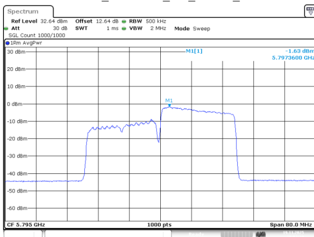
802.11be40_5795MHz_RU_242/62_Chain 1
