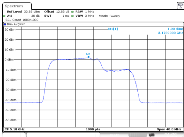
802.11be20_5180MHz_RU_26&106_MRU1_Chain 3
