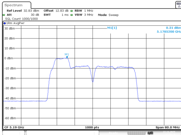
802.11be40_5190MHz_RU_26&52_MRU1_Chain 0
