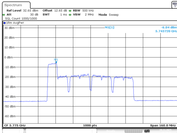
802.11be80_5775MHz_RU_106/53_Chain 0
