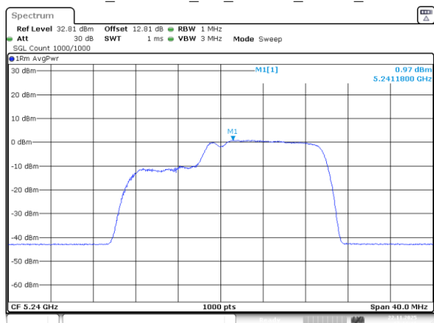
802.11be20_5240MHz_RU_26&106_MRU2_Chain 3
