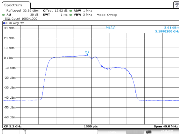
802.11be20_5200MHz_RU_26&106_MRU1_Chain 1
