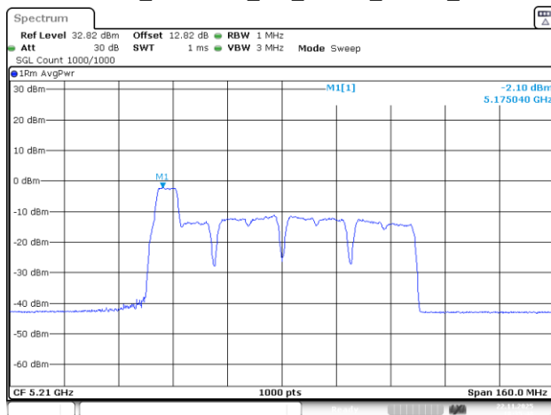
802.11be80_5210MHz_RU_26&52_MRU2_Chain 2
