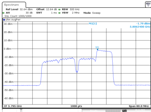
802.11be40_5795MHz_RU_106/56_Chain 1
