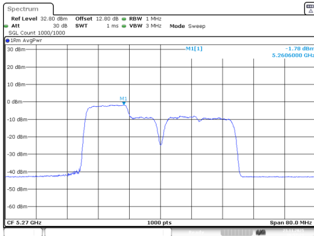
802.11be40_5270MHz_RU_26&106_MRU1_Chain 2
