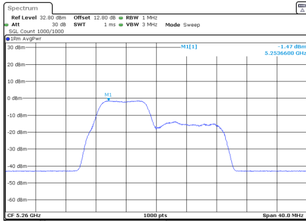
802.11be20_5260MHz_RU_26&52_MRUI_Chain 0
