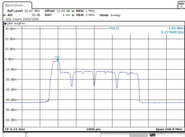
802.11be80_5210MHz_RU_26&52_MRU2_Chain 1
