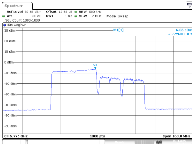
802.11be80_5775MHz_RU_484/65_Chain 2
