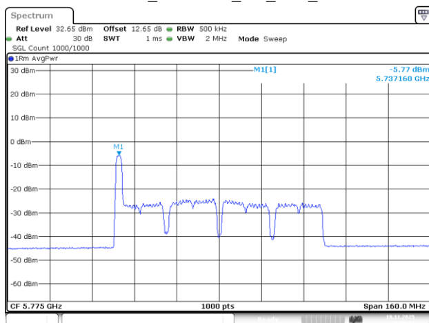
802.11be80_5775MHz_RU_26/0_Chain 0
