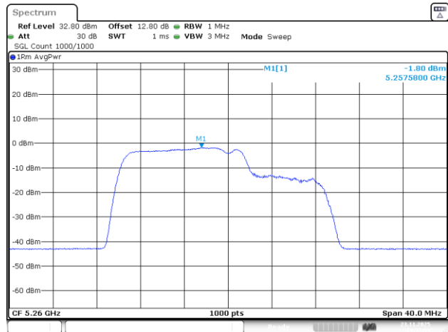
802.11be20_5260MHz_RU_26&106_MRU1_Chain 3
