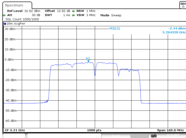
802.11be80_5210MHz_RU_242&484_MRU4_Chain 1
