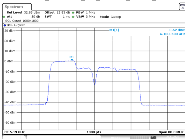
802.11be40_5190MHz_RU_26&106_MRU1_Chain 1
