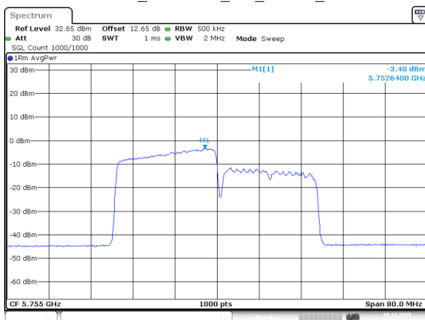
802.11be40_5755MHz_RU_242/61_Chain 3
