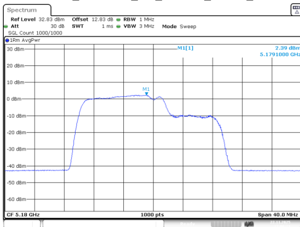
802.11be20_5180MHz_RU_26&106_MRU1_Chain 2
