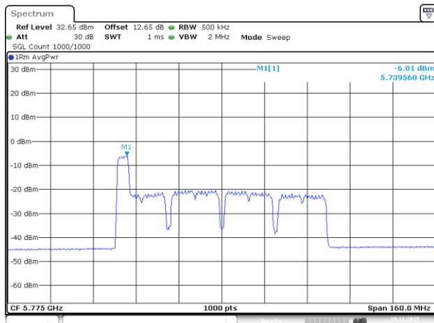
802.11be80_5775MHz_RU_52/37_Chain 0
