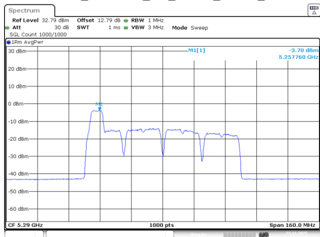
802.11be80_5290MHz_RU_26&52_MRU2_Chain 3
