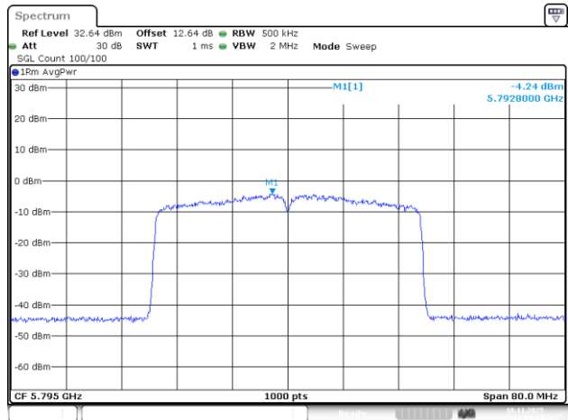
802.11be40_5795MHz_RU_484/65_Chain 2
