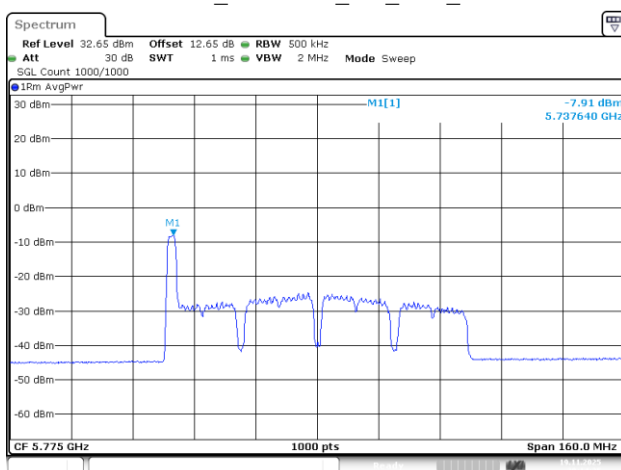
802.11be80_5775MHz_RU_26/0_Chain 3
