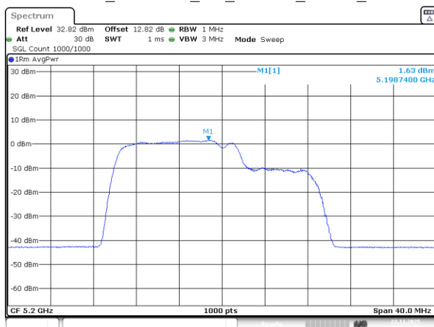
802.11be20_5200MHz_RU_26&106_MRU1_Chain 3
