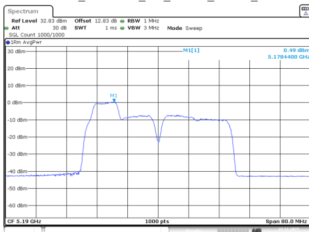
802.11be40_5190MHz_RU_26&52_MRU1_Chain 3
