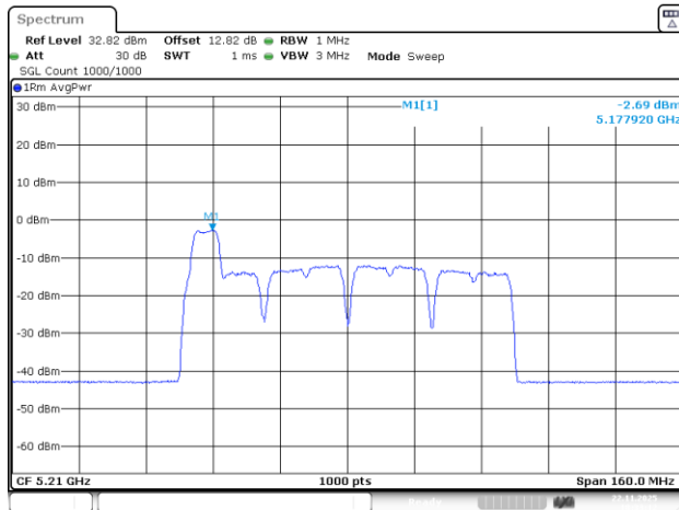
802.11be80_5210MHz_RU_26&52_MRU2_Chain 0
