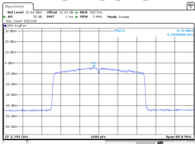
802.11be40_5795MHz_RU_484/65_Chain 3
