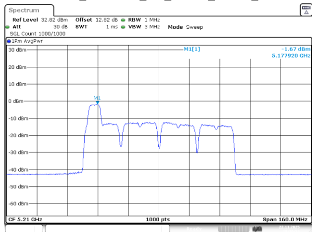
802.11be80_5210MHz_RU_26&52_MRU2_Chain 3
