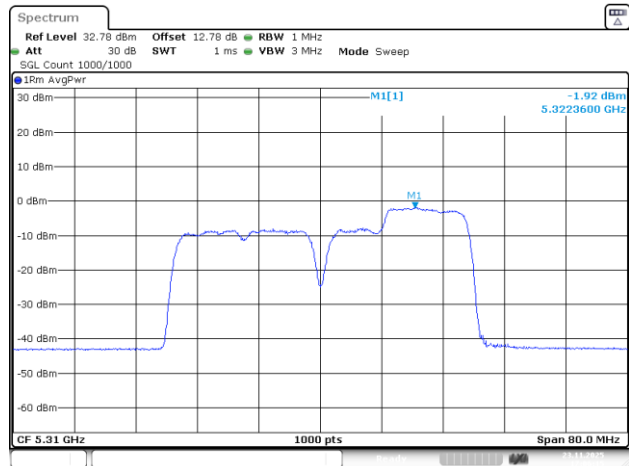
802.11be40_5310MHz_RU_26&106_MRU4_Chain 2
