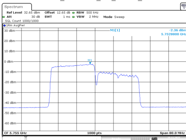
802.11be40_5755MHz_RU_242/61_Chain 1
