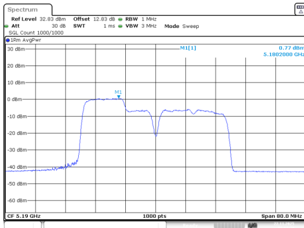
802.11be40_5190MHz_RU_26&106_MRU1_Chain 2
