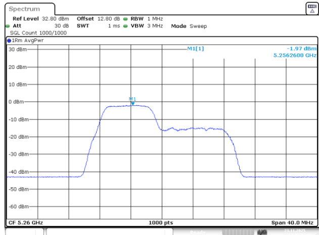
802.11be20_5260MHz_RU_26&52_MRU1_Chain 3
