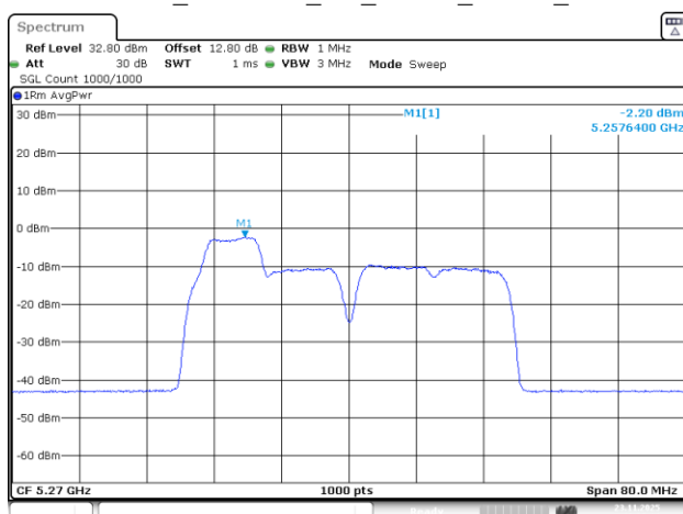
802.11be40_5270MHz_RU_26&52_MRU1_Chain 1
