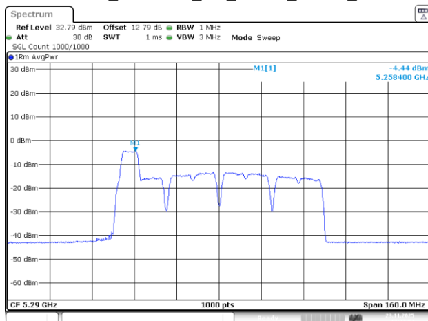
802.11be80_5290MHz_RU_26&52_MRU2_Chain 2
