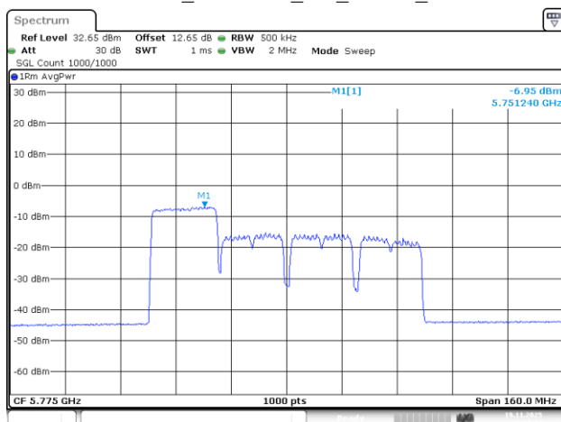
802.11be80_5775MHz_RU_242/61_Chain 2
