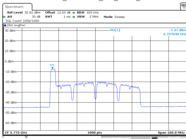
802.11be80_5775MHz_RU_52/37_Chain 3
