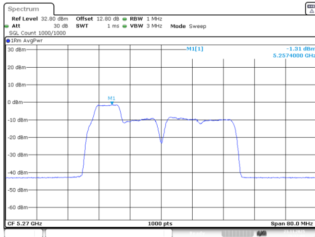
802.11be40_5270MHz_RU_26&52_MRU1_Chain 2
