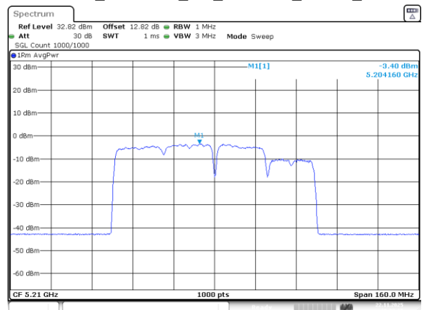
802.11be80_5210MHz_RU_242&484_MRU4_Chain 3
