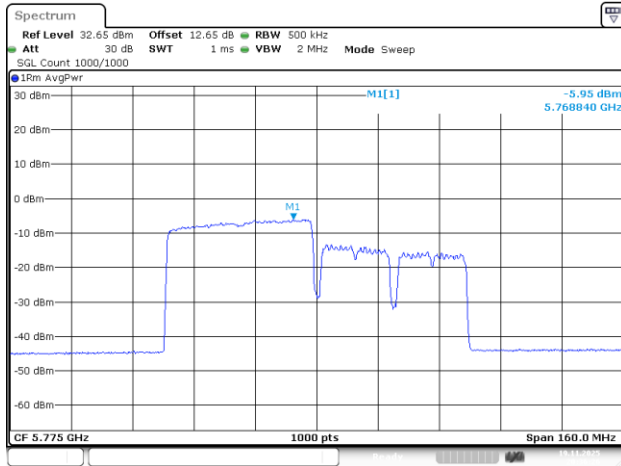
802.11be80_5775MHz_RU_484/65_Chain 0
