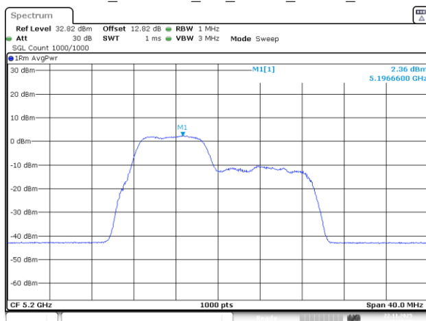
802.11be20_5200MHz_RU_26&52_MRU1_Chain 3
