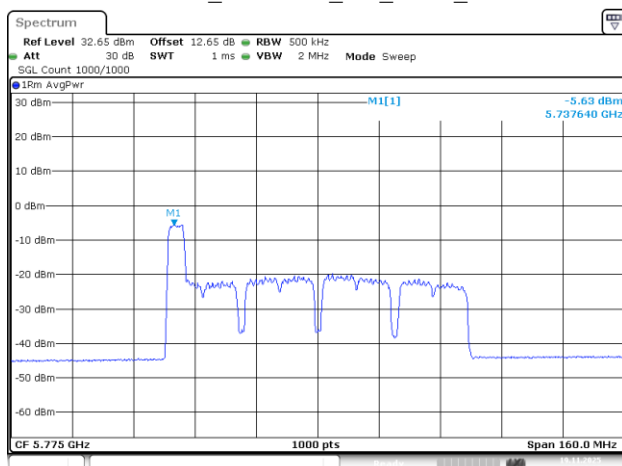
802.11be80_5775MHz_RU_52/37_Chain 2
