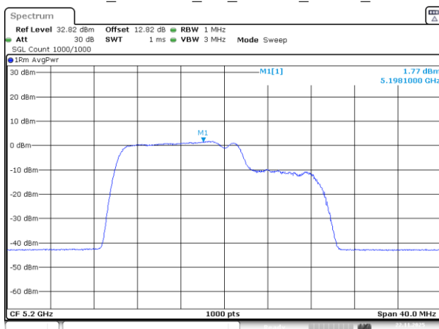
802.11be20_5200MHz_RU_26&106_MRU1_Chain 0
