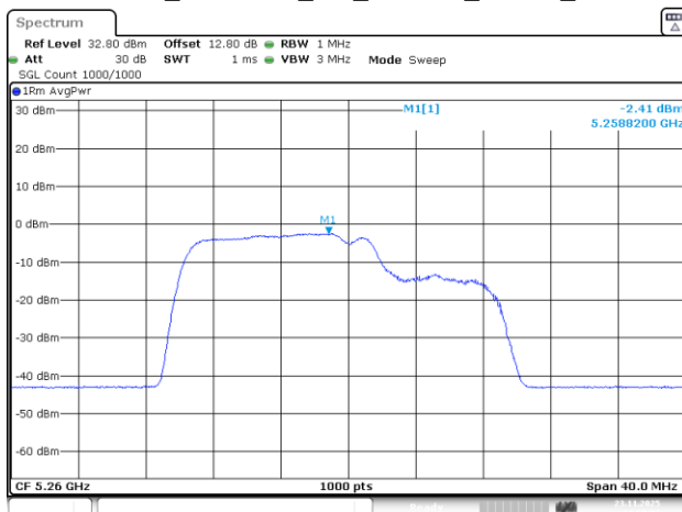
802.11be20_5260MHz_RU_26&106_MRU1_Chain 2
