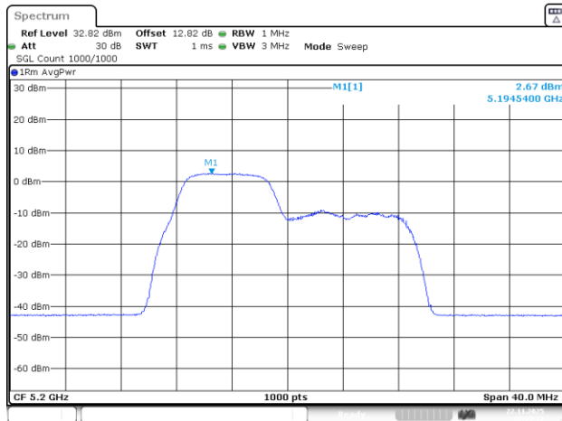
802.11be20_5200MHz_RU_26&52_MRU1_Chain 1
