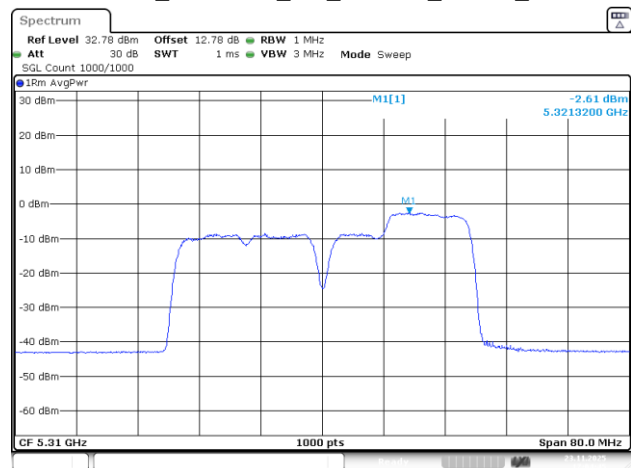
802.11be40_5310MHz_RU_26&106_MRU4_Chain 1
