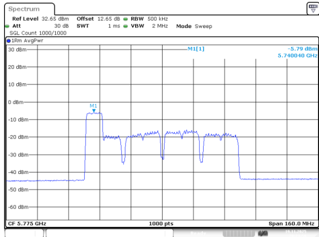
802.11be80_5775MHz_RU_106/53_Chain 1
