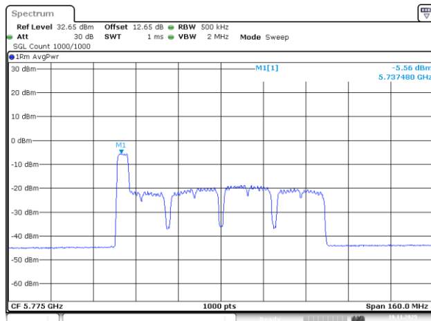
802.11be80_5775MHz_RU_52/37_Chain 1
