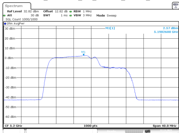
802.11be20_5200MHz_RU_26&106_MRU1_Chain 2
