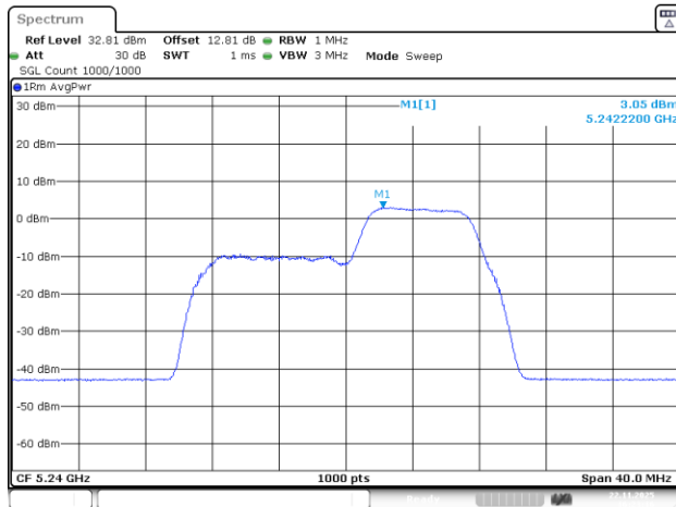
802.11be20_5240MHz_RU_26&52_MRU3_Chain 2
