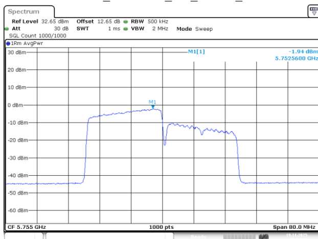
802.11be40_5755MHz_RU_242/61_Chain 0
