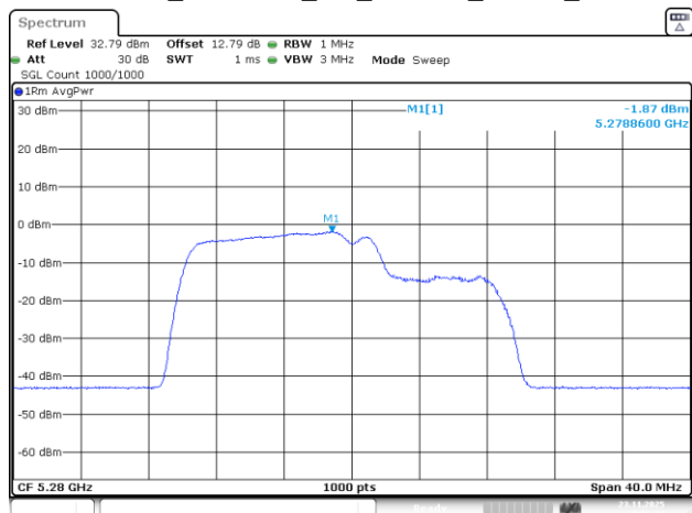
802.11be20_5280MHz_RU_26&106_MRU1_Chain 2
