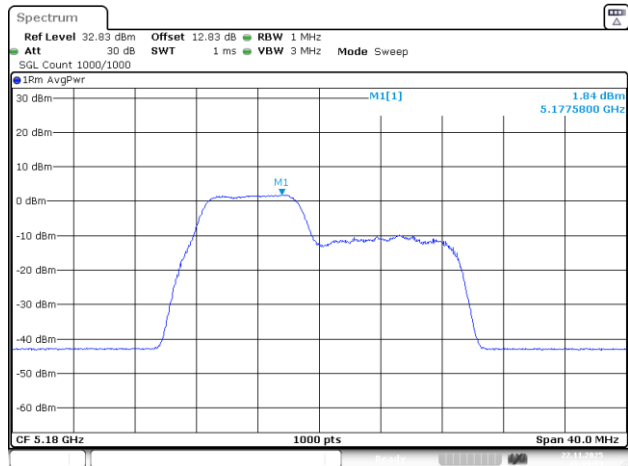
802.11be20_5180MHz_RU_26&52_MRU1_Chain 3
