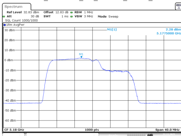
802.11be20_5180MHz_RU_26&106_MRU1_Chain 0
