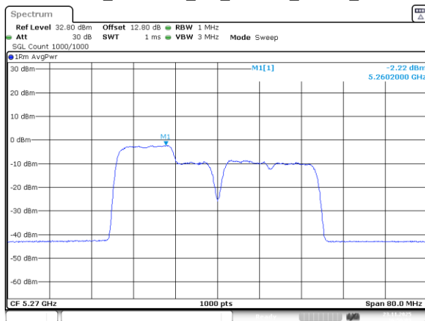
802.11be40_5270MHz_RU_26&106_MRU1_Chain 1
