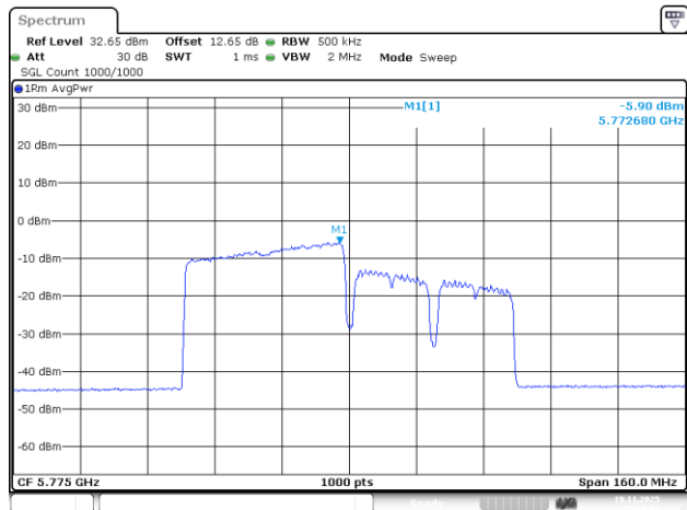
802.11be80_5775MHz_RU_484/65_Chain 3
