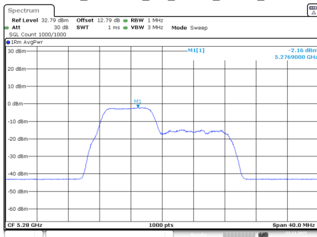
802.11be20_5280MHz_RU_26&52_MRU1_Chain 3
