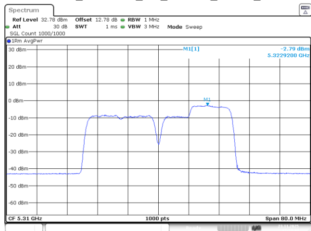
802.11be40_5310MHz_RU_26&106_MRU4_Chain 3
