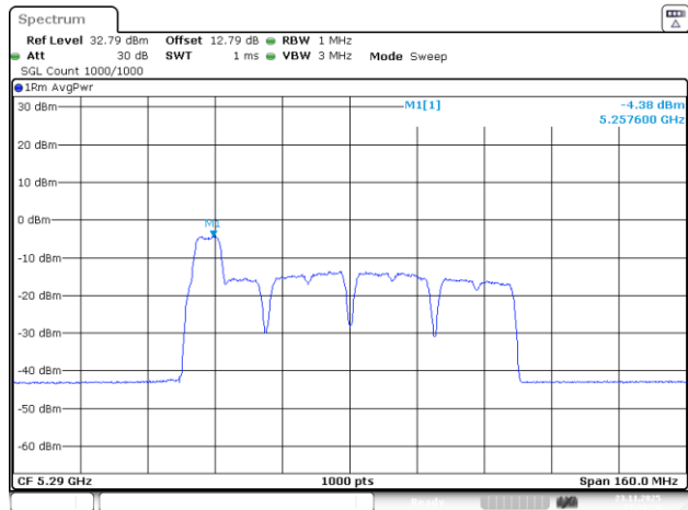
802.11be80_5290MHz_RU_26&52_MRU2_Chain 1
