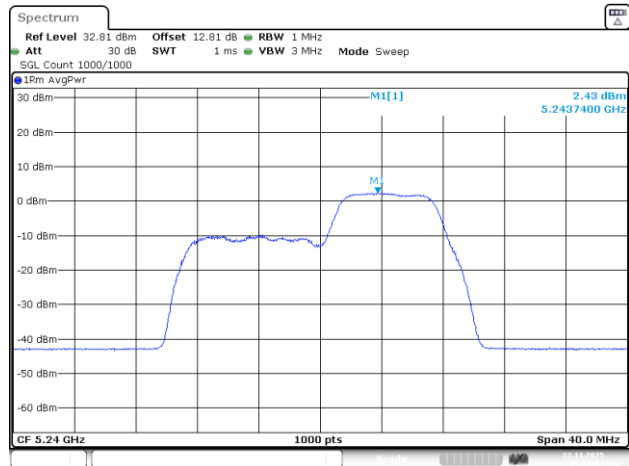
802.11be20_5240MHz_RU_26&52_MRU3_Chain 1
