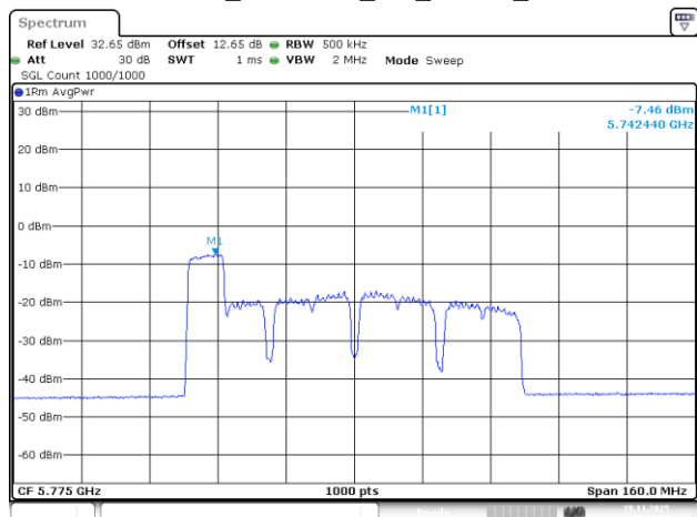
802.11be80_5775MHz_RU_106/53_Chain 3
