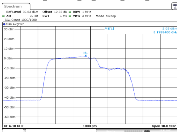
802.11be20_5180MHz_RU_26&106_MRU1_Chain 1
