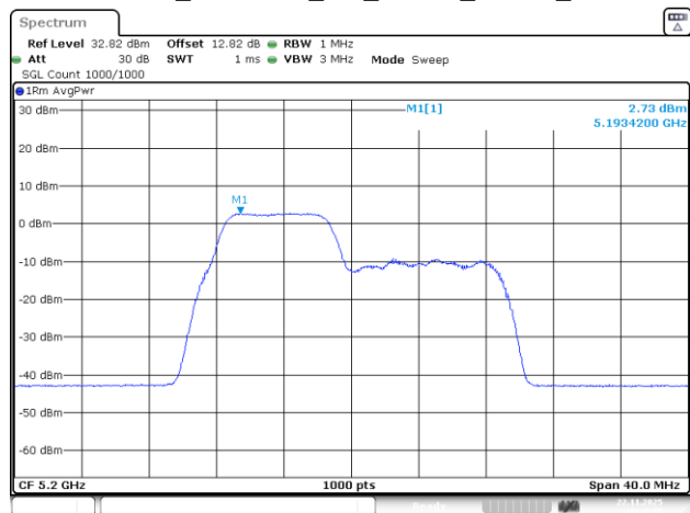
802.11be20_5200MHz_RU_26&52_MRU1_Chain 2
