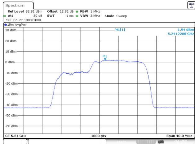
802.11be20_5240MHz_RU_26&106_MRU2_Chain 1
