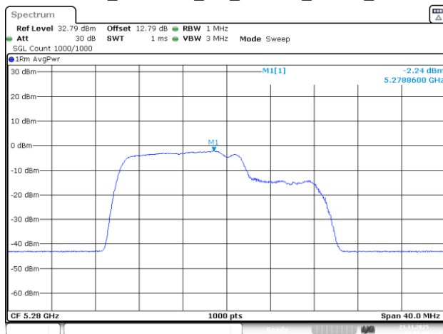
802.11be20_5280MHz_RU_26&106_MRU1_Chain 3
