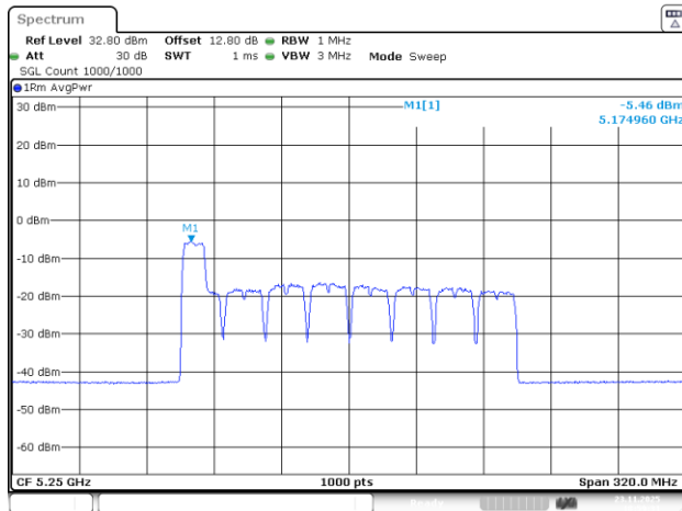
802.11be160_5250MHz_RU_26&106_MRU1_Chain 0
