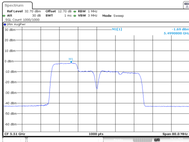
802.11be40_5510MHz_RU_26&106_MRU1_Chain 0
