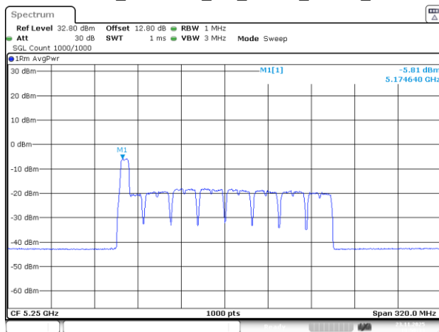
802.11be160_5250MHz_RU_26&52_MRU2_Chain 0
