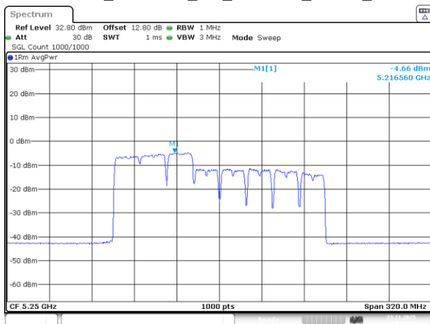
802.11be160_5250MHz_RU_242&484_MRU8_Chain 2
