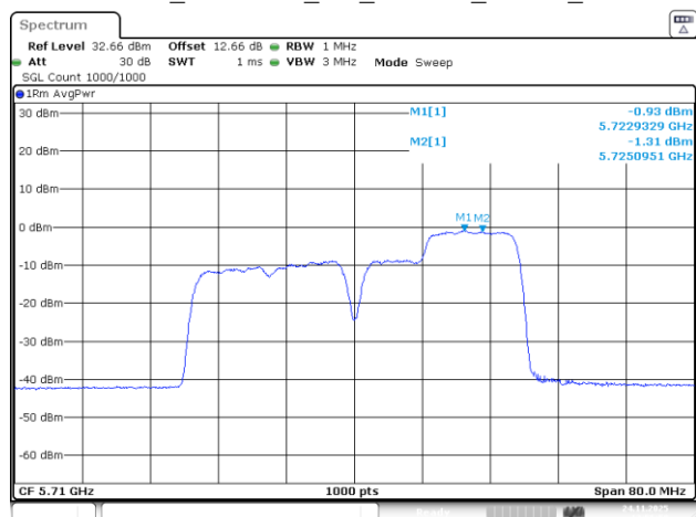
802.11be40_5710MHz_RU_26&106_MRU4_Chain 1
