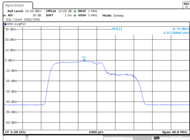
802.11be20_5580MHz_RU_26&106_MRU1_Chain 1
