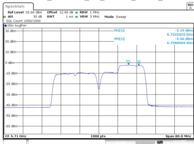
802.11be40_5710MHz_RU_26&106_MRU4_Chain 0
