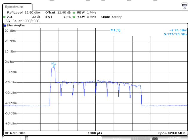
802.11be160_5250MHz_RU_26&52_MRU2_Chain 3
