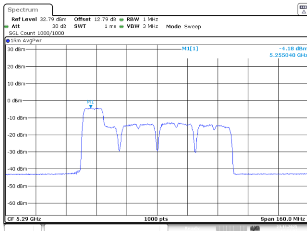
802.11be80_5290MHz_RU_26&106_MRU1_Chain 0
