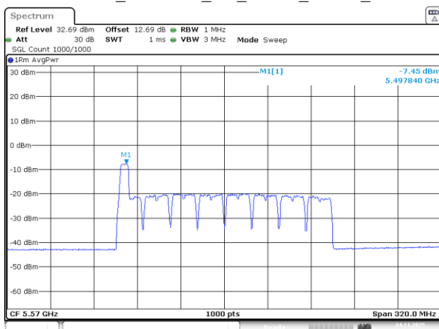
802.11be160_5570MHz_RU_26&52_MRU2_Chain 3
