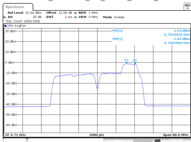
802.11be40_5710MHz_RU_26&52_MRU6_Chain 2
