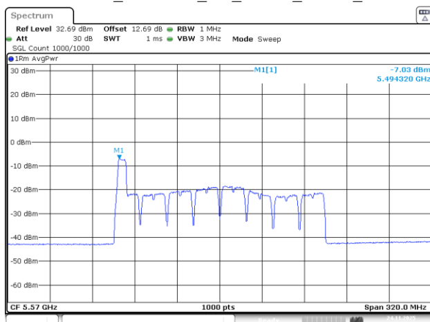
802.11be160_5570MHz_RU_26&52_MRU2_Chain 0
