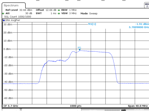
802.11be20_5700MHz_RU_26&106_MRU2_Chain 0
