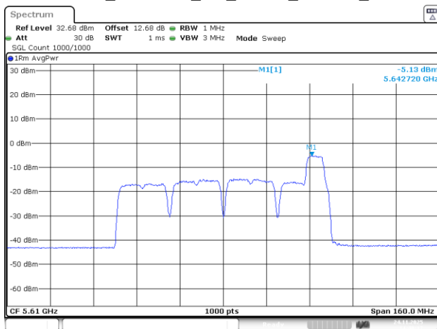
802.11be80_5610MHz_RU_26&52_MRU11_Chain 3
