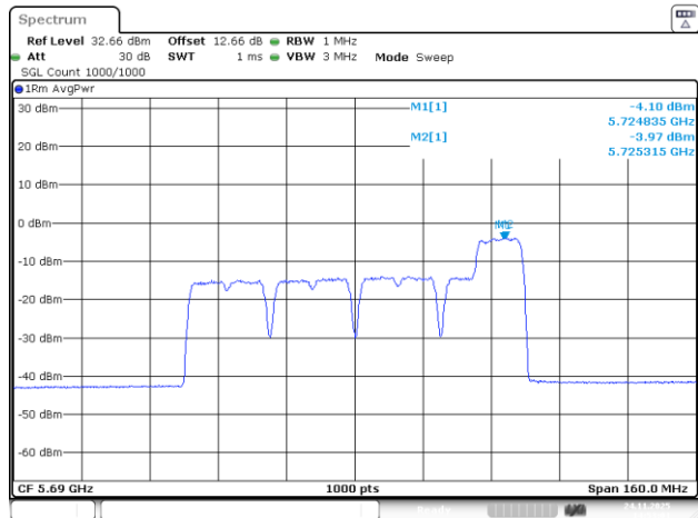
802.11be80_5690MHz_RU_26&106_MRU8_Chain 1
