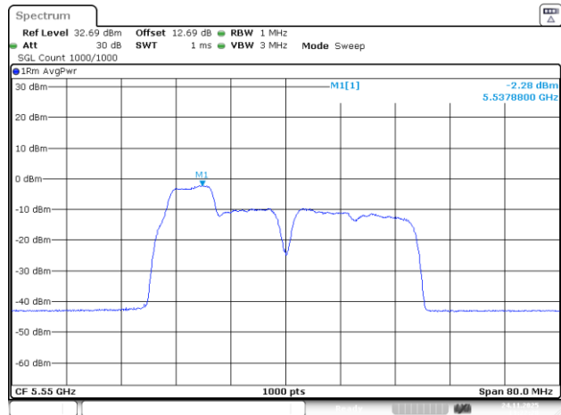
802.11be40_5550MHz_RU_26&52_MRU1_Chain 1
