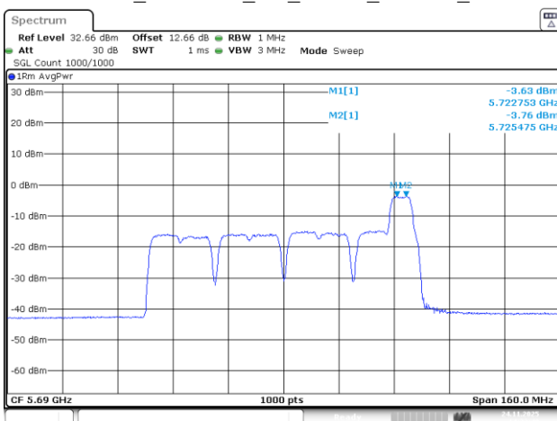
802.11be80_5690MHz_RU_26&52_MRU11_Chain 1
