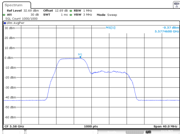
802.11be20_5580MHz_RU_26&52_MRU1_Chain 2
