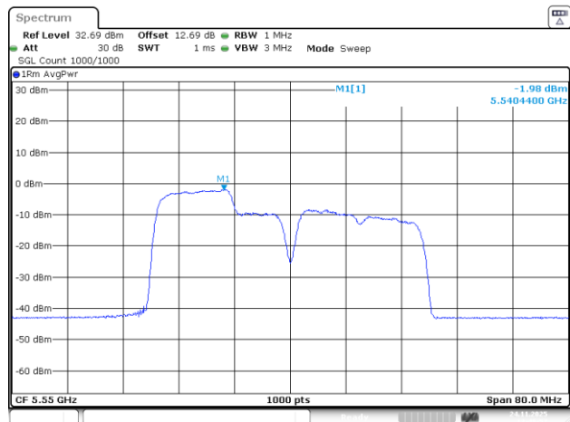
802.11be40_5550MHz_RU_26&106_MRU1_Chain 1
