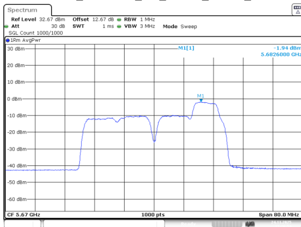
802.11be40_5670MHz_RU_26&52_MRU6_Chain 1
