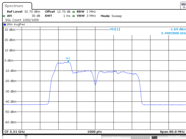
802.11be40_5510MHz_RU_26&52_MRU1_Chain 2
