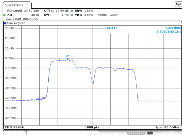
802.11be40_5550MHz_RU_26&106_MRU1_Chain 0
