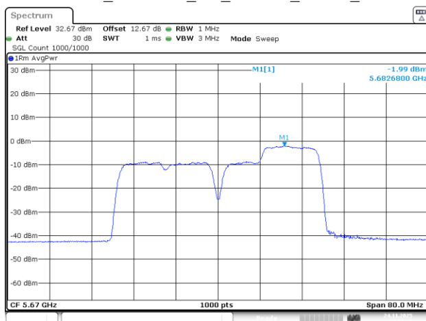
802.11be40_5670MHz_RU_26&106_MRU4_Chain 1
