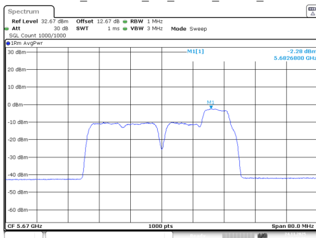
802.11be40_5670MHz_RU_26&52_MRU6_Chain 2
