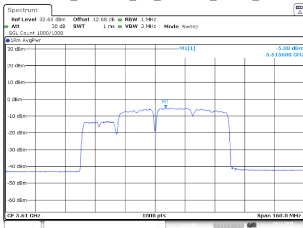
802.11be80_5610MHz_RU_242&484_MRU1_Chain 3
