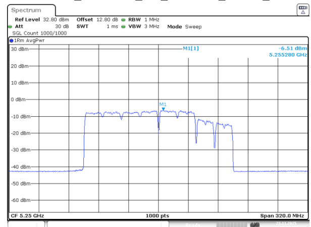
802.11be160_5250MHz_RU_484&996_MRU4_Chain 3
