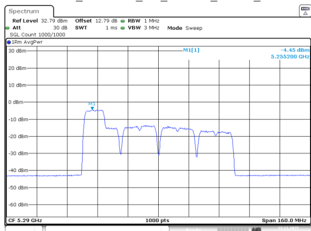
802.11be80_5290MHz_RU_26&106_MRU1_Chain 3
