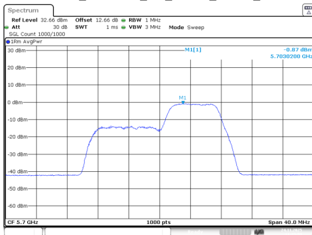
802.11be20_5700MHz_RU_26&52_MRU3_Chain 1
