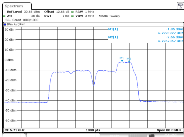
802.11be40_5710MHz_RU_26&52_MRU6_Chain 0
