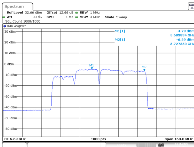
802.11be80_5690MHz_RU_242&484_MRU1_Chain 0
