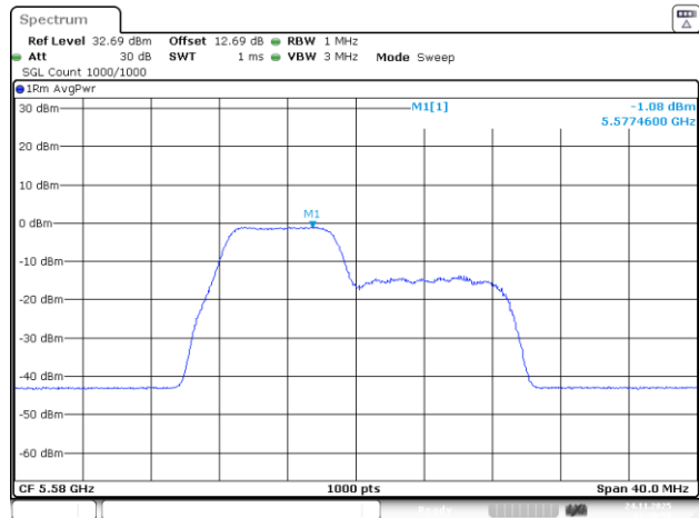
802.11be20_5580MHz_RU_26&52_MRU1_Chain 1
