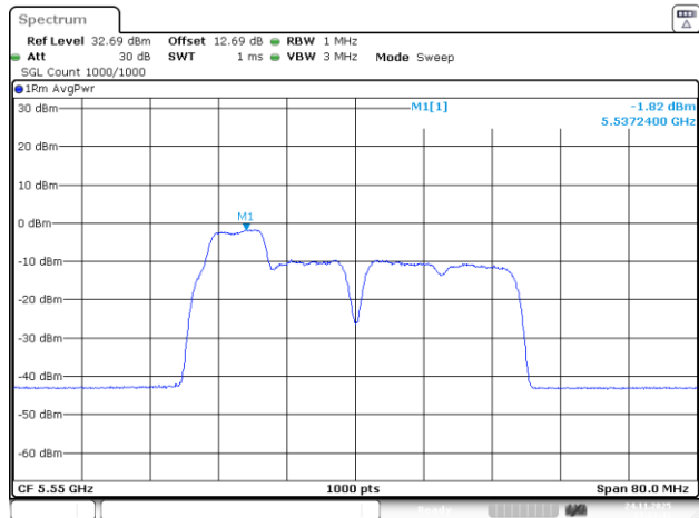
802.11be40_5550MHz_RU_26&52_MRU1_Chain 0
