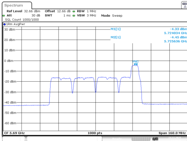
802.11be80_5690MHz_RU_26&52_MRU11_Chain 2
