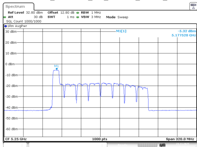
802.11be160_5250MHz_RU_26&106_MRU1_Chain 3
