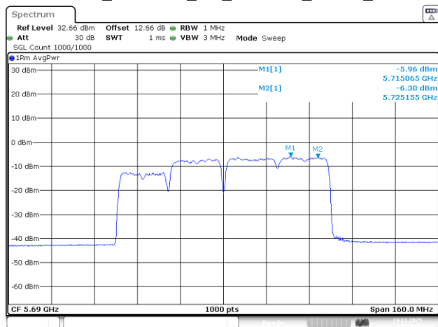
802.11be80_5690MHz_RU_242&484_MRU1_Chain 3
