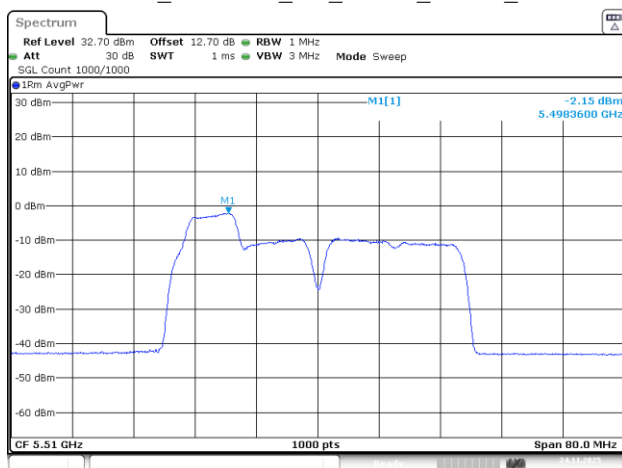
802.11be40_5510MHz_RU_26&52_MRU1_Chain 3
