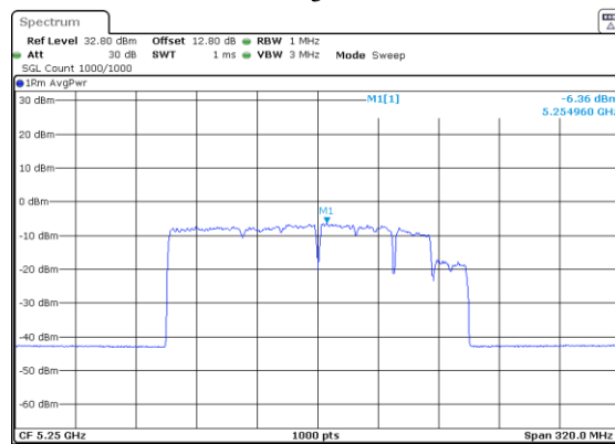
802.11be160_5250MHz_RU_242&484&996_MRU8_Chain 3
