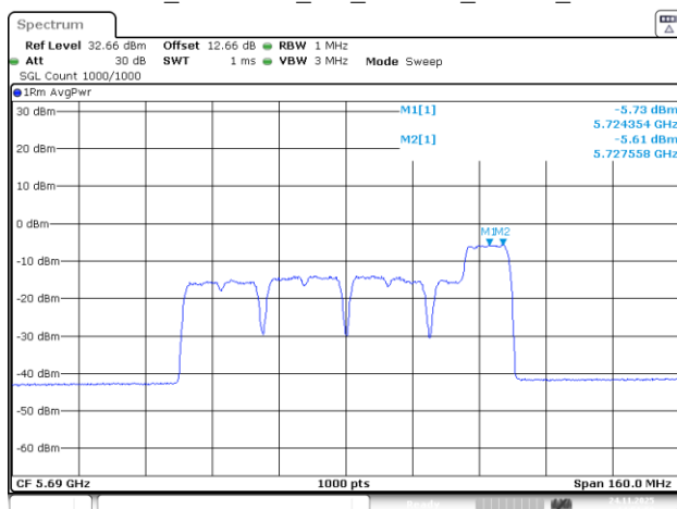
802.11be80_5690MHz_RU_26&106_MRU8_Chain 0
