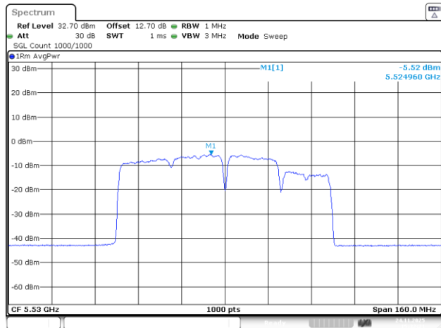
802.11be80_5530MHz_RU_242&484_MRU4_Chain 3
