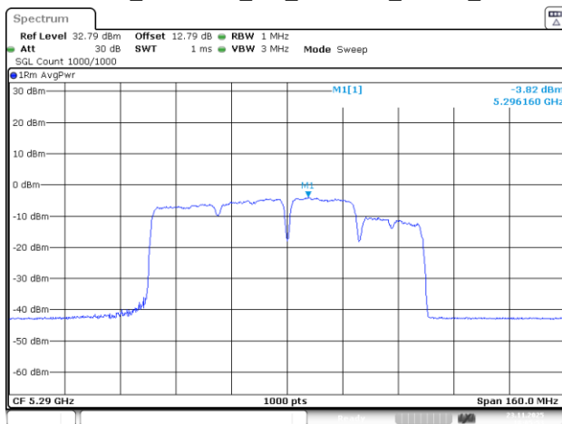
802.11be80_5290MHz_RU_242&484_MRU4_Chain 2
