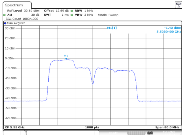
802.11be40_5550MHz_RU_26&106_MRU1_Chain 3
