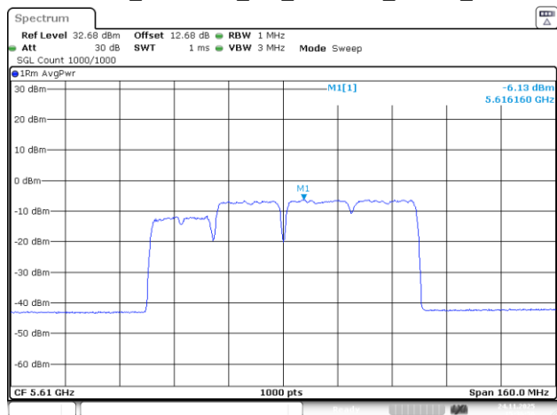
802.11be80_5610MHz_RU_242&484_MRU1_Chain 2
