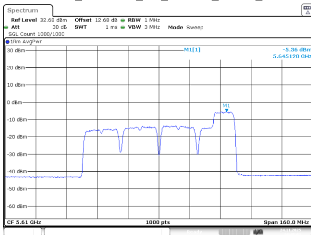
802.11be80_5610MHz_RU_26&106_MRU8_Chain 3
