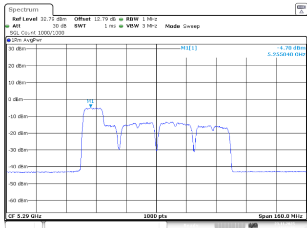
802.11be80_5290MHz_RU_26&106_MRU1_Chain 1
