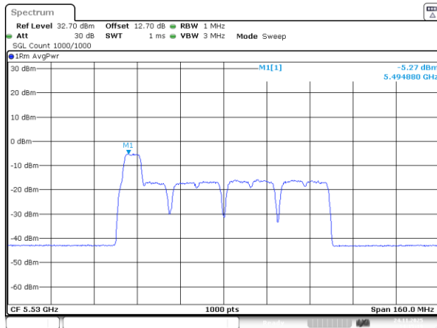
802.11be80_5530MHz_RU_26&52_MRU2_Chain 0
