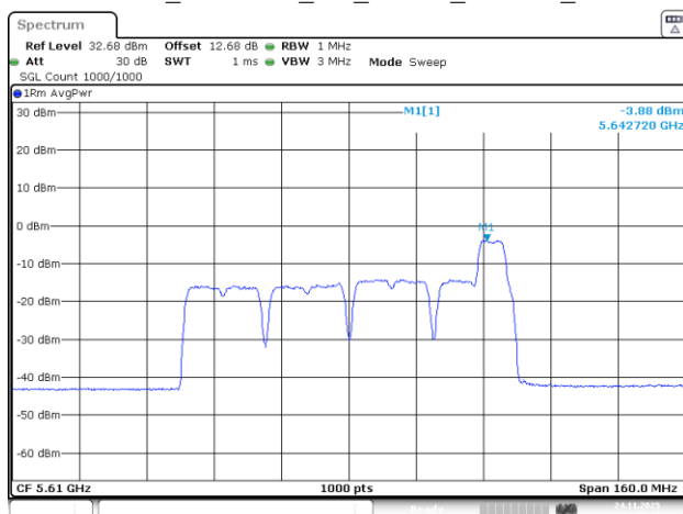
802.11be80_5610MHz_RU_26&52_MRU11_Chain 1
