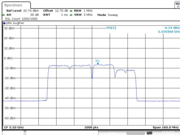
802.11be80_5530MHz_RU_242&484_MRU4_Chain 0
