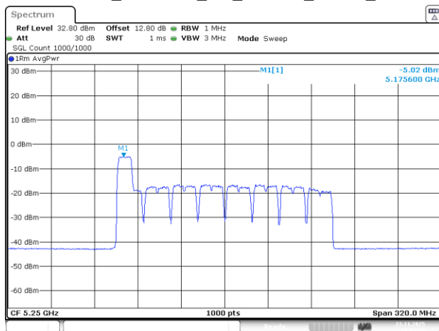
802.11be160_5250MHz_RU_26&106_MRU1_Chain 2
