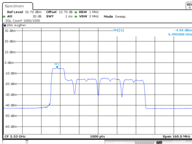
802.11be80_5530MHz_RU_26&106_MRU1_Chain 0
