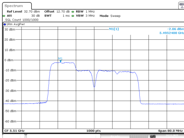
802.11be40_5510MHz_RU_26&106_MRU1_Chain 1
