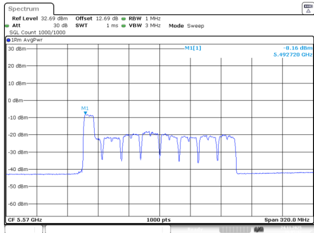
802.11be160_5570MHz_RU_26&106_MRU1_Chain 1
