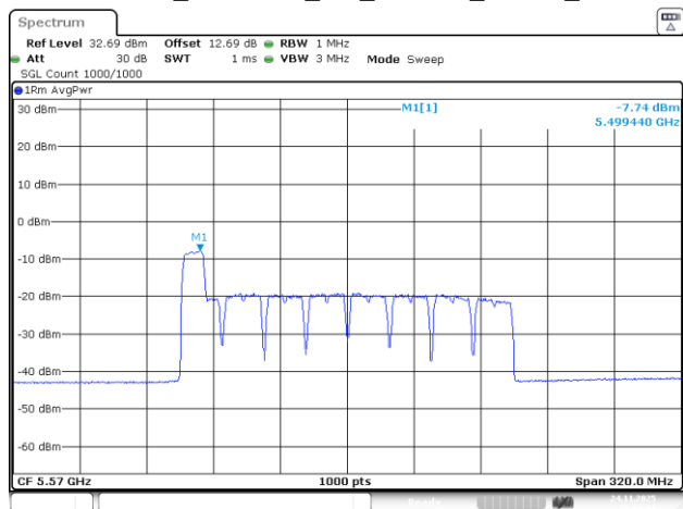
802.11be160_5570MHz_RU_26&106_MRU1_Chain 3
