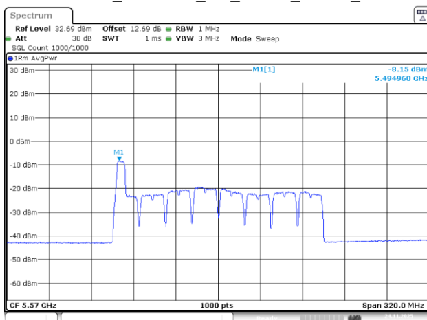
802.11be160_5570MHz_RU_26&52_MRU2_Chain 1
