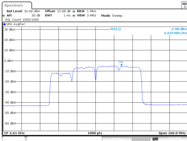
802.11be80_5610MHz_RU_242&484_MRU1_Chain 1
