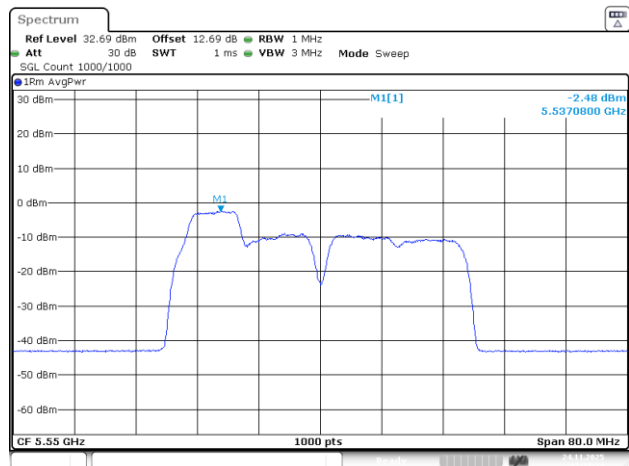
802.11be40_5550MHz_RU_26&52_MRU1_Chain 2
