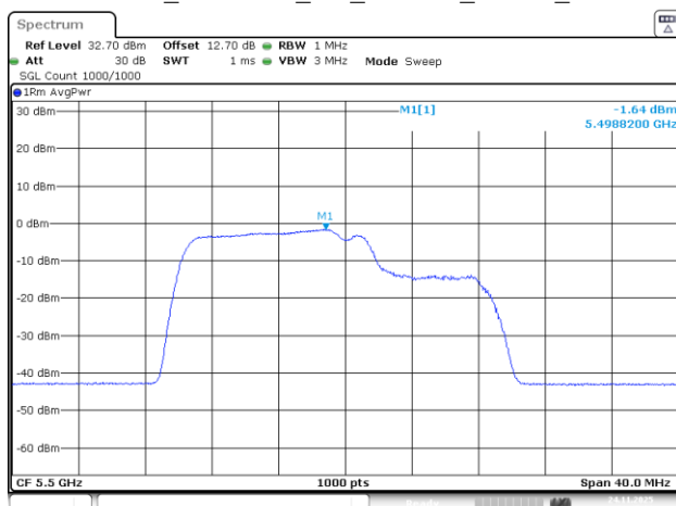
802.11be20_5500MHz_RU_26&106_MRU1_Chain 0
