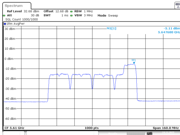
802.11be80_5610MHz_RU_26&106_MRU8_Chain 0
