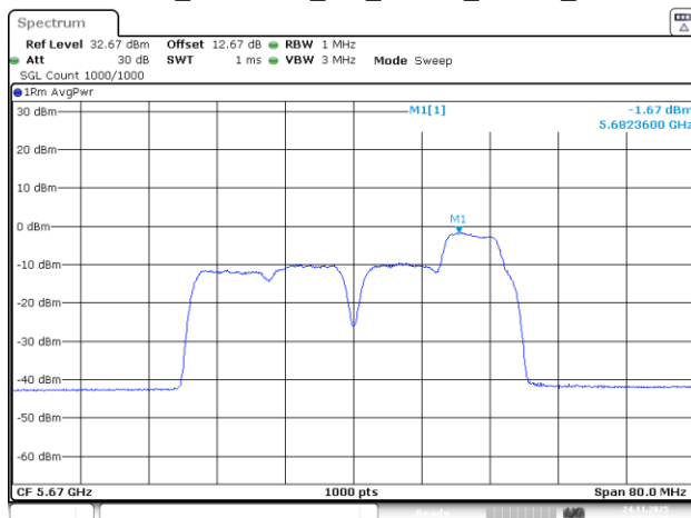
802.11be40_5670MHz_RU_26&52_MRU6_Chain 0
