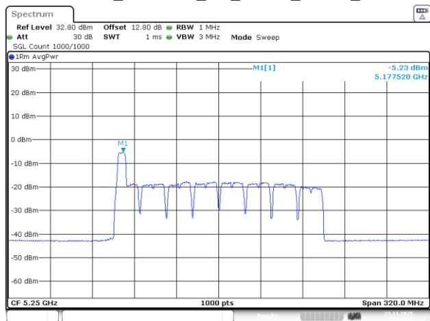
802.11be160_5250MHz_RU_26&52_MRU2_Chain 1
