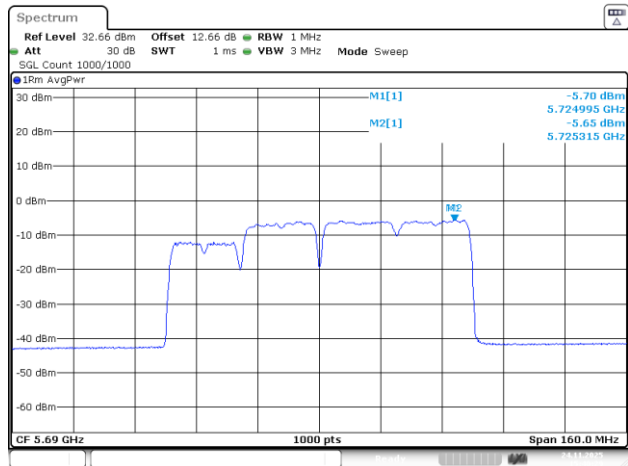
802.11be80_5690MHz_RU_242&484_MRU1_Chain 1
