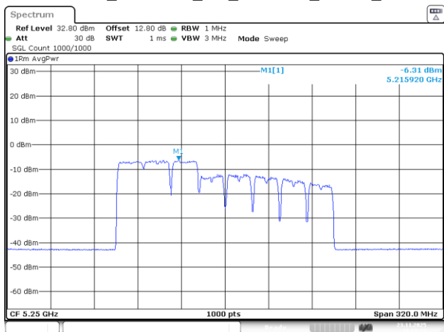
802.11be160_5250MHz_RU_242&484_MRU8_Chain 3
