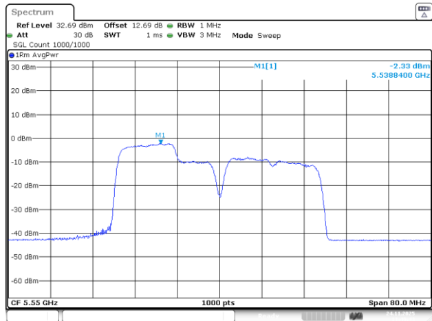
802.11be40_5550MHz_RU_26&106_MRU1_Chain 2
