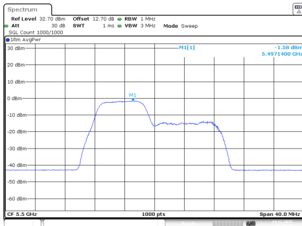
802.11be20_5500MHz_RU_26&52_MRU1_Chain 3
