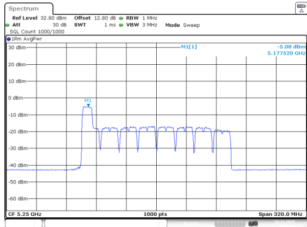
802.11be160_5250MHz_RU_26&106_MRU1_Chain 1
