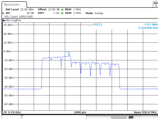
802.11be160_5250MHz_RU_242&484_MRU8_Chain 0
