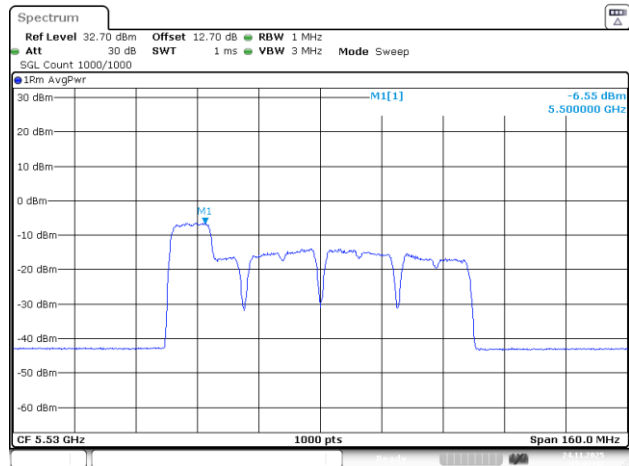
802.11be80_5530MHz_RU_26&106_MRU1_Chain 3
