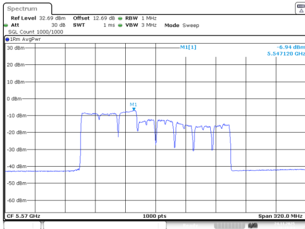
802.11be160_5570MHz_RU_242&484_MRU8_Chain 0
