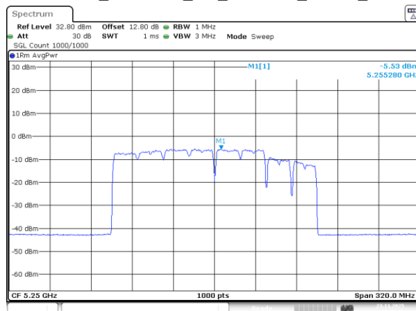
802.11be160_5250MHz_RU_484&996_MRU4_Chain 2
