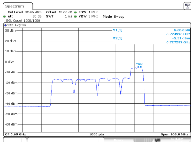
802.11be80_5690MHz_RU_26&106_MRU8_Chain 3
