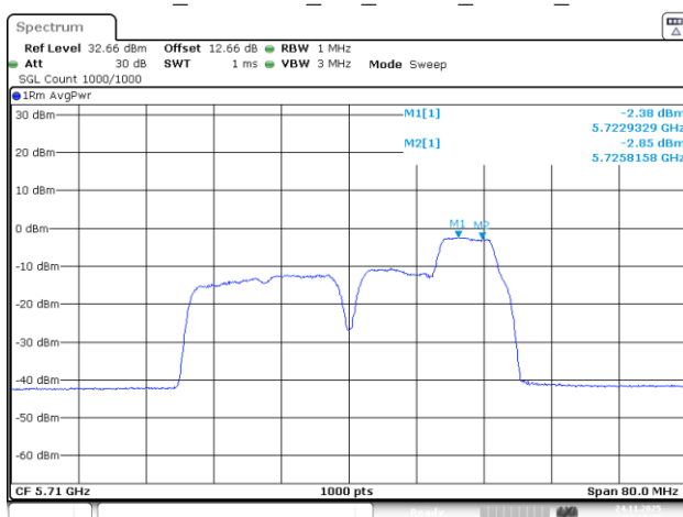
802.11be40_5710MHz_RU_26&52_MRU6_Chain 3
