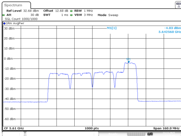
802.11be80_5610MHz_RU_26&106_MRU8_Chain 1
