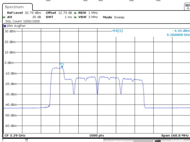
802.11be80_5290MHz_RU_26&106_MRU1_Chain 2
