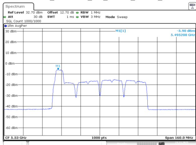
802.11be80_5530MHz_RU_26&52_MRU2_Chain 1
