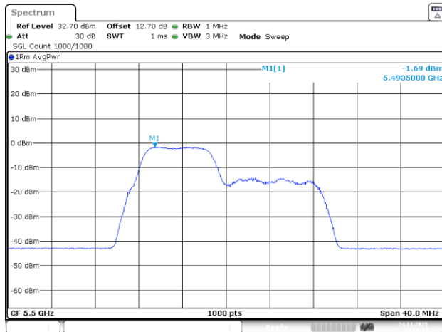
802.11be20_5500MHz_RU_26&52_MRU1_Chain 1
