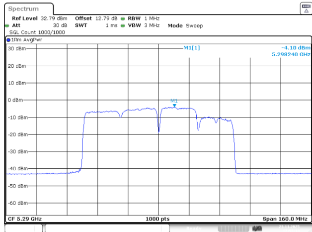
802.11be80_5290MHz_RU_242&484_MRU4_Chain 1
