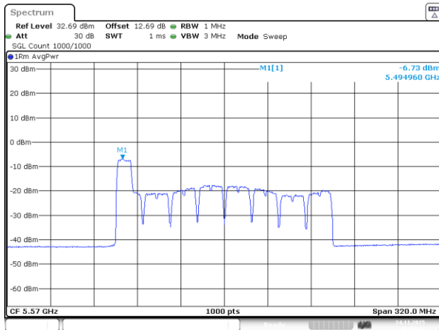
802.11be160_5570MHz_RU_26&106_MRU1_Chain 0
