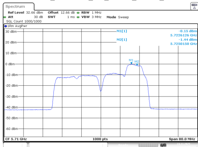
802.11be40_5710MHz_RU_26&52_MRU6_Chain 1
