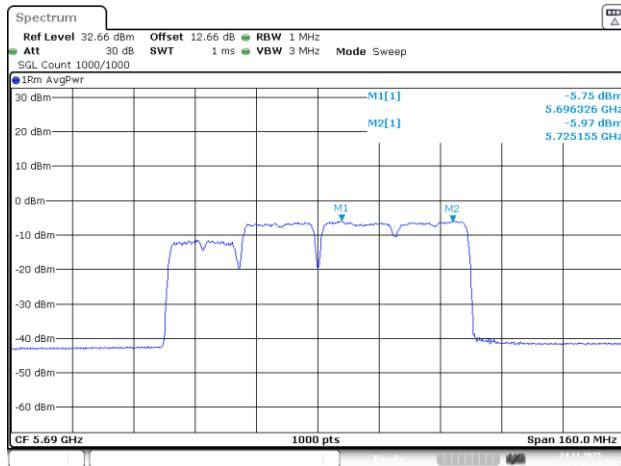
802.11be80_5690MHz_RU_242&484_MRU1_Chain 2
