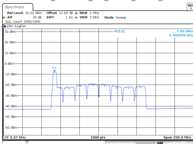
802.11be160_5570MHz_RU_26&52_MRU2_Chain 2
