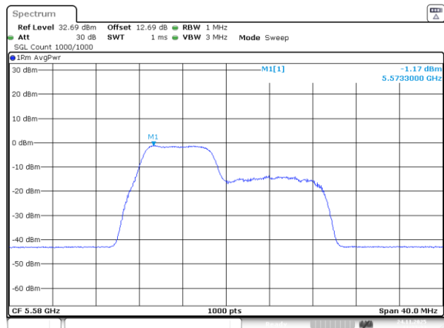
802.11be20_5580MHz_RU_26&52_MRU1_Chain 3
