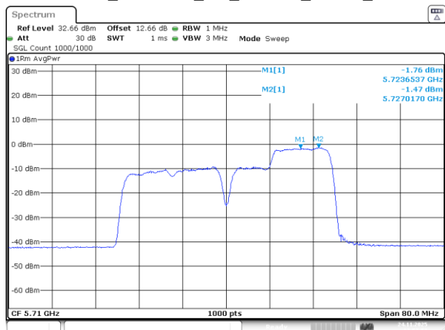
802.11be40_5710MHz_RU_26&106_MRU4_Chain 2
