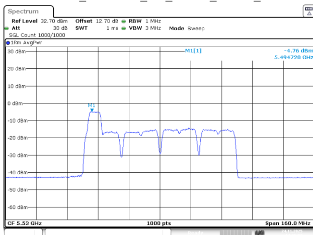
802.11be80_5530MHz_RU_26&52_MRU2_Chain 2
