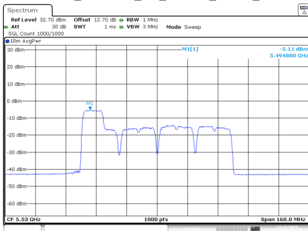
802.11be80_5530MHz_RU_26&106_MRU1_Chain 2
