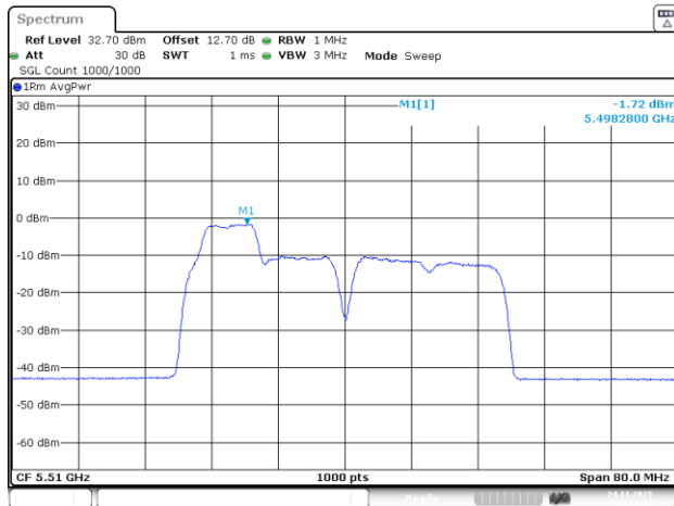
802.11be40_5510MHz_RU_26&52_MRU1_Chain 0
