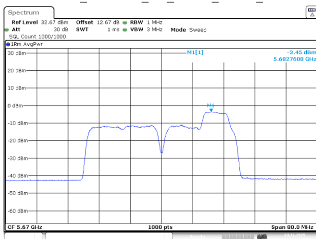
802.11be40_5670MHz_RU_26&52_MRU6_Chain 3
