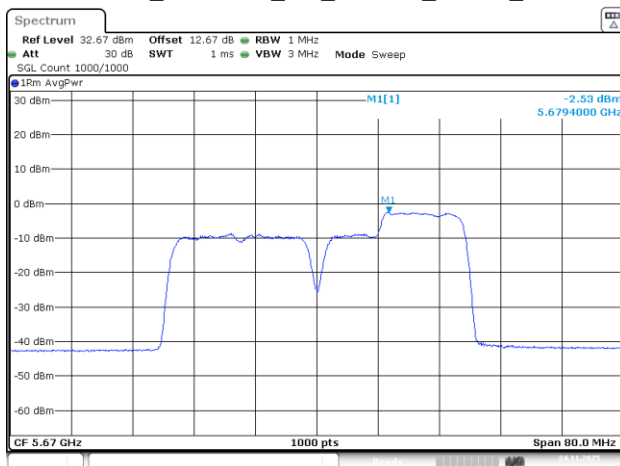
802.11be40_5670MHz_RU_26&106_MRU4_Chain 2
