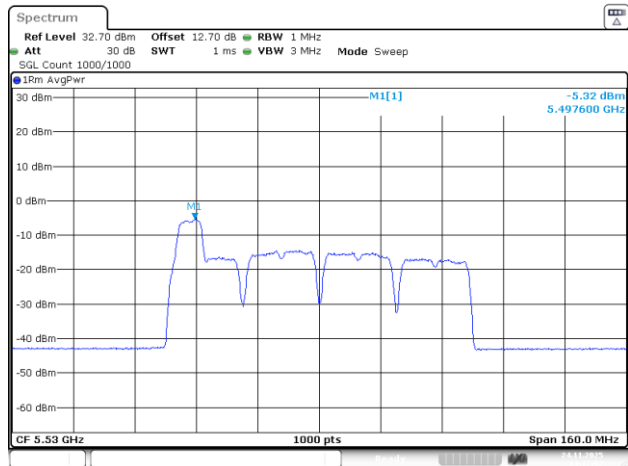
802.11be80_5530MHz_RU_26&52_MRU2_Chain 3
