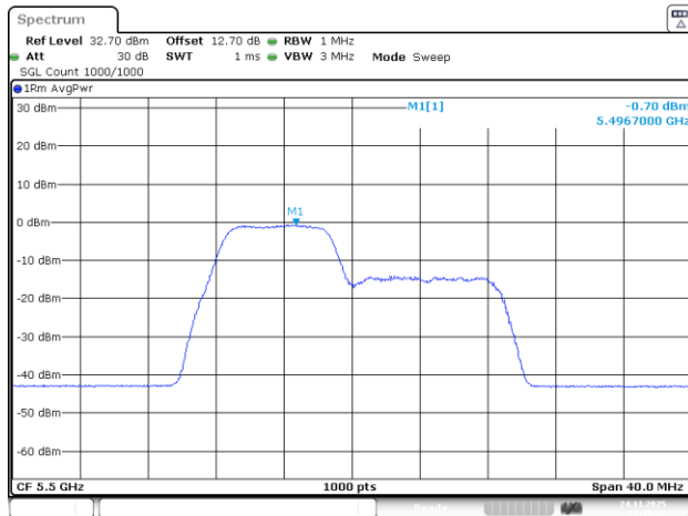
802.11be20_5500MHz_RU_26&52_MRU1_Chain 2
