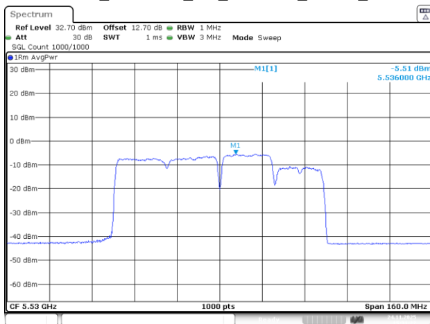
802.11be80_5530MHz_RU_242&484_MRU4_Chain 2
