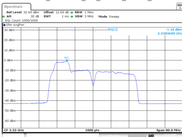
802.11be40_5550MHz_RU_26&52_MRU1_Chain 3
