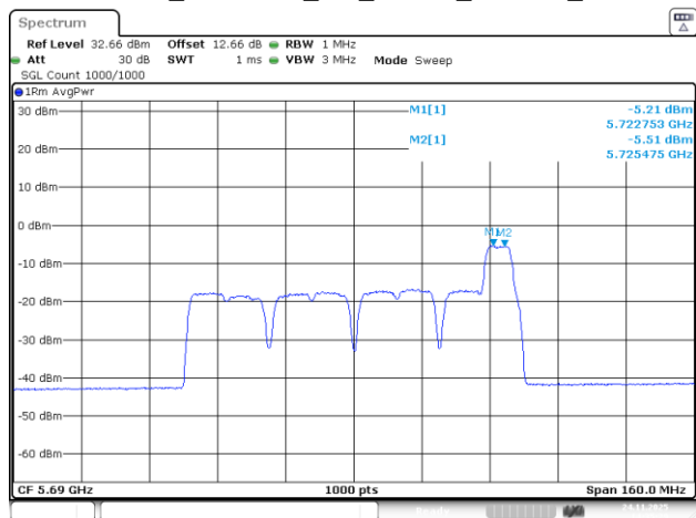
802.11be80_5690MHz_RU_26&52_MRU11_Chain 3
