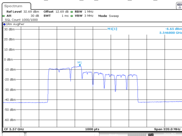
802.11be160_5570MHz_RU_242&484_MRU8_Chain 2
