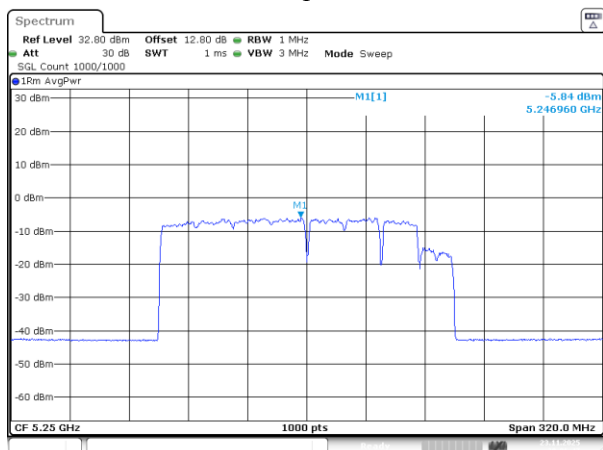
802.11be160_5250MHz_RU_242&484&996_MRU8_Chain 1
