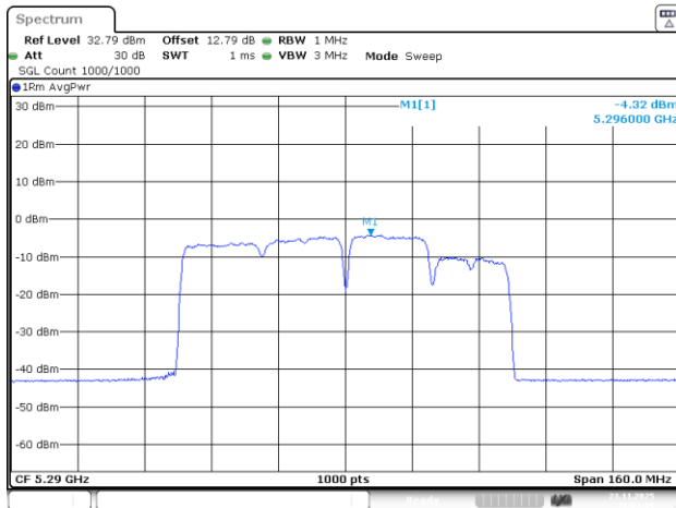
802.11be80_5290MHz_RU_242&484_MRU4_Chain 0
