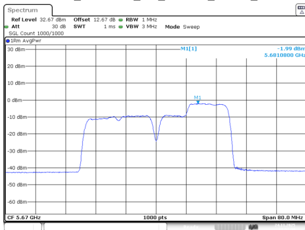
802.11be40_5670MHz_RU_26&106_MRU4_Chain 0
