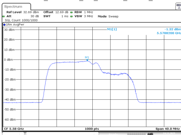
802.11be20_5580MHz_RU_26&106_MRU1_Chain 0
