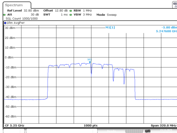
802.11be160_5250MHz_RU_484&996_MRU4_Chain 0
