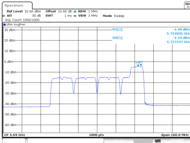
802.11be80_5690MHz_RU_26&106_MRU8_Chain 2
