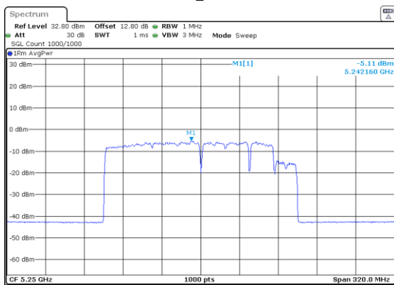
802.11be160_5250MHz_RU_242&484&996_MRU8_Chain 2
