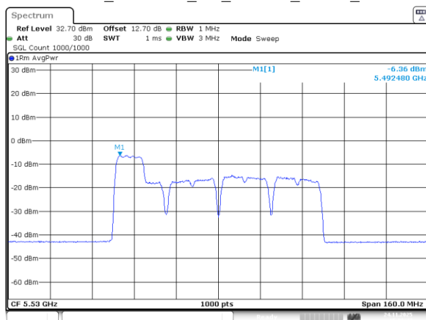
802.11be80_5530MHz_RU_26&106_MRU1_Chain 1
