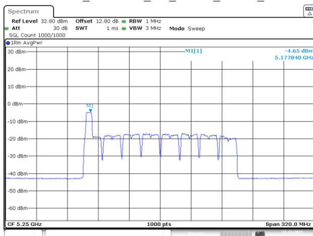
802.11be160_5250MHz_RU_26&52_MRU2_Chain 2
