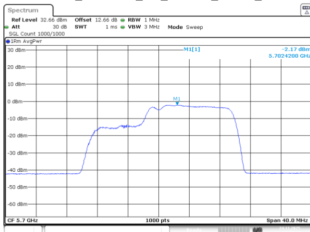
802.11be20_5700MHz_RU_26&106_MRU2_Chain 1
