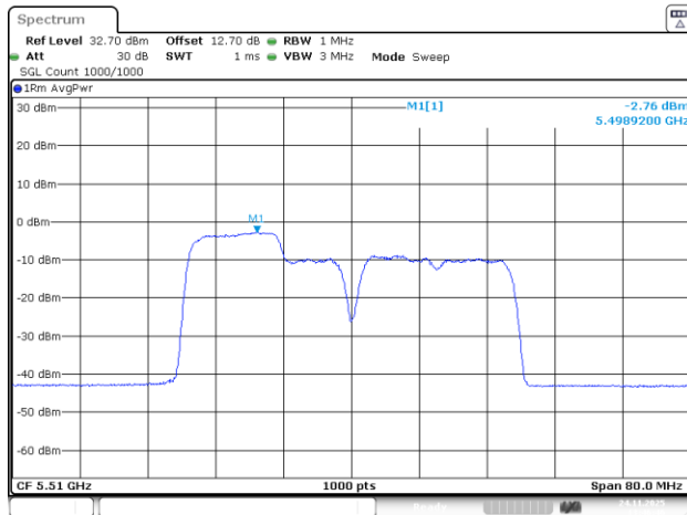
802.11be40_5510MHz_RU_26&106_MRU1_Chain 3
