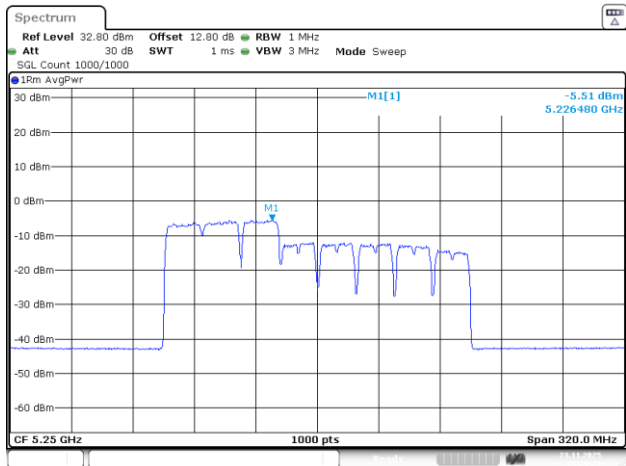
802.11be160_5250MHz_RU_242&484_MRU8_Chain 1
