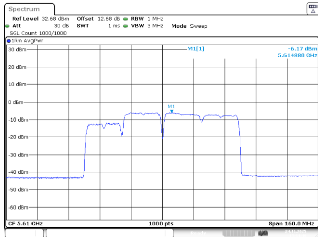
802.11be80_5610MHz_RU_242&484_MRU1_Chain 0
