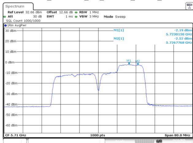
802.11be40_5710MHz_RU_26&106_MRU4_Chain 3
