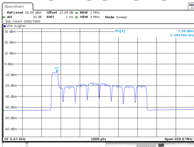
802.11be160_5570MHz_RU_26&106_MRU1_Chain 2
