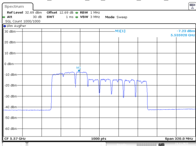
802.11be160_5570MHz_RU_242&484_MRU8_Chain 3
