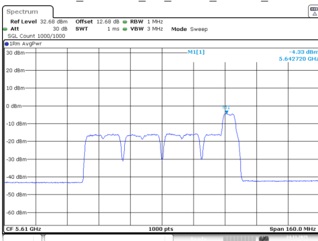
802.11be80_5610MHz_RU_26&52_MRU11_Chain 2
