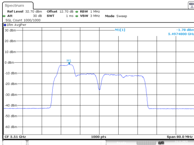
802.11be40_5510MHz_RU_26&52_MRU1_Chain 1
