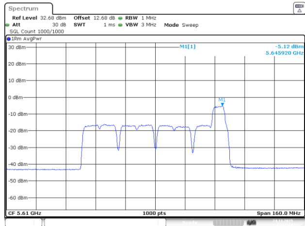
802.11be80_5610MHz_RU_26&52_MRU11_Chain 0
