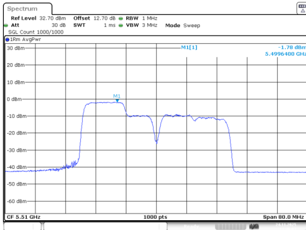
802.11be40_5510MHz_RU_26&106_MRU1_Chain 2
