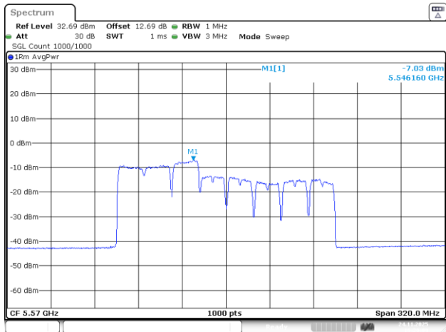
802.11be160_5570MHz_RU_242&484_MRU8_Chain 1
