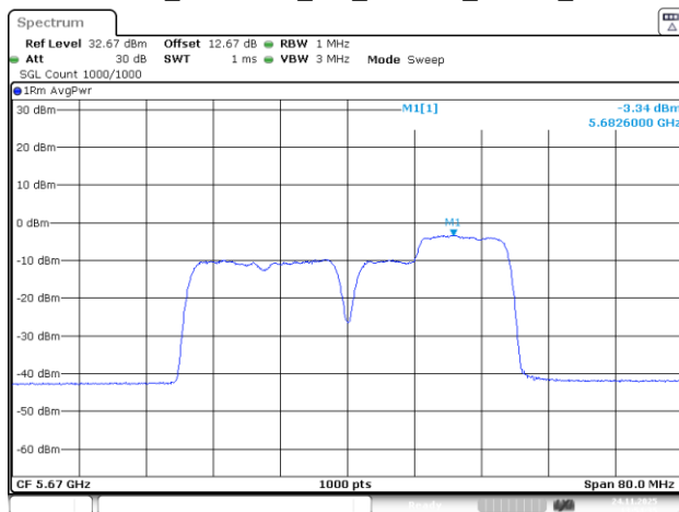
802.11be40_5670MHz_RU_26&106_MRU4_Chain 3
