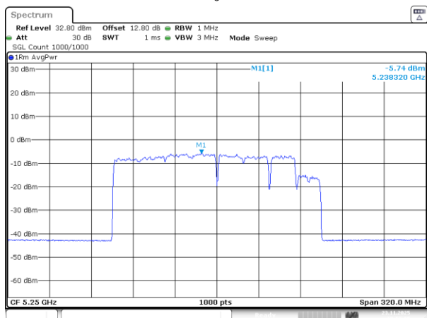
802.11be160_5250MHz_RU_242&484&996_MRU8_Chain 0
