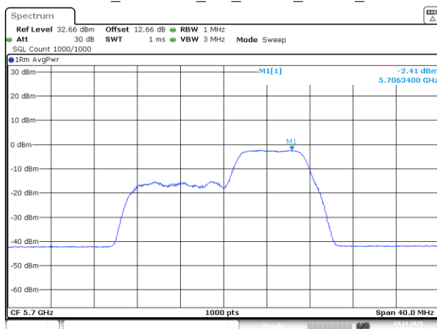
802.11be20_5700MHz_RU_26&52_MRU3_Chain 3
