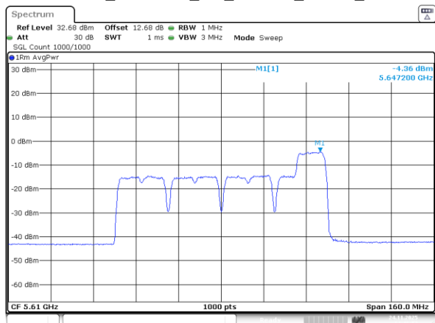
802.11be80_5610MHz_RU_26&106_MRU8_Chain 2
