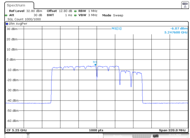
802.11be160_5250MHz_RU_484&996_MRU4_Chain 1
