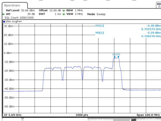
802.11be80_5690MHz_RU_26&52_MRU11_Chain 0
