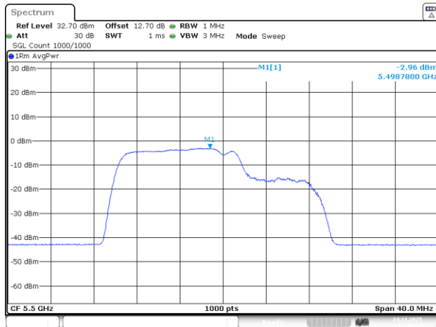
802.11be20_5500MHz_RU_26&106_MRU1_Chain 1
