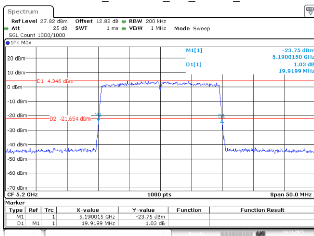
802.11be20_5200MHz_RU_242/61_Chain 0
