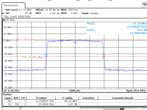
802.11be20_5280MHz_RU_242/61_Chain 3
