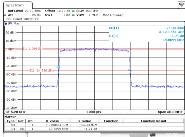
802.11be20_5280MHz_RU_242/61_Chain 0
