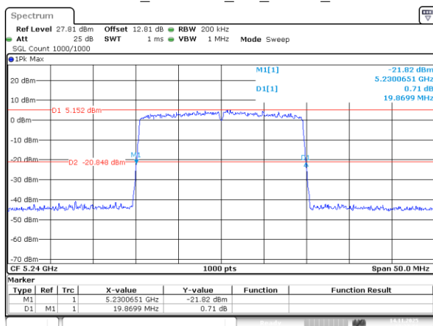
802.11be20_5240MHz_RU_242/61_Chain 0
