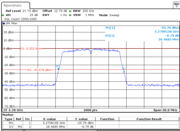
802.11a_5280MHz_Chain 2
