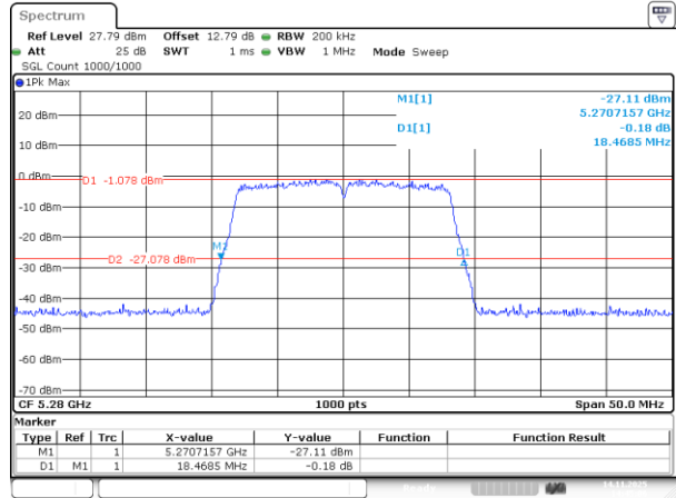
802.11a_5280MHz_Chain 0
