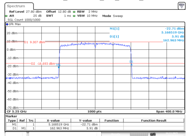
802.11be160_5250MHz_RU_2*996_Chain 2
