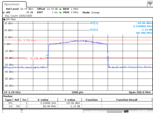
802.11be80_5290MHz_RU_996/67_Chain 1
