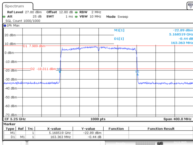
802.11be160_5250MHz_RU_2*996_Chain 0
