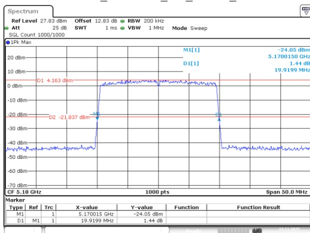
802.11be20_5180MHz_RU_242/61_Chain 0
