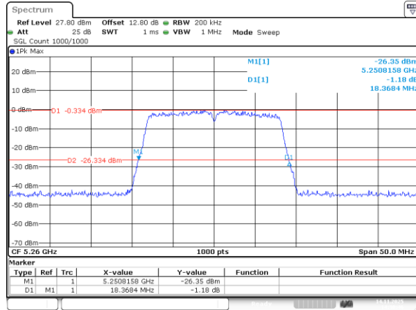
802.11a_5260MHz_Chain 0
