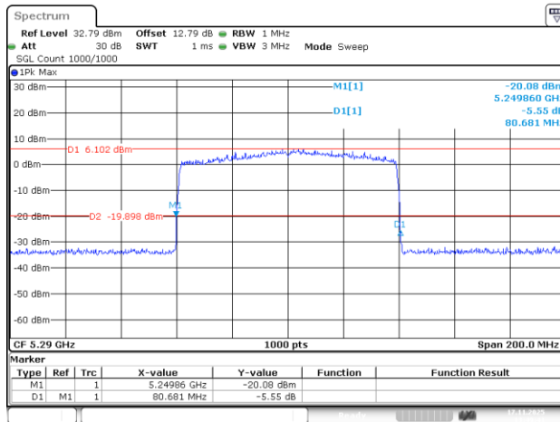
802.11be80_5290MHz_RU_996/67_Chain 0
