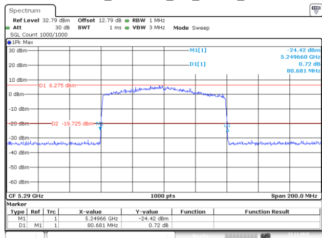
802.11be80_5290MHz_RU_996/67_Chain 3
