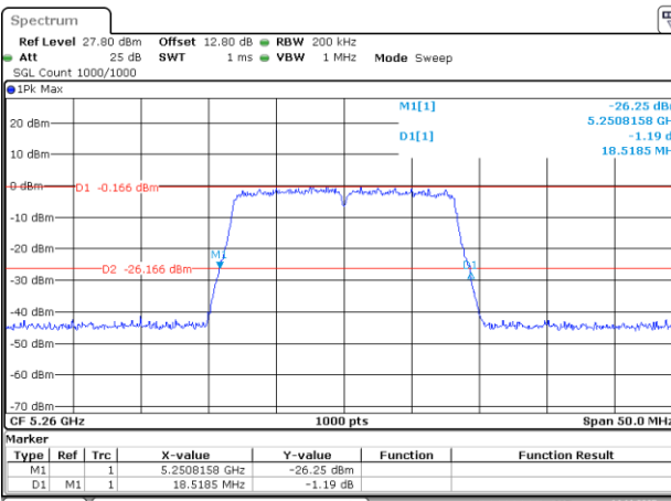
802.11a_5260MHz_Chain 2
