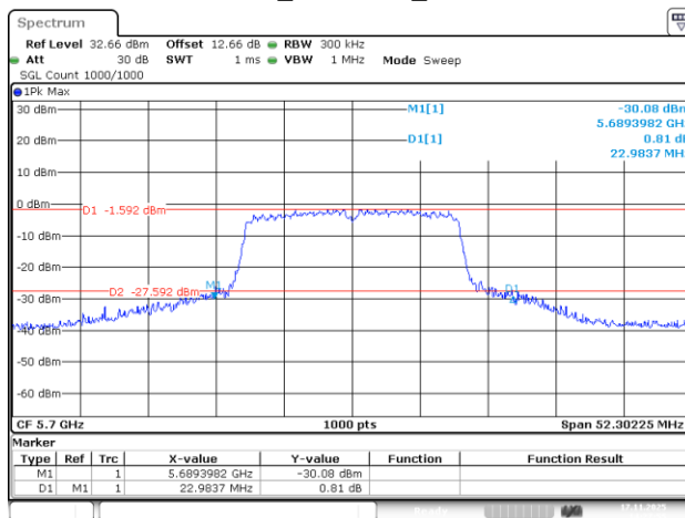
802.11a_5700MHz_Chain 3
