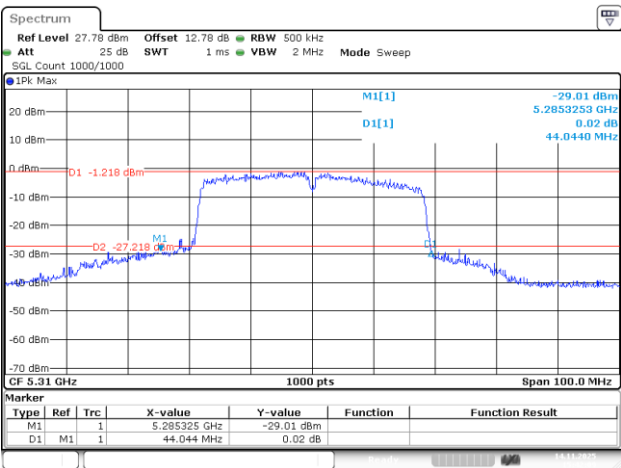
802.11ac40_5310MHz_Chain 3
