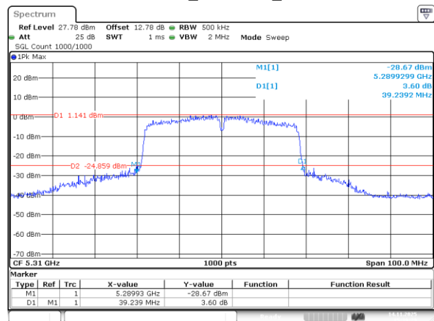
802.11ac40_5310MHz_Chain 1
