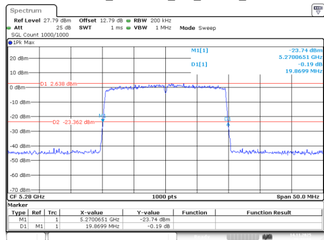
802.11be20_5280MHz_RU_242/61_Chain 2
