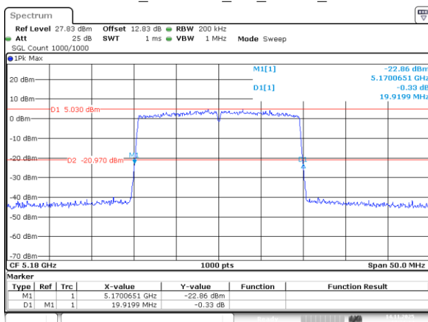
802.11be20_5180MHz_RU_242/61_Chain 1
