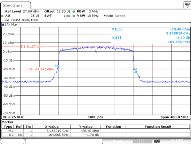
802.11ac160_5250MHz_Chain 1
