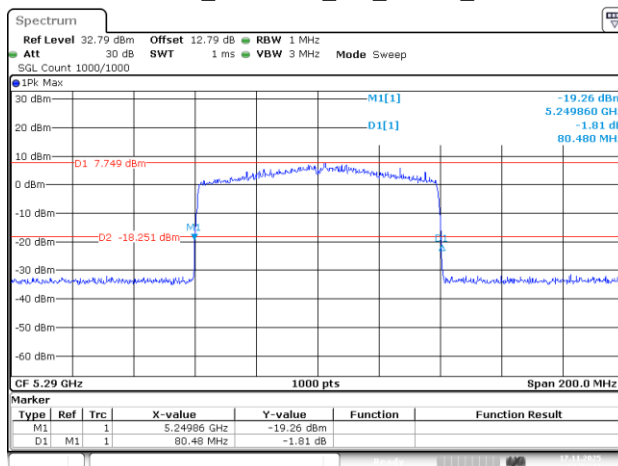
802.11be80_5290MHz_RU_996/67_Chain 2
