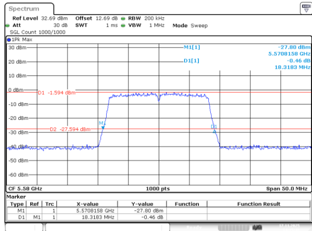
802.11a_5580MHz_Chain 3
