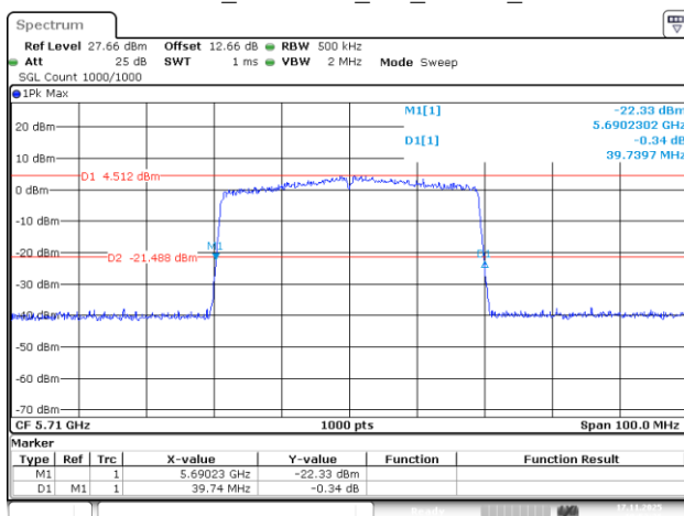
802.11be40_5710MHz_RU_484/65_Chain 2
