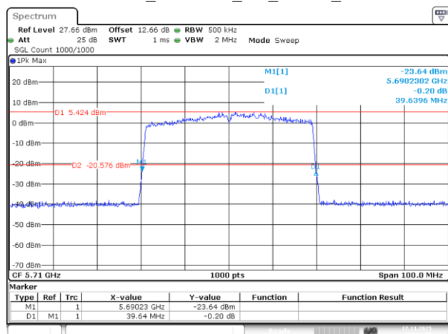
802.11be40_5710MHz_RU_484/65_Chain 1
