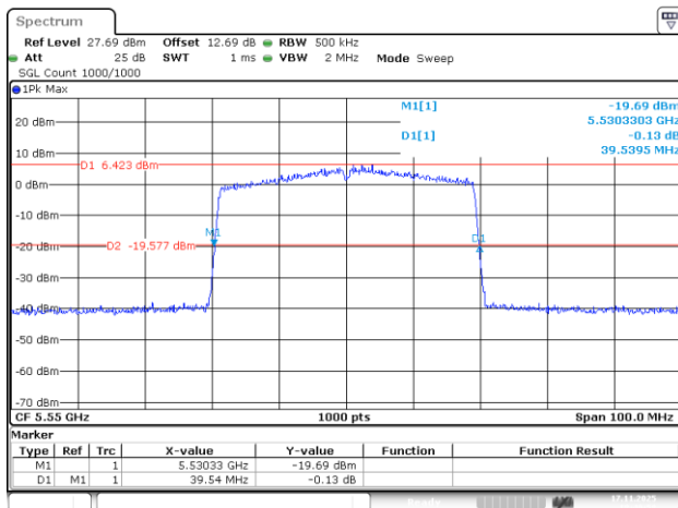
802.11be40_5550MHz_RU_484/65_Chain 2
