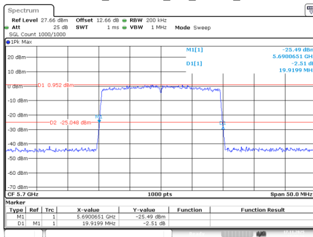
802.11be20_5700MHz_RU_242/61_Chain 0
