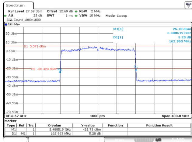
802.11be160_5570MHz_RU_2*996_Chain 1
