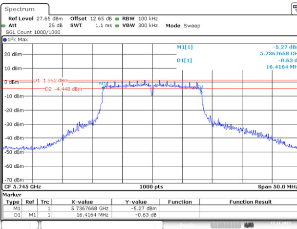
802.11a_5745MHz_Chain 2
