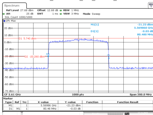
802.11be80_5610MHz_RU_996/67_Chain 1
