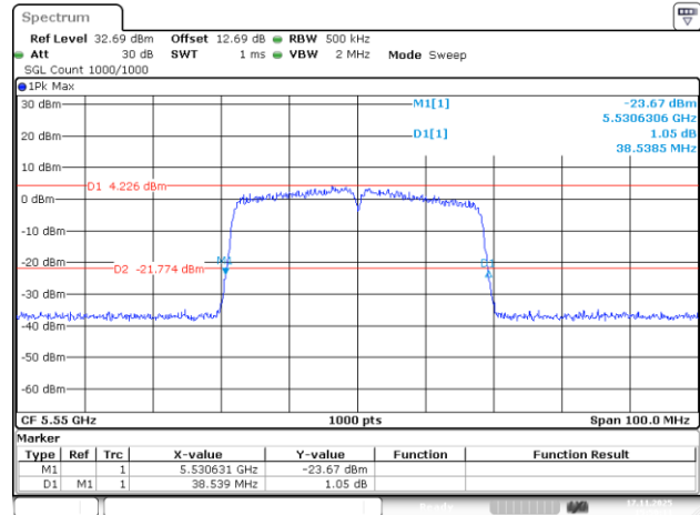
802.11ac40_5550MHz_Chain 3
