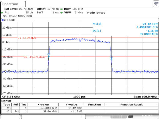
802.11be40_5510MHz_RU_484/65_Chain 0
