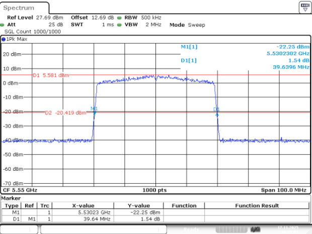
802.11be40_5550MHz_RU_484/65_Chain 0
