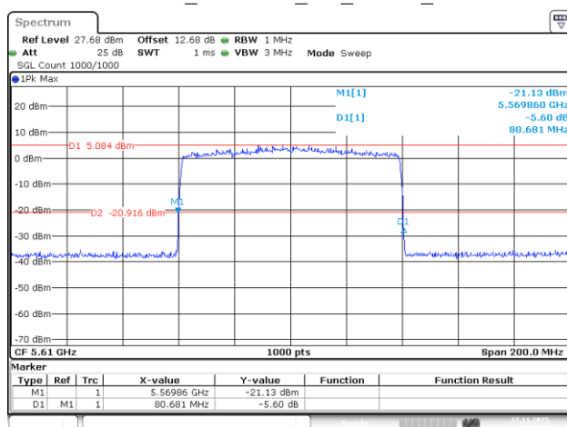
802.11be80_5610MHz_RU_996/67_Chain 2
