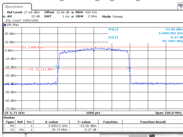
802.11be40_5710MHz_RU_484/65_Chain 3
