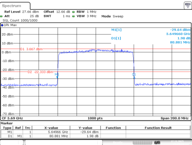
802.11be80_5690MHz_RU_996/67_Chain 3
