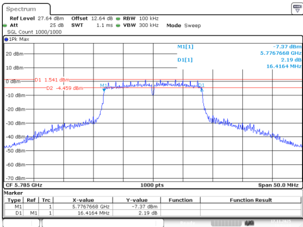
802.11a_5785MHz_Chain 2
