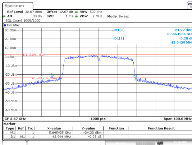
802.11ac40_5670MHz_Chain 3
