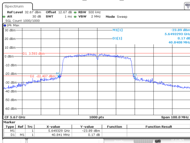
802.11ac40_5670MHz_Chain 2
