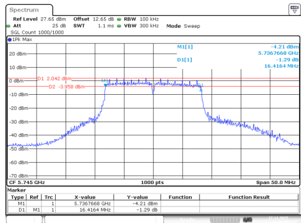
802.11a_5745MHz_Chain 1
