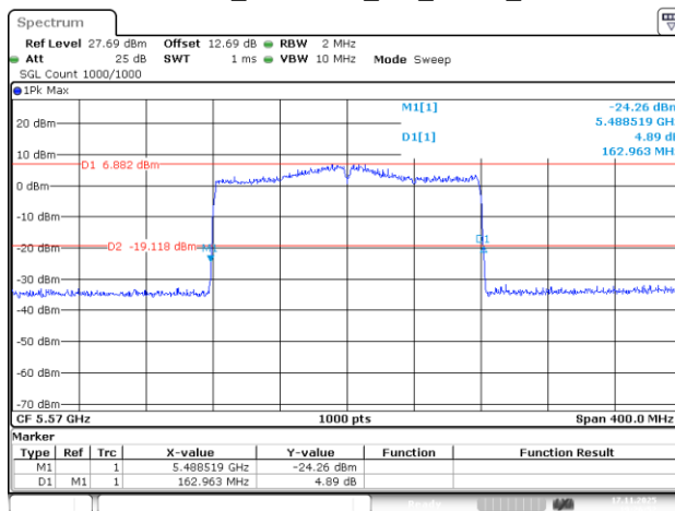
802.11be160_5570MHz_RU_2*996_Chain 2
