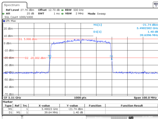
802.11be40_5510MHz_RU_484/65_Chain 3
