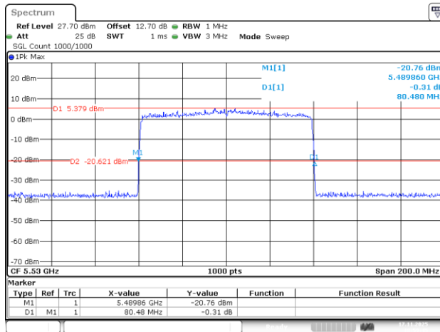
802.11be80_5530MHz_RU_996/67_Chain 0
