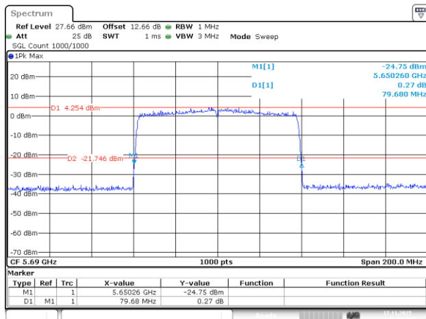
802.11ac80_5690MHz_Chain 2
