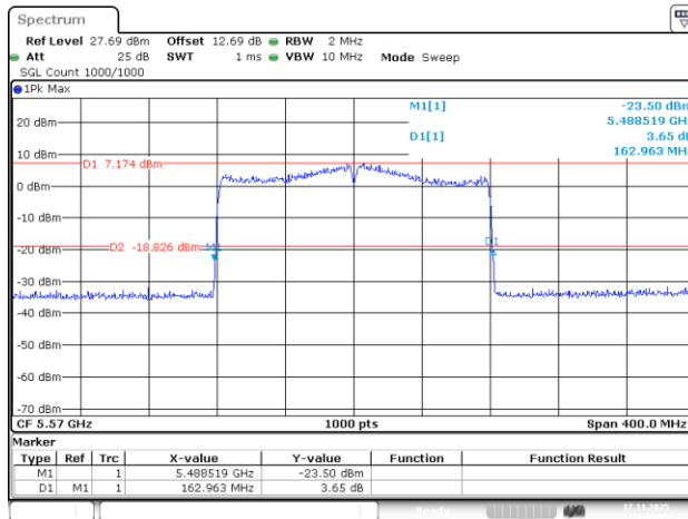
802.11be160_5570MHz_RU_2*996_Chain 0
