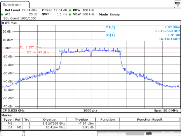
802.11a_5825MHz_Chain 2
