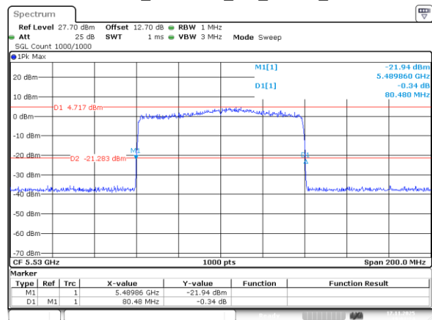
802.11be80_5530MHz_RU_996/67_Chain 1
