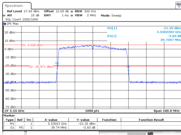
802.11be40_5550MHz_RU_484/65_Chain 3
