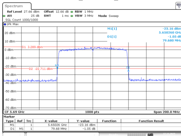
802.11ac80_5690MHz_Chain 3
