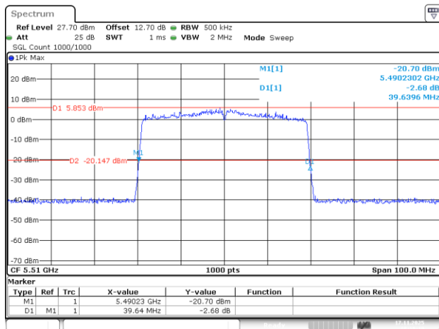
802.11be40_5510MHz_RU_484/65_Chain 2
