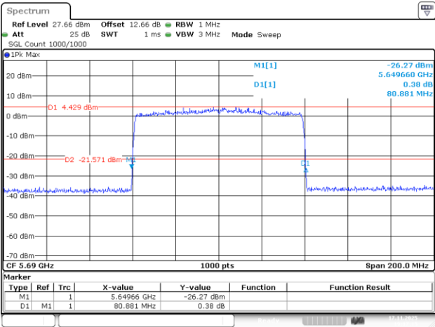
802.11be80_5690MHz_RU_996/67_Chain 2
