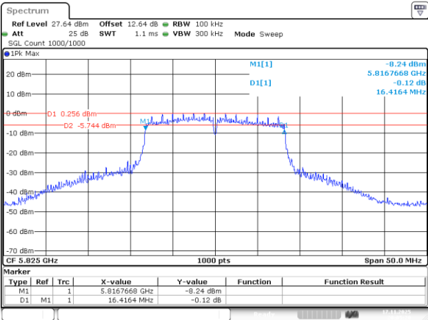
802.11a_5825MHz_Chain 3
