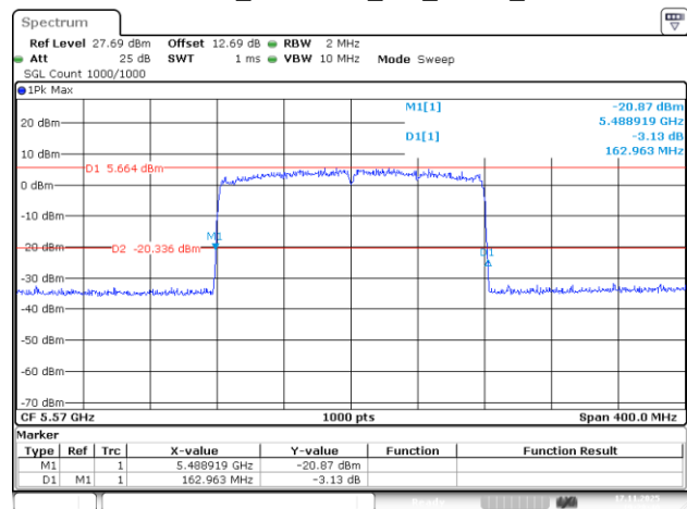
802.11be160_5570MHz_RU_2*996_Chain 3
