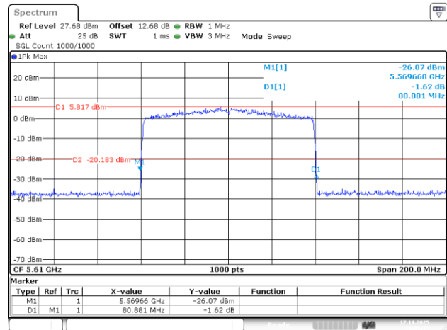
802.11be80_5610MHz_RU_996/67_Chain 0
