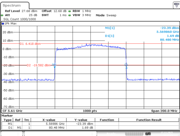
802.11be80_5610MHz_RU_996/67_Chain 3
