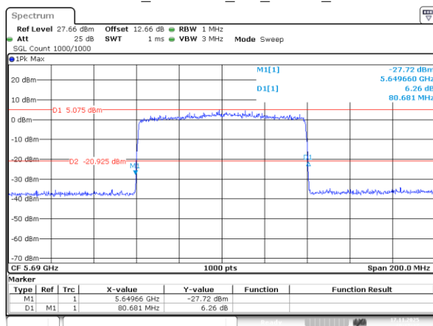
802.11be80_5690MHz_RU_996/67_Chain 1
