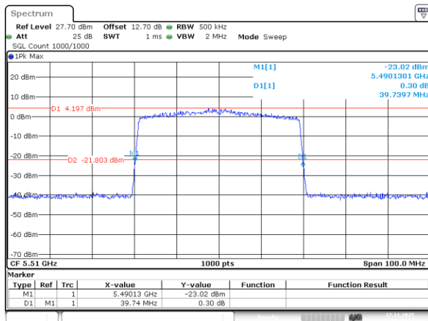
802.11be40_5510MHz_RU_484/65_Chain 1
