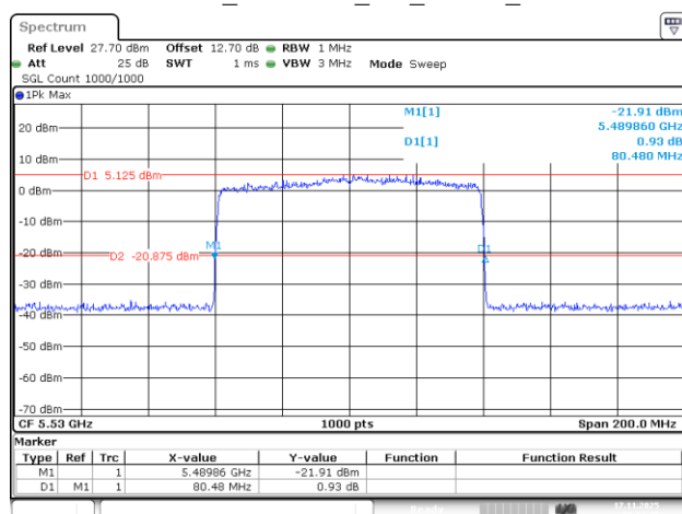
802.11be80_5530MHz_RU_996/67_Chain 2
