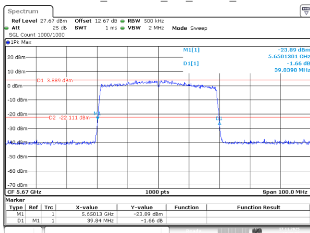
802.11be40_5670MHz_RU_484/65_Chain 3
