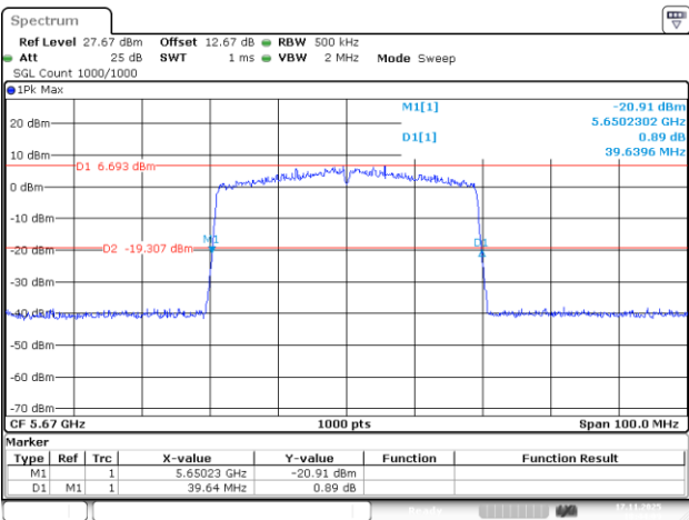
802.11be40_5670MHz_RU_484/65_Chain 0
