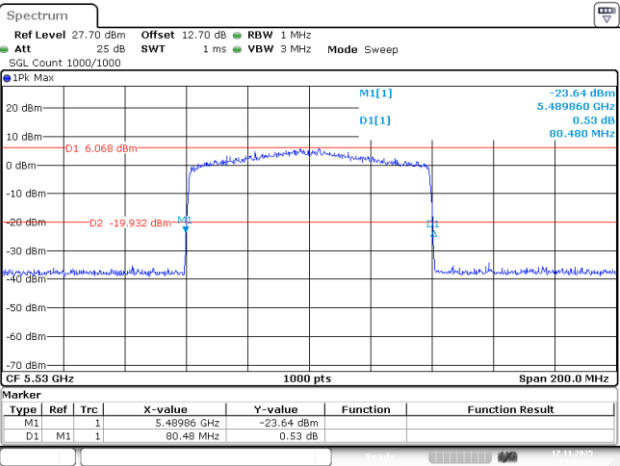
802.11be80_5530MHz_RU_996/67_Chain 3
