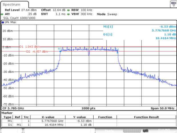
802.11a_5785MHz_Chain 3
