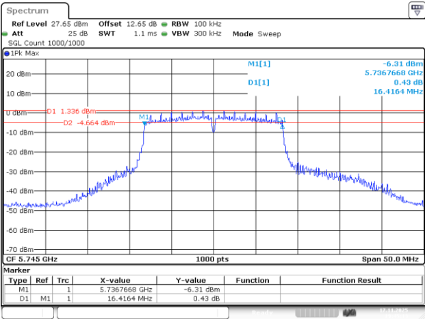
802.11a_5745MHz_Chain 3
