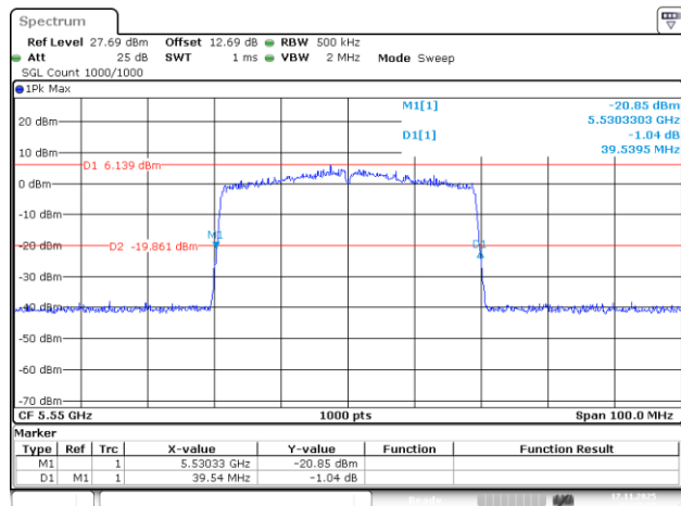
802.11be40_5550MHz_RU_484/65_Chain 1
