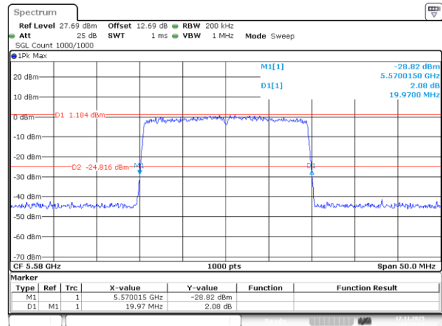
802.11be20_5580MHz_RU_242/61_Chain 0
