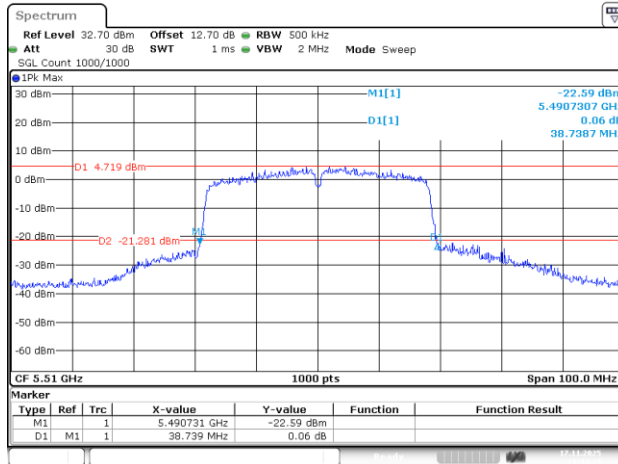
802.11ac40_5510MHz_Chain 3
