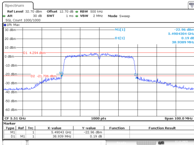
802.11ac40_5510MHz_Chain 2
