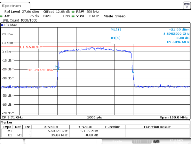
802.11be40_5710MHz_RU_484/65_Chain 0
