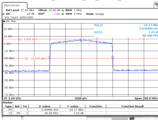
802.11be80_5690MHz_RU_996/67_Chain 0
