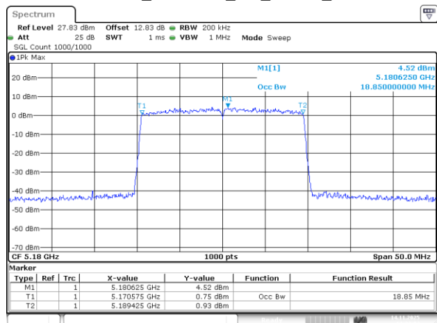
802.11be20_5180MHz_RU_242/61_Chain 1
