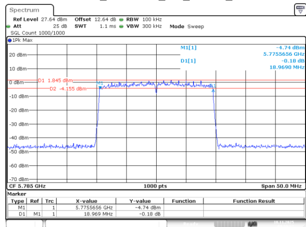
802.11be20_5785MHz_RU_242/61_Chain 2
