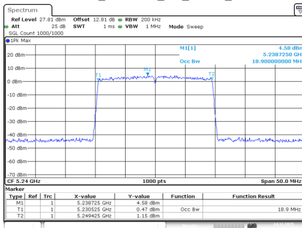
802.11be20_5240MHz_RU_242/61_Chain 0
