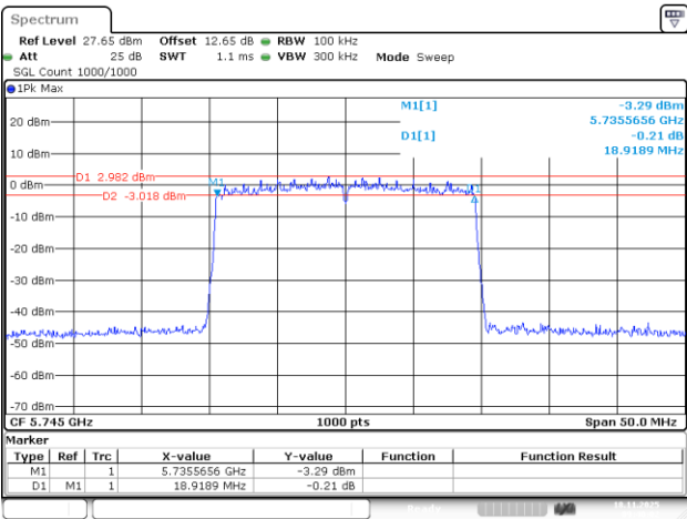
802.11be20_5745MHz_RU_242/61_Chain 0
