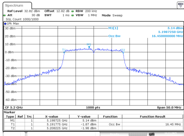
802.11a_5200MHz_Chain 2
