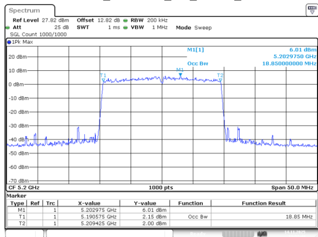
802.11be20_5200MHz_RU_242/61_Chain 2
