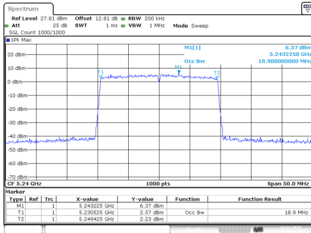
802.11be20_5240MHz_RU_242/61_Chain 2
