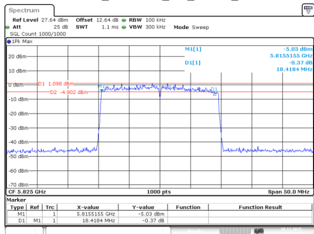
802.11be20_5825MHz_RU_242/61_Chain 3
