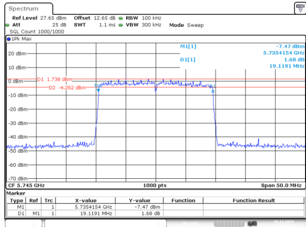
802.11be20_5745MHz_RU_242/61_Chain 3
