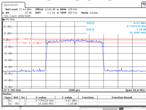
802.11be20_5785MHz_RU_242/61_Chain 3
