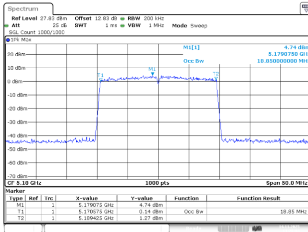
802.11be20_5180MHz_RU_242/61_Chain 0
