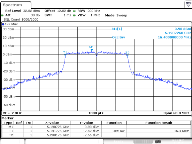
802.11a_5200MHz_Chain 3
