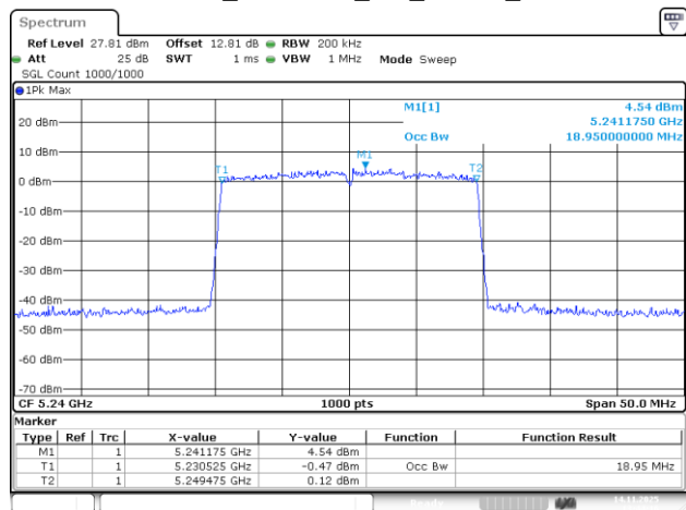
802.11be20_5240MHz_RU_242/61_Chain 3
