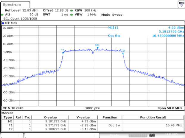
802.11a_5180MHz_Chain 3
