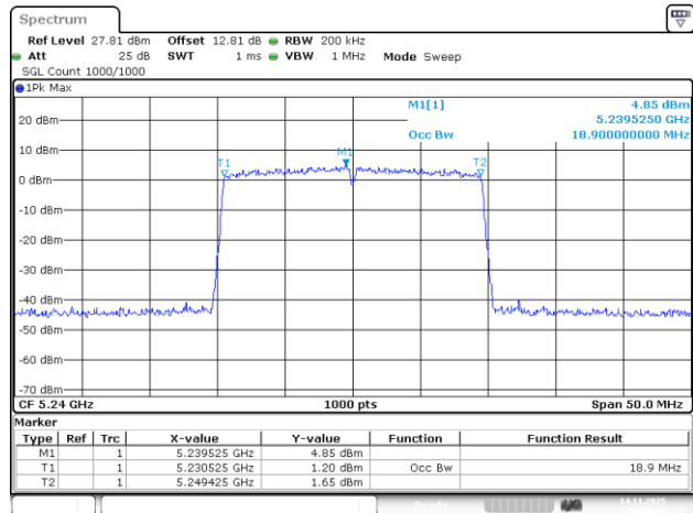
802.11be20_5240MHz_RU_242/61_Chain 1
