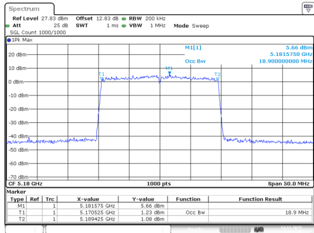
802.11be20_5180MHz_RU_242/61_Chain 3
