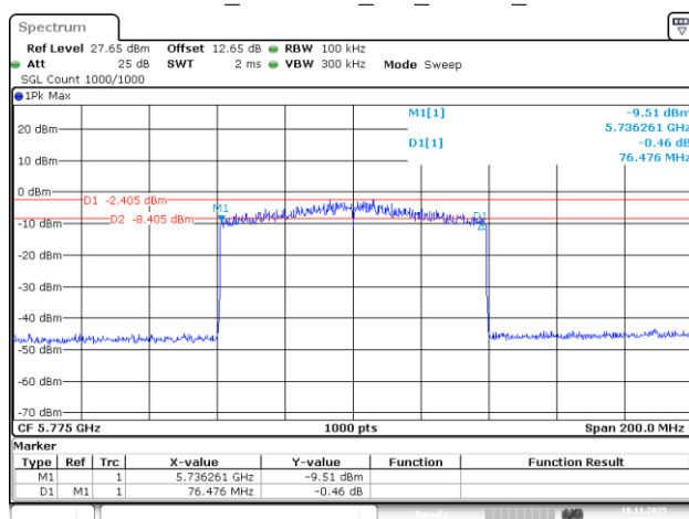
802.11be80_5775MHz_RU_996/67_Chain 3
