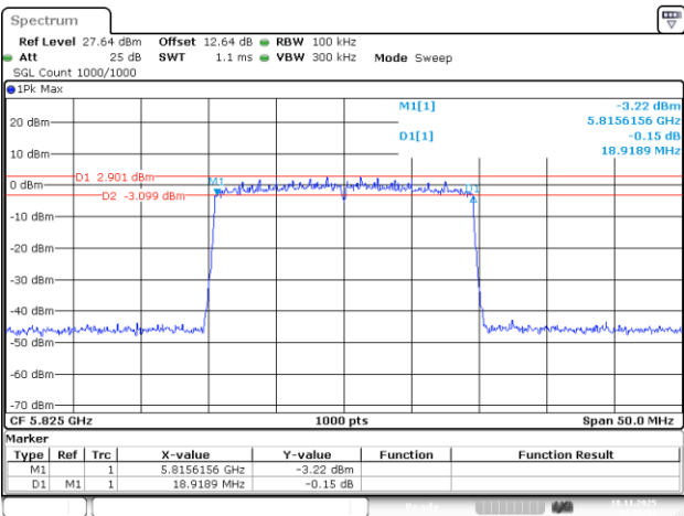
802.11be20_5825MHz_RU_242/61_Chain 0
