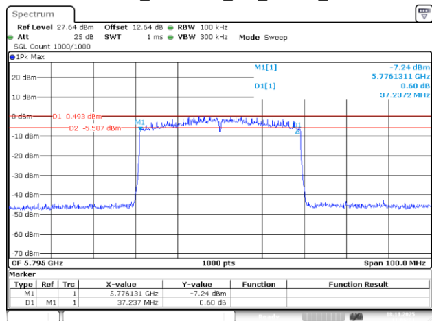
802.11be40_5795MHz_RU_484/65_Chain 1
