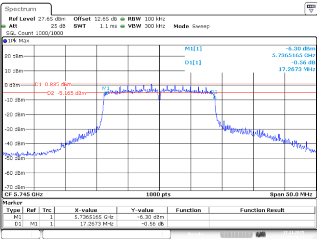
802.11ac20_5745MHz_Chain 3
