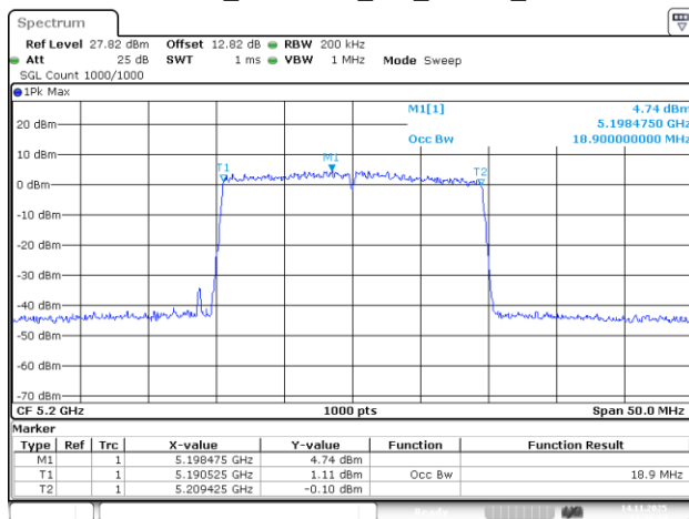
802.11be20_5200MHz_RU_242/61_Chain 3
