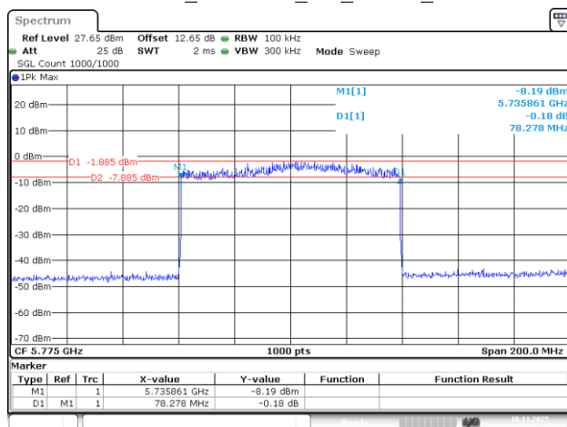
802.11be80_5775MHz_RU_996/67_Chain 1
