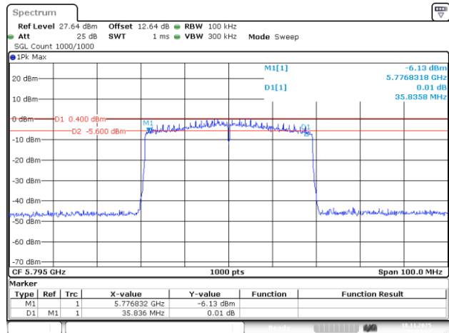
802.11be40_5795MHz_RU_484/65_Chain 0
