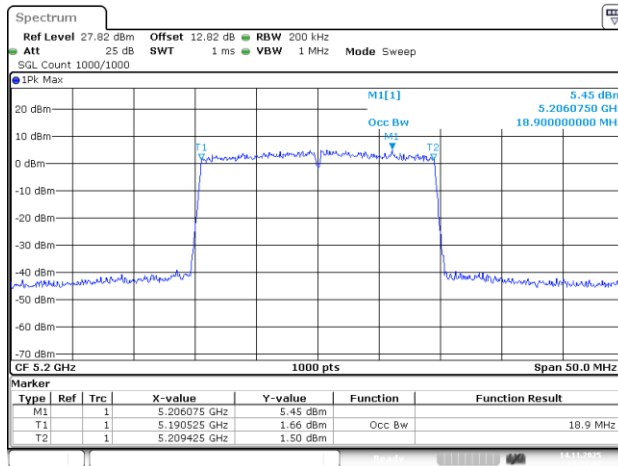
802.11be20_5200MHz_RU_242/61_Chain 1
