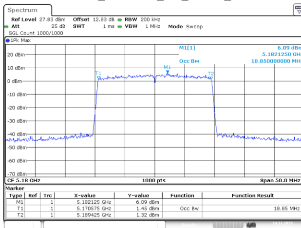
802.11be20_5180MHz_RU_242/61_Chain 2
