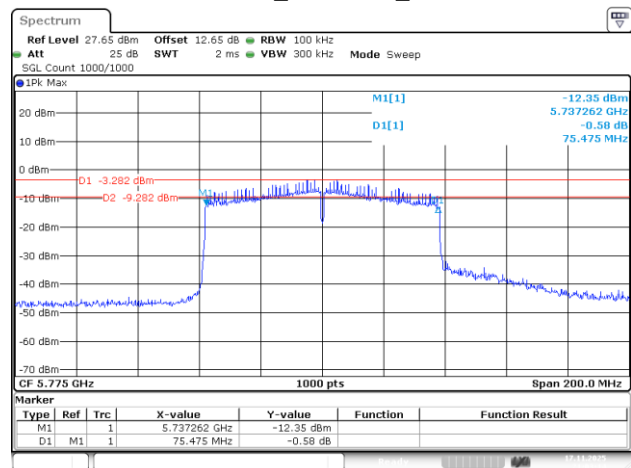
802.11ac80_5775MHz_Chain 3
