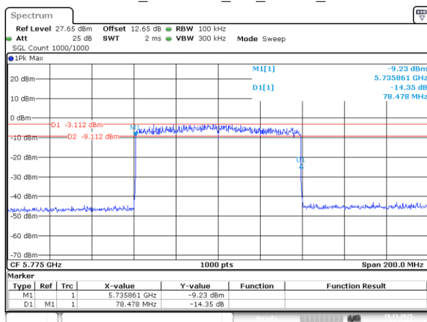
802.11be80_5775MHz_RU_996/67_Chain 0
