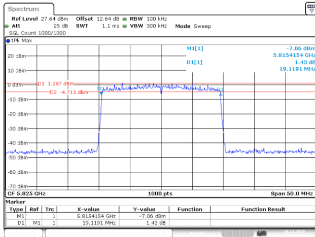
802.11be20_5825MHz_RU_242/61_Chain 2
