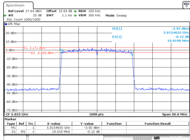
802.11be20_5825MHz_RU_242/61_Chain 1
