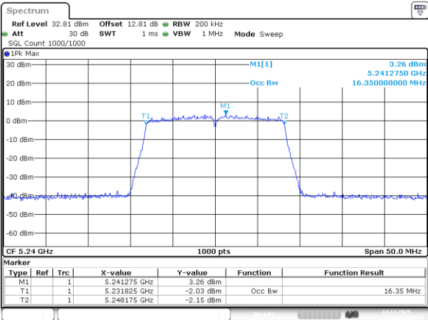
802.11a_5240MHz_Chain 3
