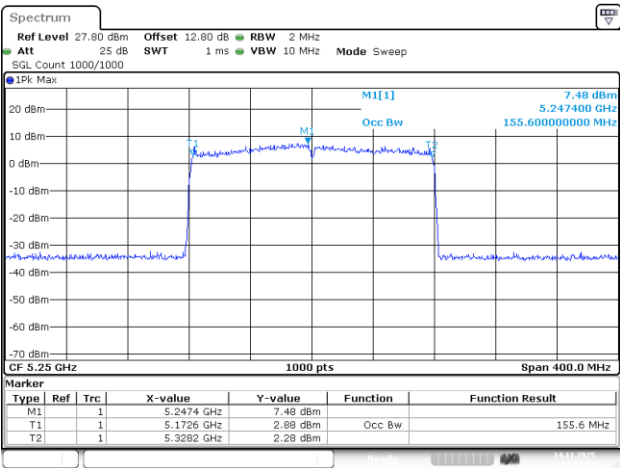
802.11be160_5250MHz_RU_2*996_Chain 0
