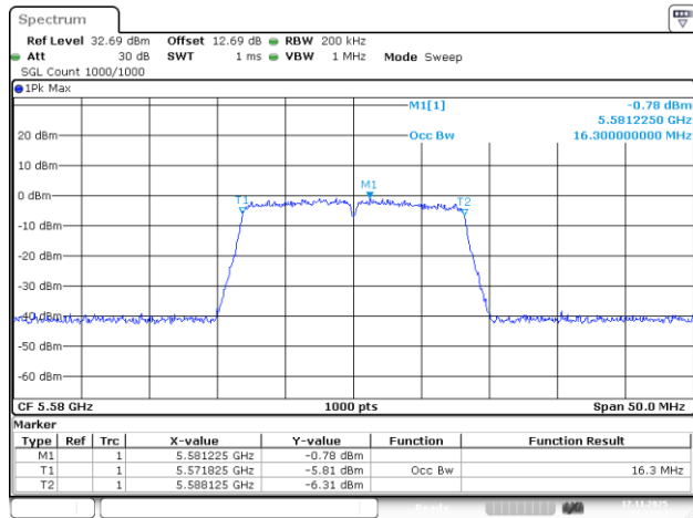
802.11a_5580MHz_Chain 1
