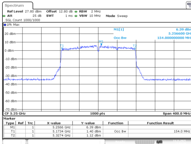
802.11ac160_5250MHz_Chain 0
