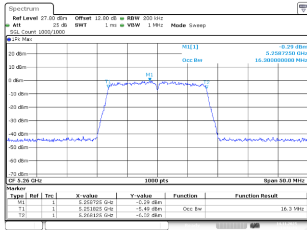
802.11a_5260MHz_Chain 0
