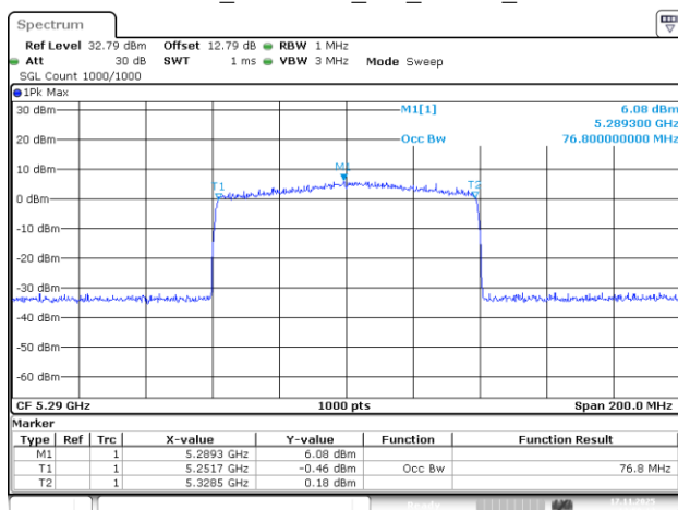
802.11be80_5290MHz_RU_996/67_Chain 0
