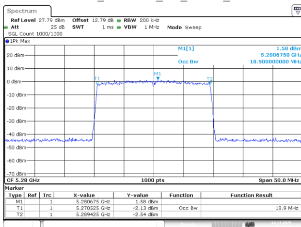
802.11be20_5280MHz_RU_242/61_Chain 0
