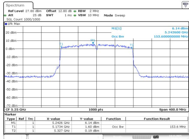
802.11ac160_5250MHz_Chain 1
