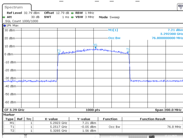
802.11be80_5290MHz_RU_996/67_Chain 2
