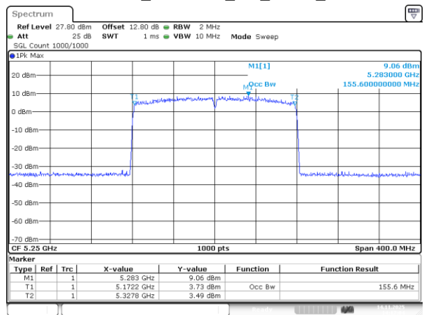
802.11be160_5250MHz_RU_2*996_Chain 2
