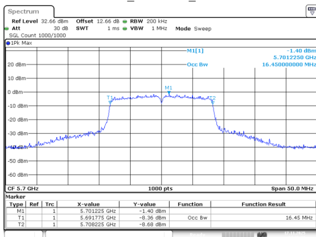
802.11a_5700MHz_Chain 2
