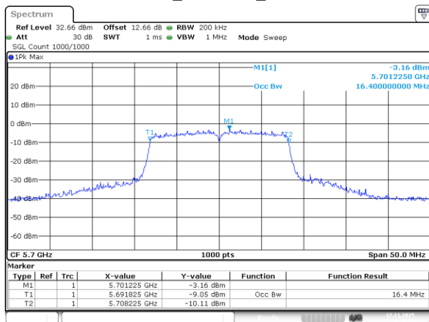
802.11a_5700MHz_Chain 3
