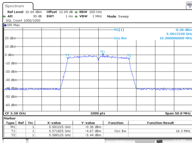
802.11a_5580MHz_Chain 2
