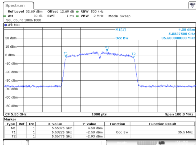
802.11ac40_5550MHz_Chain 1
