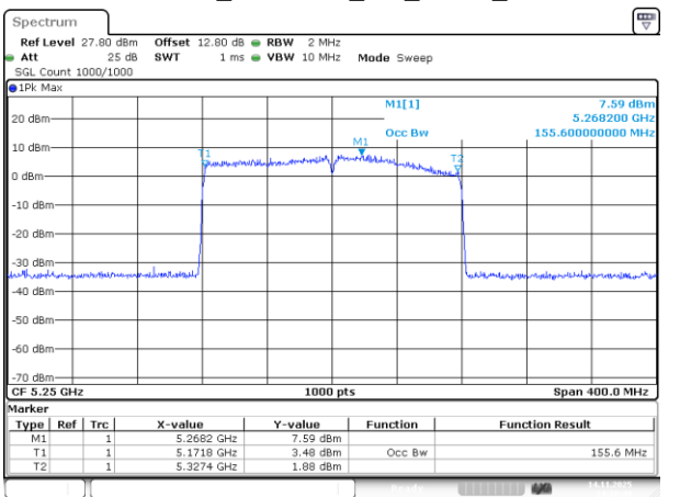
802.11be160_5250MHz_RU_2*996_Chain 3
