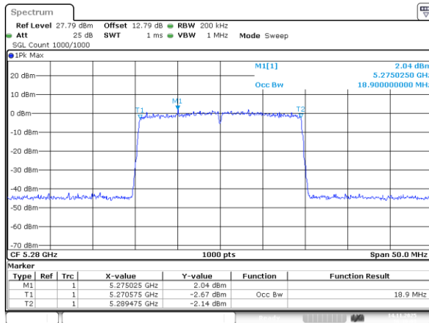
802.11be20_5280MHz_RU_242/61_Chain 1
