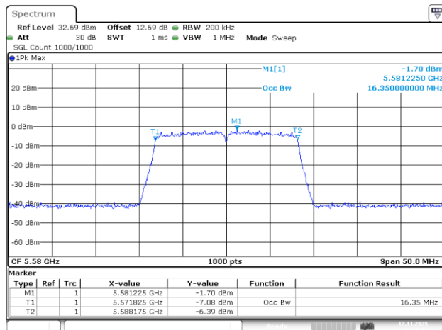
802.11a_5580MHz_Chain 3
