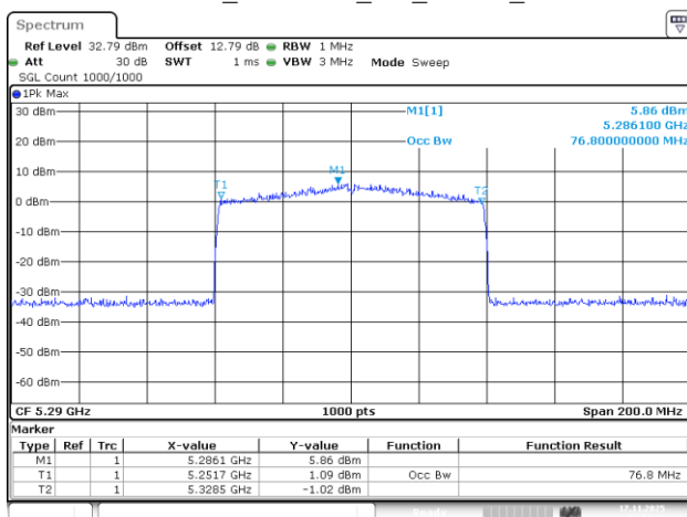
802.11be80_5290MHz_RU_996/67_Chain 1
