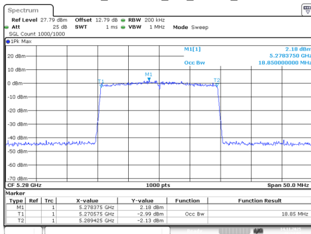
802.11be20_5280MHz_RU_242/61_Chain 3
