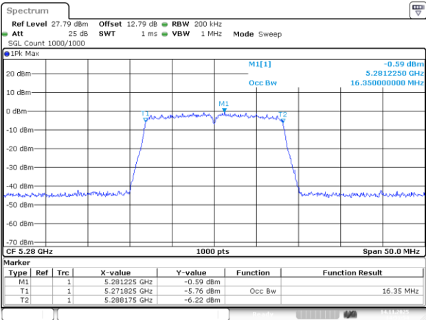
802.11a_5280MHz_Chain 3
