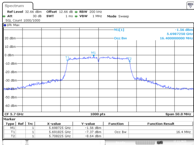
802.11a_5700MHz_Chain 1
