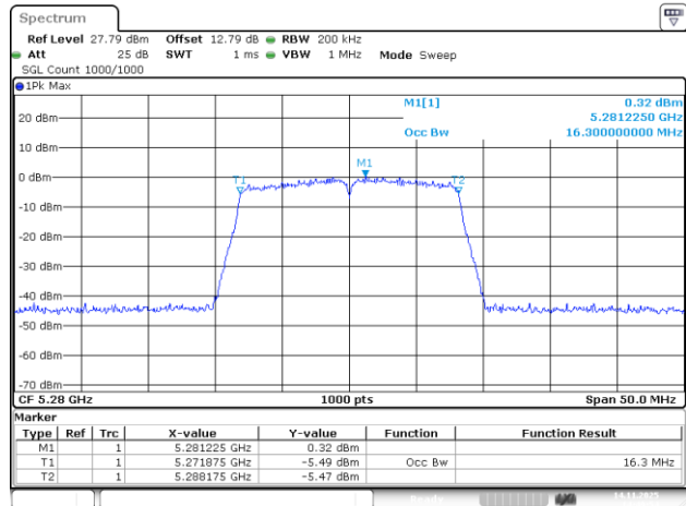
802.11a_5280MHz_Chain 2
