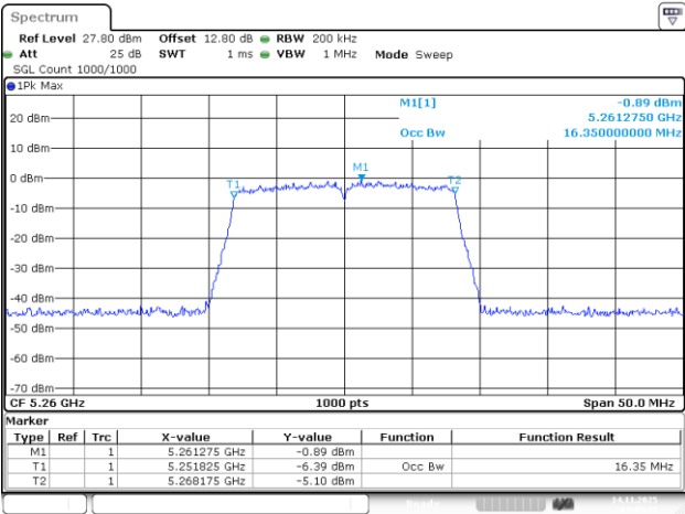
802.11a_5260MHz_Chain 3
