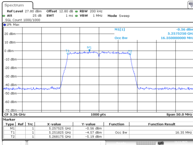
802.11a_5260MHz_Chain 2
