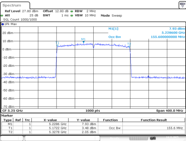
802.11be160_5250MHz_RU_2*996_Chain 1
