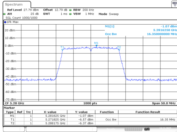
802.11a_5280MHz_Chain 1
