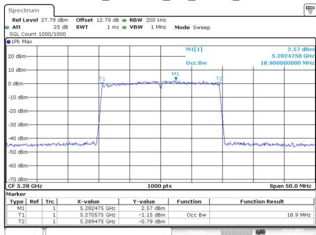
802.11be20_5280MHz_RU_242/61_Chain 2
