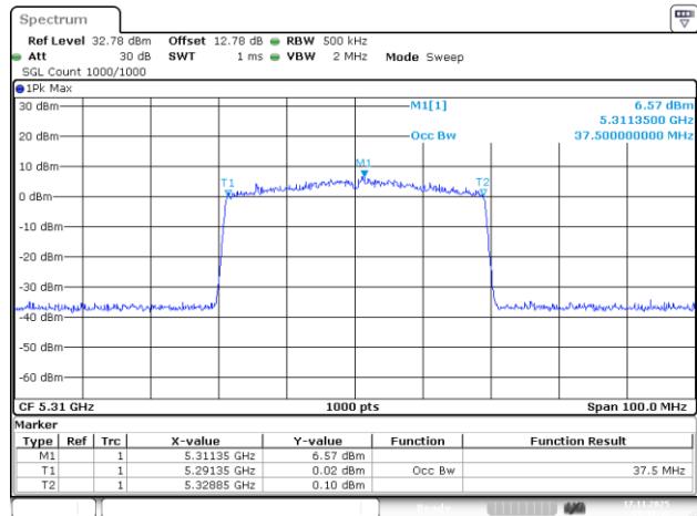
802.11be40_5310MHz_RU_484/65_Chain 0
