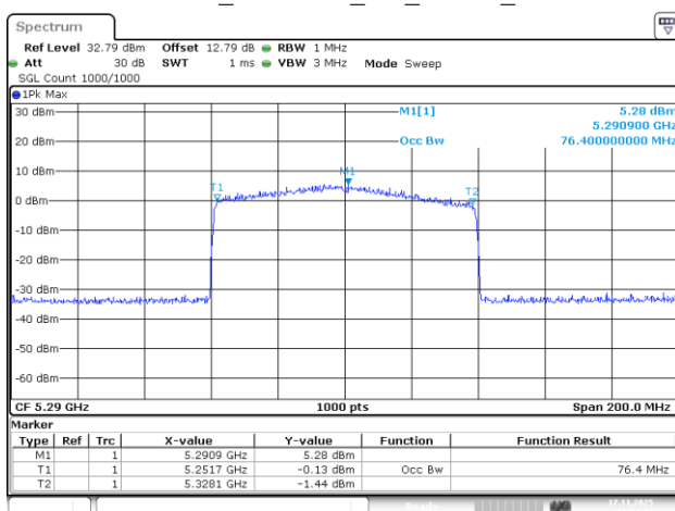
802.11be80_5290MHz_RU_996/67_Chain 3
