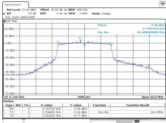
802.11a_5745MHz_Chain 3
