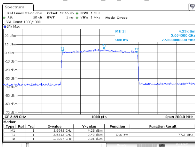
802.11be80_5690MHz_RU_996/67_Chain 2
