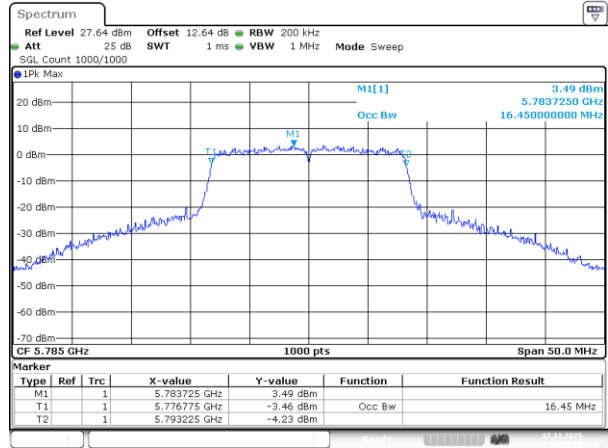
802.11a_5785MHz_Chain 0
