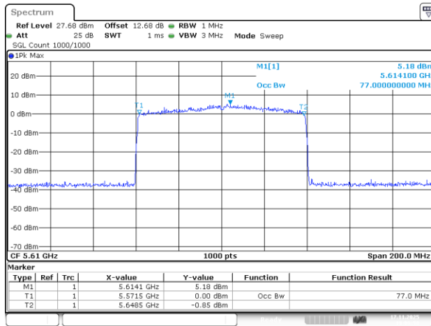
802.11be80_5610MHz_RU_996/67_Chain 1
