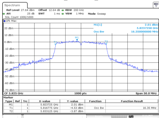
802.11a_5825MHz_Chain 3
