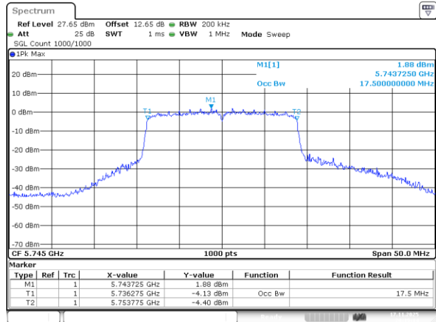
802.11ac20_5745MHz_Chain 3
