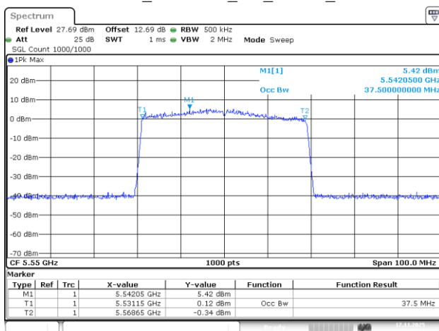
802.11be40_5550MHz_RU_484/65_Chain 3
