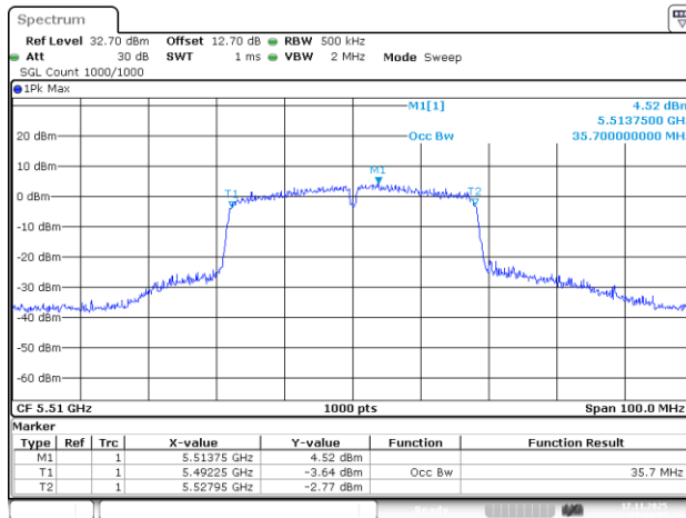
802.11ac40_5510MHz_Chain 3
