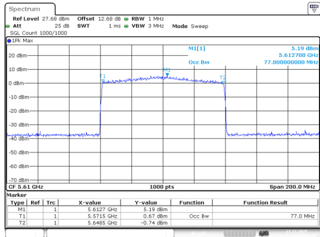
802.11be80_5610MHz_RU_996/67_Chain 0
