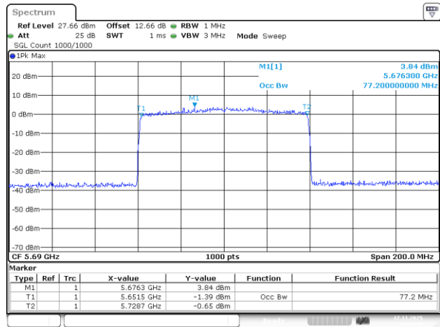
802.11be80_5690MHz_RU_996/67_Chain 1
