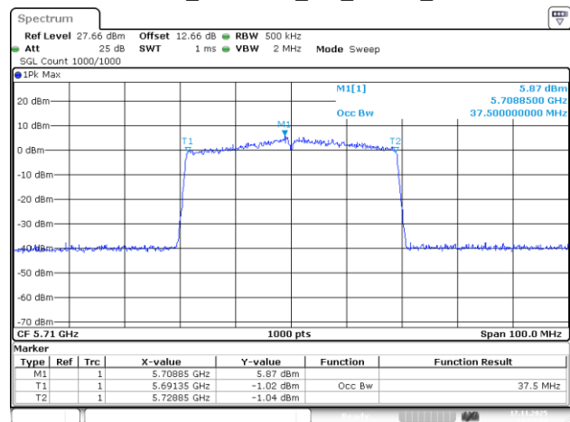
802.11be40_5710MHz_RU_484/65_Chain 1
