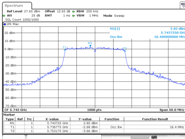
802.11a_5745MHz_Chain 2
