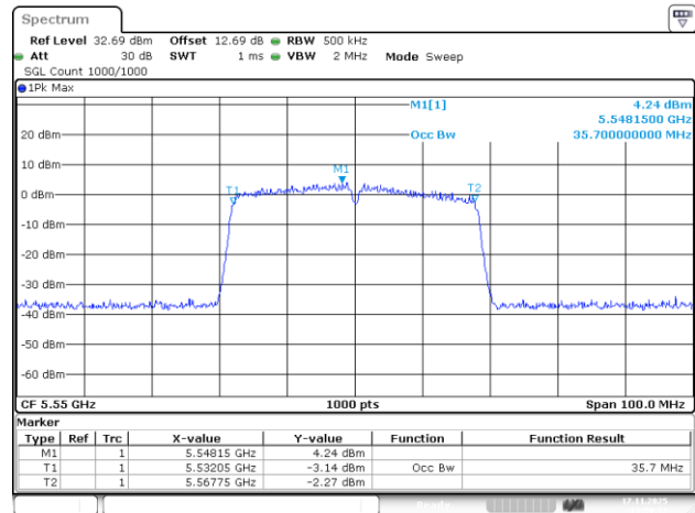
802.11ac40_5550MHz_Chain 3
