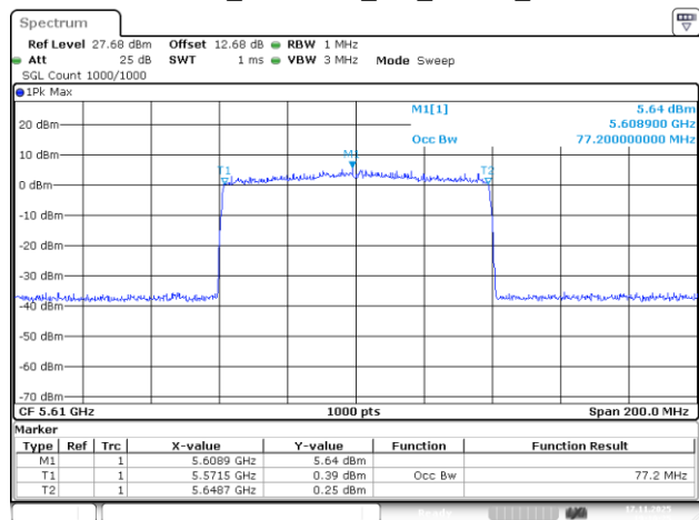
802.11be80_5610MHz_RU_996/67_Chain 2
