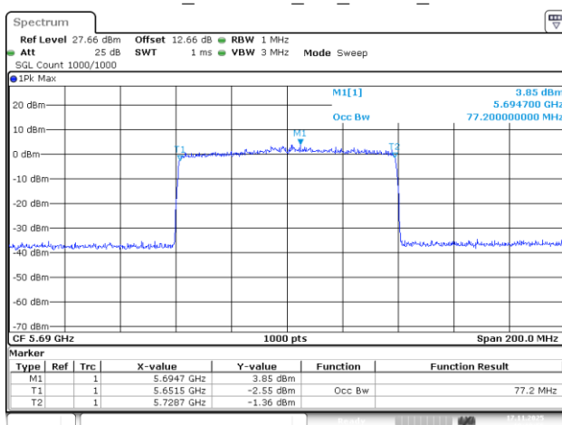
802.11be80_5690MHz_RU_996/67_Chain 3
