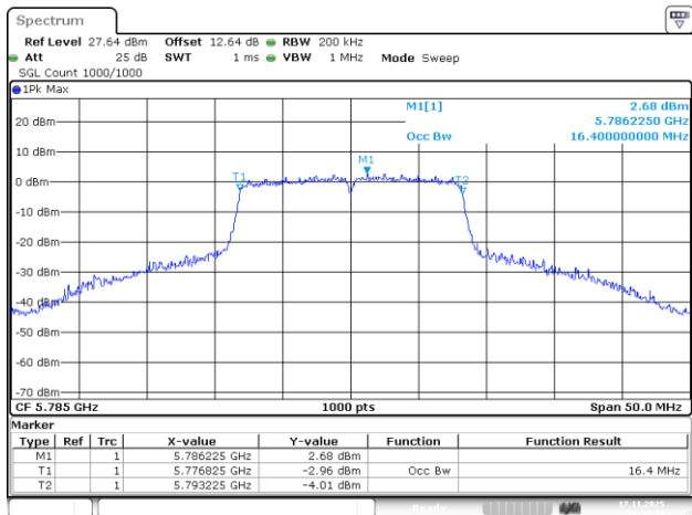
802.11a_5785MHz_Chain 2
