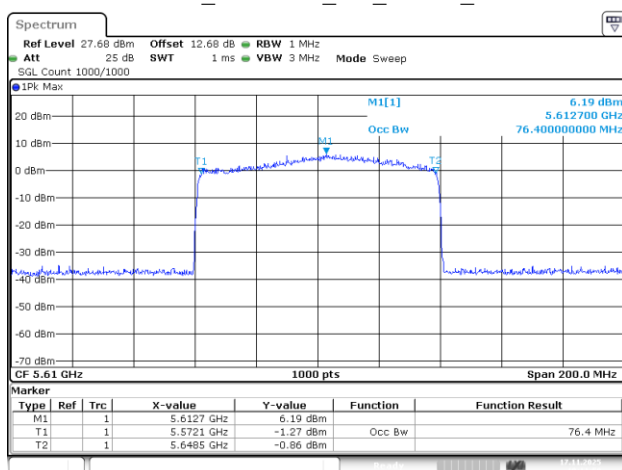
802.11be80_5610MHz_RU_996/67_Chain 3
