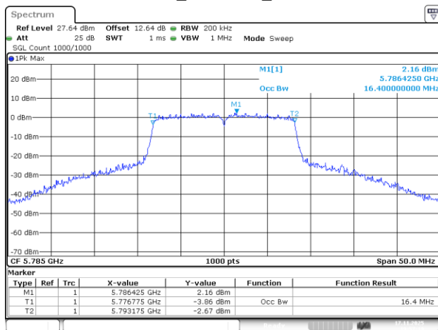
802.11a_5785MHz_Chain 3
