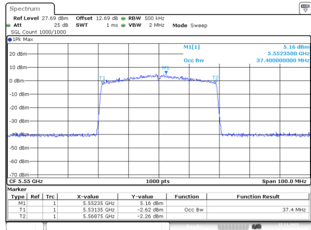
802.11be40_5550MHz_RU_484/65_Chain 1
