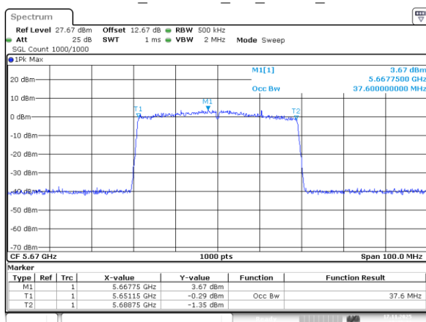
802.11be40_5670MHz_RU_484/65_Chain 3
