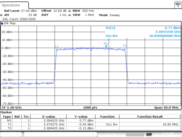
802.11be20_5580MHz_RU_242/61_Chain 0
