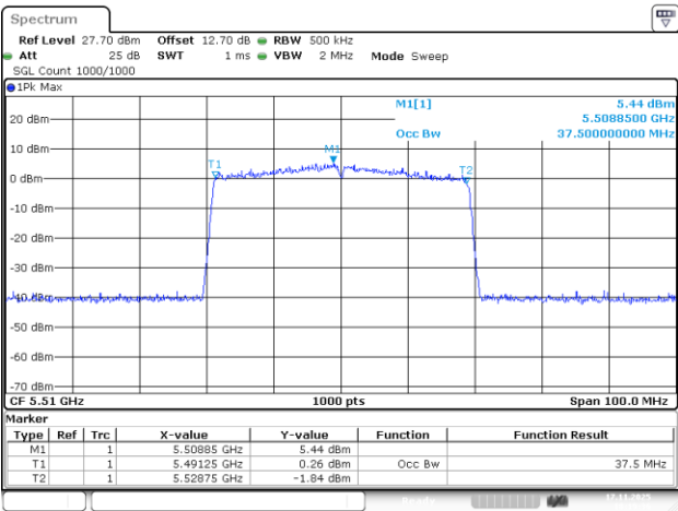
802.11be40_5510MHz_RU_484/65_Chain 2
