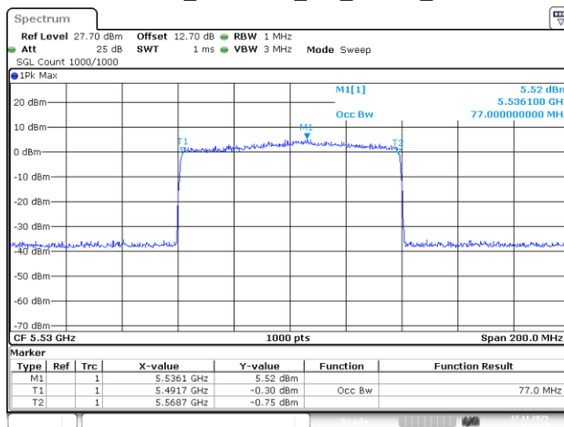
802.11be80_5530MHz_RU_996/67_Chain 2
