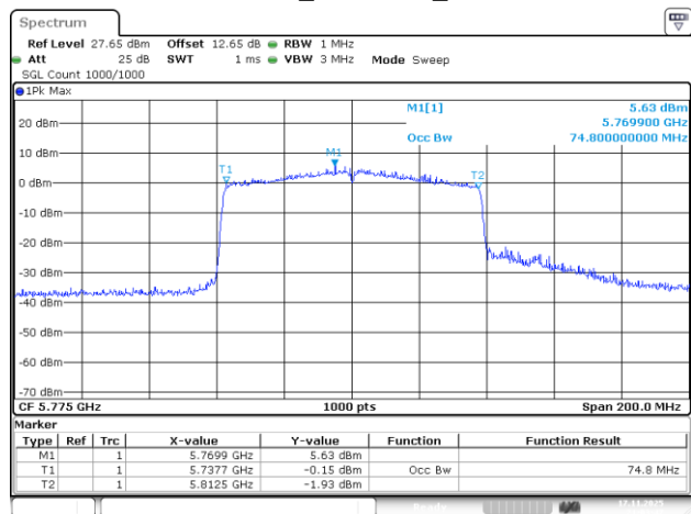
802.11ac80_5775MHz_Chain 3
