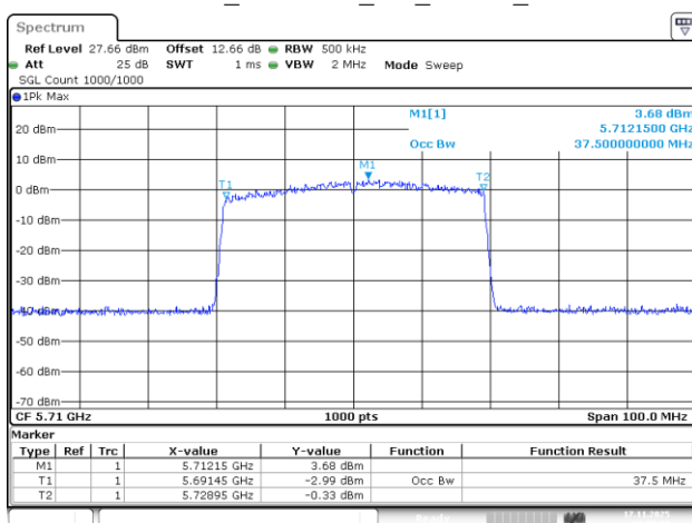
802.11be40_5710MHz_RU_484/65_Chain 3
