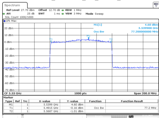
802.11be80_5530MHz_RU_996/67_Chain 1
