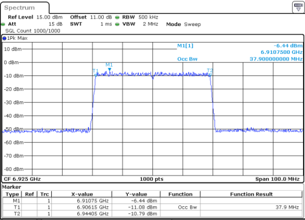
802.11be40_6925MHz_RU_484/65_Chain 0
