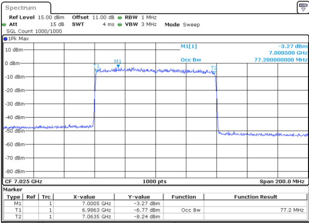
802.11be80_7025MHz_RU_996/67_Chain 1
