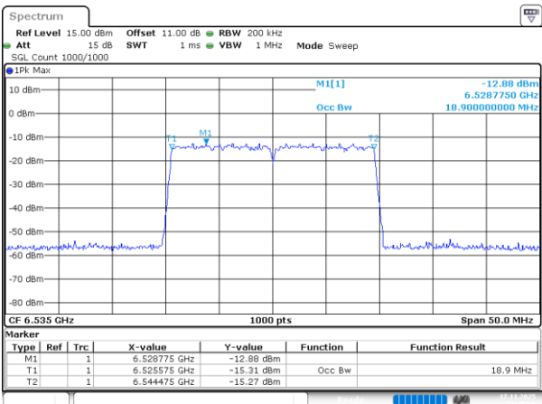
802.11be20_6535MHz_RU_242/61_Chain 0
