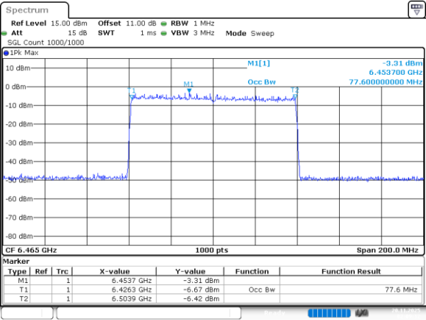
802.11be80_6465MHz_RU_996/67_Chain 0
