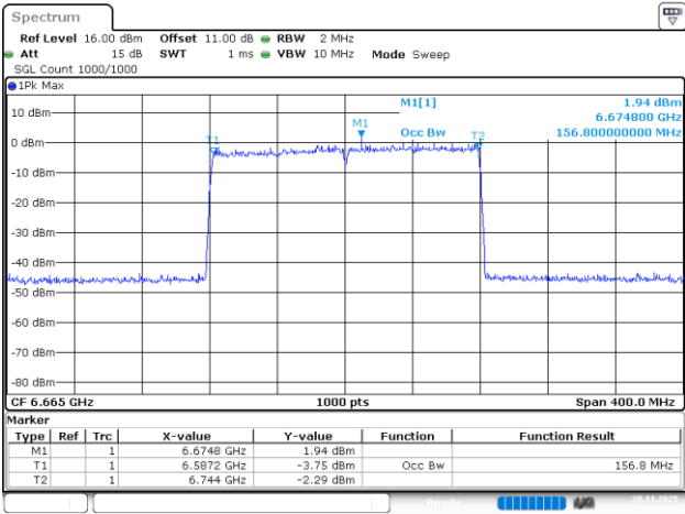
802.11be160_6665MHz_RU_2*996_Chain 0
