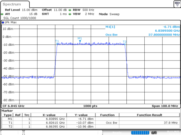
802.11be40_6845MHz_RU_484/65_Chain 0
