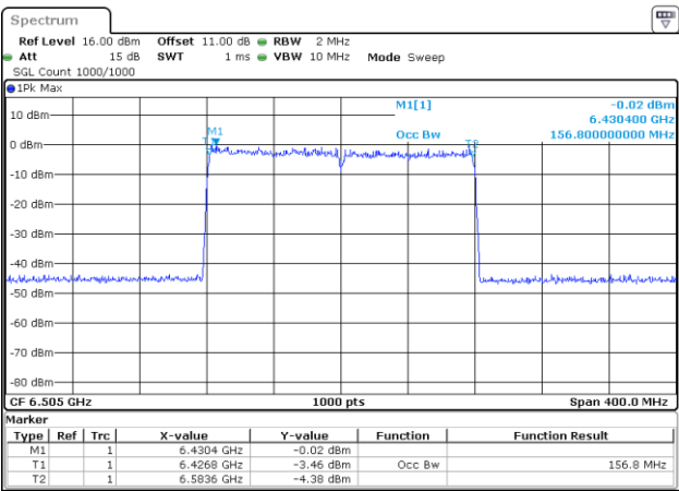
802.11be160_6505MHz_RU_2*996_Chain 0
