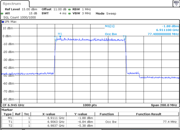
802.11be80_6945MHz_RU_996/67_Chain 2
