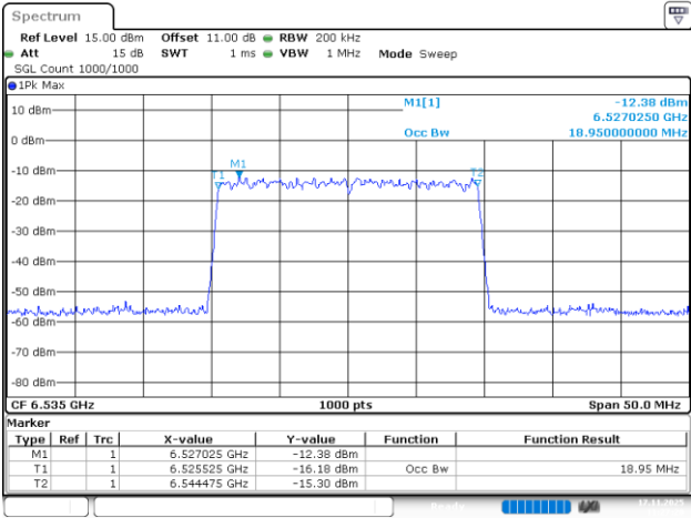
802.11be20_6535MHz_RU_242/61_Chain 3
