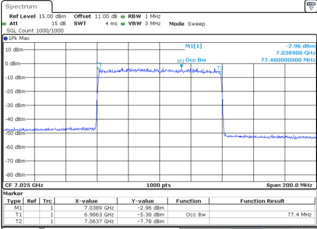
802.11be80_7025MHz_RU_996/67_Chain 2
