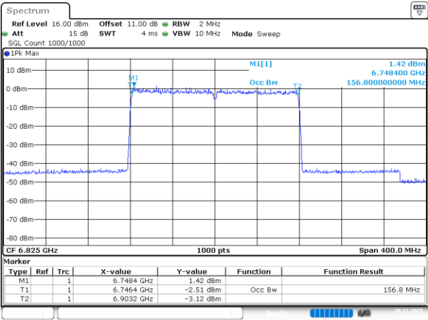
802.11be160_6825MHz_RU_2*996_Chain 0
