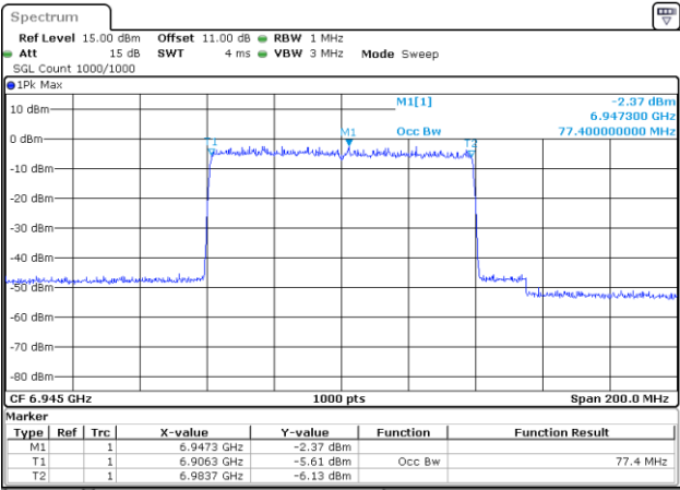
802.11be80_6945MHz_RU_996/67_Chain 1
