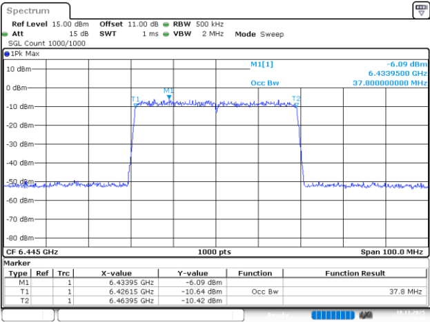
802.11be40_6445MHz_RU_484/65_Chain 3
