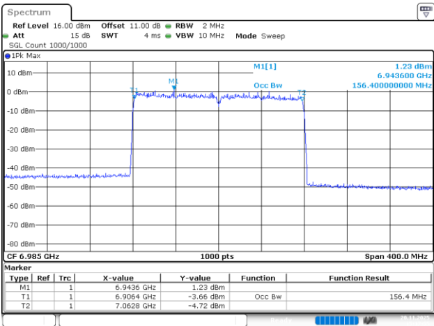
802.11be160_6985MHz_RU_2*996_Chain 1
