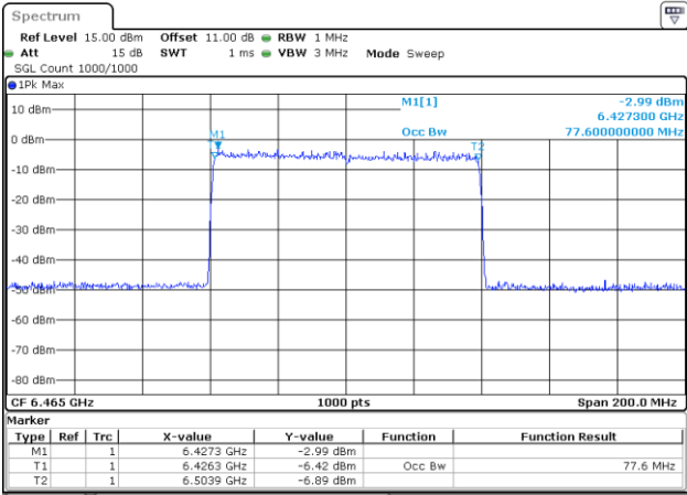
802.11be80_6465MHz_RU_996/67_Chain 3
