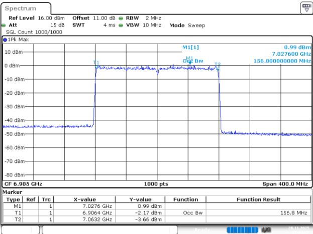
802.11be160_6985MHz_RU_2*996_Chain 2
