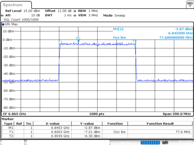
802.11be80_6865MHz_RU_996/67_Chain 0
