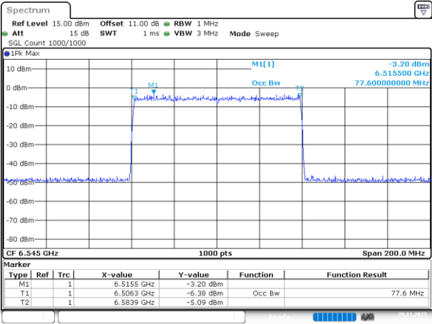
802.11be80_6545MHz_RU_996/67_Chain 0
