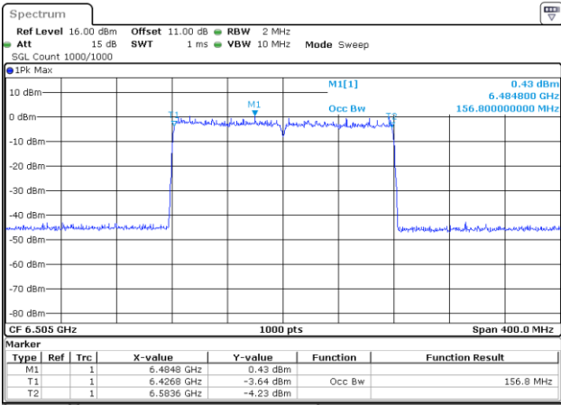
802.11be160_6505MHz_RU_2*996_Chain 3
