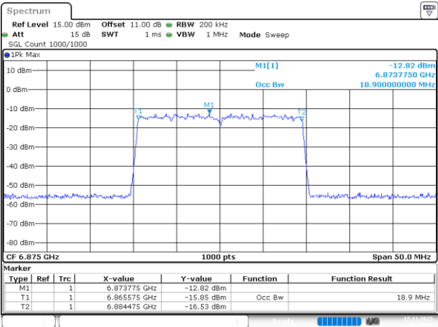
802.11be20_6875MHz_RU_242/61_Chain 1
