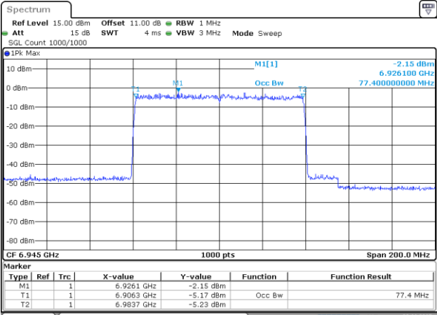
802.11be80_6945MHz_RU_996/67_Chain 3
