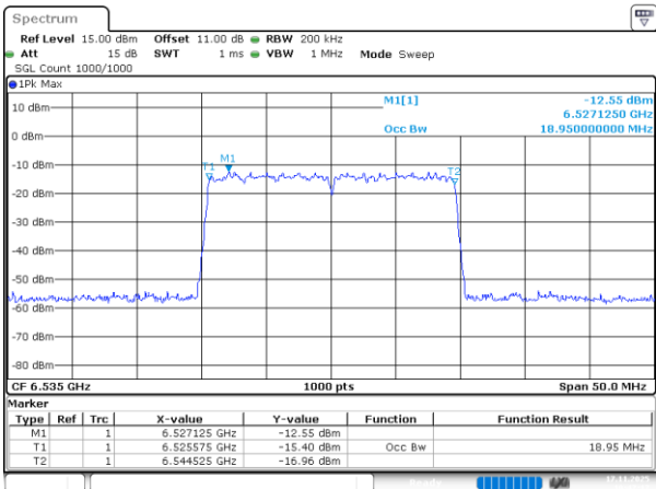
802.11be20_6535MHz_RU_242/61_Chain 1
