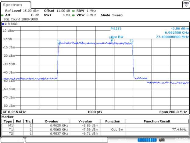
802.11be80_6945MHz_RU_996/67_Chain 0
