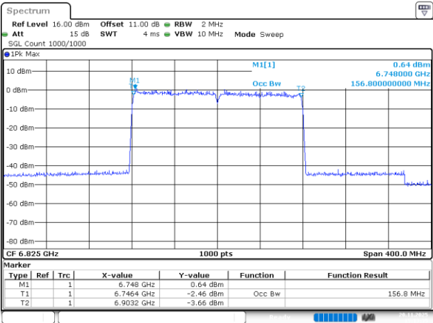
802.11be160_6825MHz_RU_2*996_Chain 1
