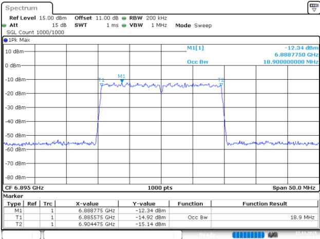
802.11be20_6895MHz_RU_242/61_Chain 2
