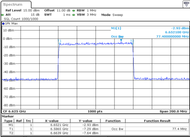
802.11be80_6625MHz_RU_996/67_Chain 2
