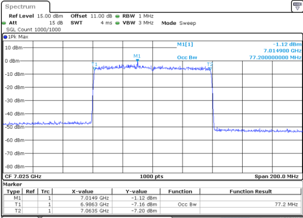
802.11be80_7025MHz_RU_996/67_Chain 3
