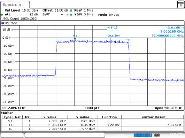
802.11be80_7025MHz_RU_996/67_Chain 0
