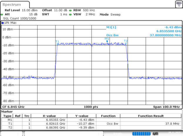
802.11be40_6845MHz_RU_484/65_Chain 1
