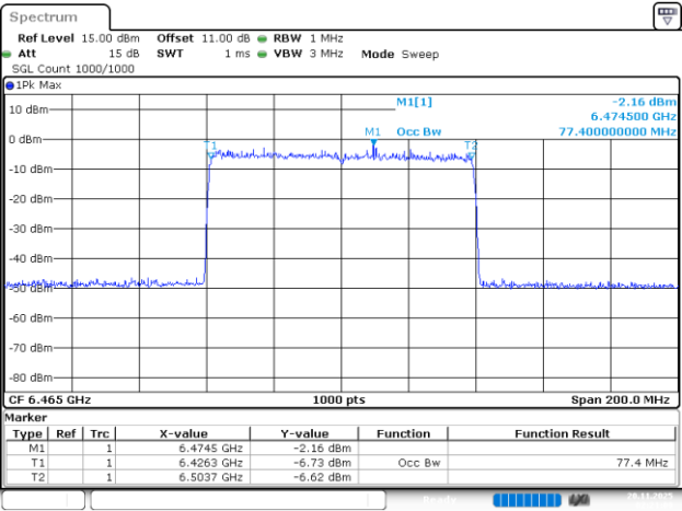
802.11be80_6465MHz_RU_996/67_Chain 1
