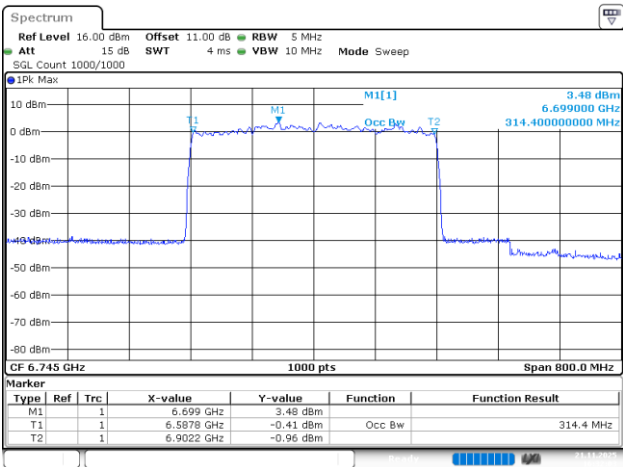
802.11be320_6745MHz_RU_4*996_Chain 0
