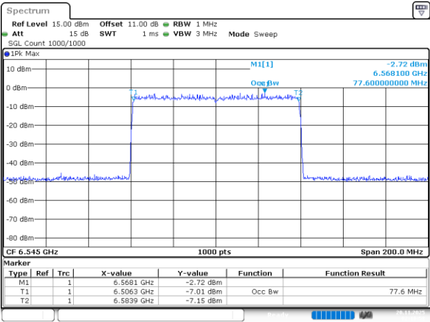
802.11be80_6545MHz_RU_996/67_Chain 1
