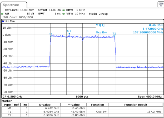
802.11be160_6505MHz_RU_2*996_Chain 1
