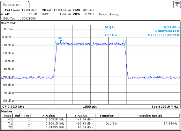
802.11be40_6925MHz_RU_484/65_Chain 1
