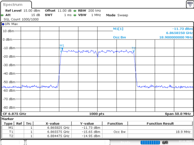
802.11be20_6875MHz_RU_242/61_Chain 3
