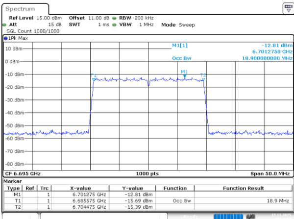
802.11be20_6695MHz_RU_242/61_Chain 0
