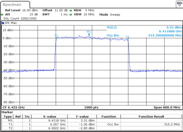
802.11be320_6425MHz_RU_4*996_Chain 2
