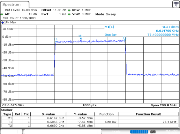
802.11be80_6625MHz_RU_996/67_Chain 0
