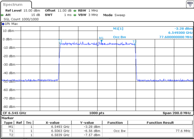
802.11be80_6545MHz_RU_996/67_Chain 3
