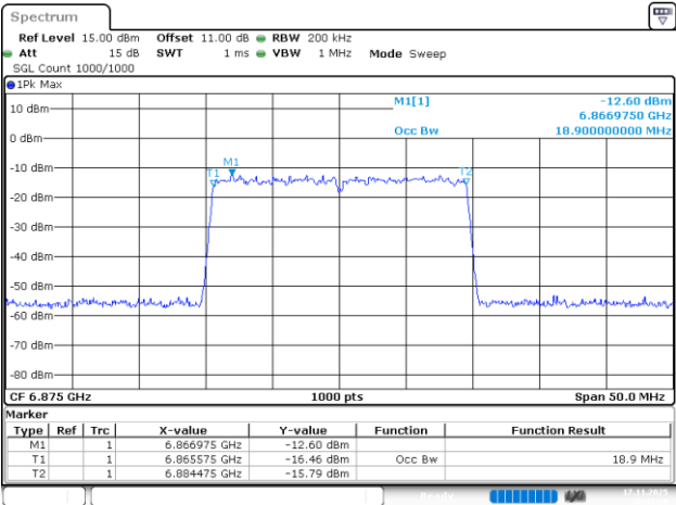
802.11be20_6875MHz_RU_242/61_Chain 2
