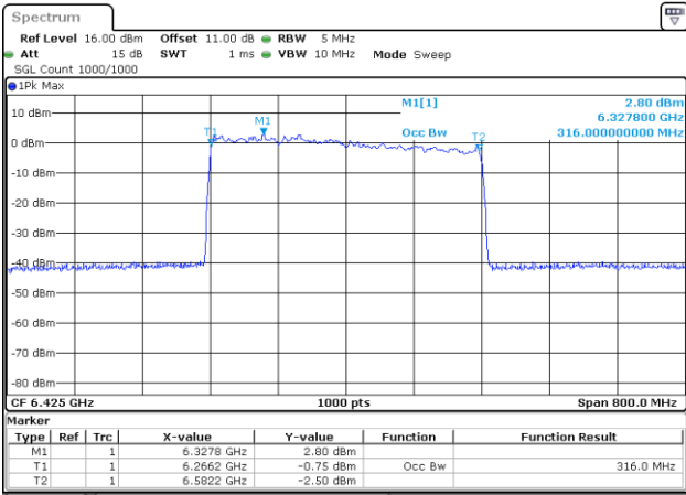
802.11be320_6425MHz_RU_4*996_Chain 3
