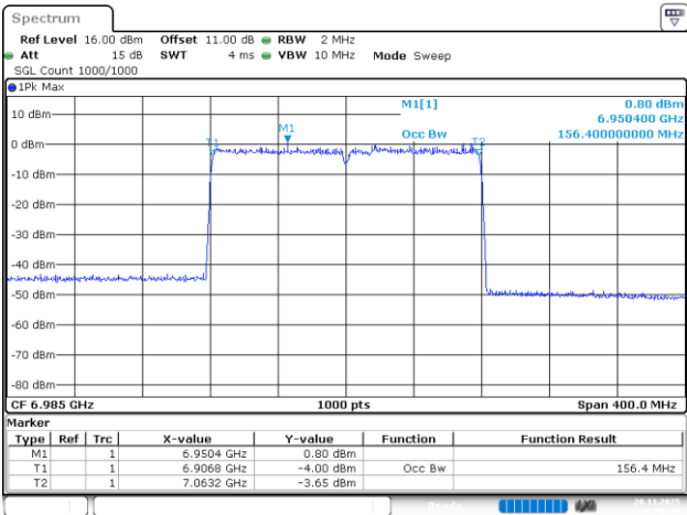
802.11be160_6985MHz_RU_2*996_Chain 3
