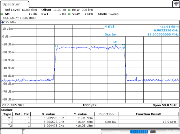
802.11be20_6895MHz_RU_242/61_Chain 3
