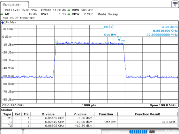
802.11be40_6845MHz_RU_484/65_Chain 3
