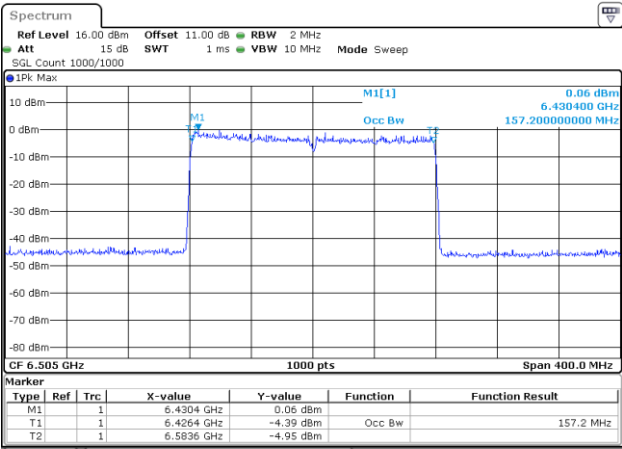
802.11be160_6505MHz_RU_2*996_Chain 2
