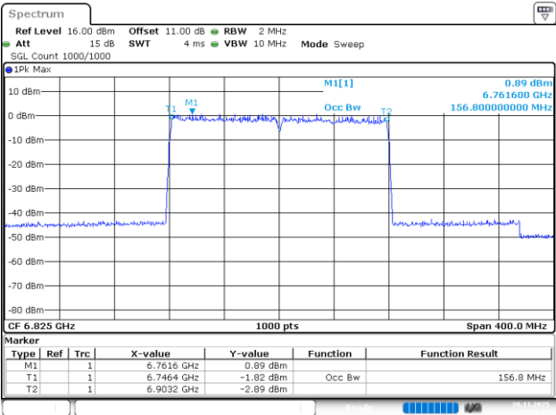
802.11be160_6825MHz_RU_2*996_Chain 3
