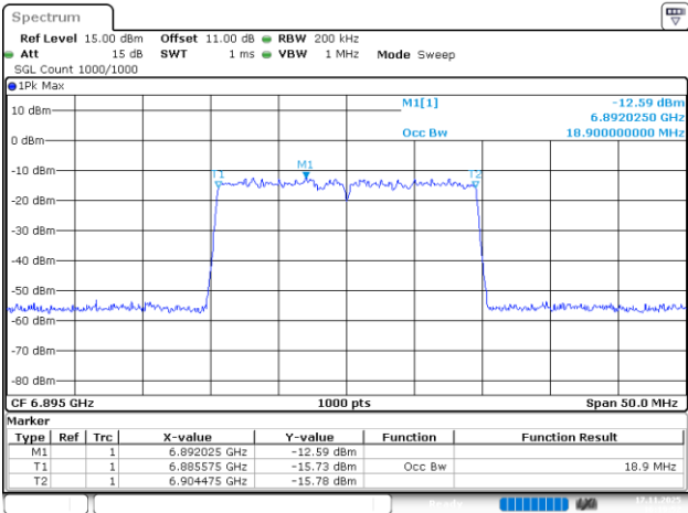
802.11be20_6895MHz_RU_242/61_Chain 1
