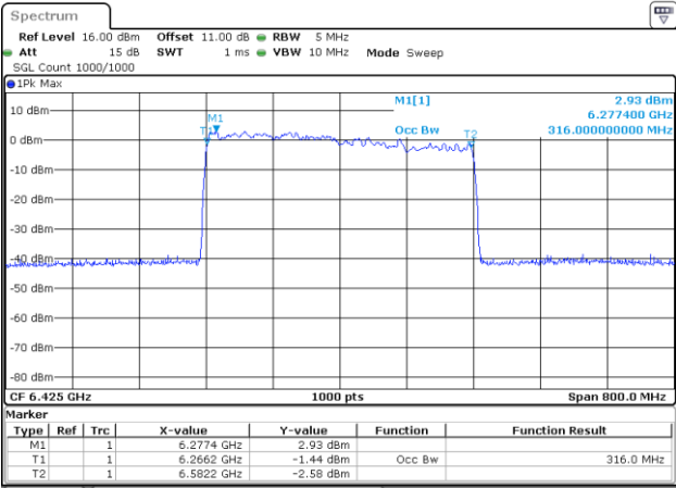
802.11be320_6425MHz_RU_4*996_Chain 0
