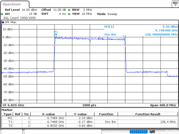
802.11be160_6825MHz_RU_2*996_Chain 2
