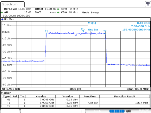
802.11be160_6985MHz_RU_2*996_Chain 0
