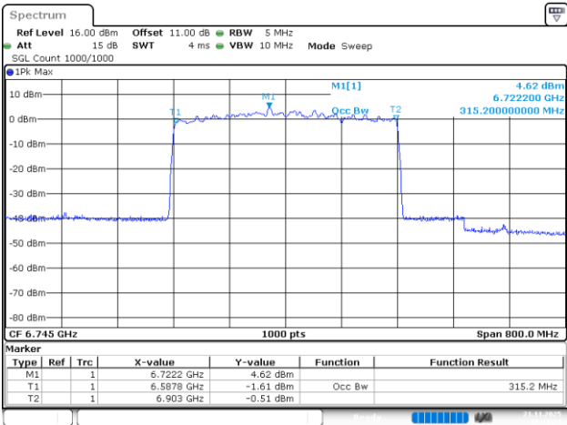
802.11be320_6745MHz_RU_4*996_Chain 1
