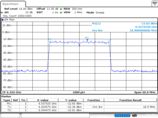
802.11be20_6535MHz_RU_242/61_Chain 2
