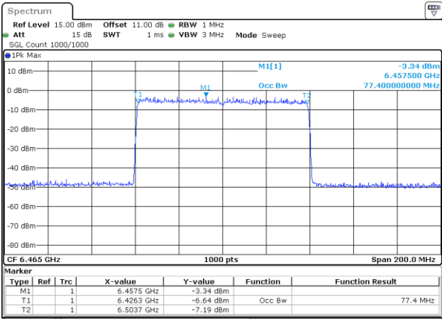
802.11be80_6465MHz_RU_996/67_Chain 2
