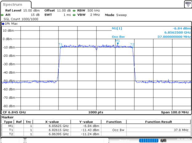
802.11be40_6845MHz_RU_484/65_Chain 2
