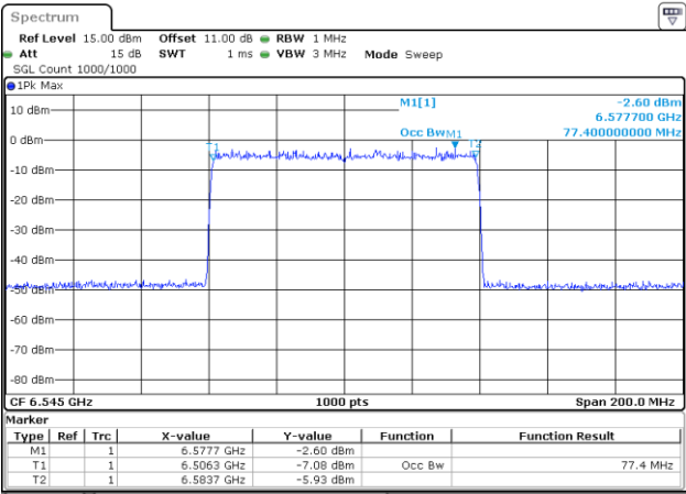
802.11be80_6545MHz_RU_996/67_Chain 2
