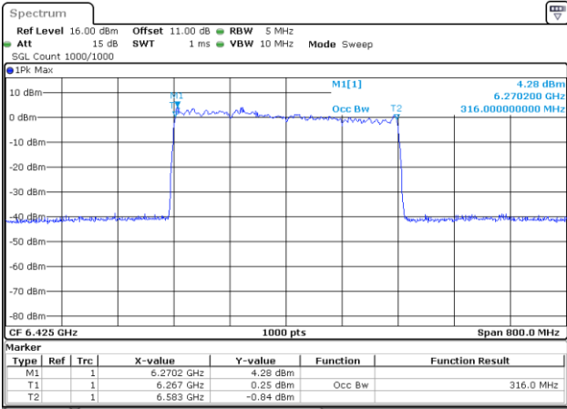
802.11be320_6425MHz_RU_4*996_Chain 1
