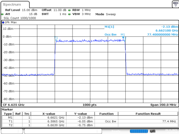
802.11be80_6625MHz_RU_996/67_Chain 3
