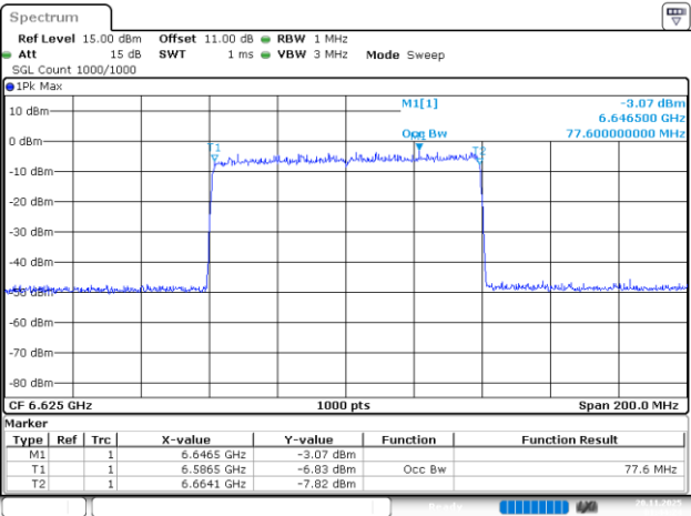
802.11be80_6625MHz_RU_996/67_Chain 1
