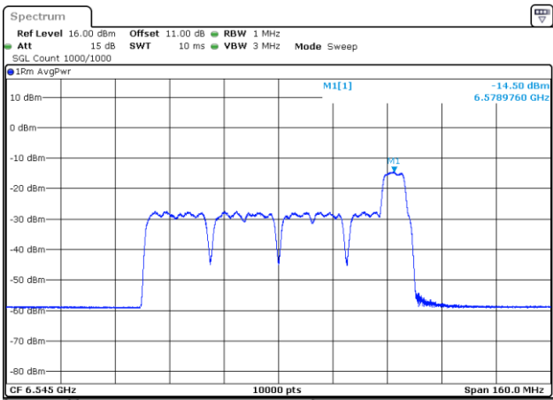
802.11be80_6545MHz_RU_26&52_MRU11_Chain 1
