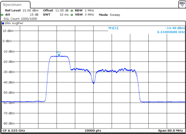
802.11be40_6525MHz_RU_106/53_Chain 2
