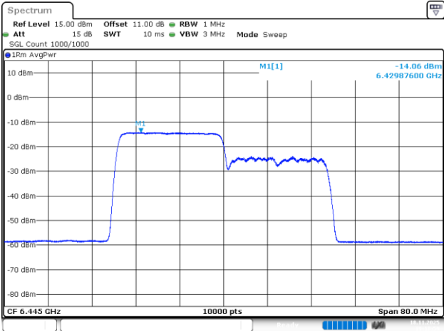
802.11be40_6445MHz_RU_242/61_Chain 0
