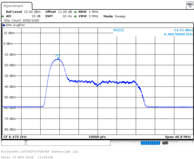
802.11be20_6475MHz_RU_26/0_Chain 1
