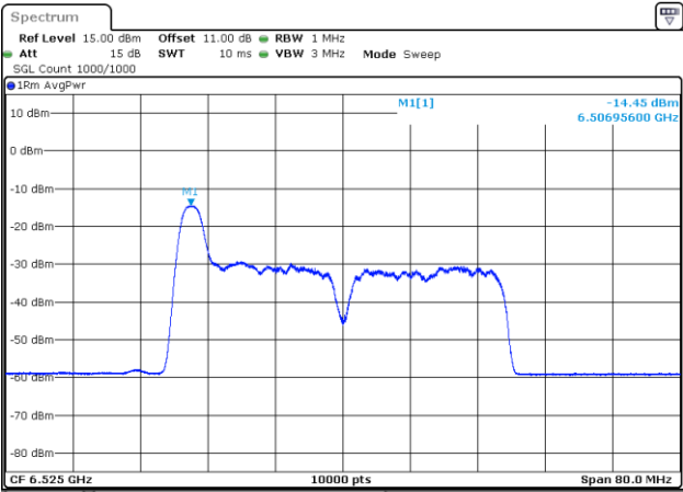
802.11be40_6525MHz_RU_26/0_Chain 2
