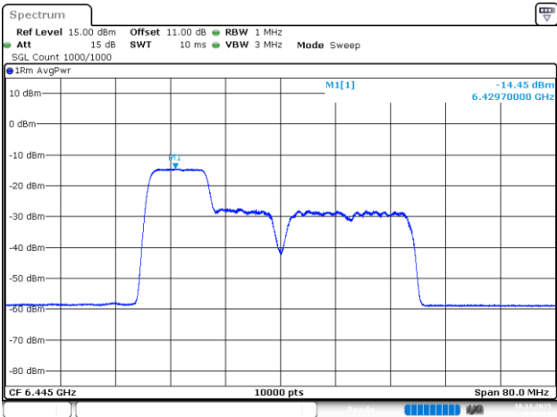
802.11be40_6445MHz_RU_106/53_Chain 0
