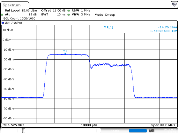
802.11be40_6525MHz_RU_242/61_Chain 2
