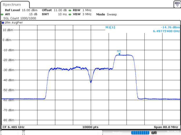
802.11be40_6485MHz_RU_106/56_Chain 2
