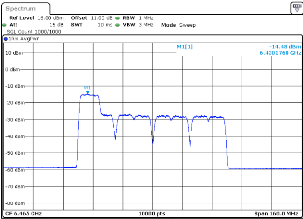
802.11be80_6465MHz_RU_26&106_MRU1_Chain 0
