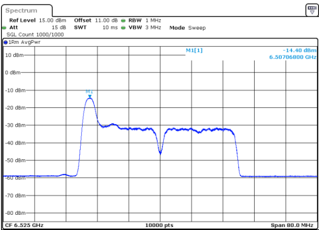
802.11be40_6525MHz_RU_26/0_Chain 1
