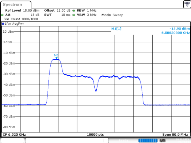
802.11be40_6525MHz_RU_52/37_Chain 3
