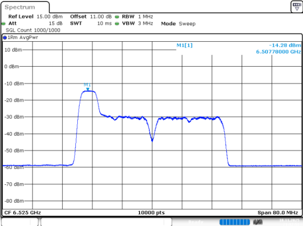
802.11be40_6525MHz_RU_52/37_Chain 0
