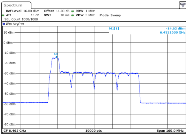
802.11be80_6465MHz_RU_26&52_MRU2_Chain 0
