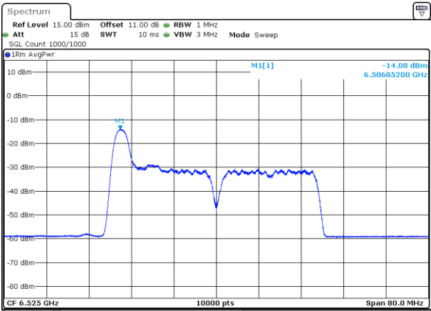
802.11be40_6525MHz_RU_26/0_Chain 0
