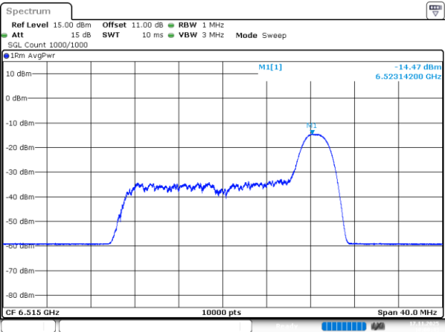
802.11be20_6515MHz_RU_26/8_Chain 3
