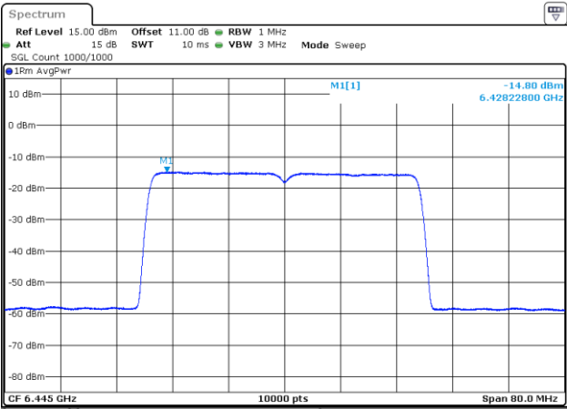
802.11be40_6445MHz_RU_484/65_Chain 1
