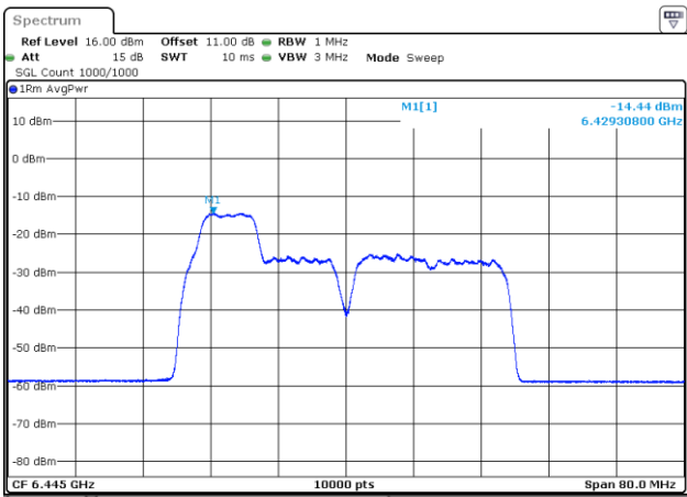
802.11be40_6445MHz_RU_26&52_MRU1_Chain 1
