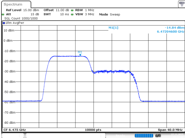
802.11be20_6475MHz_RU_106/53_Chain 0
