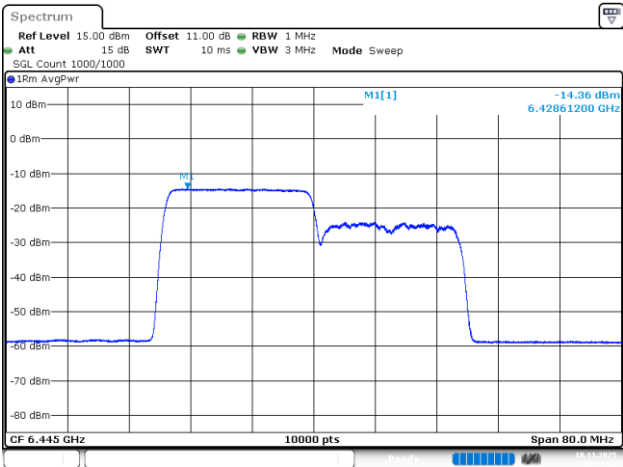
802.11be40_6445MHz_RU_242/61_Chain 3
