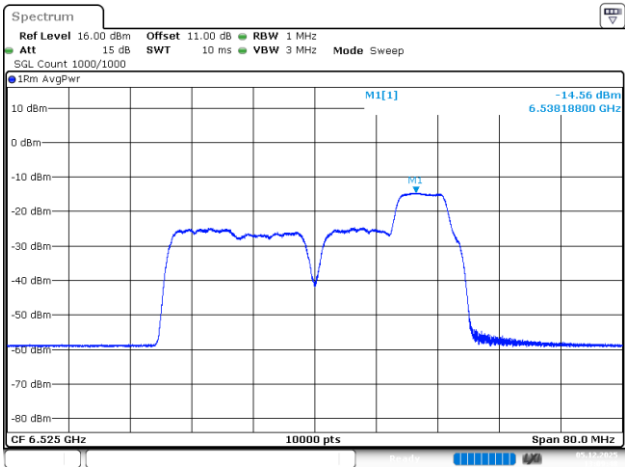
802.11be40_6525MHz_RU_26&52_MRU6_Chain 2
