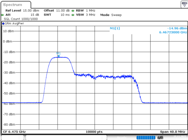
802.11be20_6475MHz_RU_52/37_Chain 2
