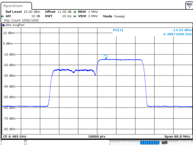
802.11be40_6485MHz_RU_242/62_Chain 1
