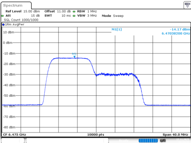
802.11be20_6475MHz_RU_106/53_Chain 2
