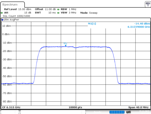
802.11be20_6515MHz_RU_242/61_Chain 0
