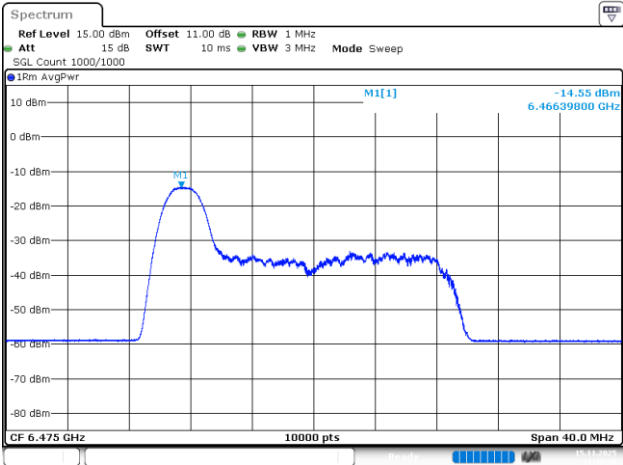
802.11be20_6475MHz_RU_26/0_Chain 3
