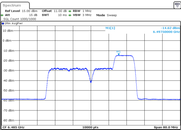
802.11be40_6485MHz_RU_106/56_Chain 0
