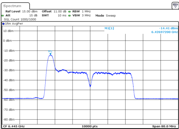
802.11be40_6445MHz_RU_26/0_Chain 1
