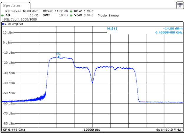
802.11be40_6445MHz_RU_26&106_MRU1_Chain 1
