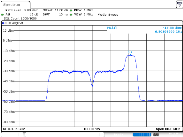
802.11be40_6485MHz_RU_52/44_Chain 1
