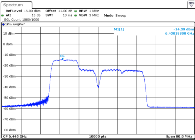
802.11be40_6445MHz_RU_26&106_MRU1_Chain 0
