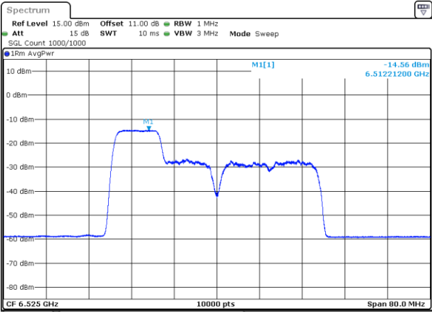
802.11be40_6525MHz_RU_106/53_Chain 3
