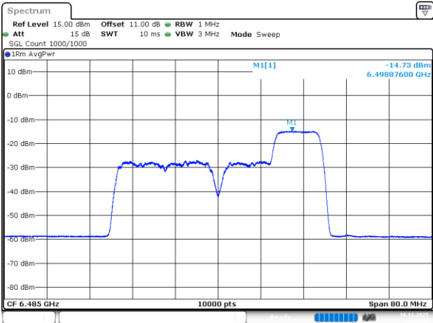
802.11be40_6485MHz_RU_106/56_Chain 3
