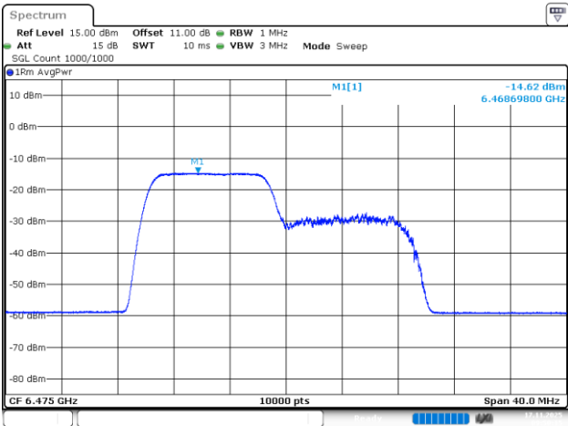
802.11be20_6475MHz_RU_106/53_Chain 3
