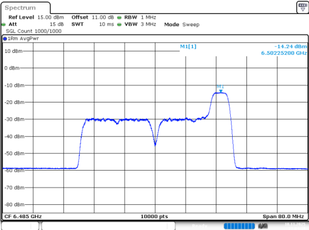
802.11be40_6485MHz_RU_52/44_Chain 0
