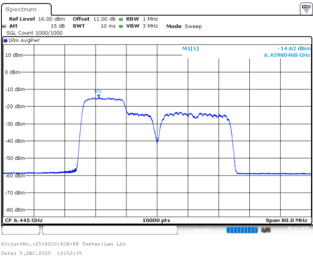
802.11be40_6445MHz_RU_26&106_MRU1_Chain 3
