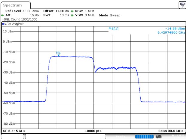
802.11be40_6445MHz_RU_242/61_Chain 2
