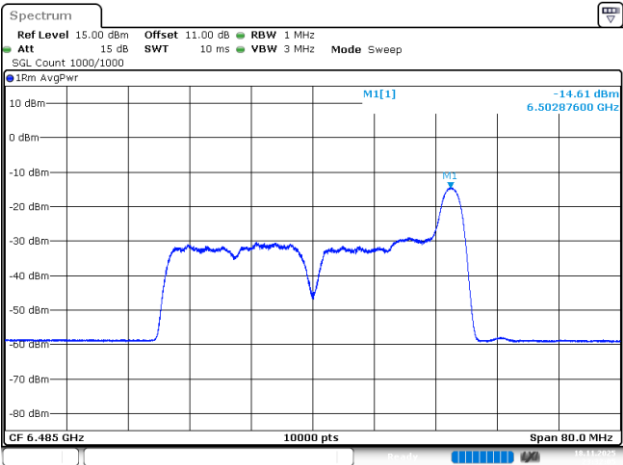
802.11be40_6485MHz_RU_26/17_Chain 2
