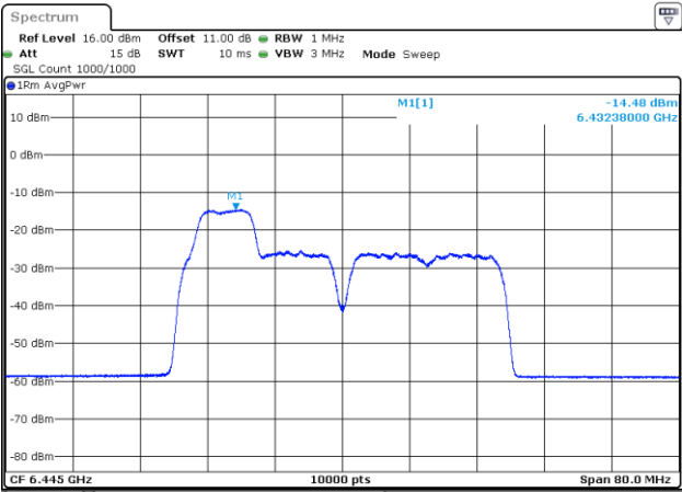
802.11be40_6445MHz_RU_26&52_MRU1_Chain 0
