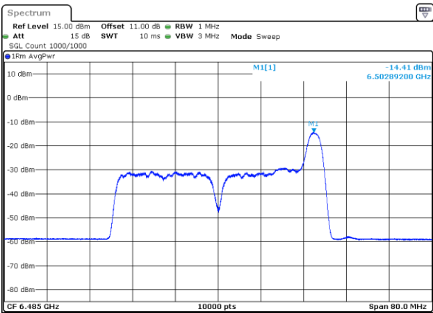
802.11be40_6485MHz_RU_26/17_Chain 1
