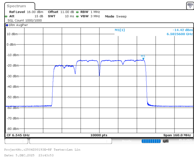
802.11be80_6545MHz_RU_26&52_MRU11_Chain 0
