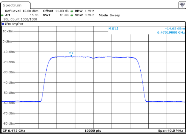
802.11be20_6475MHz_RU_242/61_Chain 1
