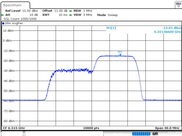
802.11be20_6515MHz_RU_106/54_Chain 3
