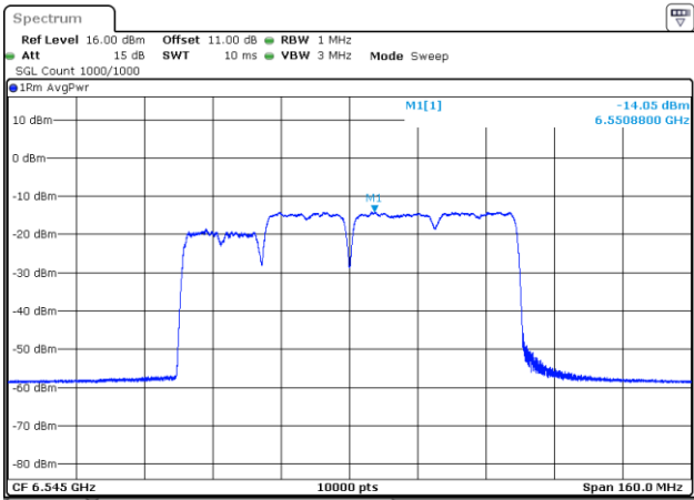
802.11be80_6545MHz_RU_242&484_MRU1_Chain 1
