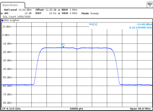
802.11be20_6515MHz_RU_242/61_Chain 2
