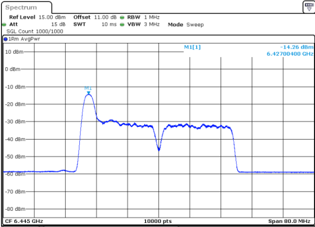
802.11be40_6445MHz_RU_26/0_Chain 3
