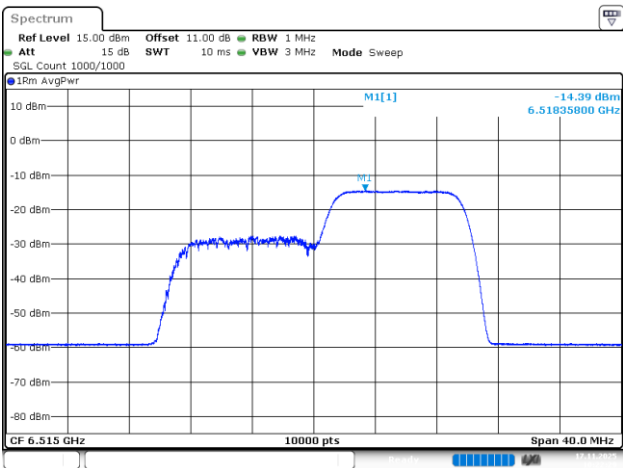
802.11be20_6515MHz_RU_106/54_Chain 1
