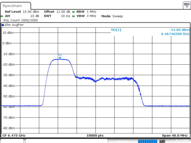
802.11be20_6475MHz_RU_52/37_Chain 1
