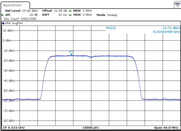
802.11be20_6515MHz_RU_242/61_Chain 1
