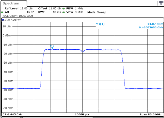
802.11be40_6445MHz_RU_484/65_Chain 2
