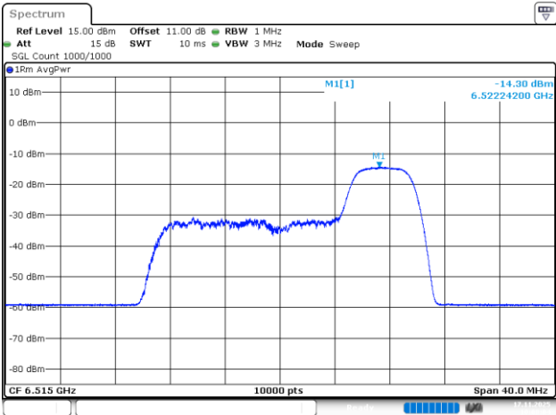
802.11be20_6515MHz_RU_52/40_Chain 1
