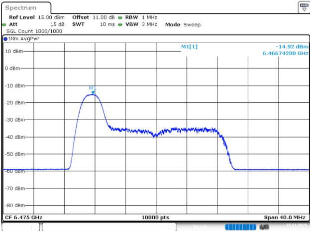
802.11be20_6475MHz_RU_26/0_Chain 2
