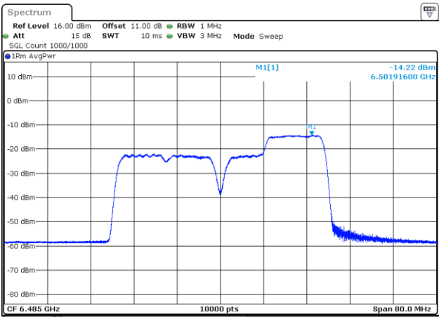
802.11be40_6485MHz_RU_26&106_MRU4_Chain 0
