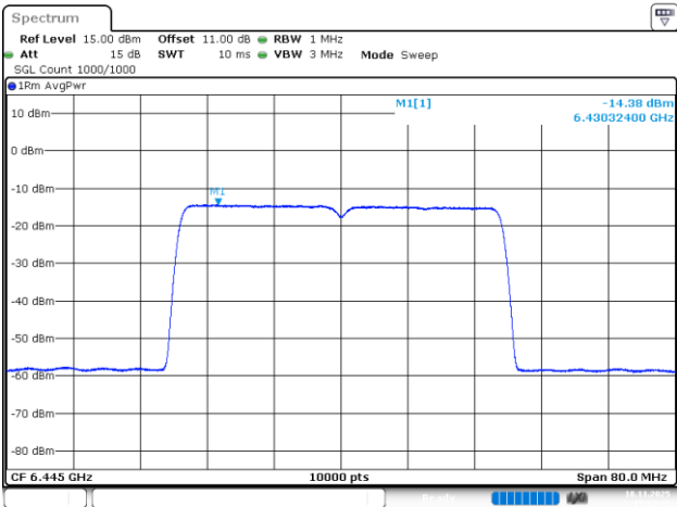
802.11be40_6445MHz_RU_484/65_Chain 0
