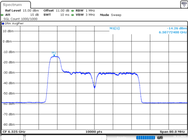
802.11be40_6525MHz_RU_52/37_Chain 1
