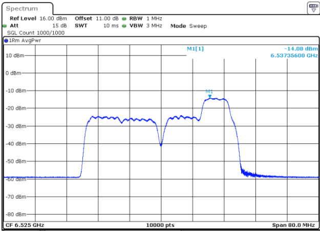
802.11be40_6525MHz_RU_26&52_MRU6_Chain 1
