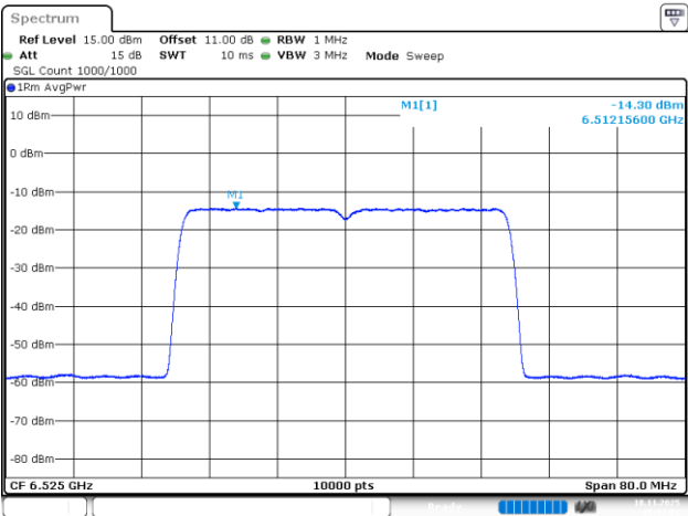
802.11be40_6525MHz_RU_484/65_Chain 0
