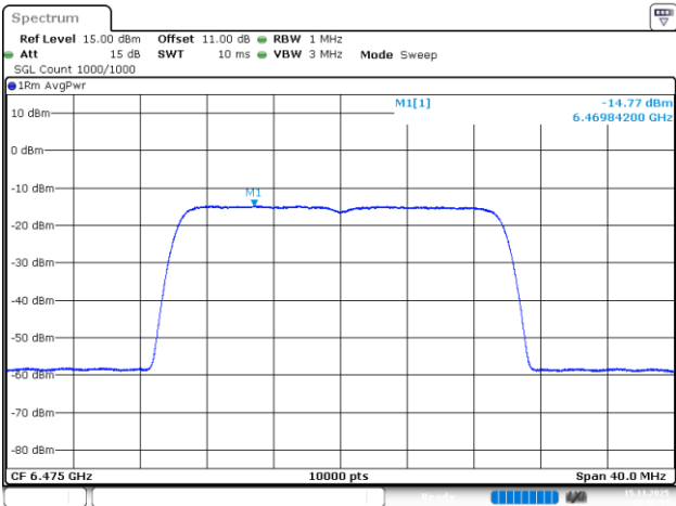
802.11be20_6475MHz_RU_242/61_Chain 0
