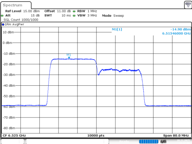
802.11be40_6525MHz_RU_242/61_Chain 3
