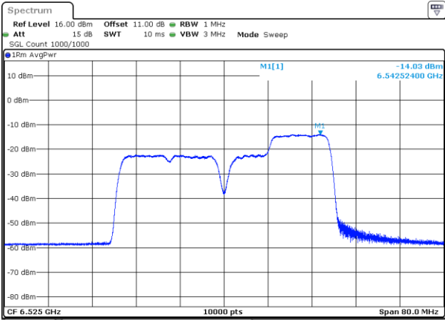
802.11be40_6525MHz_RU_26&106_MRU4_Chain 0
