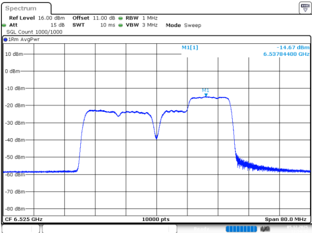
802.11be40_6525MHz_RU_26&106_MRU4_Chain 2
