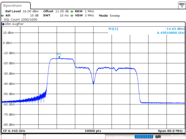
802.11be40_6445MHz_RU_26&106_MRU1_Chain 2
