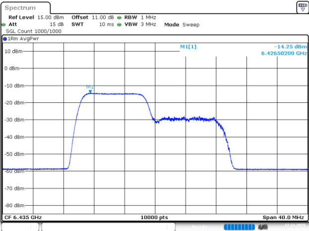
802.11be20_6435MHz_RU_106/53_Chain 1
