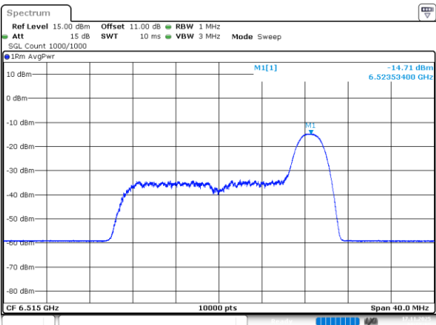
802.11be20_6515MHz_RU_26/8_Chain 0
