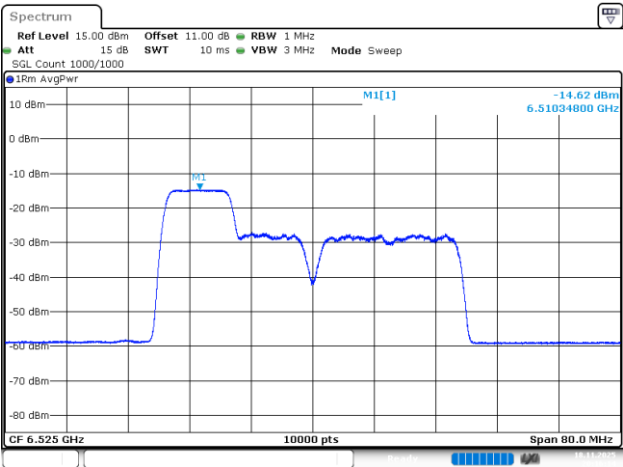
802.11be40_6525MHz_RU_106/53_Chain 0
