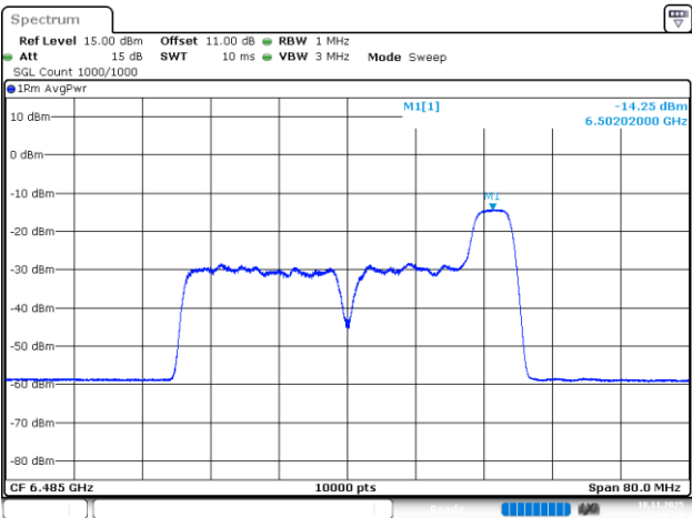
802.11be40_6485MHz_RU_52/44_Chain 2
