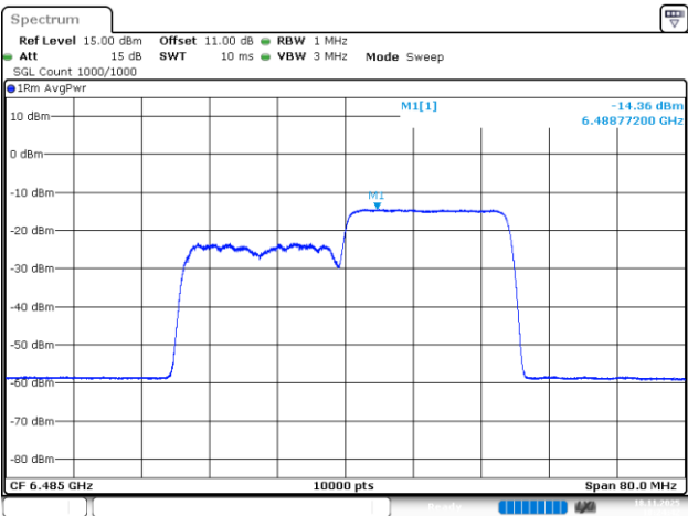
802.11be40_6485MHz_RU_242/62_Chain 2
