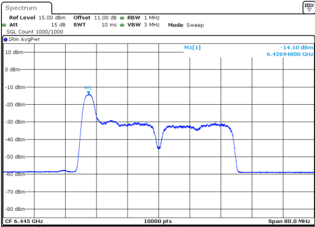
802.11be40_6445MHz_RU_26/0_Chain 2
