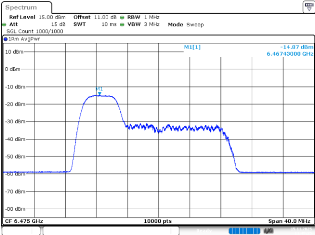
802.11be20_6475MHz_RU_52/37_Chain 3
