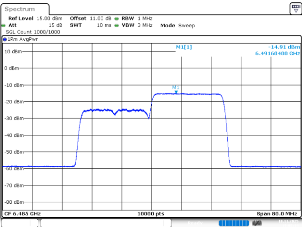
802.11be40_6485MHz_RU_242/62_Chain 0
