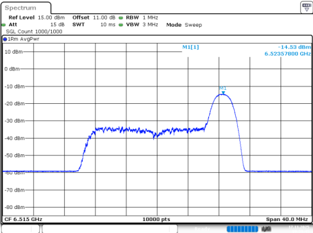
802.11be20_6515MHz_RU_26/8_Chain 2
