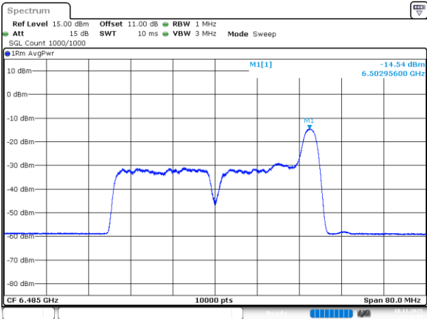
802.11be40_6485MHz_RU_26/17_Chain 3
