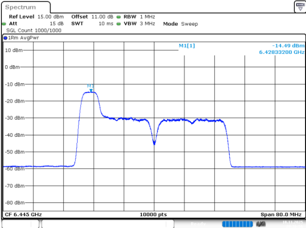
802.11be40_6445MHz_RU_52/37_Chain 3
