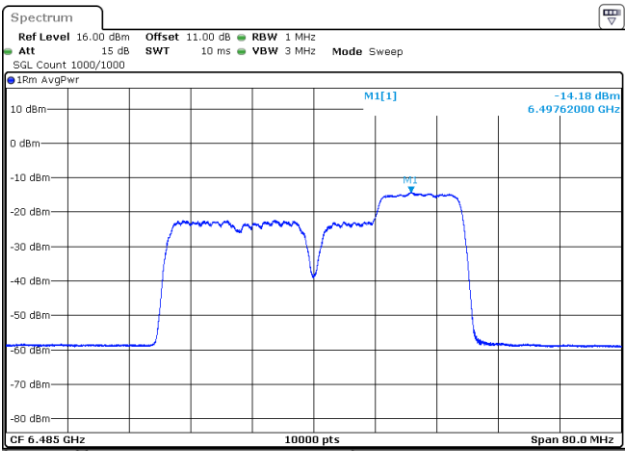
802.11be40_6485MHz_RU_26&106_MRU4_Chain 3
