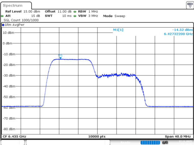
802.11be20_6435MHz_RU_106/53_Chain 2
