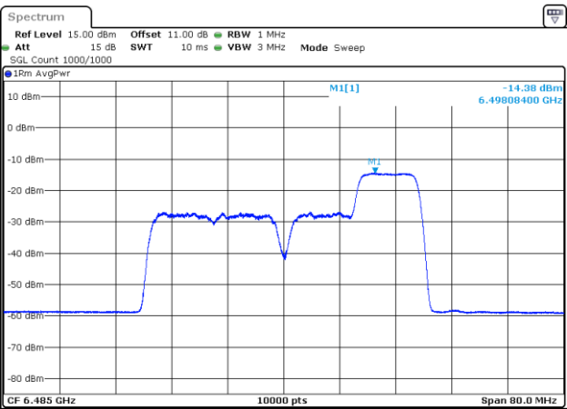
802.11be40_6485MHz_RU_106/56_Chain 1
