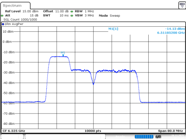
802.11be40_6525MHz_RU_106/53_Chain 1
