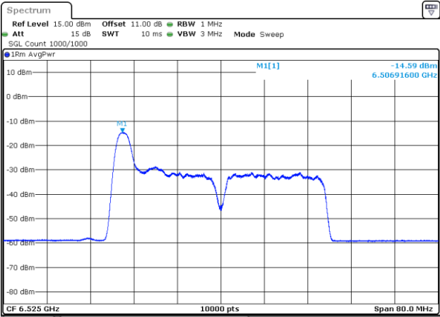
802.11be40_6525MHz_RU_26/0_Chain 3
