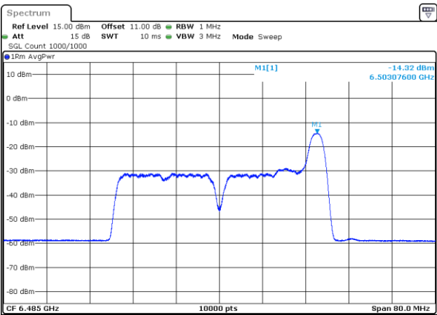
802.11be40_6485MHz_RU_26/17_Chain 0
