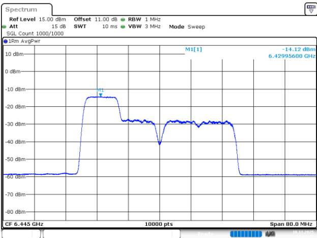
802.11be40_6445MHz_RU_106/53_Chain 1
