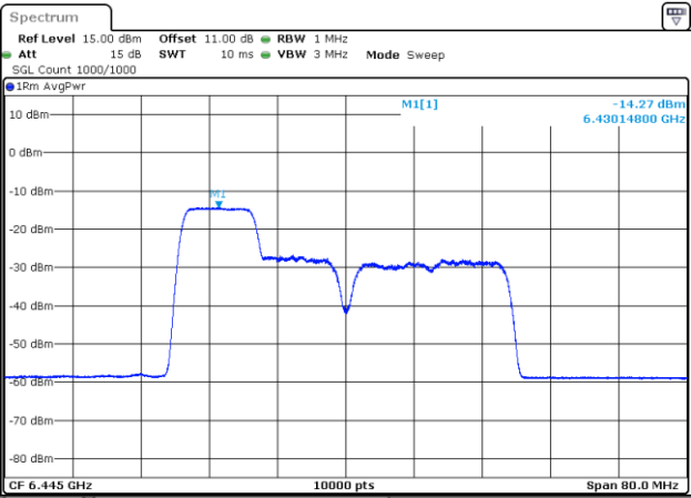
802.11be40_6445MHz_RU_106/53_Chain 2
