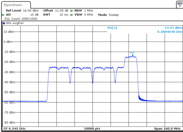
802.11be80_6545MHz_RU_26&106_MRU8_Chain 1
