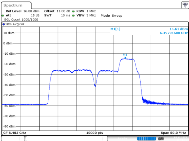
802.11be40_6485MHz_RU_26&52_MRU6_Chain 1
