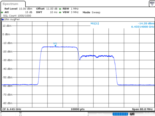
802.11be40_6445MHz_RU_242/61_Chain 1
