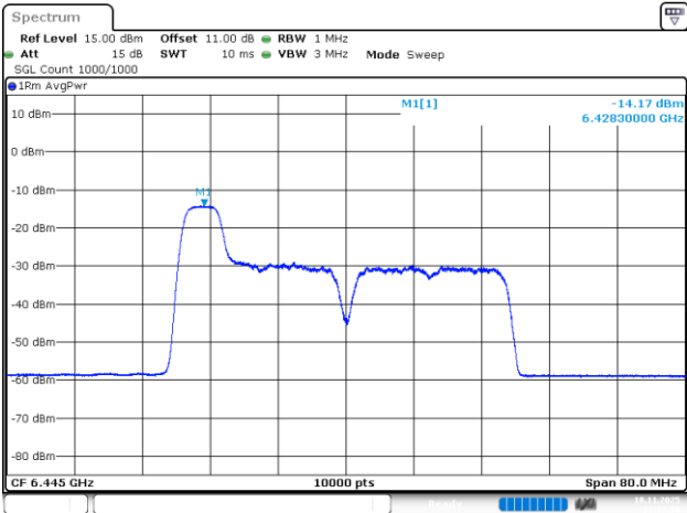
802.11be40_6445MHz_RU_52/37_Chain 1
