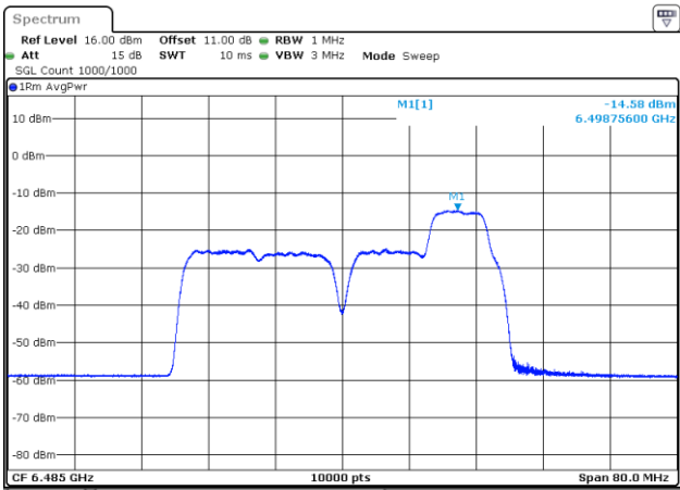
802.11be40_6485MHz_RU_26&52_MRU6_Chain 3
