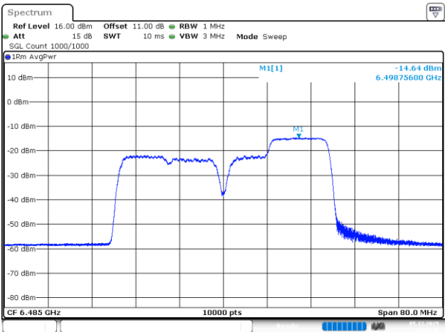
802.11be40_6485MHz_RU_26&106_MRU4_Chain 1
