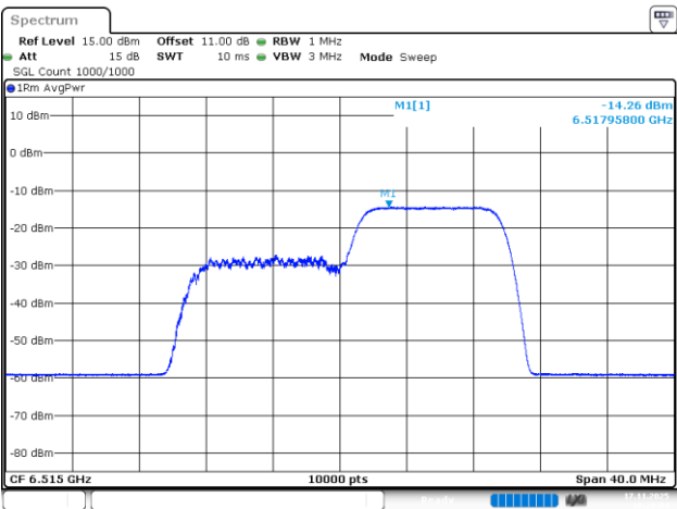
802.11be20_6515MHz_RU_106/54_Chain 0
