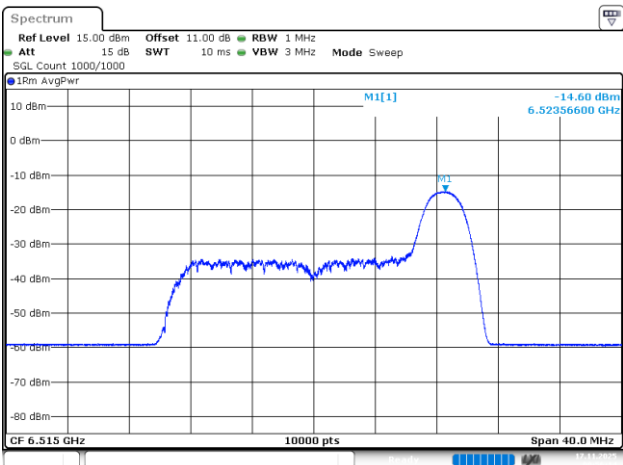
802.11be20_6515MHz_RU_26/8_Chain 1
