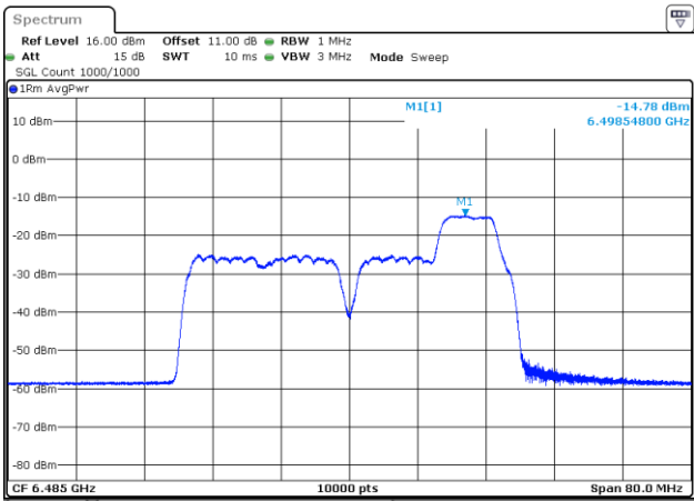
802.11be40_6485MHz_RU_26&52_MRU6_Chain 0
