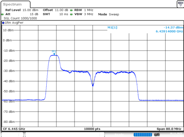
802.11be40_6445MHz_RU_52/37_Chain 0
