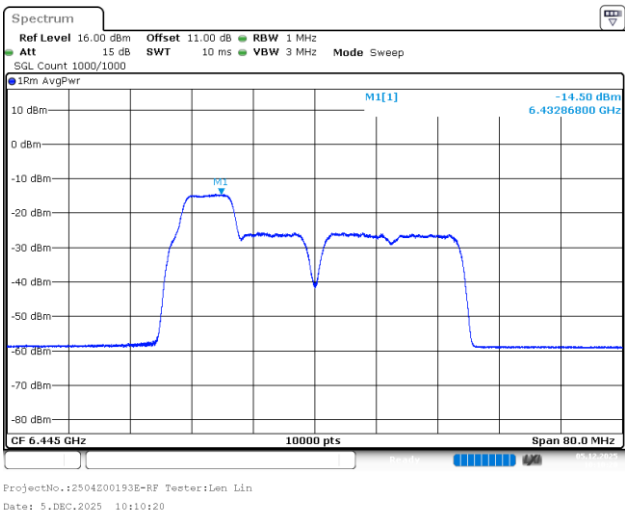
802.11be40_6445MHz_RU_26&52_MRU1_Chain 3
