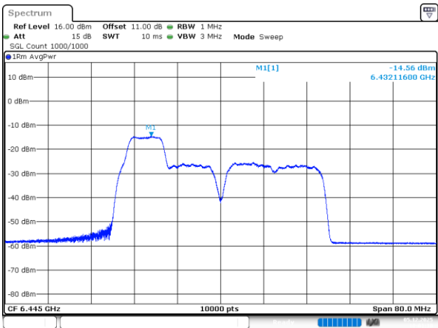
802.11be40_6445MHz_RU_26&52_MRU1_Chain 2
