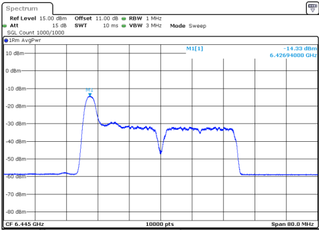
802.11be40_6445MHz_RU_26/0_Chain 0
