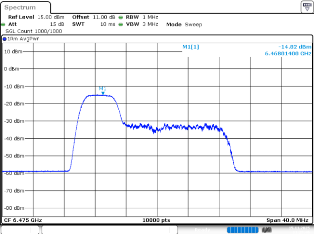
802.11be20_6475MHz_RU_52/37_Chain 0
