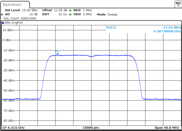
802.11be20_6515MHz_RU_242/61_Chain 3
