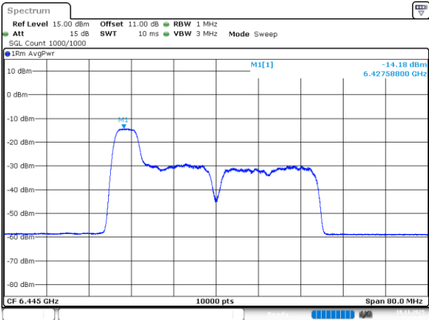
802.11be40_6445MHz_RU_52/37_Chain 2
