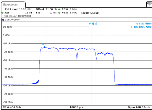
802.11be80_6465MHz_RU_242&484_MRU4_Chain 1
