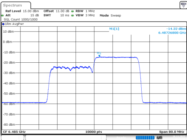
802.11be40_6485MHz_RU_242/62_Chain 3
