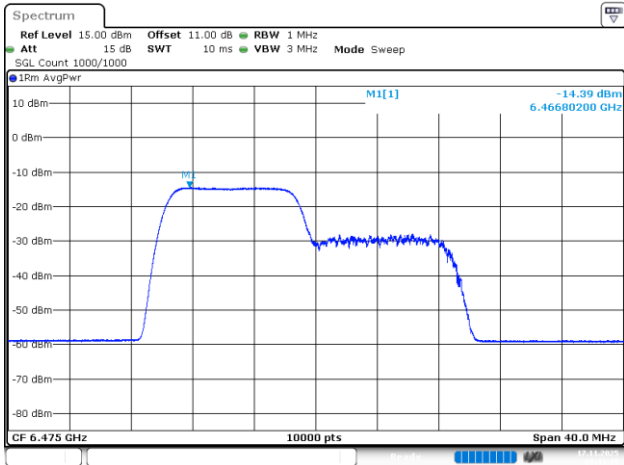
802.11be20_6475MHz_RU_106/53_Chain 1
