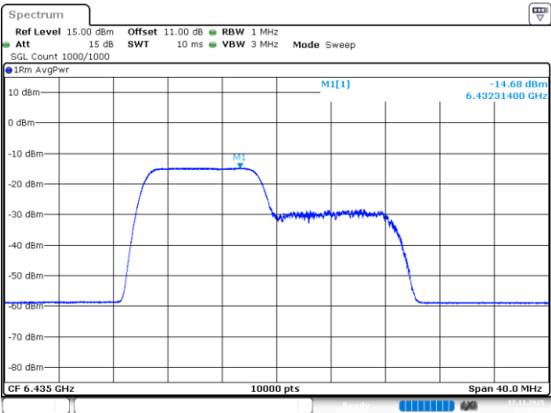
802.11be20_6435MHz_RU_106/53_Chain 3
