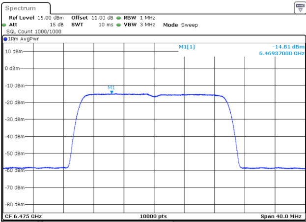
802.11be20_6475MHz_RU_242/61_Chain 2
