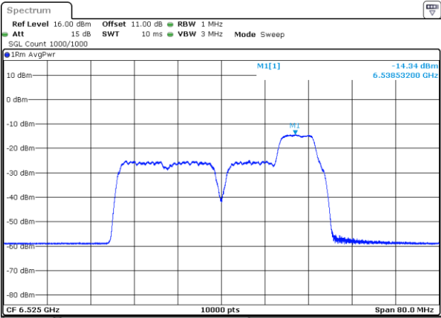
802.11be40_6525MHz_RU_26&52_MRU6_Chain 0
