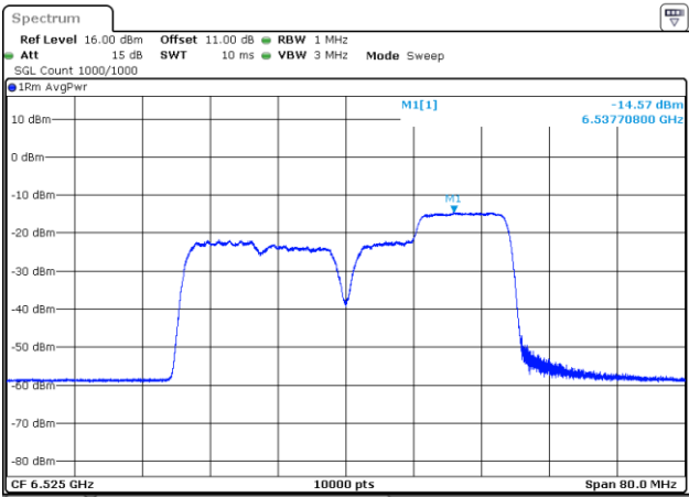
802.11be40_6525MHz_RU_26&106_MRU4_Chain 1
