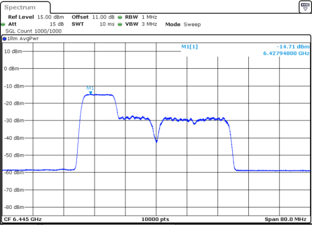
802.11be40_6445MHz_RU_106/53_Chain 3
