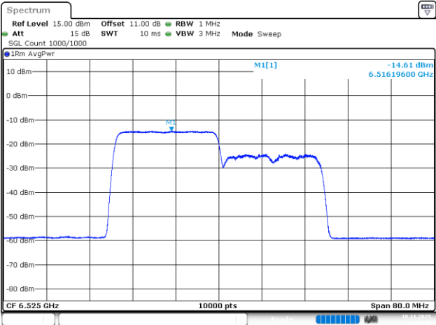
802.11be40_6525MHz_RU_242/61_Chain 0
