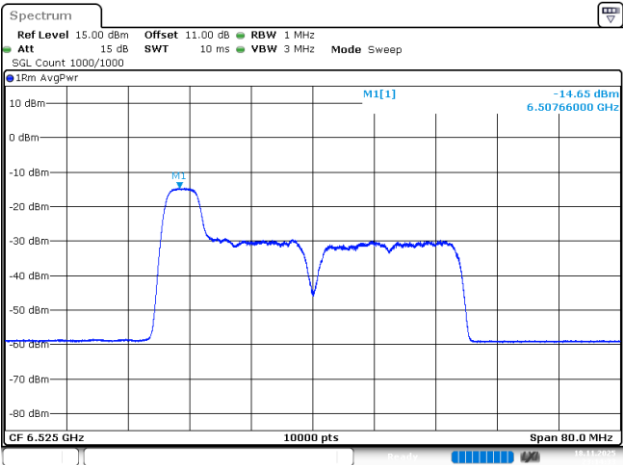
802.11be40_6525MHz_RU_52/37_Chain 2
