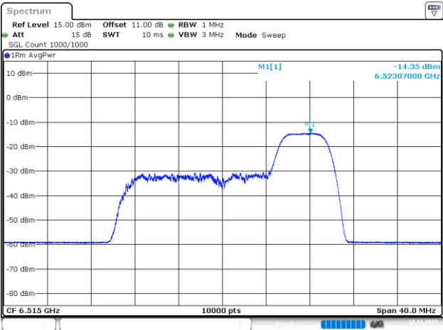
802.11be20_6515MHz_RU_52/40_Chain 0
