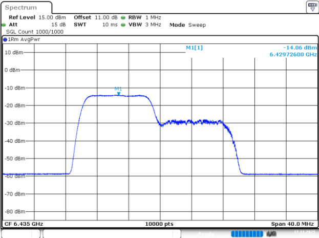
802.11be20_6435MHz_RU_106/53_Chain 0
