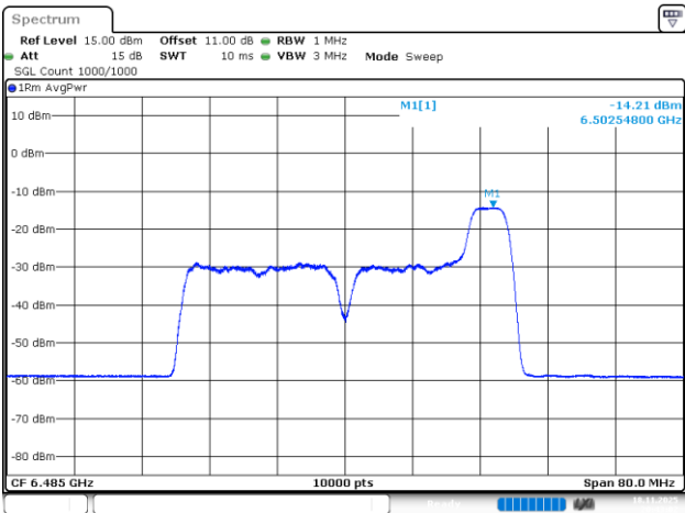
802.11be40_6485MHz_RU_52/44_Chain 3
