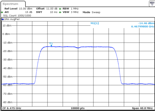
802.11be20_6475MHz_RU_242/61_Chain 3
