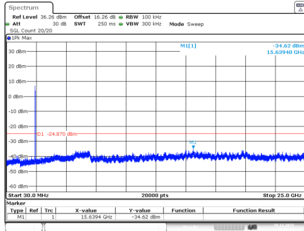
802.11g_2412MHz_Chain 3
