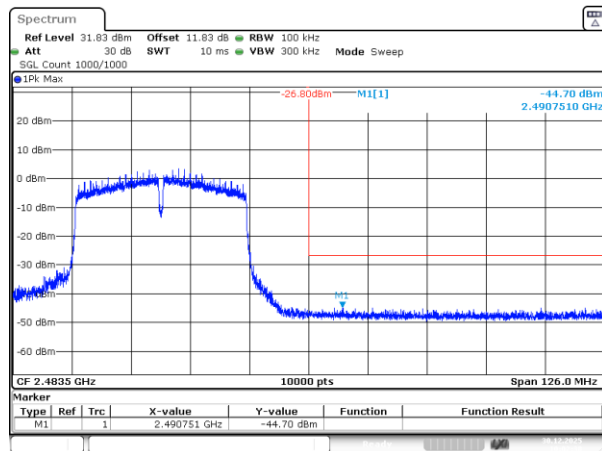
802.11n40_2452MHz_Chain 0
