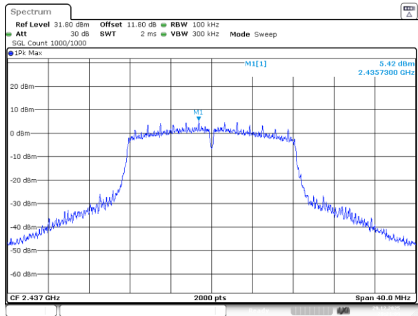
802.11g_2437MHz_Chain 0
