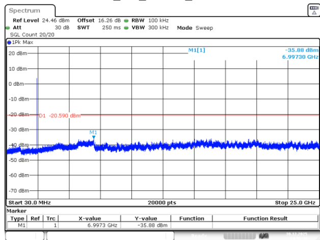
BLE_2M_Middle_Channel
