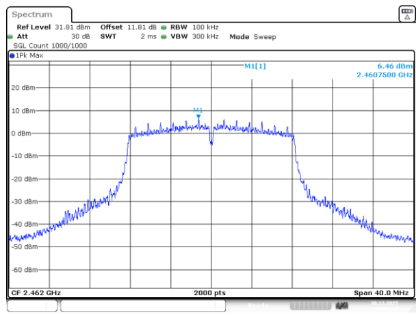
802.11g_2462MHz_Chain 3
