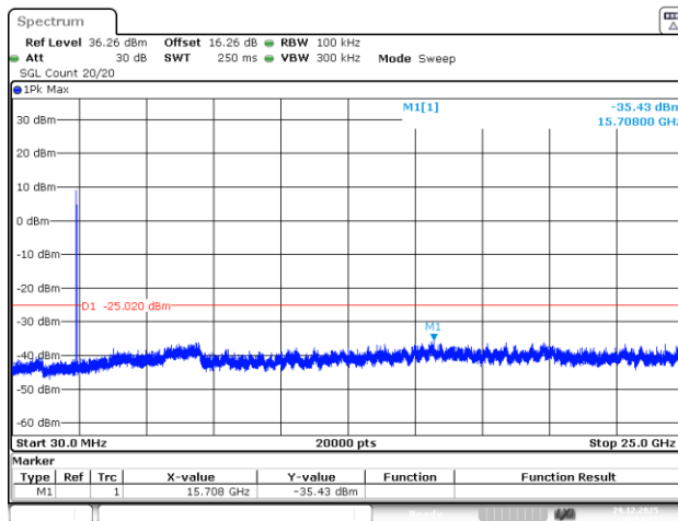
802.11g_2412MHz_Chain 1
