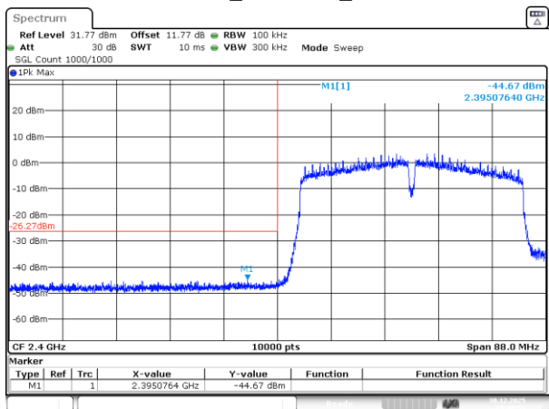
802.11n40_2422MHz_Chain 0
