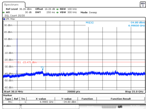
802.11g_2462MHz_Chain 0
