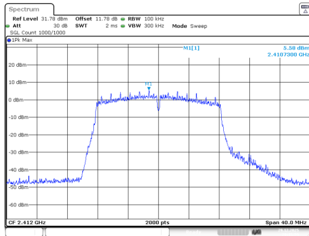
802.11g_2412MHz_Chain 2
