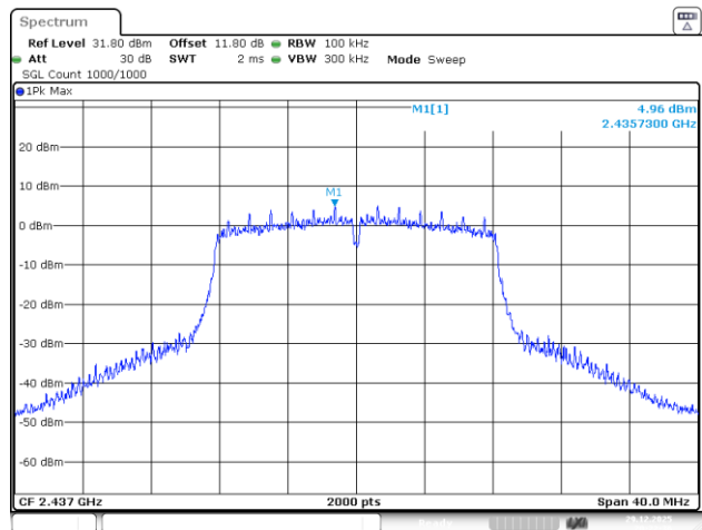
802.11g_2437MHz_Chain 1
