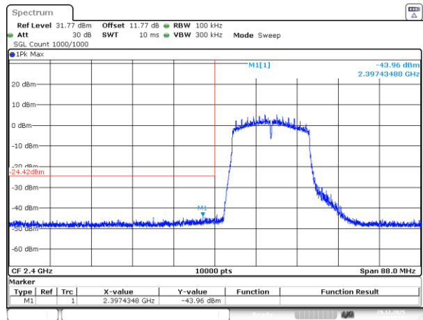
802.11g_2412MHz_Chain 2
