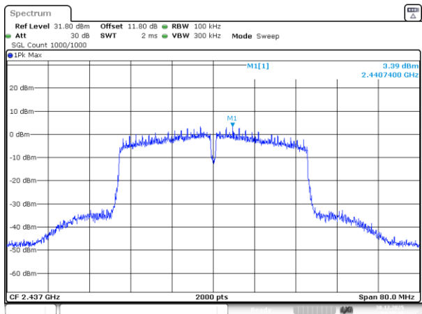
802.11n40_2437MHz_Chain 0
