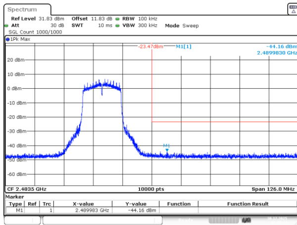
802.11g_2462MHz_Chain 0
