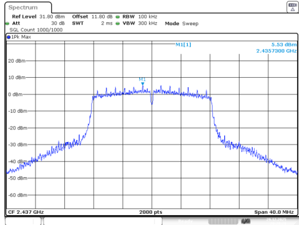
802.11g_2437MHz_Chain 3
