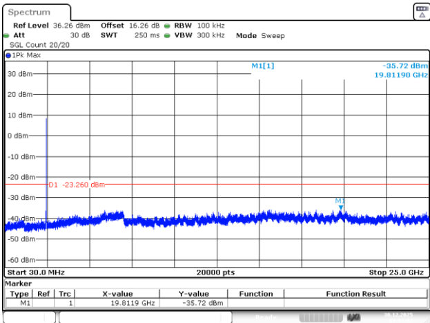
802.11g_2462MHz_Chain 1
