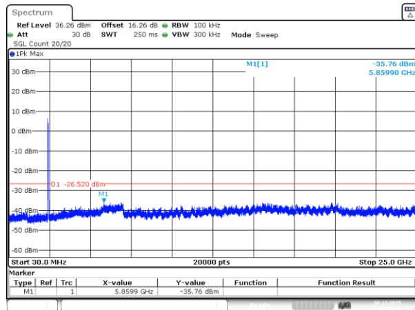
802.11n40_2422MHz_Chain 1
