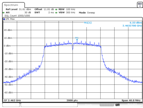
802.11g_2462MHz_Chain 0
