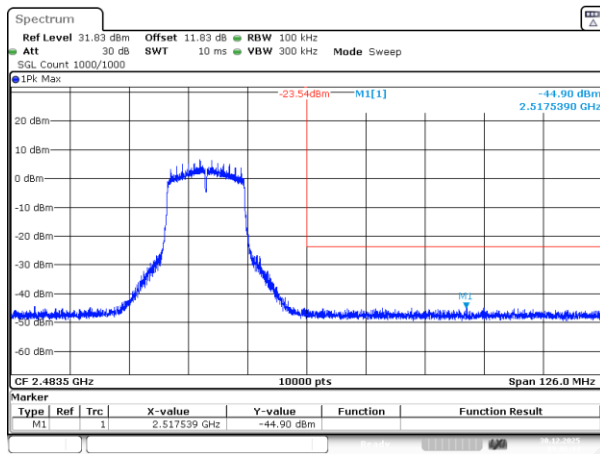
802.11g_2462MHz_Chain 3
