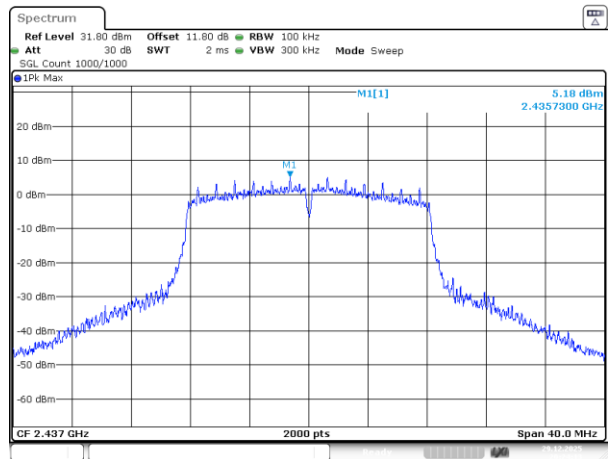
802.11g_2437MHz_Chain 2
