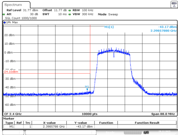
802.11g_2412MHz_Chain 0
