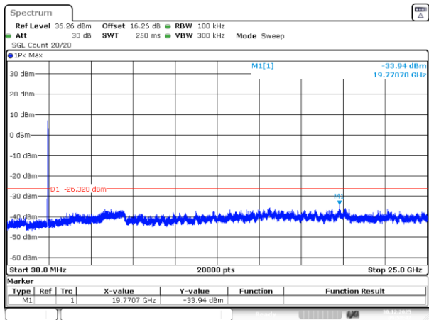
802.11n40_2437MHz_Chain 1
