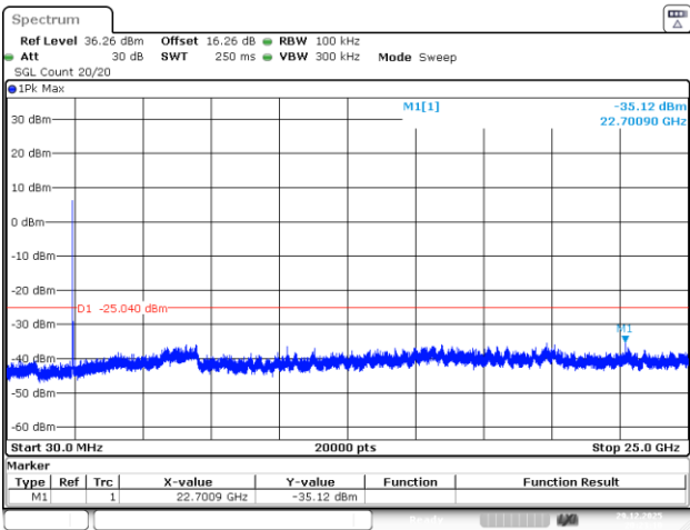
802.11g_2437MHz_Chain 1
