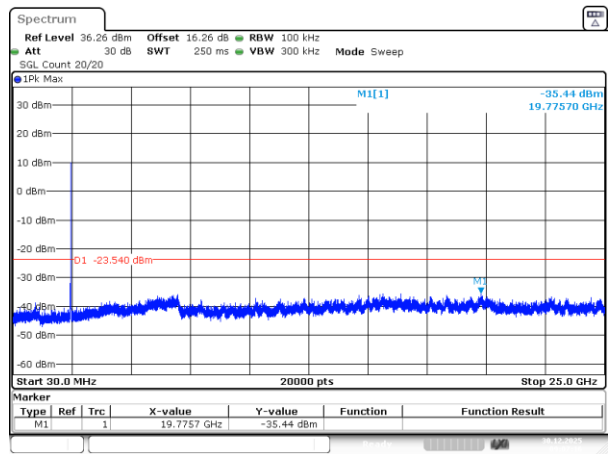
802.11g_2462MHz_Chain 3
