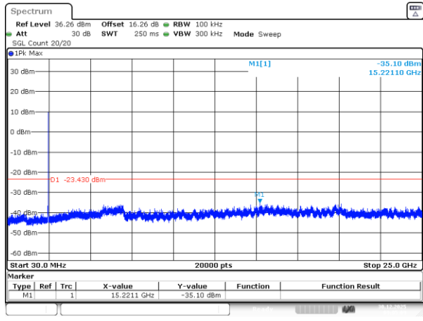
802.11g_2462MHz_Chain 2
