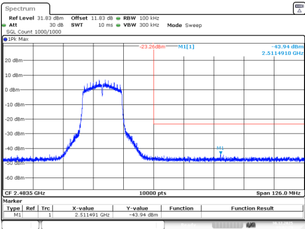
802.11g_2462MHz_Chain 1
