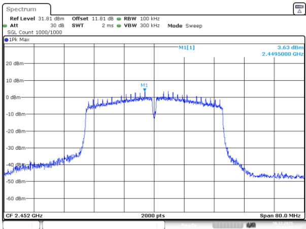
802.11n40_2452MHz_Chain 1
