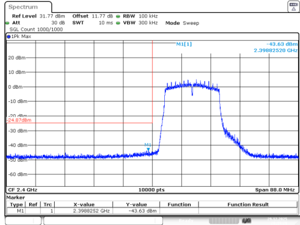
802.11g_2412MHz_Chain 3
