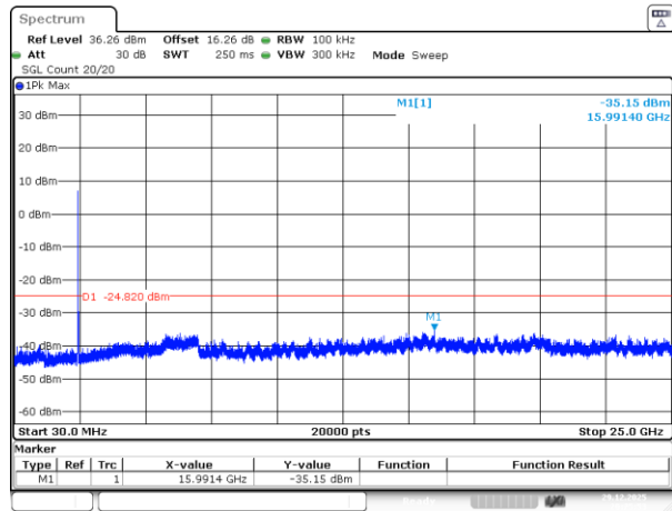
802.11g_2437MHz_Chain 2
