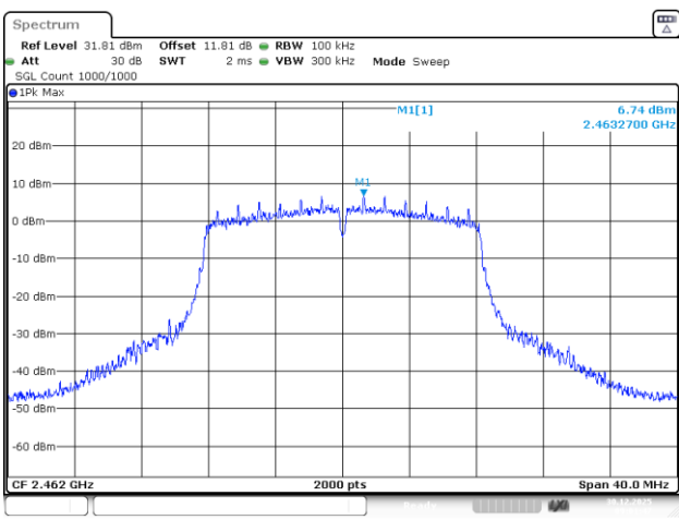
802.11g_2462MHz_Chain 1
