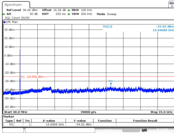
802.11g_2437MHz_Chain 0
