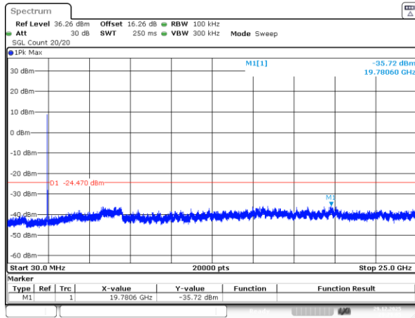
802.11g_2437MHz_Chain 3
