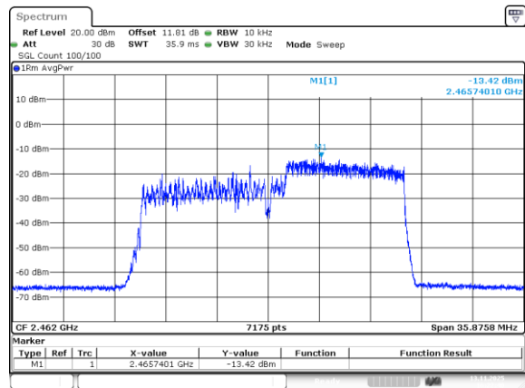
802.11be20_2462MHz_RU_106/54_Chain 2
