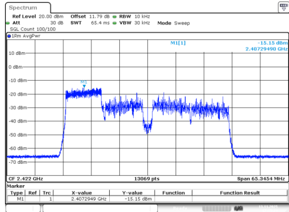
802.11be40_2422MHz_RU_106/53_Chain 1
