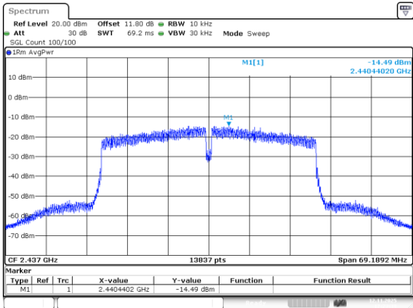
802.11n40_2437MHz_Chain 0
