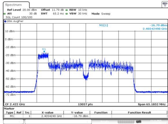
802.11be40_2422MHz_RU_52/37_Chain 2
