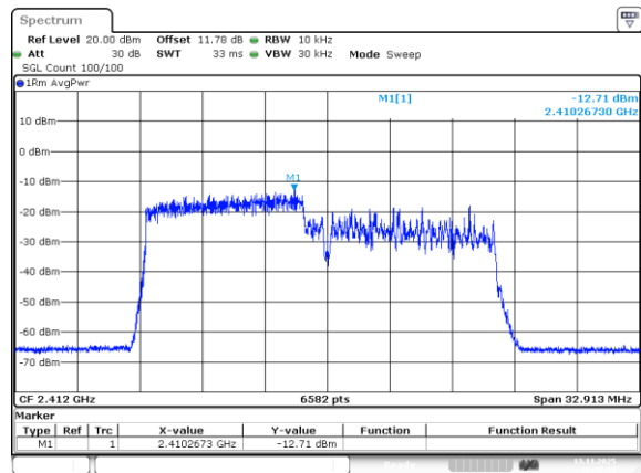
802.11be20_2412MHz_RU_106/53_Chain 1
