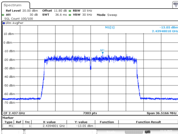
802.11be20_2437MHz_RU_242/61_Chain 0
