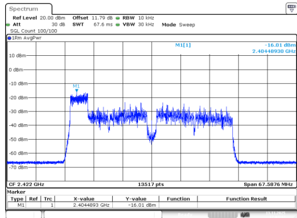
802.11be40_2422MHz_RU_52/37_Chain 3
