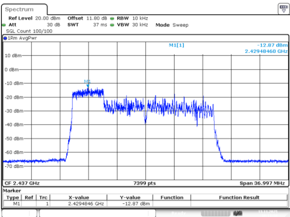
802.11be20_2437MHz_RU_52/37_Chain 1
