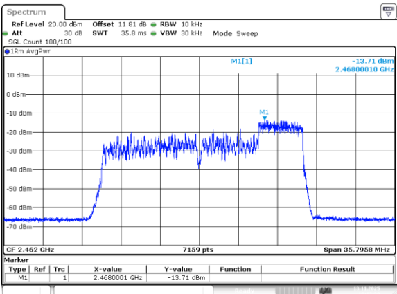
802.11be20_2462MHz_RU_52/40_Chain 1
