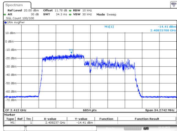
802.11be20_2412MHz_RU_106/53_Chain 2
