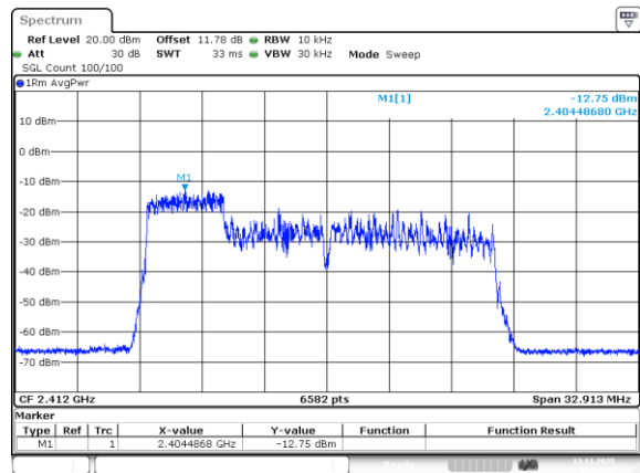
802.11be20_2412MHz_RU_52/37_Chain 1
