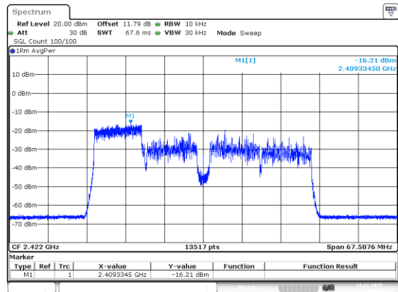
802.11be40_2422MHz_RU_106/53_Chain 3
