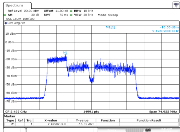
802.11be40_2437MHz_RU_106/53_Chain 3
