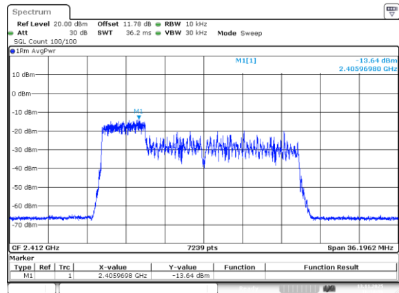
802.11be20_2412MHz_RU_52/37_Chain 3
