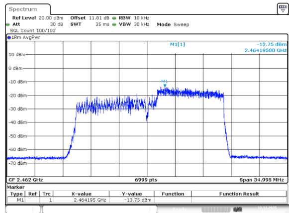
802.11be20_2462MHz_RU_106/54_Chain 3
