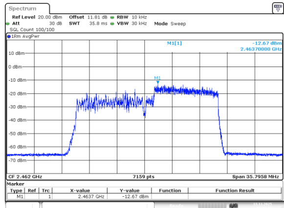
802.11be20_2462MHz_RU_106/54_Chain 1
