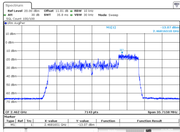
802.11be20_2462MHz_RU_52/40_Chain 0
