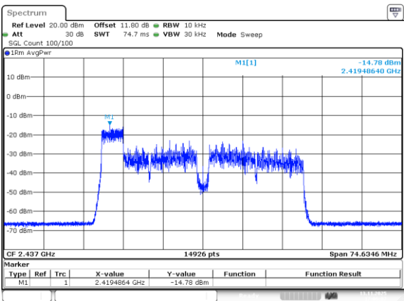
802.11be40_2437MHz_RU_52/37_Chain 1
