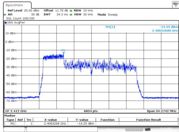
802.11be20_2412MHz_RU_52/37_Chain 2
