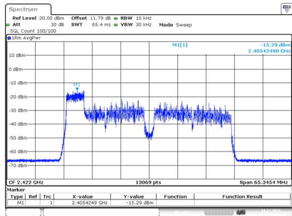
802.11be40_2422MHz_RU_52/37_Chain 1
