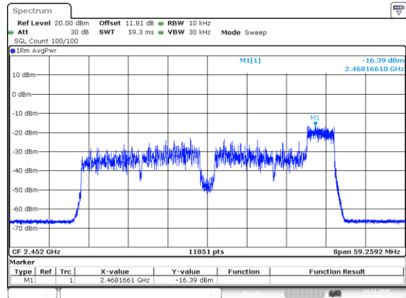
802.11be40_2452MHz_RU_52/44_Chain 0
