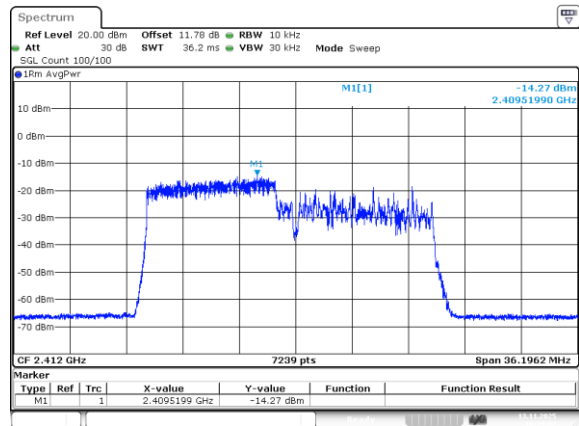
802.11be20_2412MHz_RU_106/53_Chain 3
