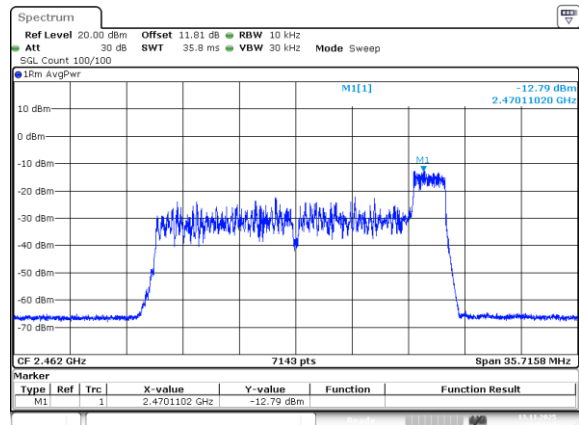
802.11be20_2462MHz_RU_26/8_Chain 0
