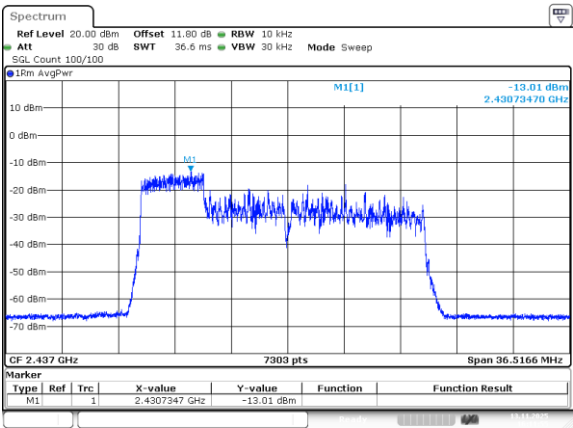
802.11be20_2437MHz_RU_52/37_Chain 2
