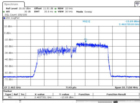
802.11be20_2462MHz_RU_106/54_Chain 0
