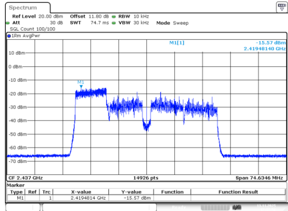
802.11be40_2437MHz_RU_106/53_Chain 1
