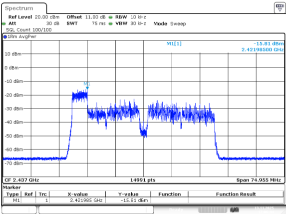
802.11be40_2437MHz_RU_52/37_Chain 2
