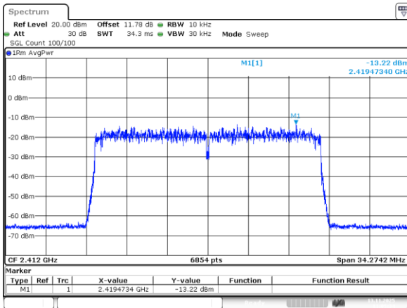
802.11be20_2412MHz_RU_242/61_Chain 0
