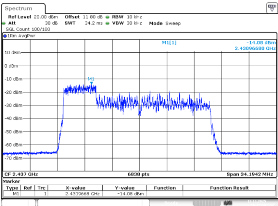
802.11be20_2437MHz_RU_52/37_Chain 3
