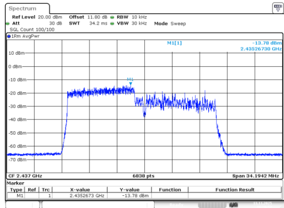
802.11be20_2437MHz_RU_106/53_Chain 3
