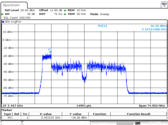
802.11be40_2437MHz_RU_52/37_Chain 3
