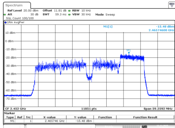
802.11be40_2452MHz_RU_106/56_Chain 0
