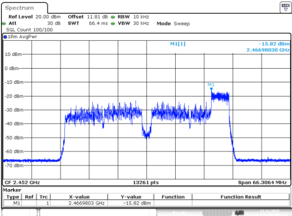
802.11be40_2452MHz_RU_52/44_Chain 1
