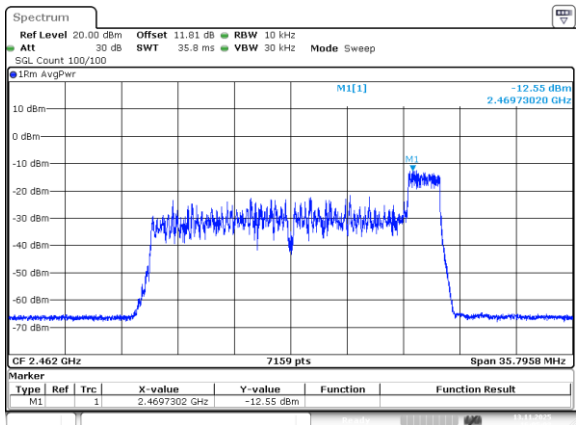
802.11be20_2462MHz_RU_26/8_Chain 1
