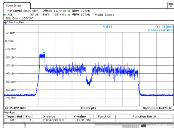
802.11be40_2422MHz_RU_26/0_Chain 1
