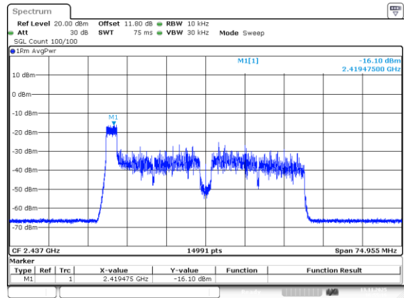
802.11be40_2437MHz_RU_26/0_Chain 2
