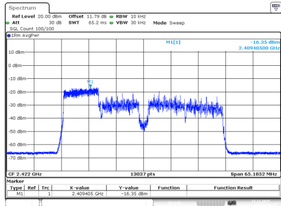
802.11be40_2422MHz_RU_106/53_Chain 2
