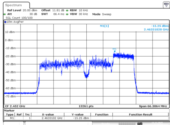
802.11be40_2452MHz_RU_106/56_Chain 1
