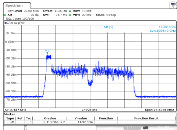
802.11be40_2437MHz_RU_26/0_Chain 1
