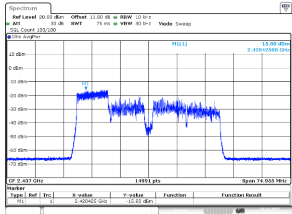
802.11be40_2437MHz_RU_106/53_Chain 2
