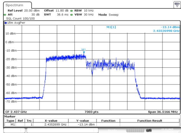
802.11be20_2437MHz_RU_106/53_Chain 2
