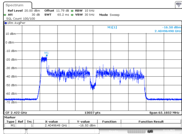
802.11be40_2422MHz_RU_26/0_Chain 2
