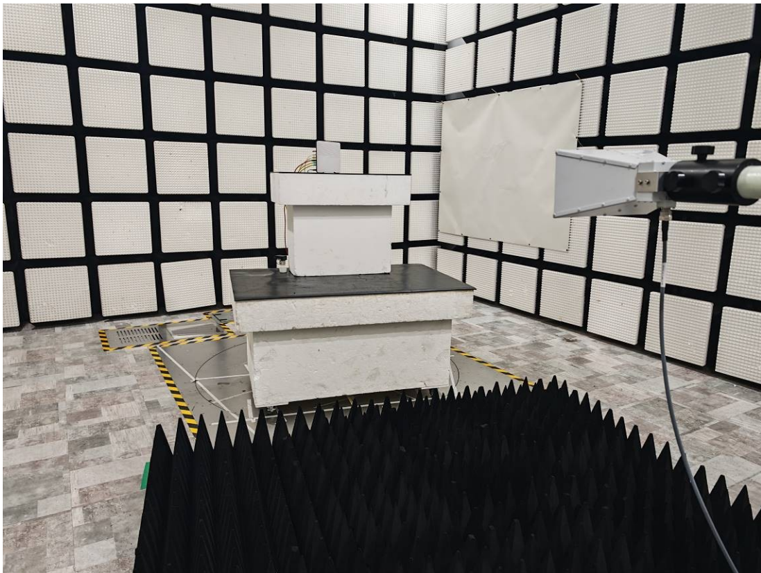
Radiated Emission 18-40GHz View
