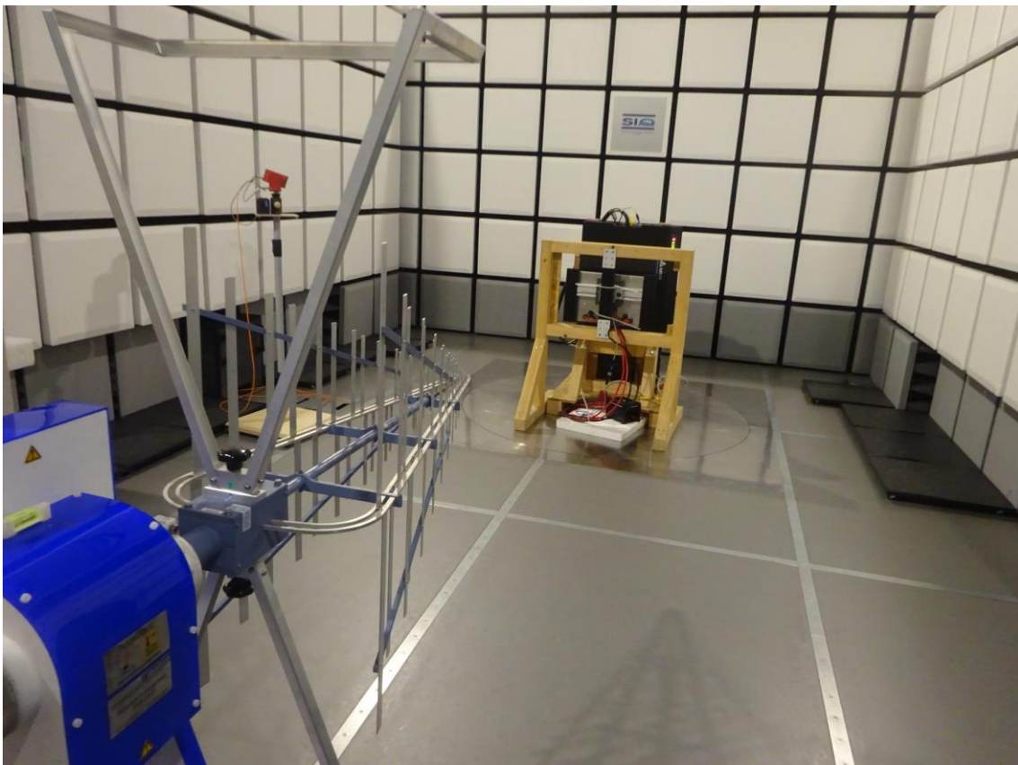
Figure 8: Radiated emissions from 30 MHz – 1000 MHz Portrait mode
