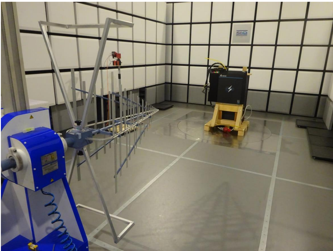
Figure 4: Radiated emissions from 30 MHz – 1000 MHz Landscape mode
