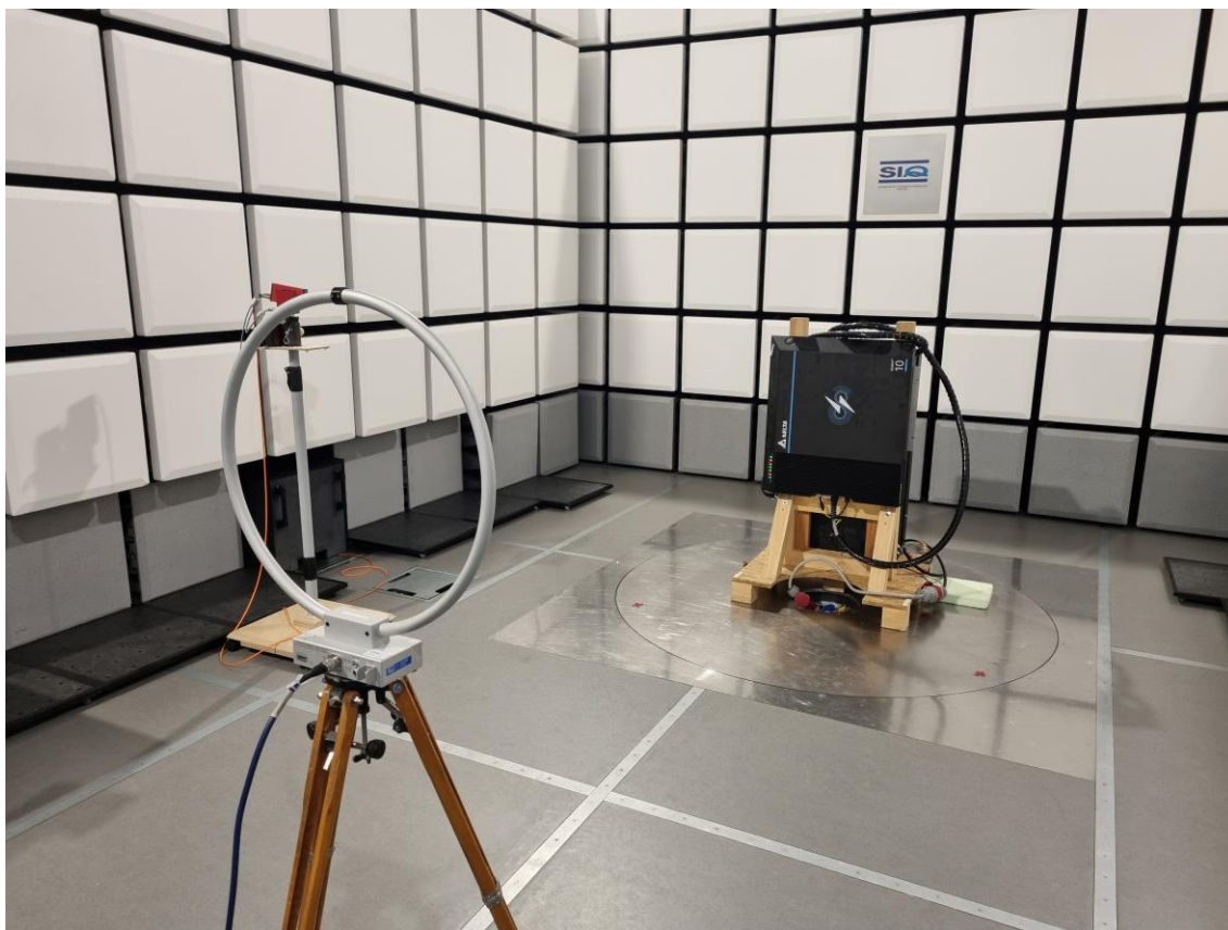
Figure 6: Radiated emissions from 9 kHz – 30 MHz Portrait mode
