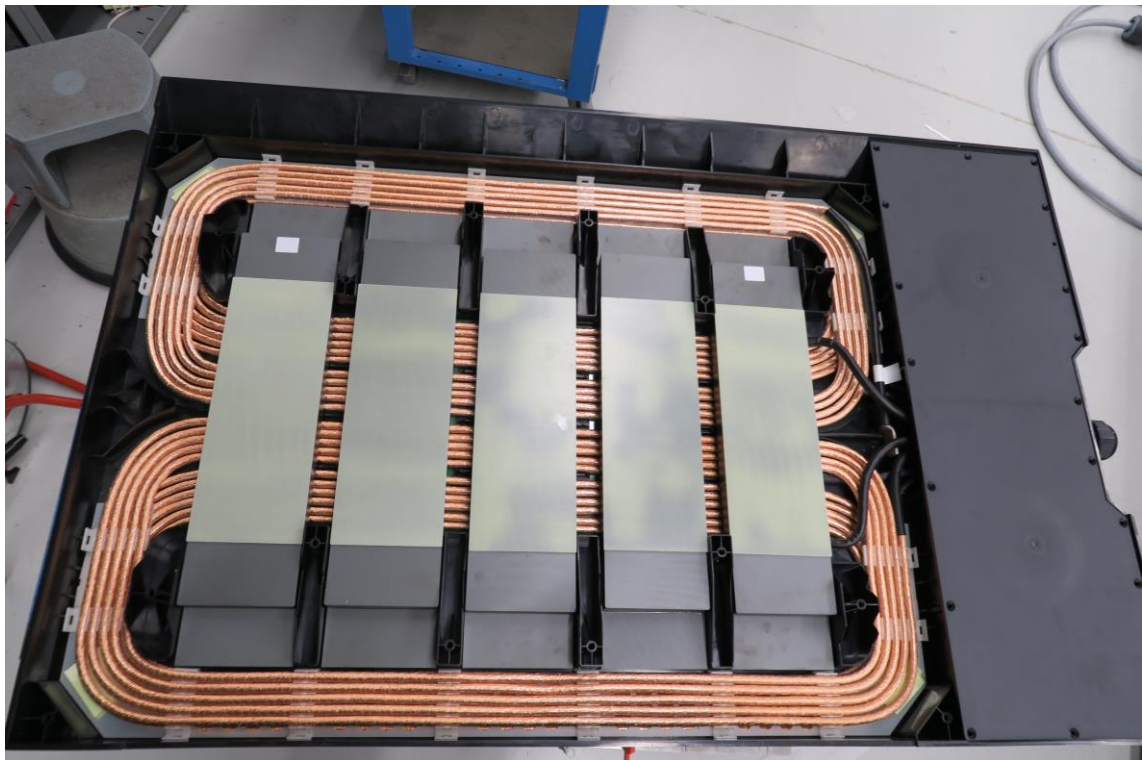
Figure 4: Primary Pad
