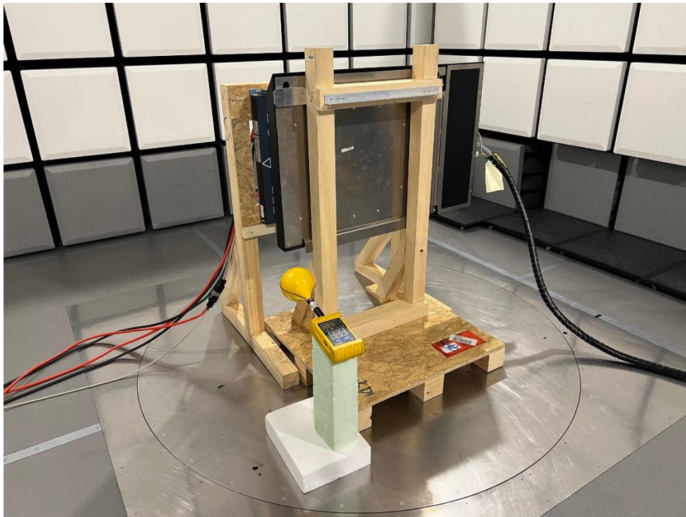
Back of WPP at 260 mm distance
