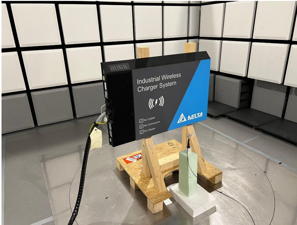
Front of WPP at 200 mm distance
