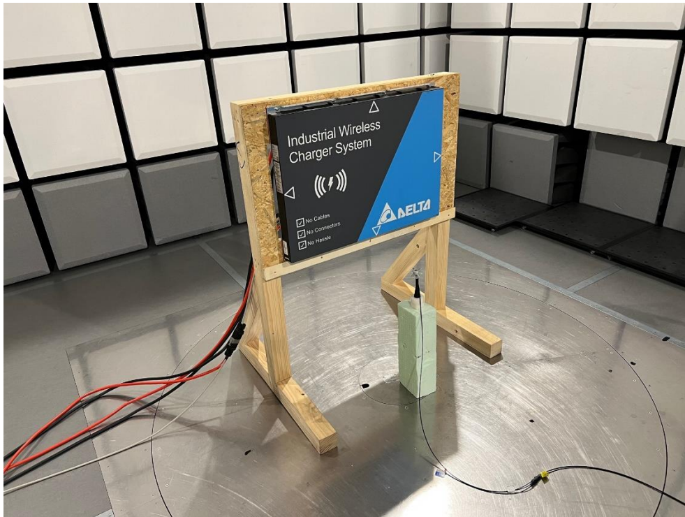
Front of WSU at 200 mm distance
