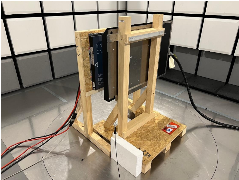
Below WPP at 347 mm distance
