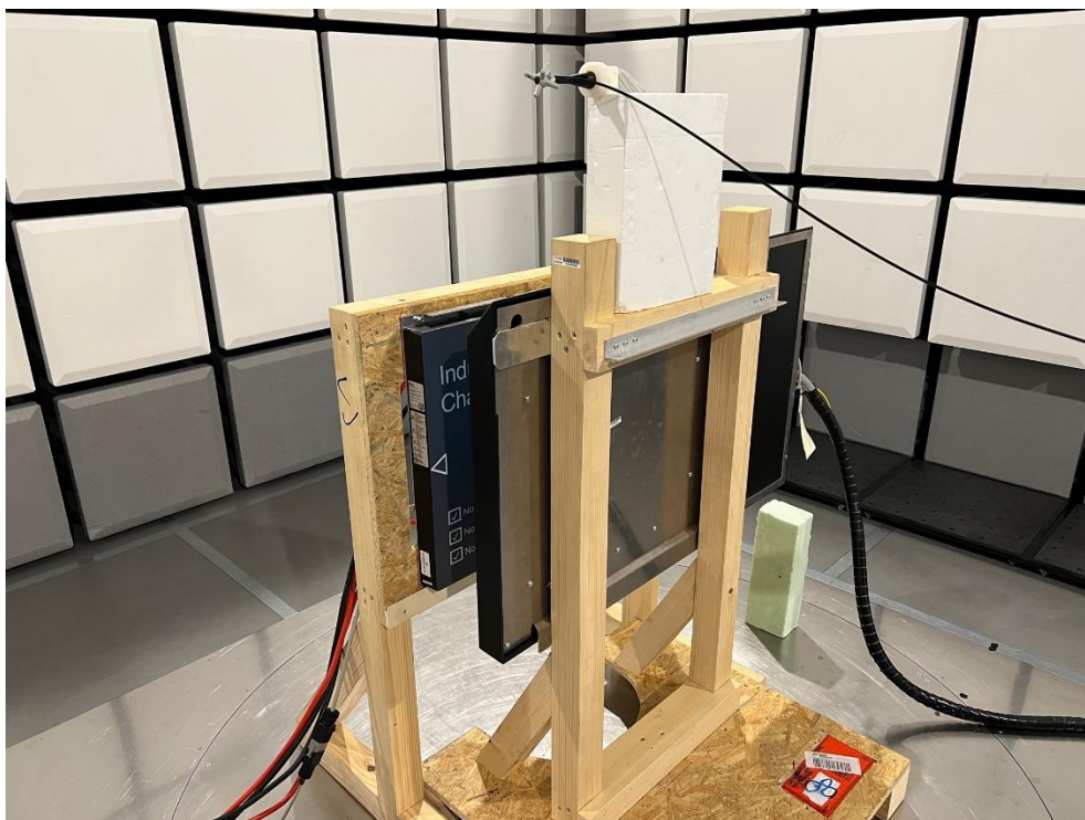
Above WPP at 347 mm distance
