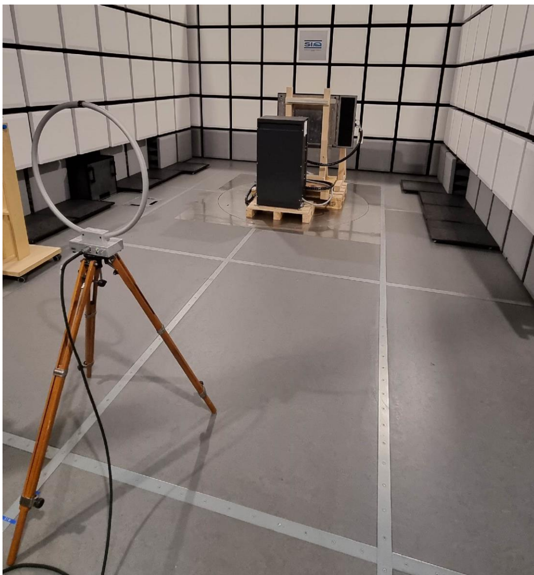
Figure 5: Radiated measurements 9 kHz-30 MHz
