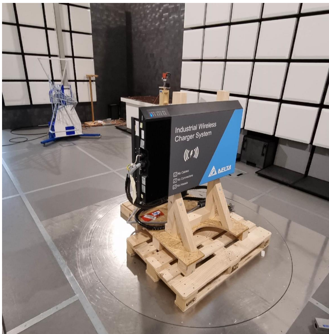
Figure 3: Radiated measurements 30 MHz-1000 MHz
