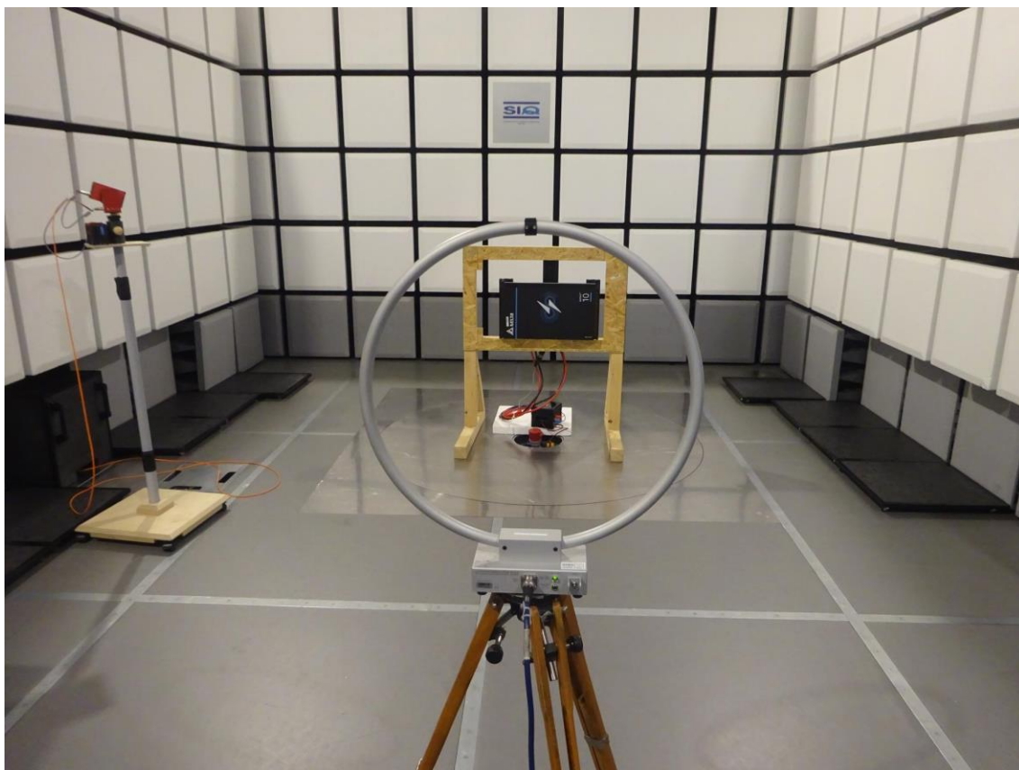
Figure 6: Radiated emissions from 30 MHz – 1000 MHz Portrait mode
