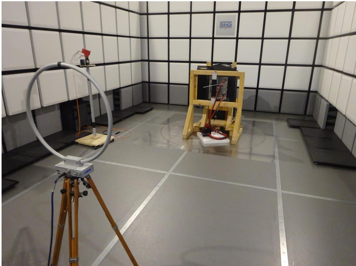
Figure 1: Radiated emissions from 9 kHz – 30 MHz Landscape mode
