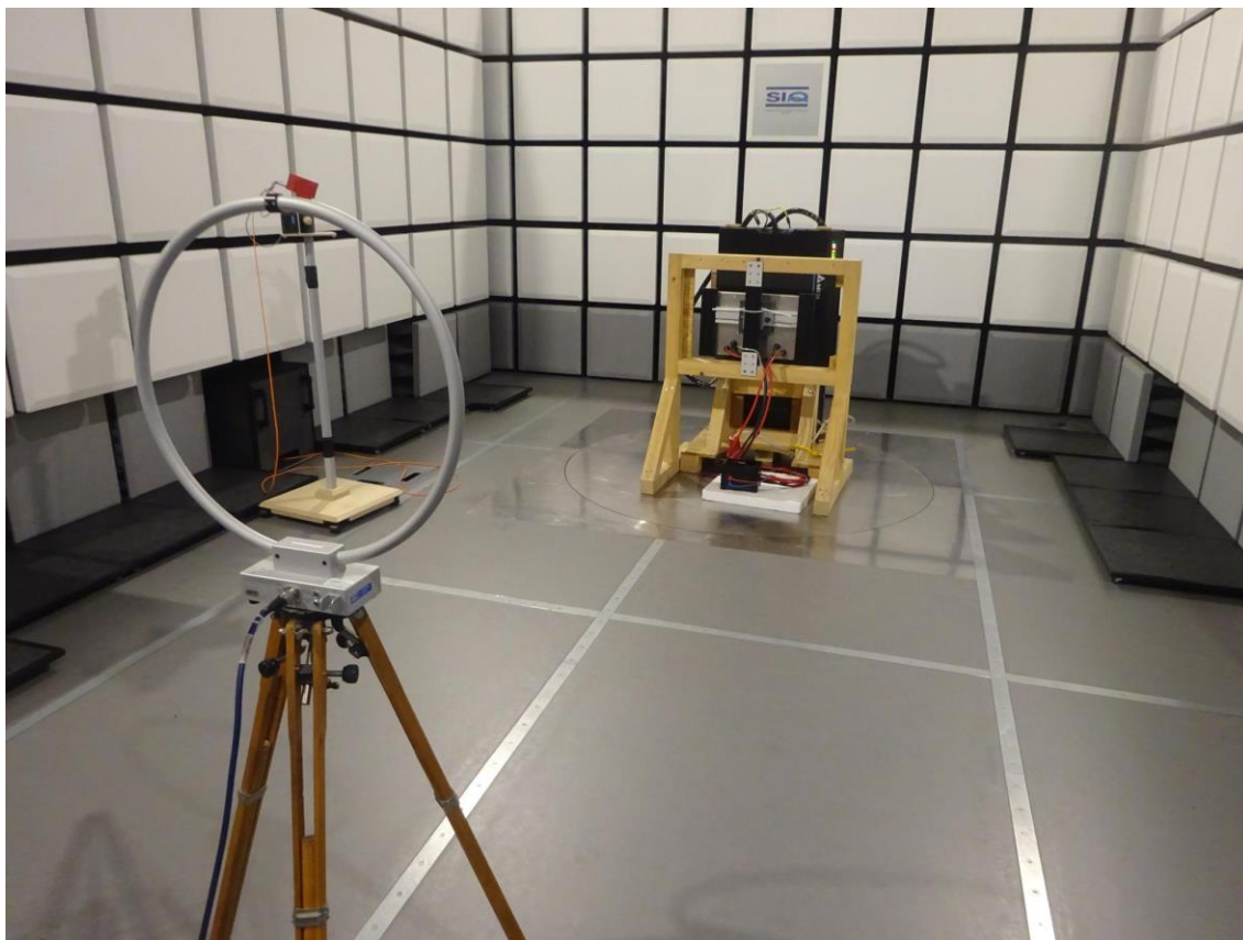
Figure 5: Radiated emissions from 9 kHz – 30 MHz Portrait mode
