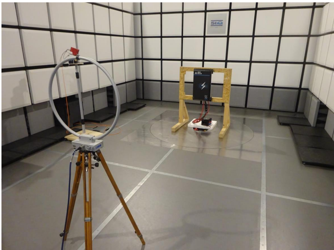
Figure 2: Radiated emissions from 9 kHz – 30 MHz Landscape mode
