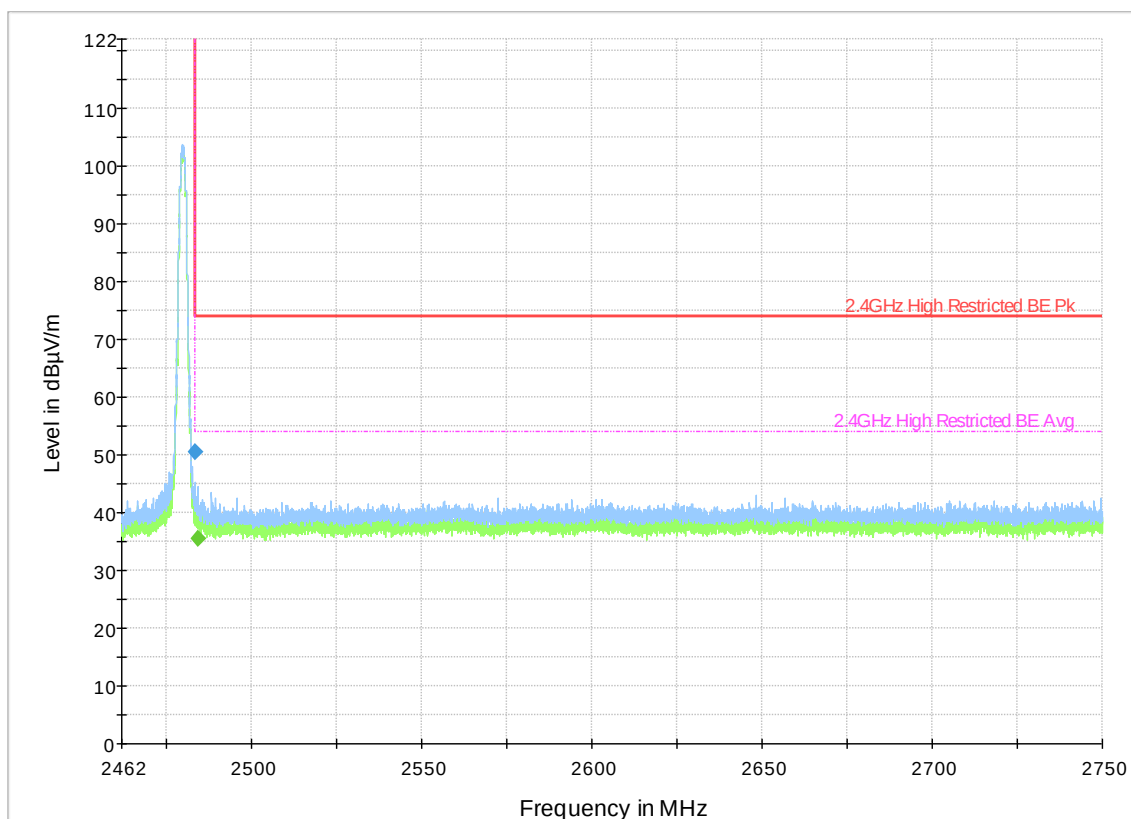
Plot 44. Upper Restricted Band Edge, 2480MHz, 3DH5
