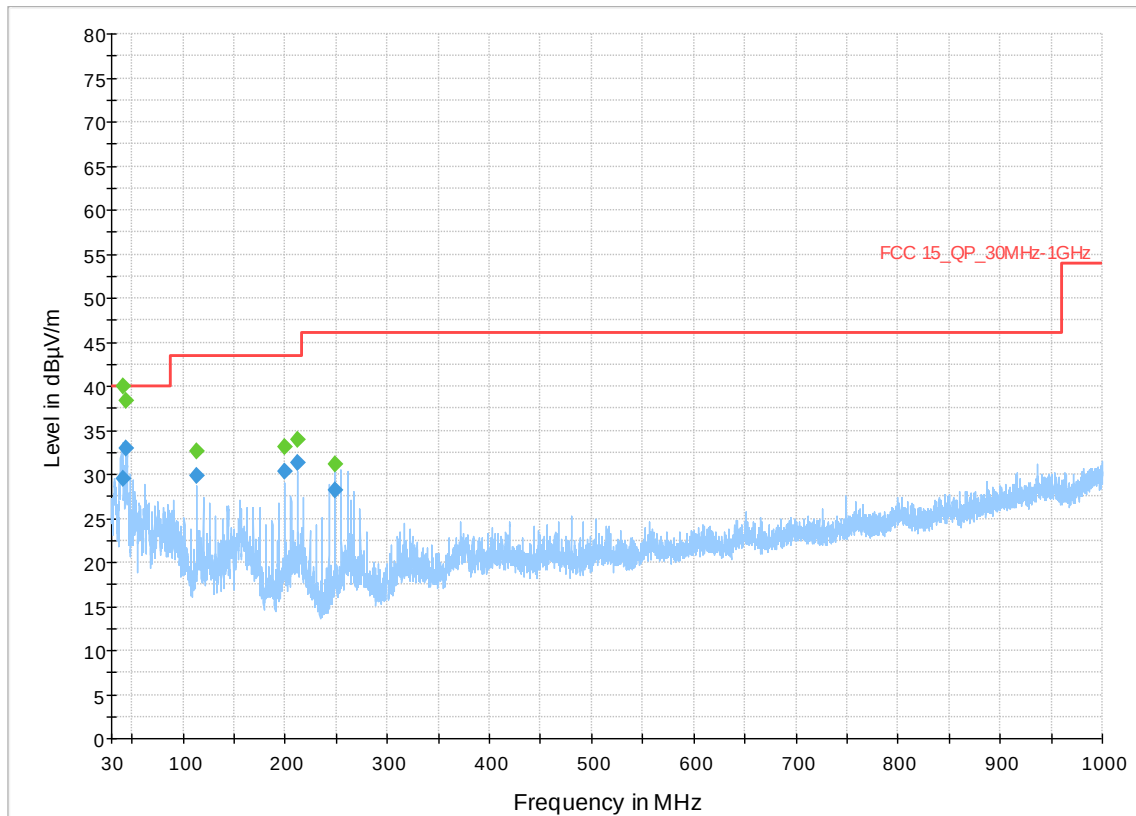
Plot 46. 30-1000MHz, 2480 MHz, DH5
