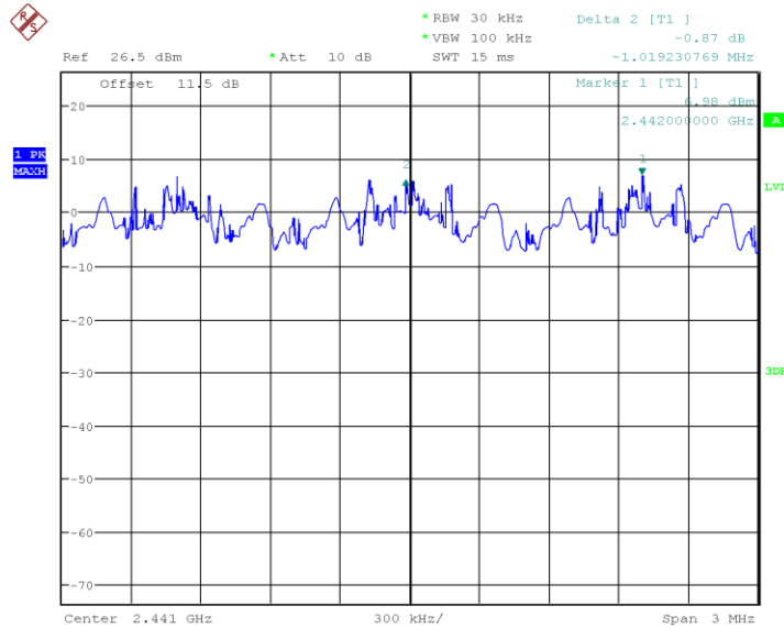
Plot 22. Hopping Separation for 2DH5
