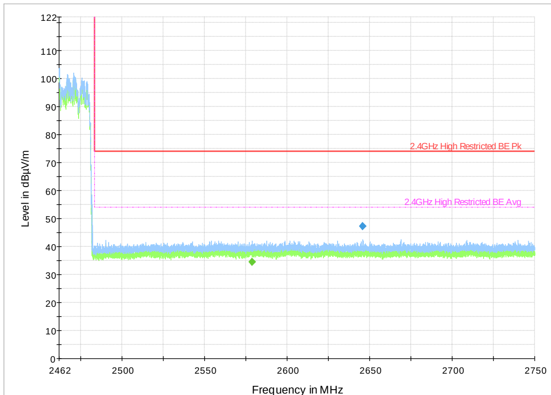
Plot 45. Upper Restricted Band Edge, 2480MHz, 3DH5, Hopping
