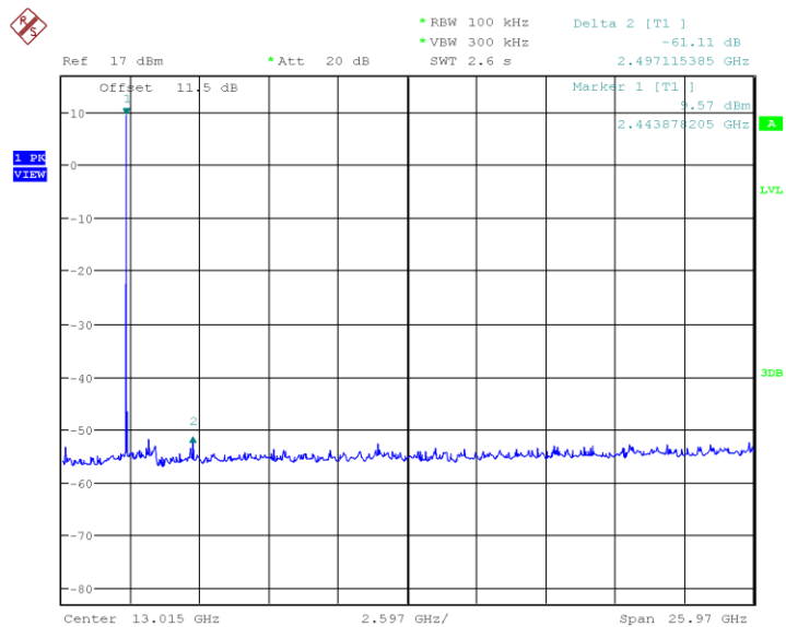
Plot 34. DH5 2441MHz, 30MHz-26.5GHz Spurious
