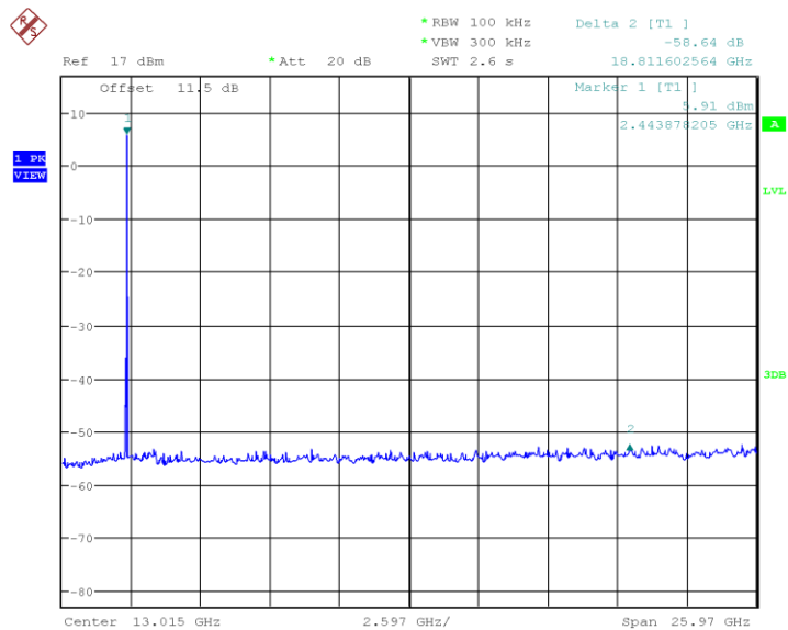
Plot 36. 2DH5 2402MHz, 30MHz-26.5GHz Spurious
