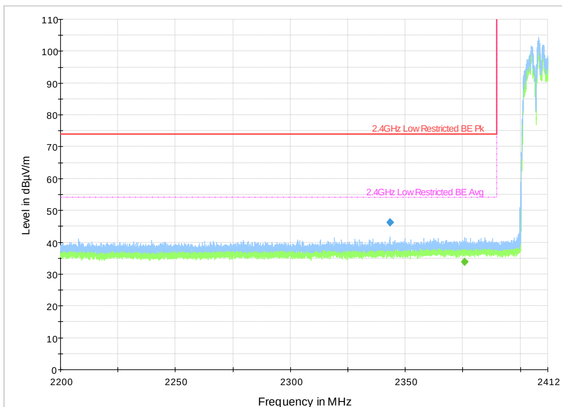
Plot 43. Lower Restricted Band Edge, 2402MHz, 3DH5, Hopping
