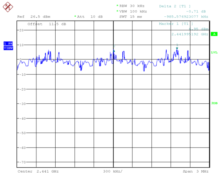
Plot 21. Hopping Separation for DH5
