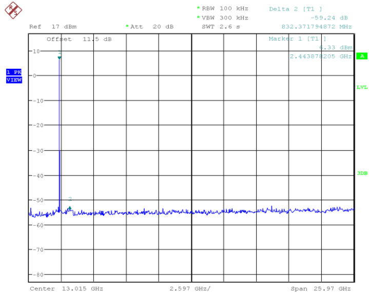
Plot 40. 3DH5 2441MHz, 30MHz-26.5GHz Spurious
