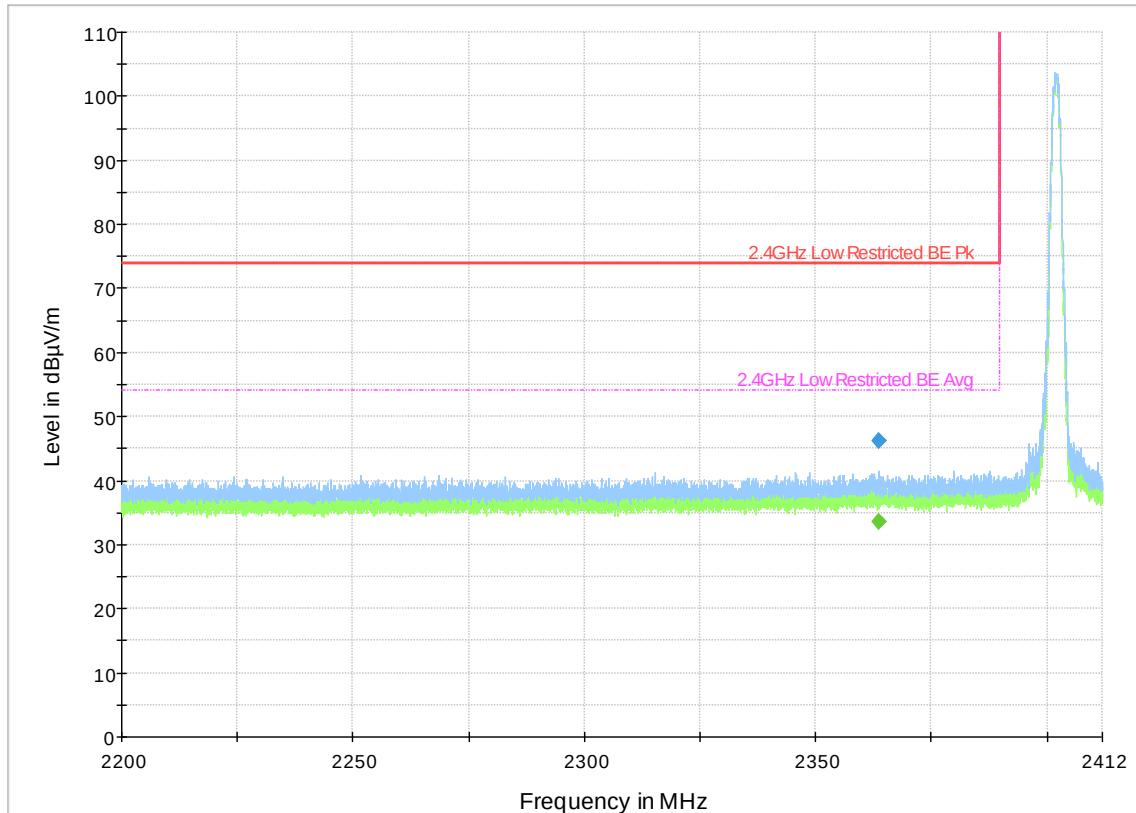
Plot 42. Lower Restricted Band Edge, 2402MHz, 3DH5
