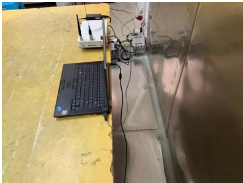
Conducted Emissions (Side View)
