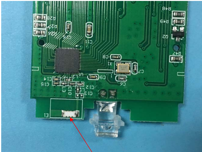
TX Antenna
