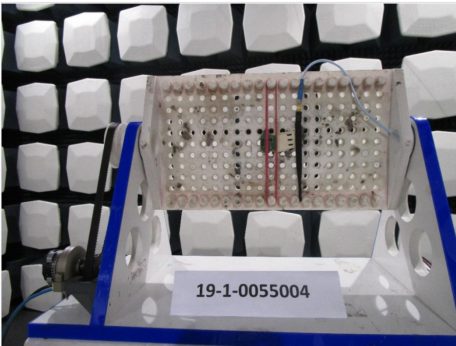
Photograph 8: EUT Setup Electrical Field Measurements in the Fully anechoic chamber
