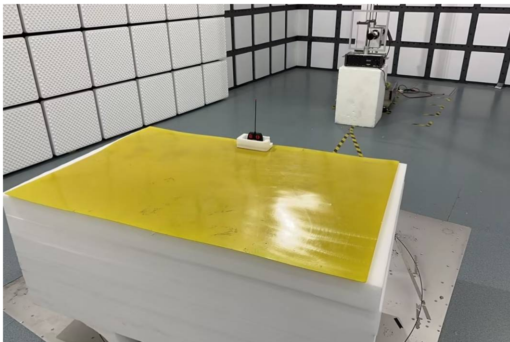
Photo of Radiated Emission Measurement (Below 30MHz)
