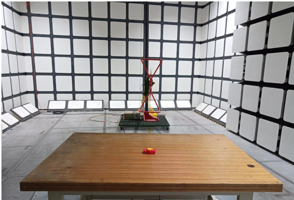
Radiated Emissions View (Below 1 GHz)
