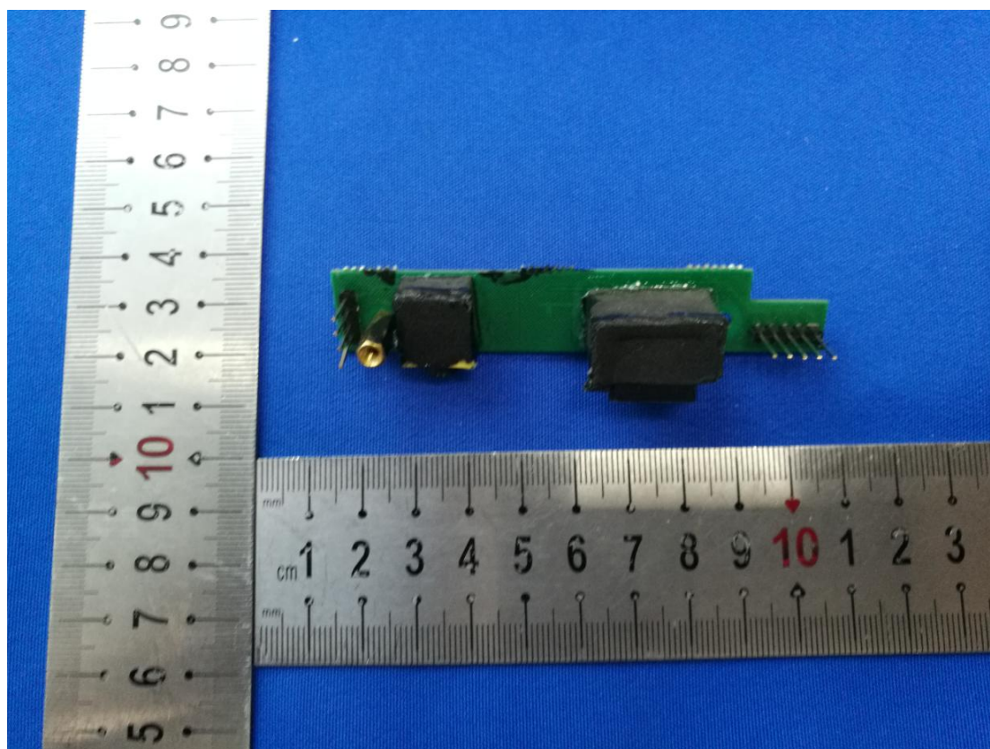
Master control module
