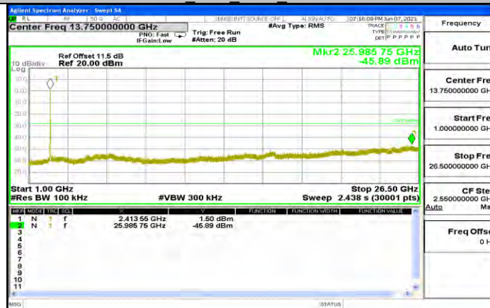
11G Ant1_2412_1000~26500
