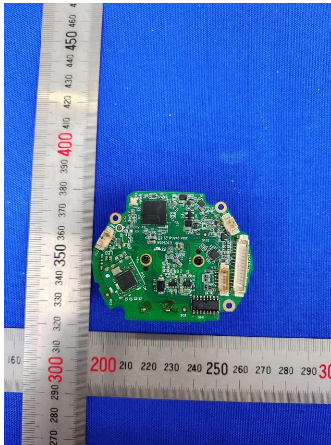
Internal View of EUT-3
