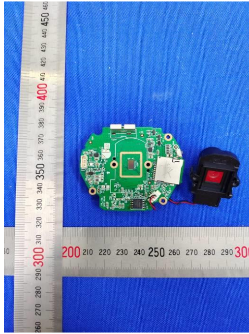
Internal View of EUT-5
