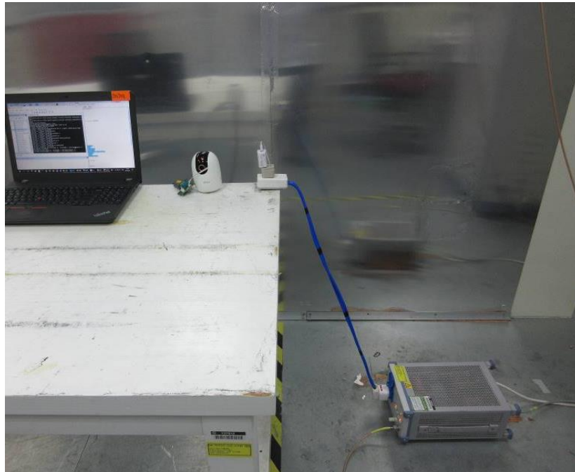
POWERLINE CONDUCTED EMISSIONS MEASUREMENT SETUP
