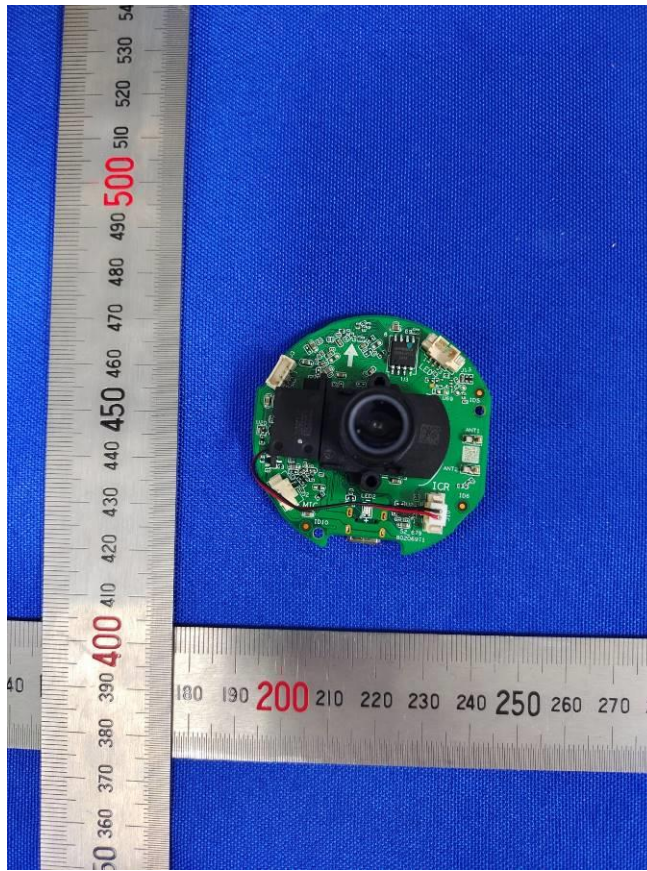
Internal View of EUT-5
