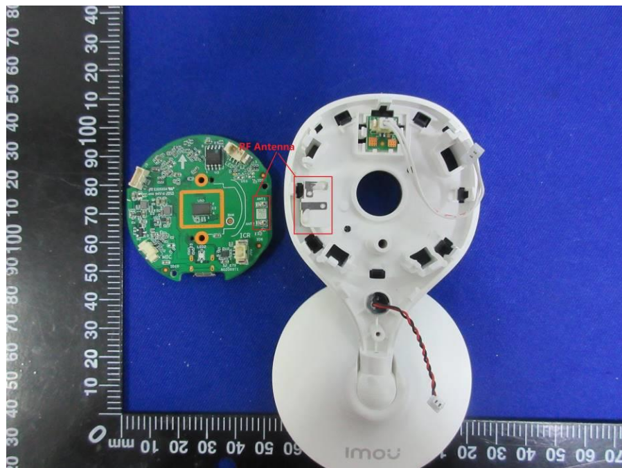
Antenna location
