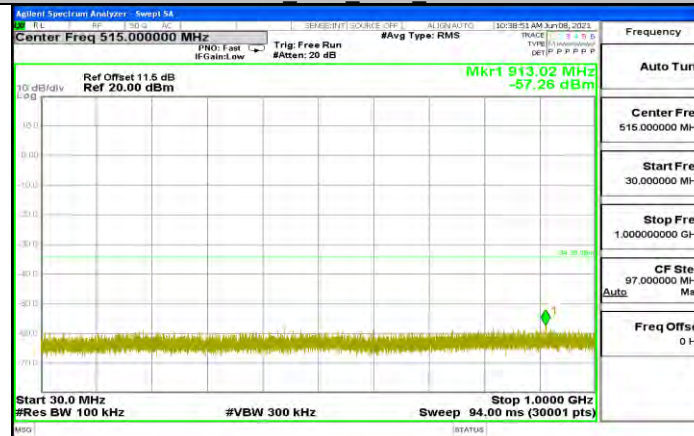
11N20SISO Ant1 2437 30~1000
