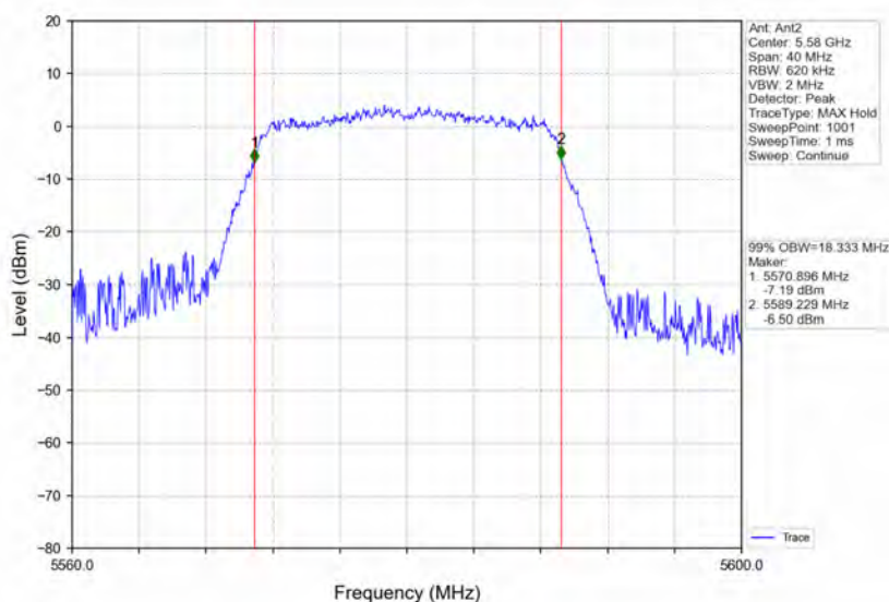
802.11ac(VHT20)_MCH_5580MHz_Ant2_NTNV
