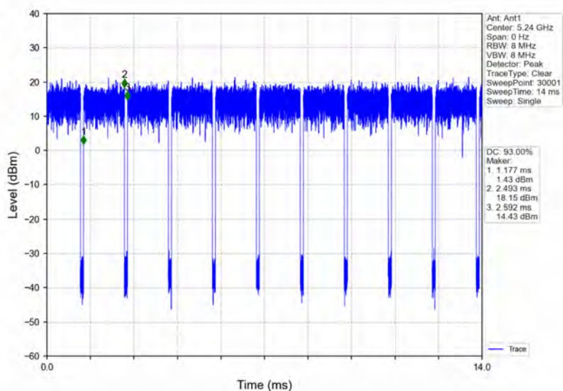
802.11ac(VHT20)_HCH_5240MHz_Ant1_NTNV
