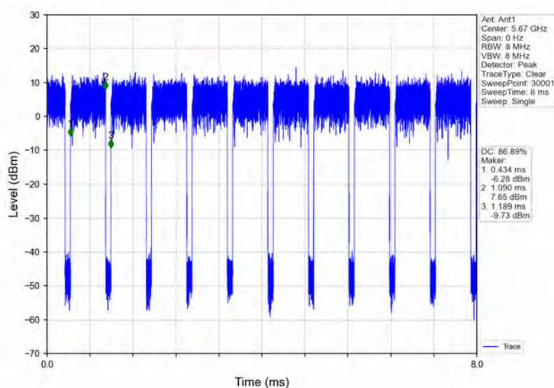
802.11ac(VHT40)_HCH_5670MHz_Ant1_NTNV
