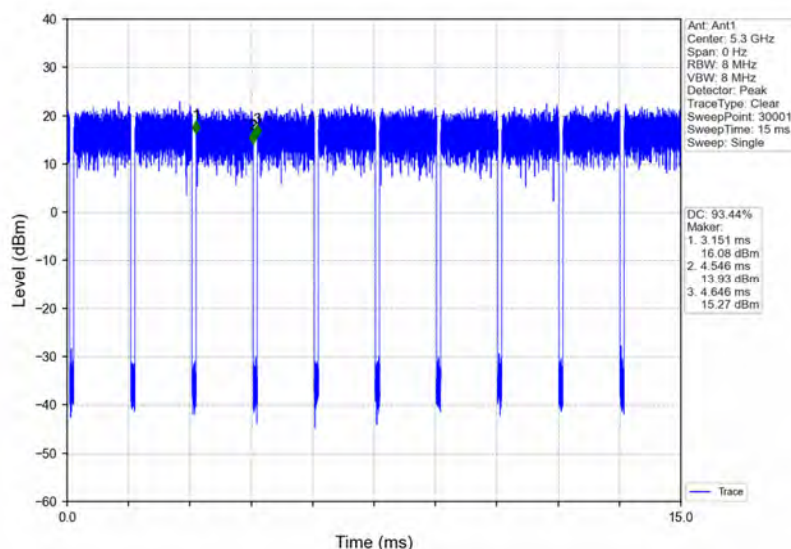
802.11a_HCH_5320MHz_Ant1_NTNV
