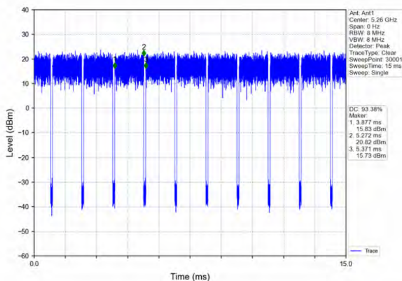
802.11a_LCH_5260MHz_Ant1_NTNV
