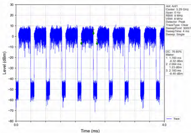
802.11ac(VHT80)_MCH_5290MHz_Ant1_NTNV
