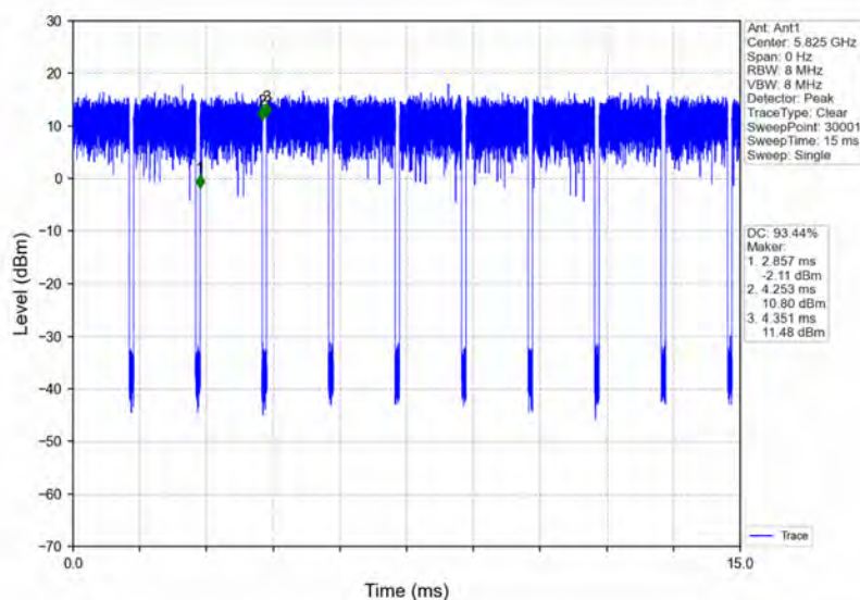
802.11a_HCH_5825MHz_Ant1_NTNV
