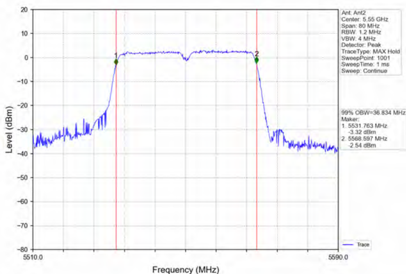
802.11ac(VHT40)_MCH_5550MHz_Ant2_NTNV
