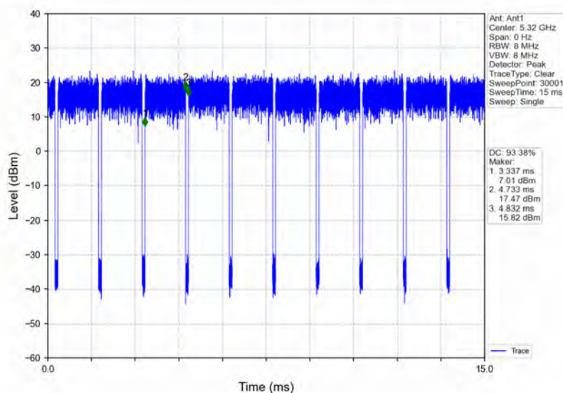
802.11a_HCH_5320MHz_Ant1_NTNV
