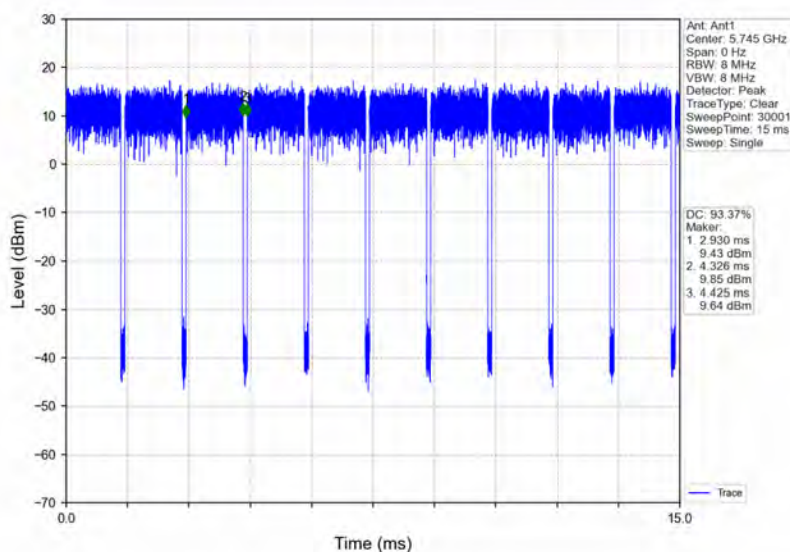
802.11a_LCH_5745MHz_Ant1_NTNV
