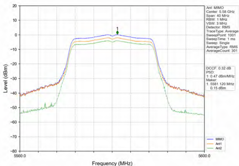
802.11ac(VHT20)_MCH_5580MHz_MIMO_NTNV
