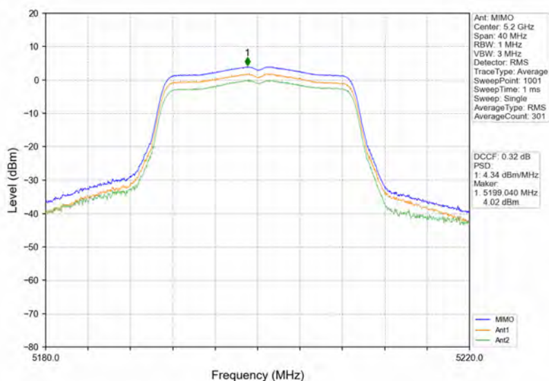
802.11ac(VHT20)_MCH_5200MHz_MIMO_NTNV
