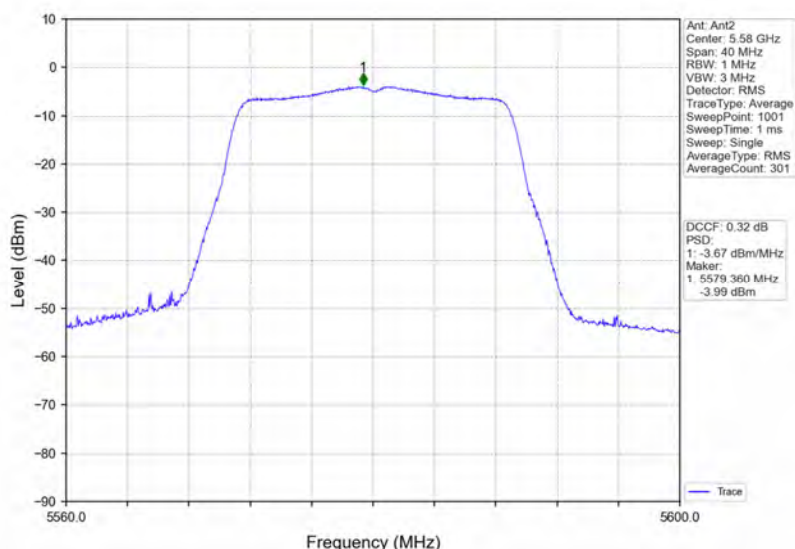
802.11ac(VHT20)_MCH_5580MHz_MIMO_NTNV
