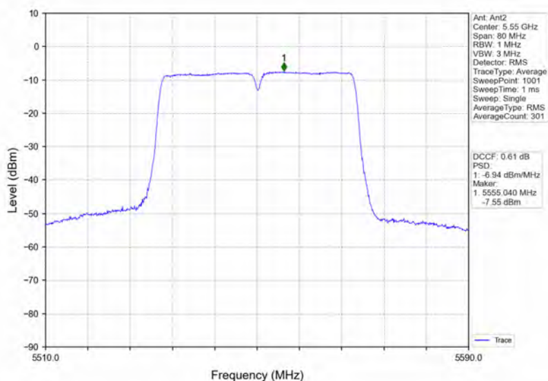
802.11ac(VHT40)_MCH_5550MHz_Ant2_NTNV
