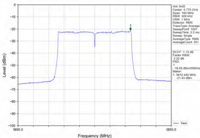
802.11ac(VHT80)_MCH_5775MHz_Ant2_NTNV
