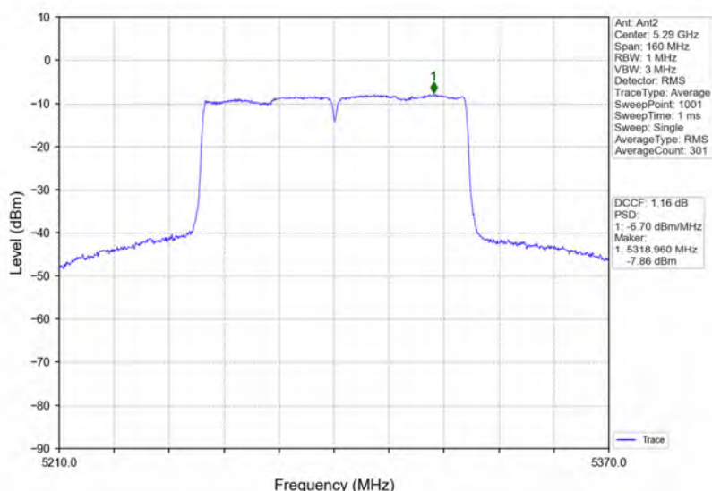
802.11ac(VHT80)_MCH_5290MHz_MIMO_NTNV
