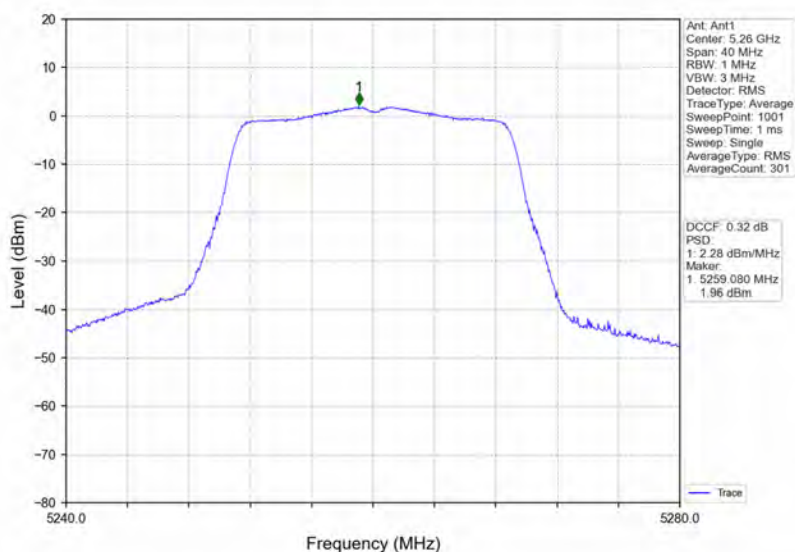
802.11ac(VHT20)_LCH_5260MHz_Ant1_NTNV
