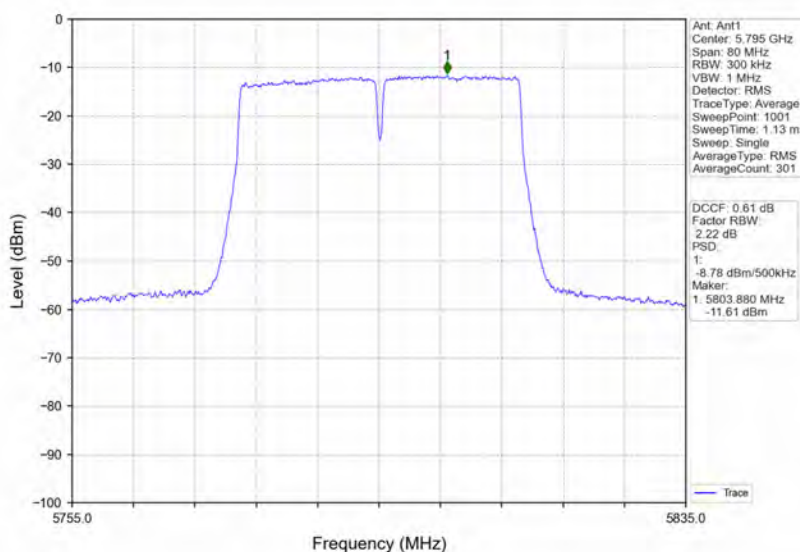
802.11ac(VHT40)_HCH_5795MHz_Ant1_NTNV
