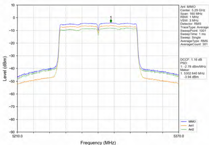
802.11ac(VHT80)_MCH_5290MHz_MIMO_NTNV
