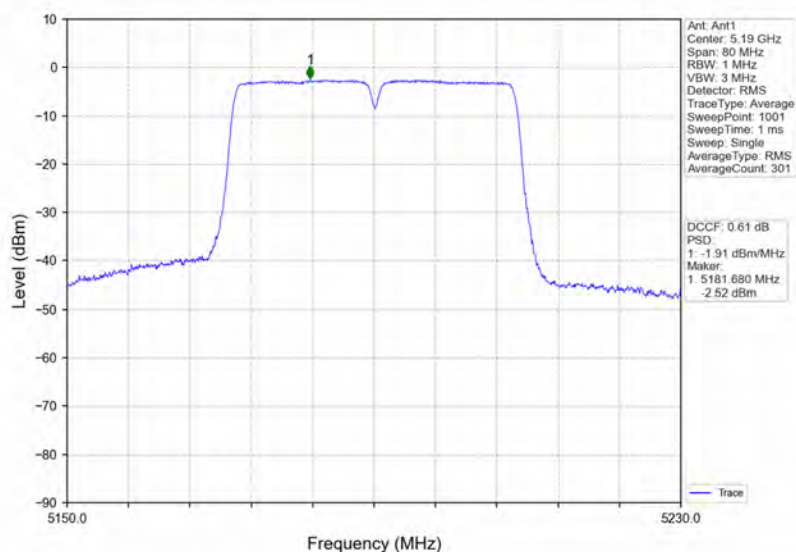
802.11ac(VHT40)_LCH_5190MHz_Ant1_NTNV
