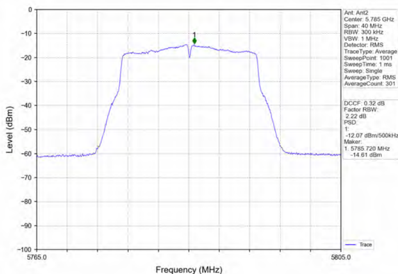
802.11ac(VHT20)_MCH_5785MHz_Ant2_NTNV
