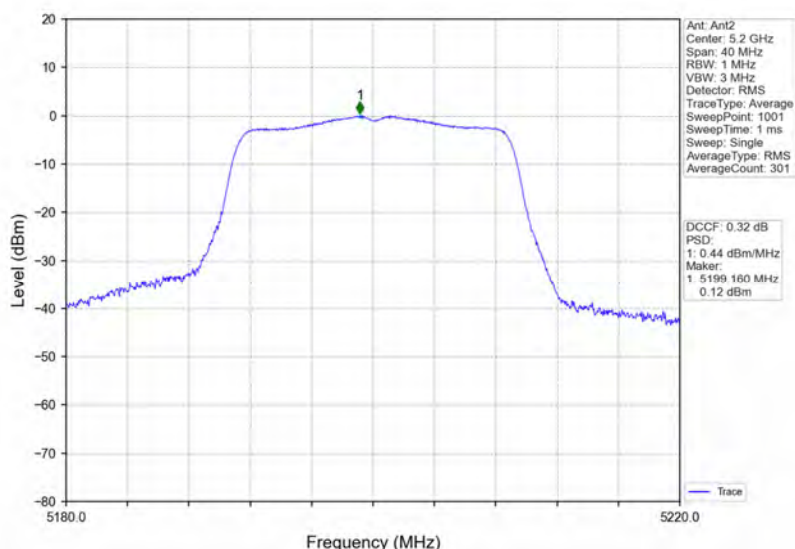
802.11ac(VHT20)_MCH_5200MHz_MIMO_NTNV
