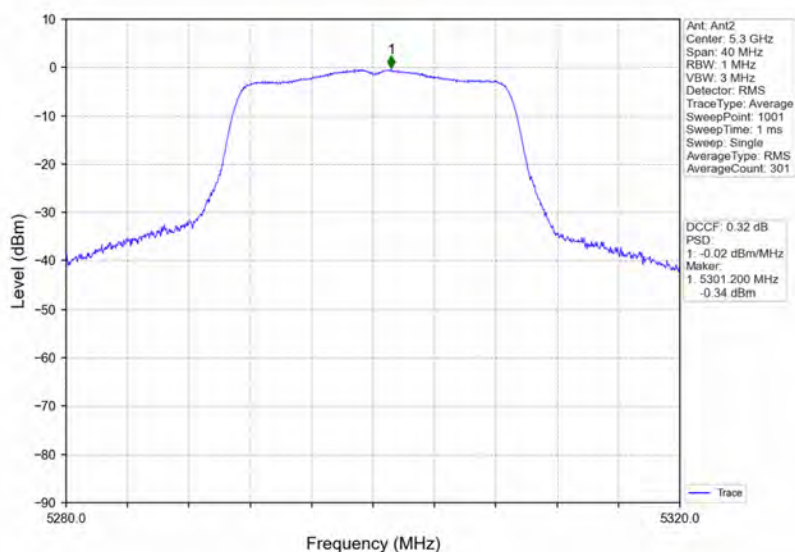
802.11ac(VHT20)_MCH_5300MHz_Ant2_NTNV
