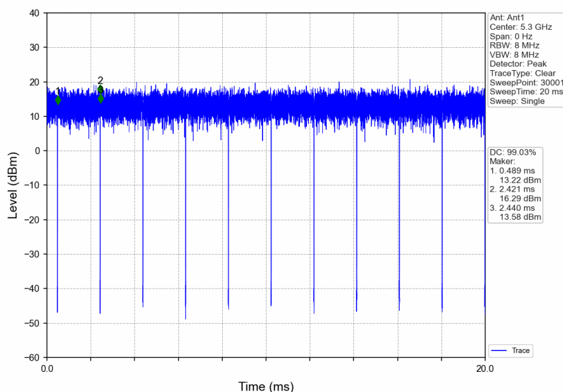
802.11ac(VHT20)_MCH_5300MHz_Ant1_NTNV
