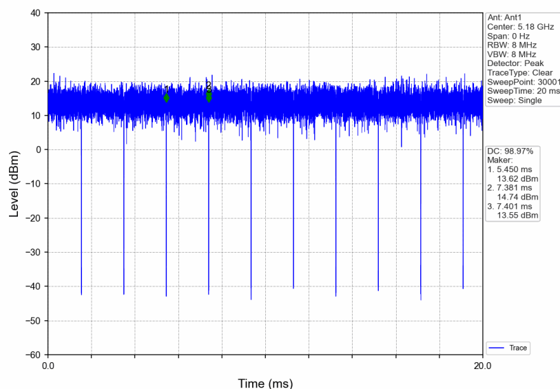
802.11ac(VHT20)_LCH_5180MHz_Ant1_NTNV
