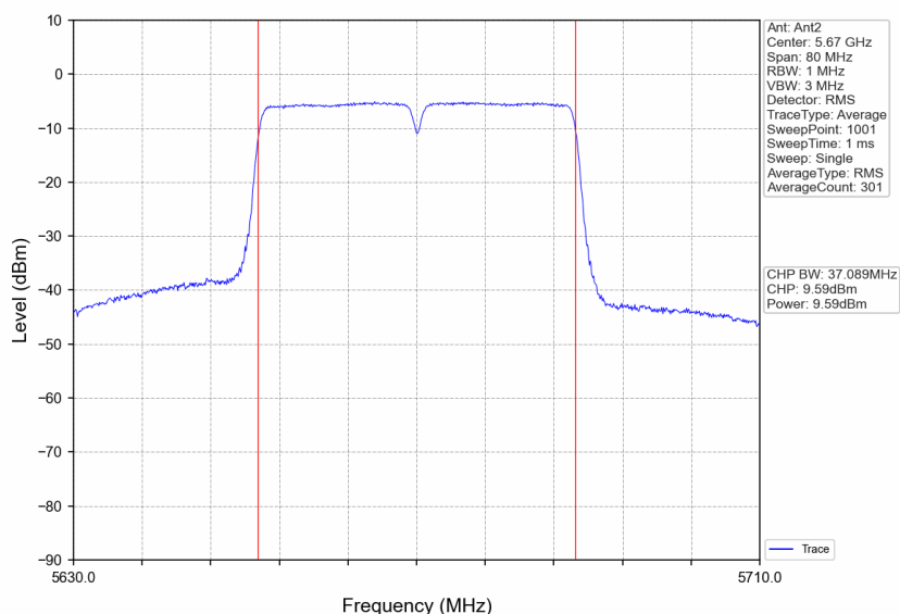
802.11ac(VHT40)_HCH_5670MHz_Ant2_NTNV
