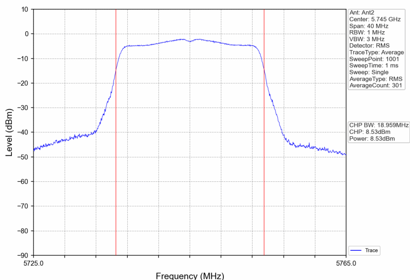
802.11ac(VHT20)_LCH_5745MHz_Ant2_NTNV
