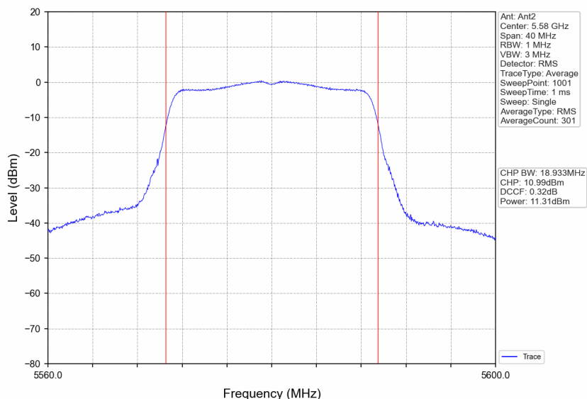
802.11n(HT20)_MCH_5580MHz_Ant2_NTNV
