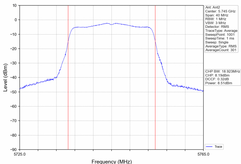
802.11n(HT20)_LCH_5745MHz_Ant2_NTNV
