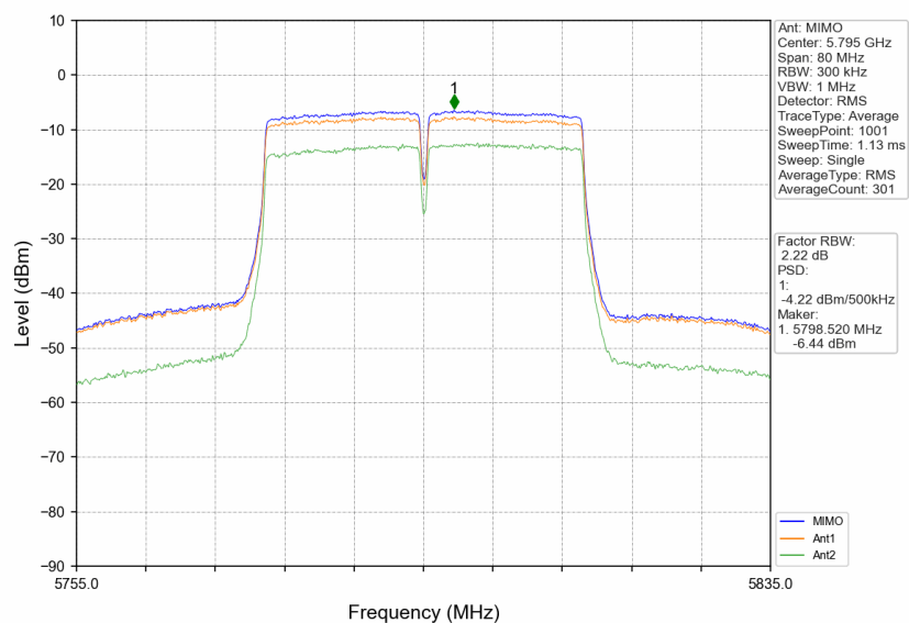
802.11ac(VHT40)_HCH_5795MHz_MIMO_NTNV
