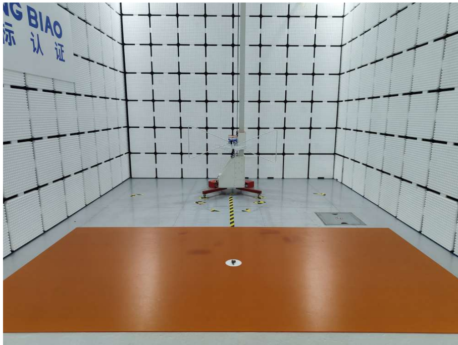
Radiated Emission Above 1GHz (Left Earphone)
