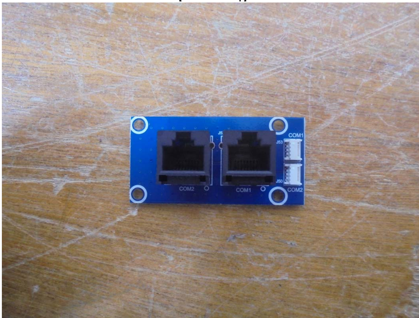
[Sub board1 Top]
