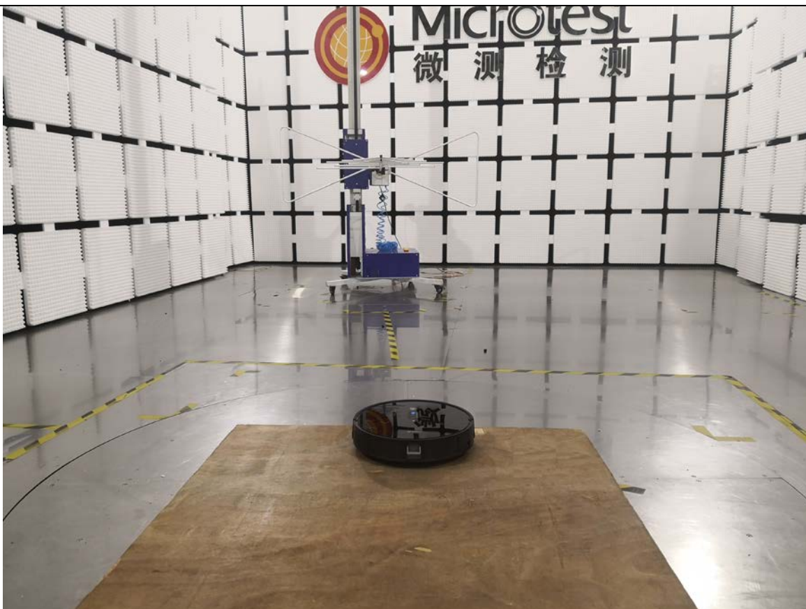
Radiated emission
