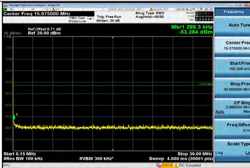
EGPRS1900-512-0.15~30
