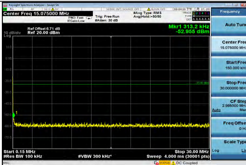
GPRS1900-512-0.15~30
