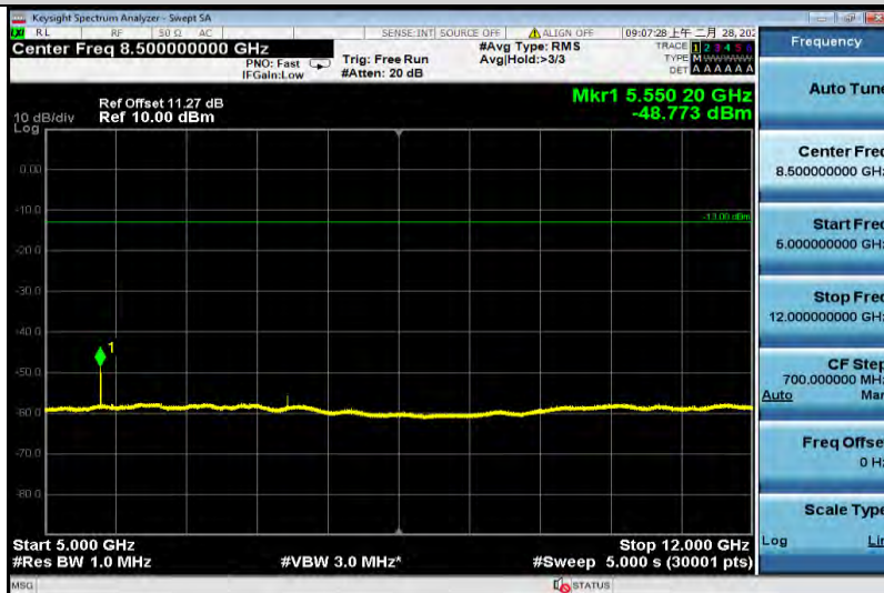
EGPRS1900-512-5000~12000
