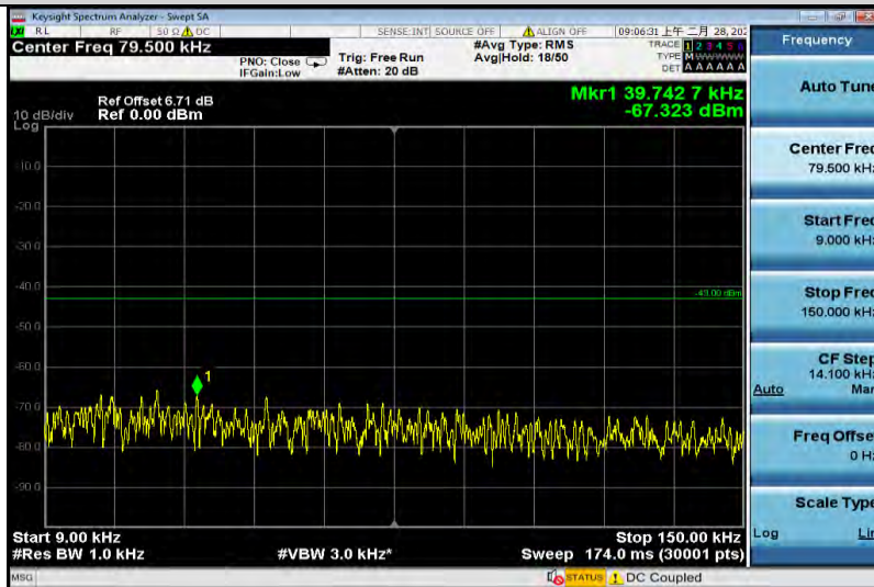
EGPRS1900-512-0.009~0.15
