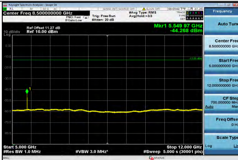
GPRS1900-512-5000~12000
