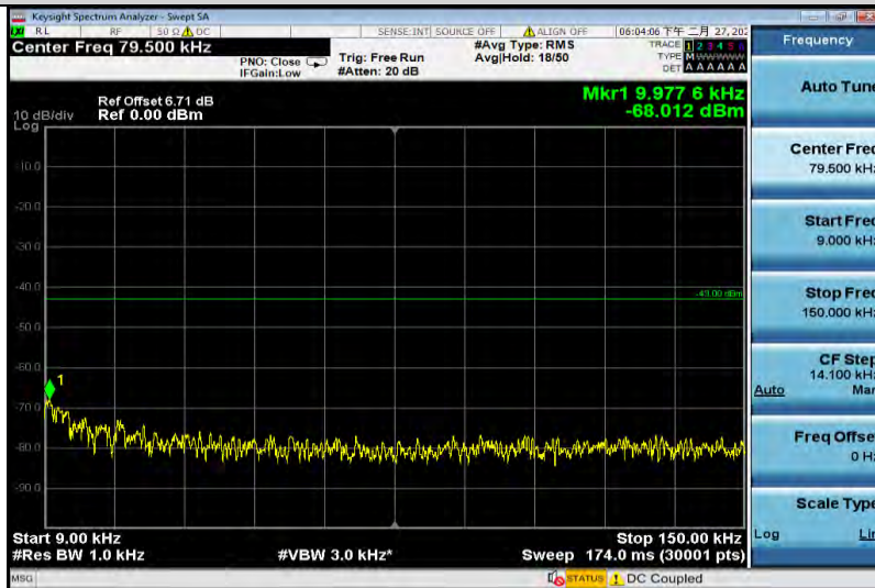
GPRS1900-512-0.009~0.15
