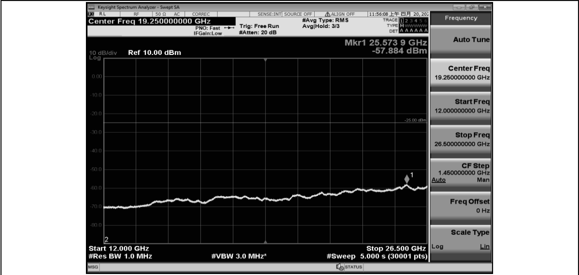
Band41-10MHz-QPSK-40620-1RB#0-Range1:30~1000MHz
