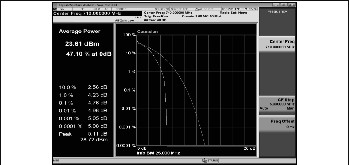
Band17-5MHz-QPSK-23790-25RB#0
