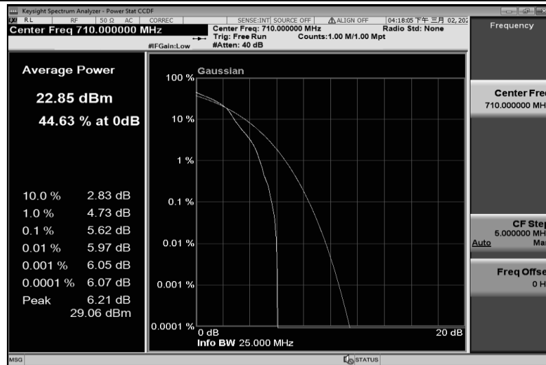
Band17-10MHz-16QAM-23790-50RB#0
