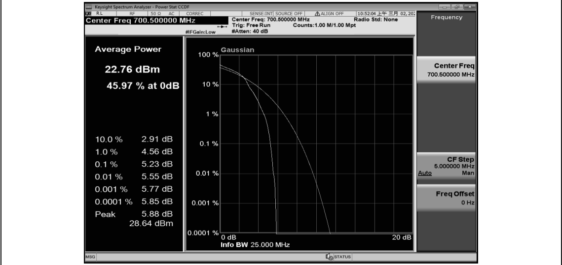
Band12-3MHz-16QAM-23025-15RB#0
