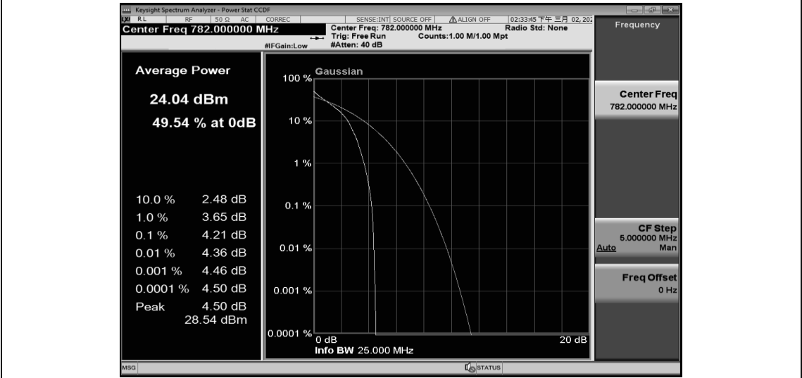
Band13-10MHz-QPSK-23230-50RB#0
