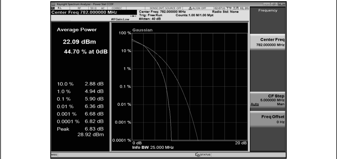
Band13-5MHz-16QAM-23255-1RB#0
