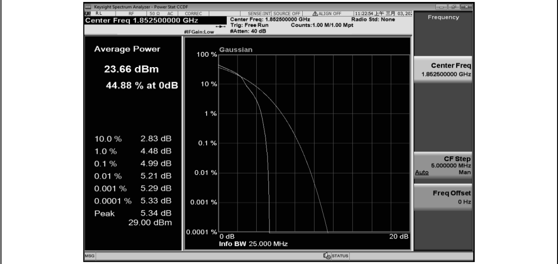
Band25-5MHz-16QAM-26065-25RB#0
