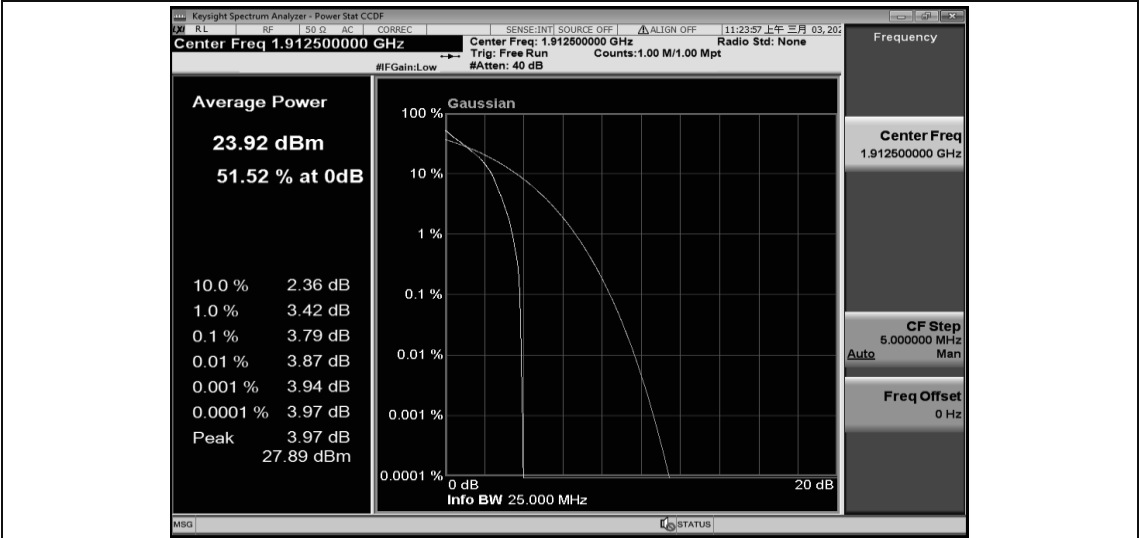
Band25-5MHz-QPSK-26665-25RB#0
