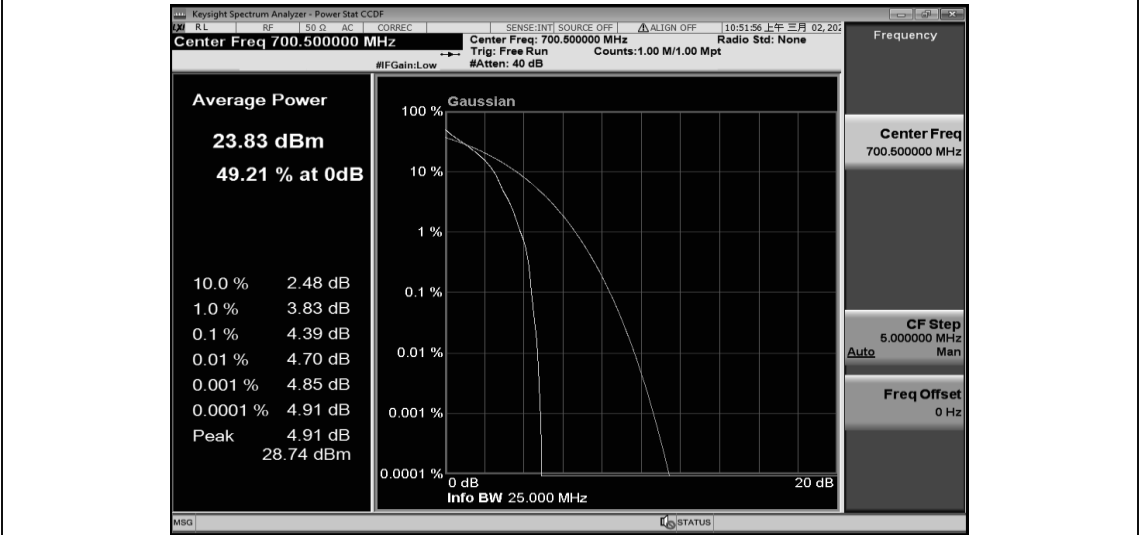
Band12-3MHz-QPSK-23025-15RB#0
