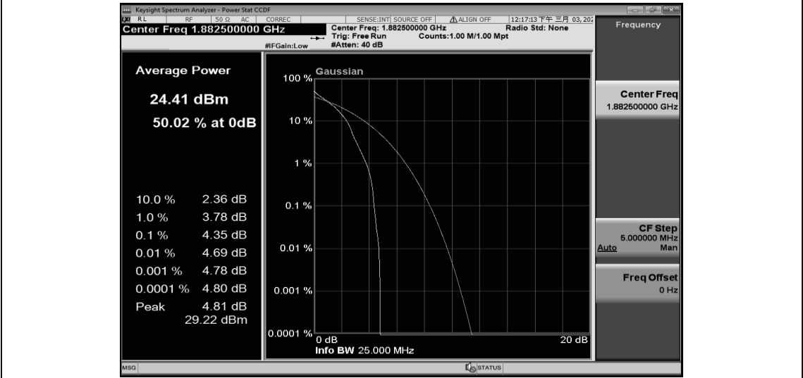
Band25-15MHz-QPSK-26365-75RB#0
