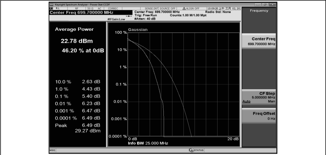
Band12-1.4MHz-QPSK-23095-1RB#0
