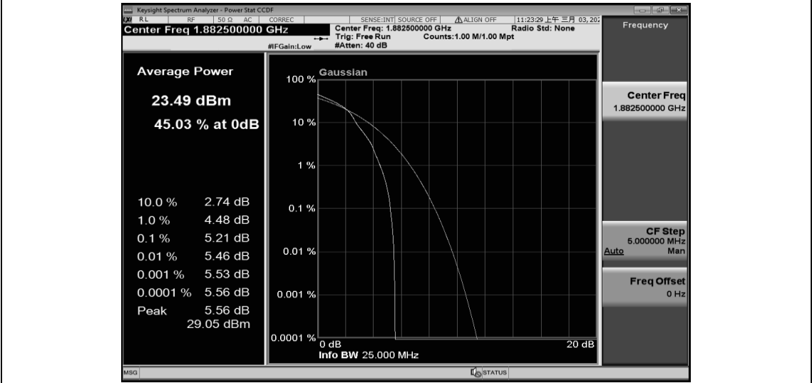
Band25-5MHz-16QAM-26365-25RB#0
