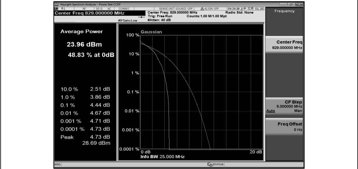
Band5-10MHz-QPSK-20450-50RB#0
