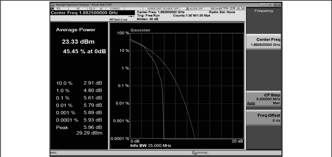
Band25-1.4MHz-16QAM-26365-6RB#0
