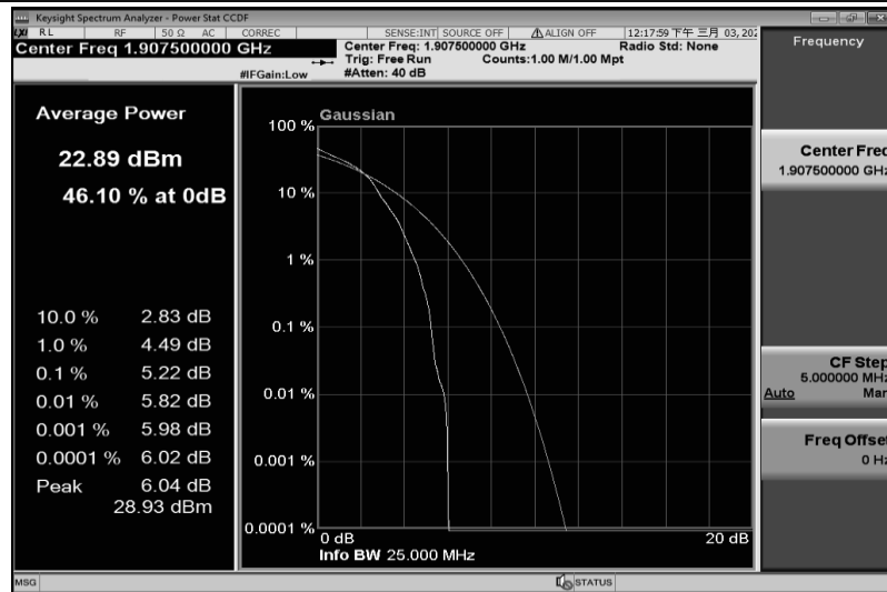
Band25-15MHz-16QAM-26615-75RB#0
