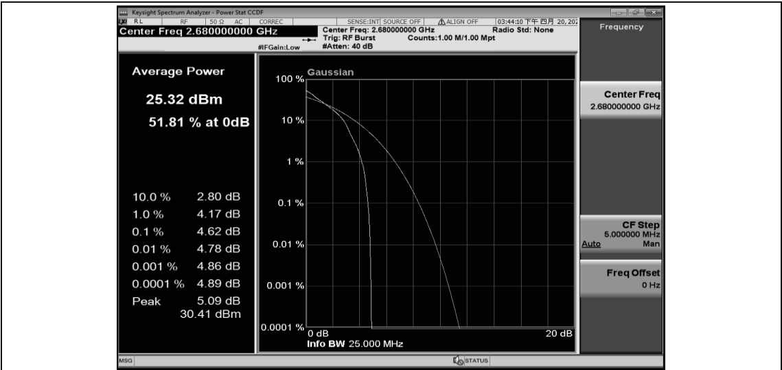
Band41-20MHz-QPSK-41490-100RB#0
