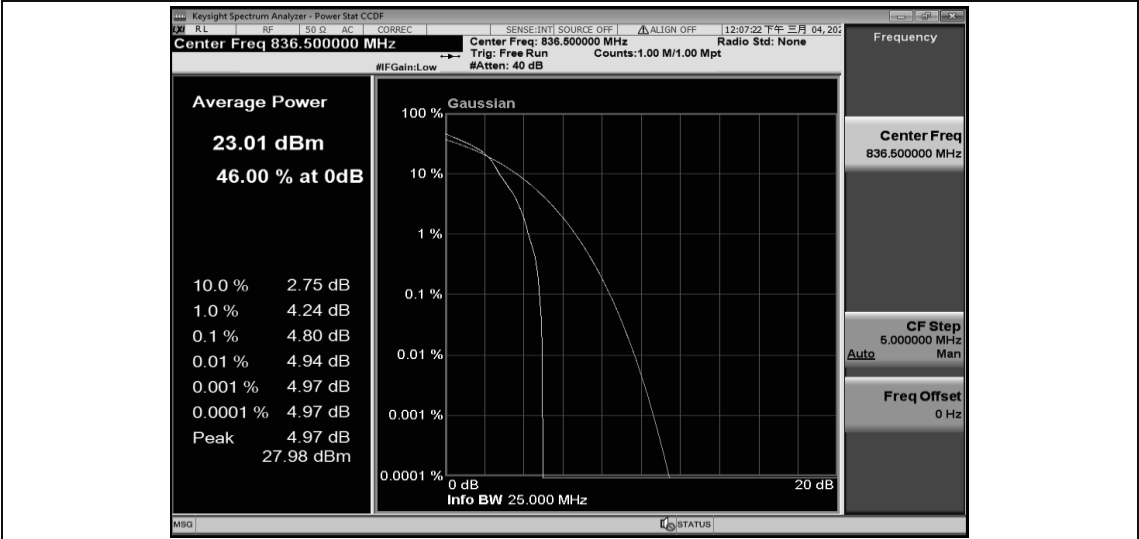
Band26-10MHz-16QAM-26915-50RB#0
