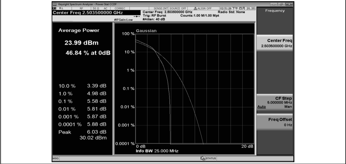
Band41-15MHz-16QAM-39725-75RB#0
