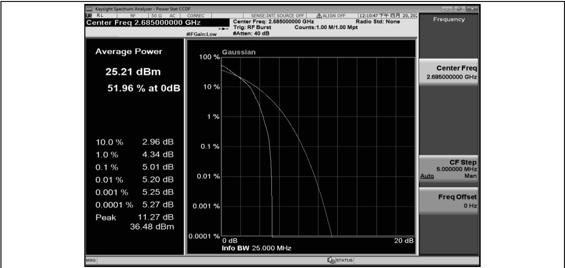
Band41-10MHz-QPSK-41540-50RB#0
