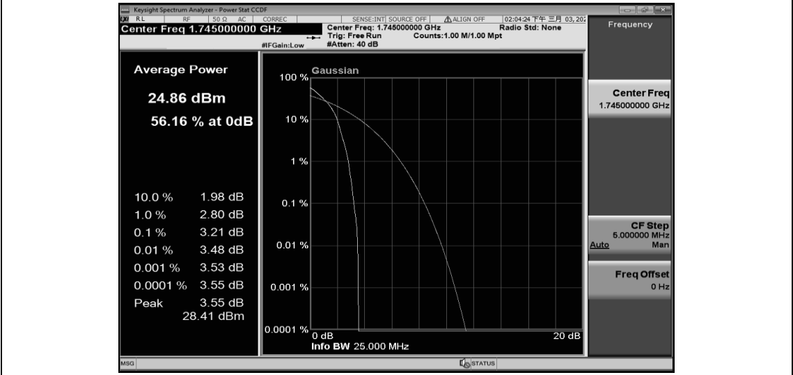
Band66-1.4MHz-QPSK-132322-6RB#0
