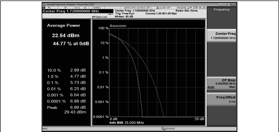
Band66-20MHz-16QAM-132322-1RB#0
