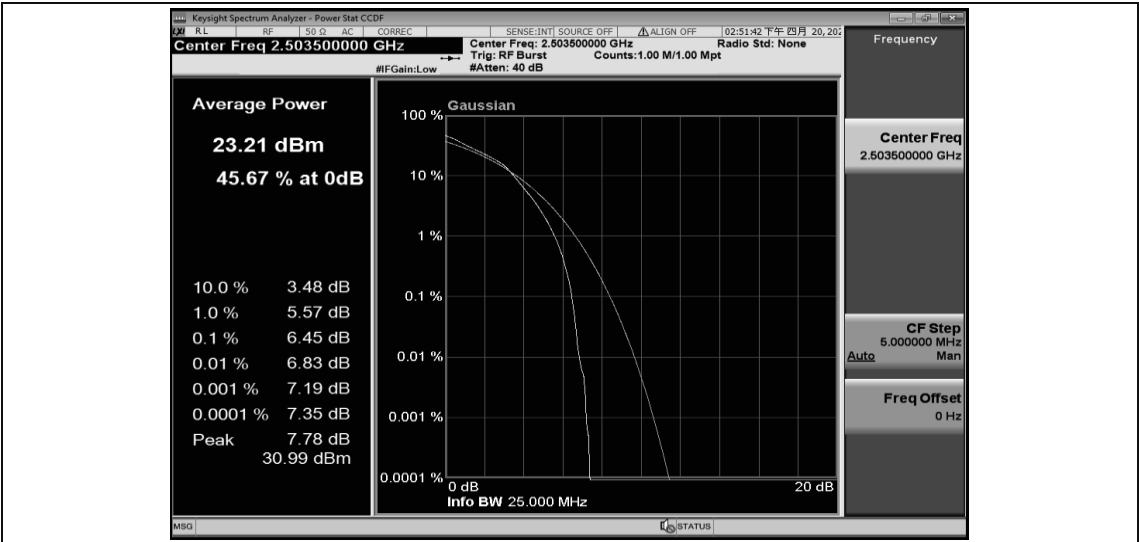
Band41-15MHz-16QAM-40620-1RB#0
