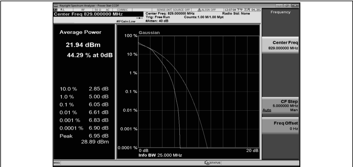
Band26-10MHz-16QAM-26915-1RB#0
