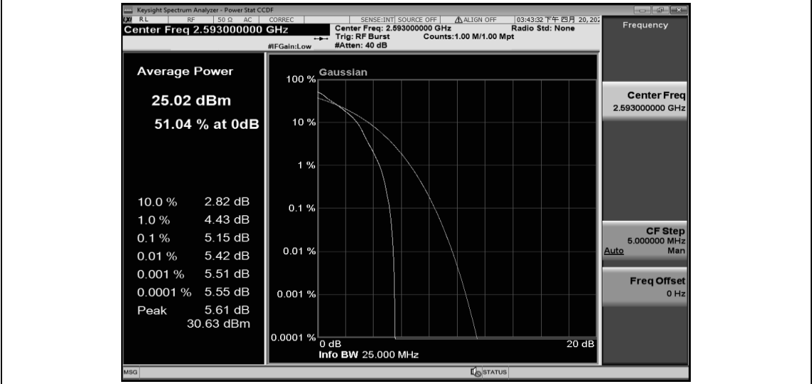
Band41-20MHz-QPSK-40620-100RB#0
