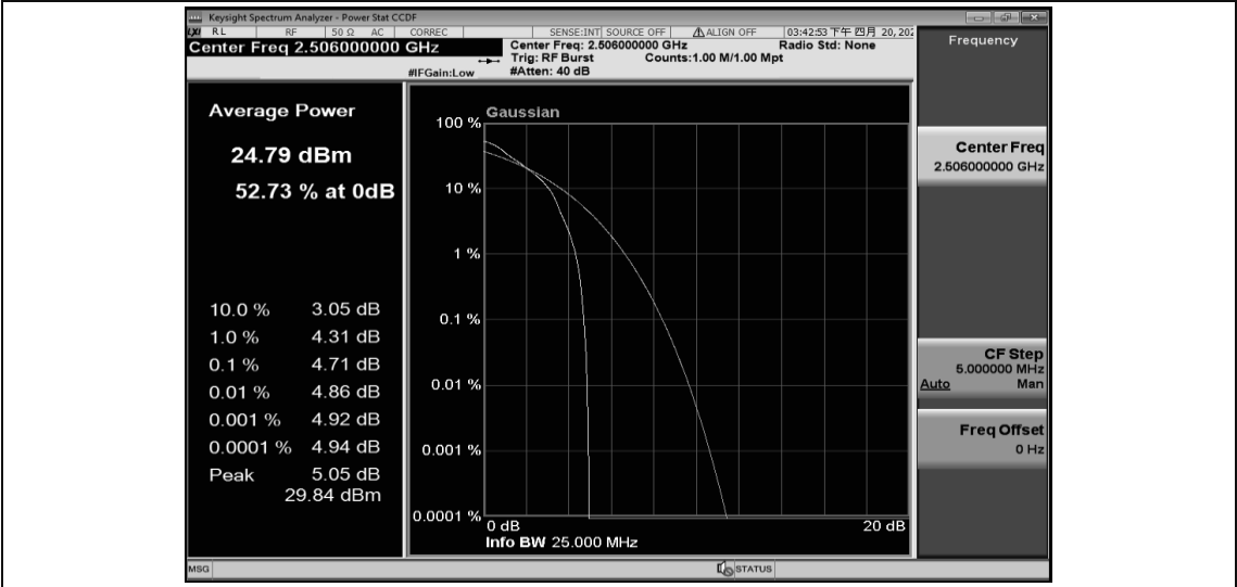
Band41-20MHz-QPSK-39750-100RB#0
