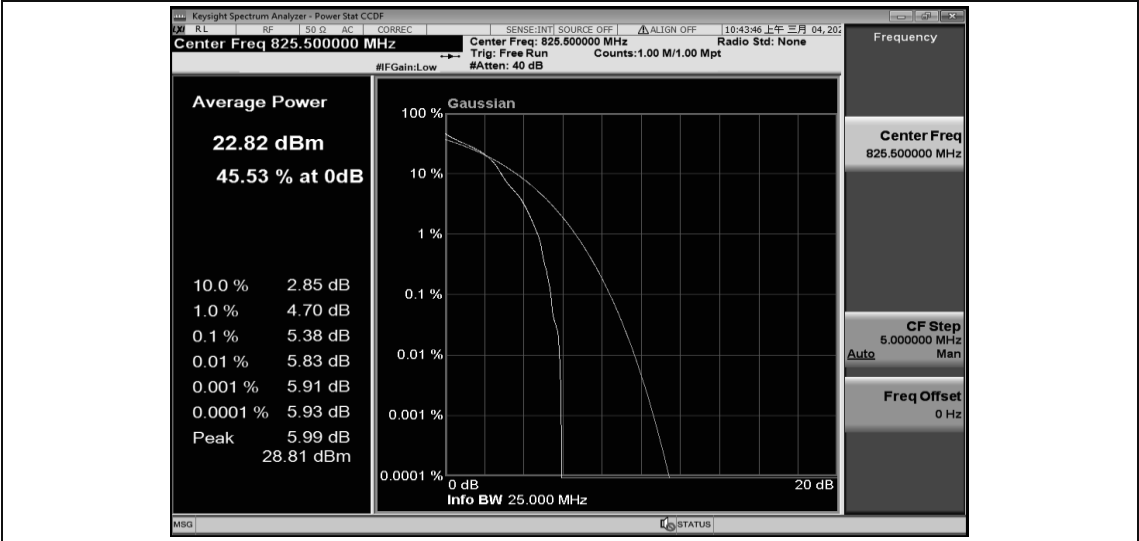
Band26-3MHz-16QAM-26805-15RB#0
