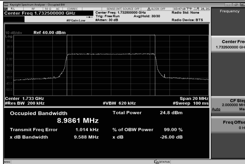
Band4-10MHz-QPSK-20350-50RB#0-8.9913
