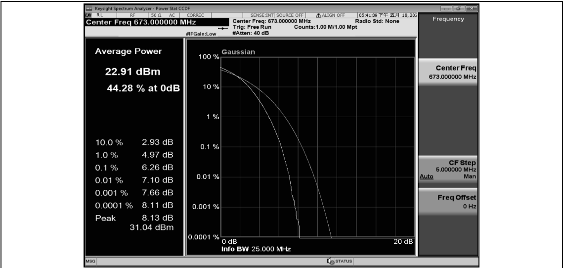
Band71-20MHz-16QAM-133322-1RB#0
