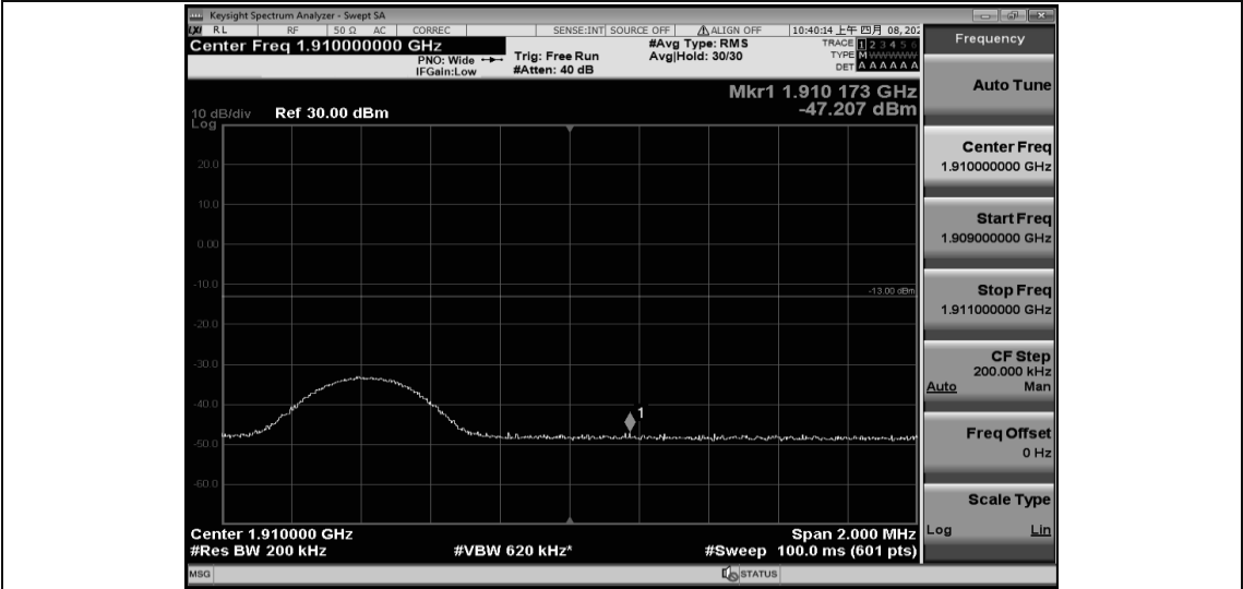
Band2-10MHz-QPSK-19150-1RB#49
