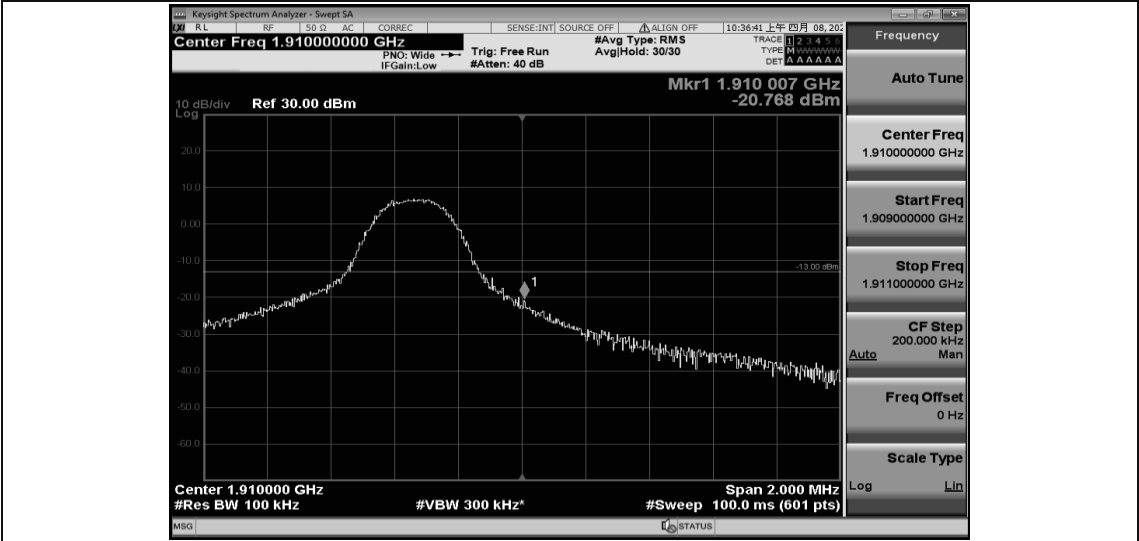
Band2-5MHz-16QAM-19175-25RB#0
