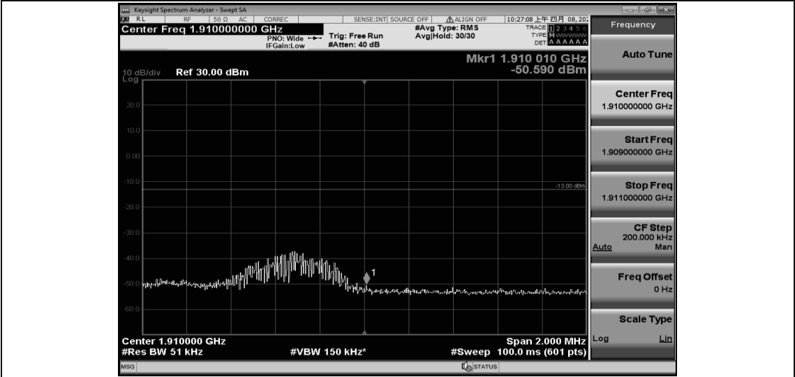
Band2-3MHz-16QAM-19185-15RB#0
