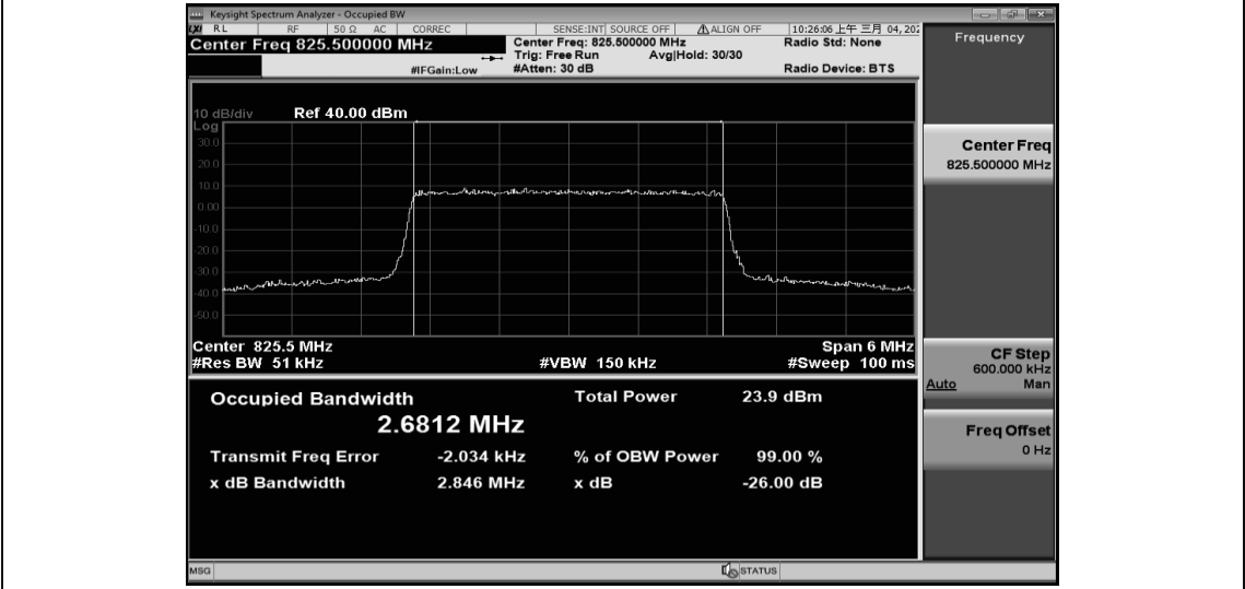
Band26-3MHz-16QAM-26915-15RB#0-2.6899
