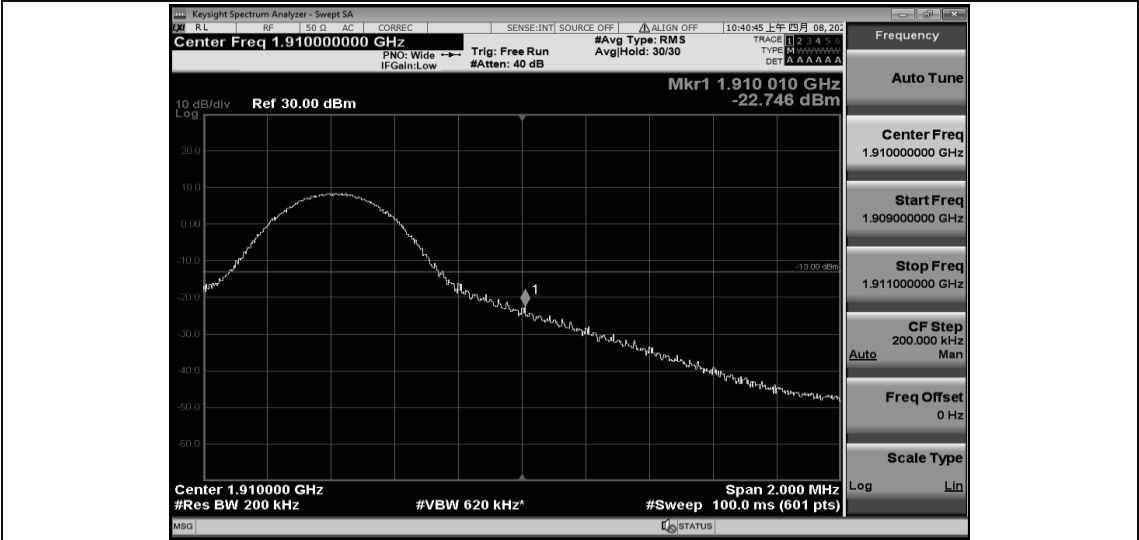
Band2-10MHz-16QAM-19150-1RB#0
