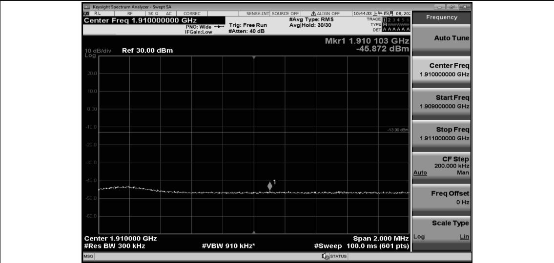
Band2-15MHz-QPSK-19125-1RB#74
