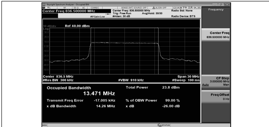
Band26-15MHz-QPSK-26965-75RB#0-13.470
