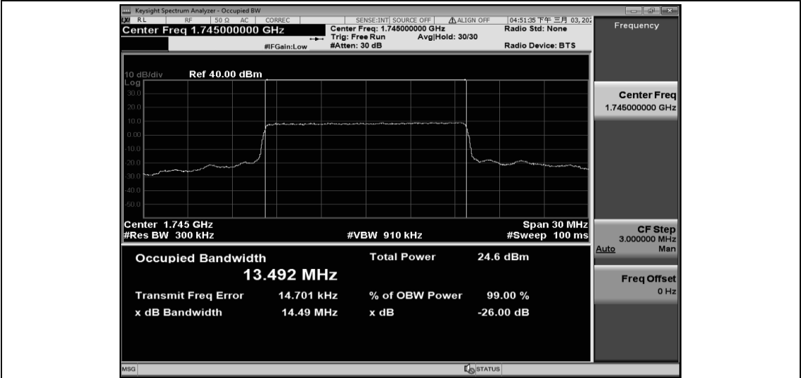
Band66-15MHz-QPSK-132597-75RB#0-13.500
