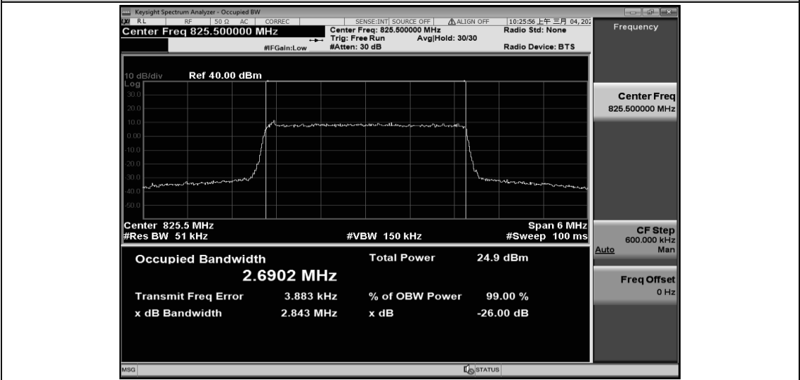
Band26-3MHz-QPSK-26915-15RB#0-2.6900
