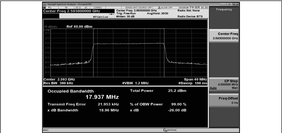
Band41-20MHz-QPSK-41490-100RB#0-17.945
